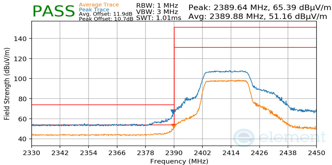
Plot 7-76. Radiated Restricted Lower Band Edge Measurement
