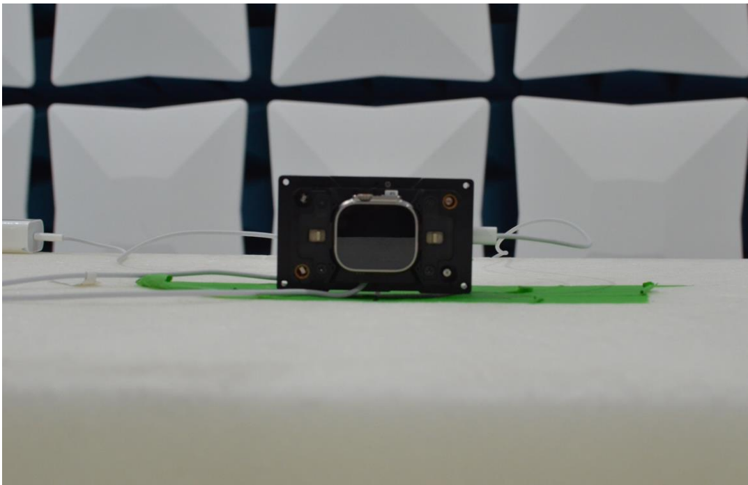
Figure 8: 1-18GHz Test Setup (Front View)
