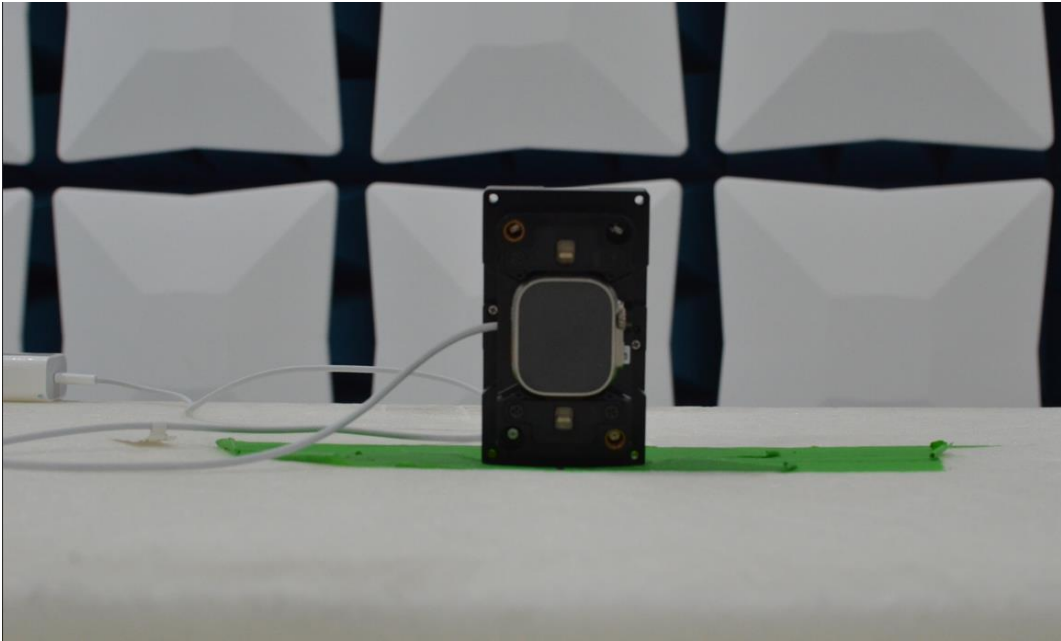
Figure 10: 1-18GHz Test Setup (Front View)
