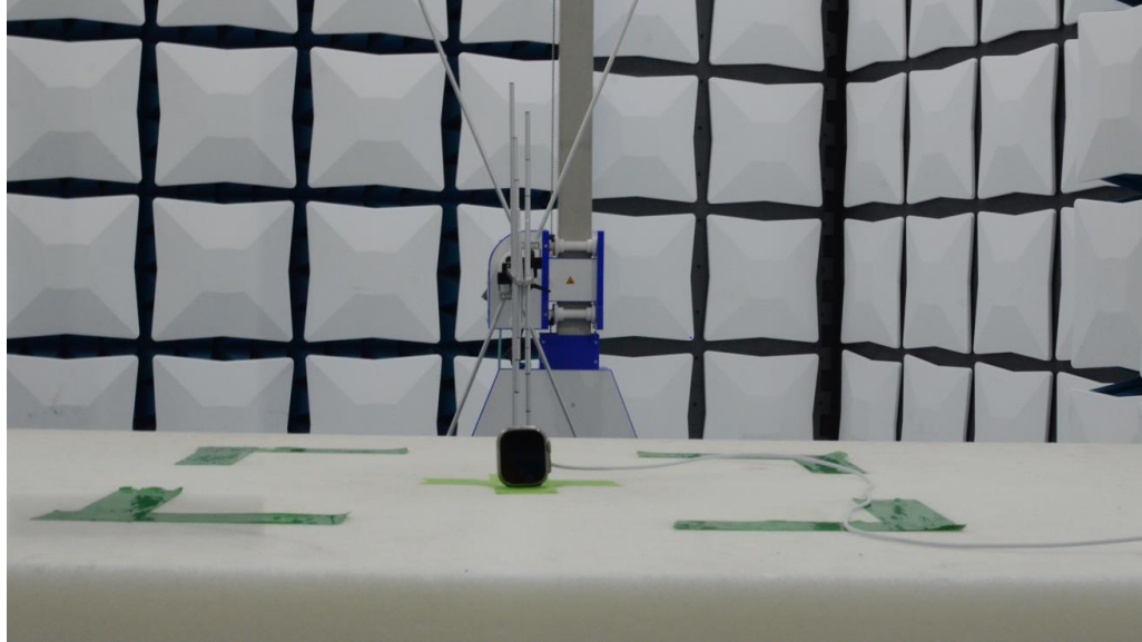
Figure 13: 30MHz-1GHz Test Setup (Rear View)
