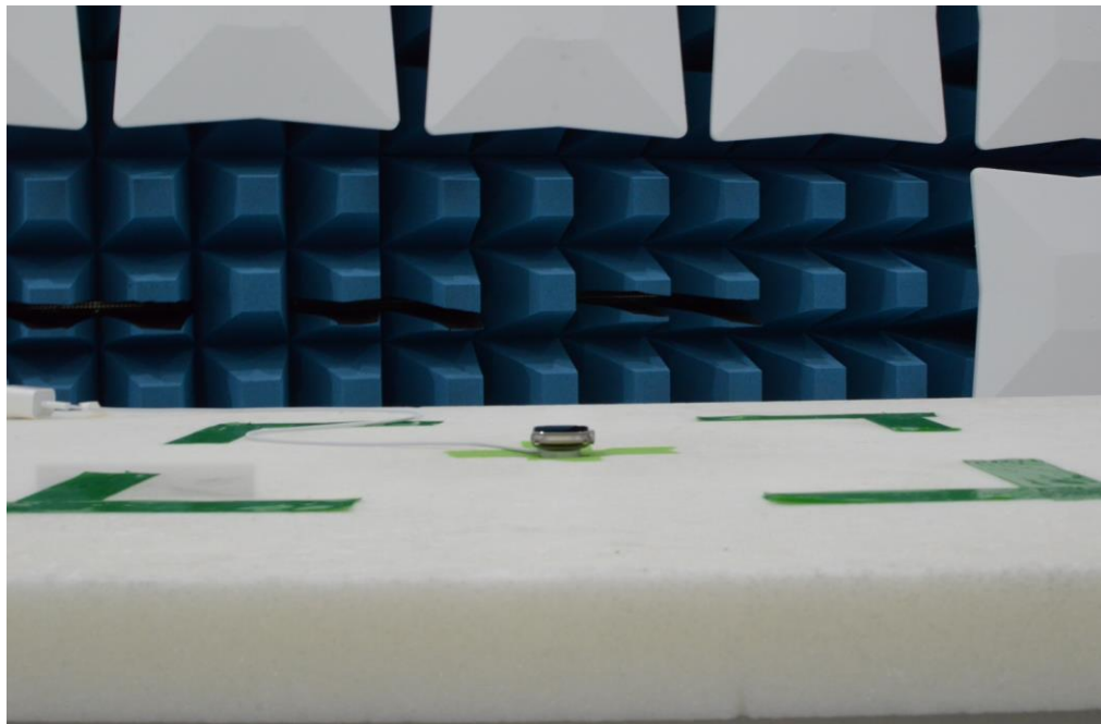
Figure 8: 30MHz-1GHz Test Setup (Front View)
