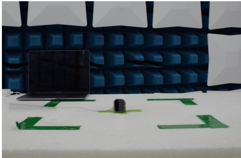
Figure 18: 30MHz-1GHz Test Setup (Front View)
