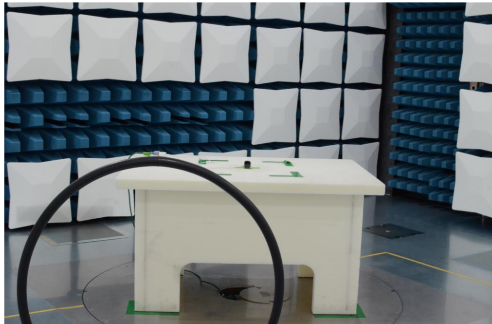
Figure 22: 9kHz-30MHz Test Setup (Front View)
