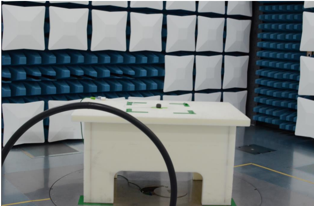
Figure 24: 9kHz-30MHz Test Setup (Front View)
