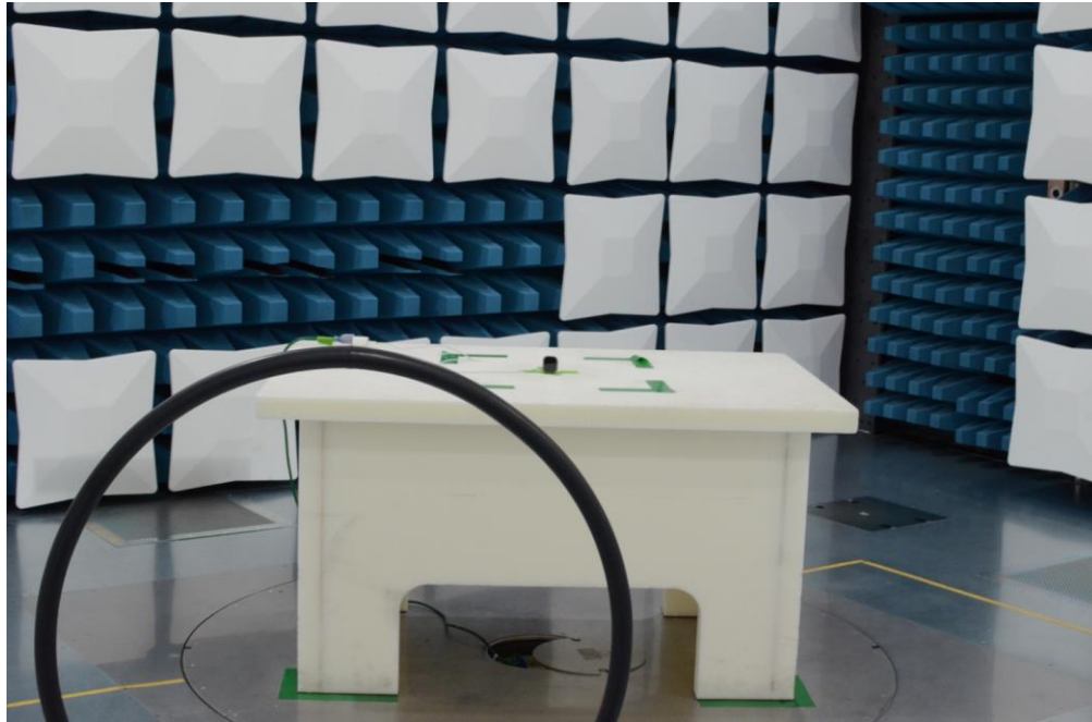
Figure 21: 9kHz-30MHz Test Setup (Front View)
