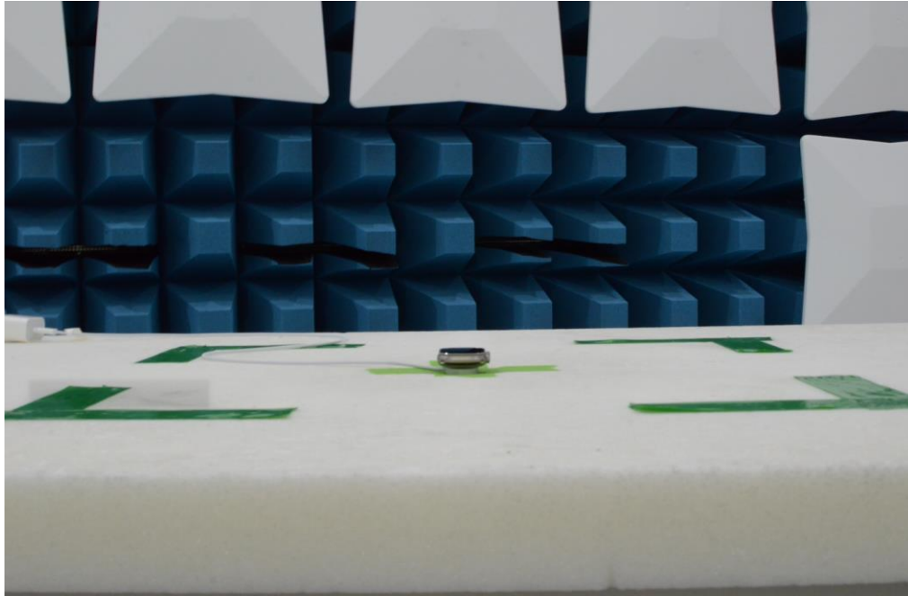
Figure 7: 30MHz-1GHz Test Setup (Front View)
