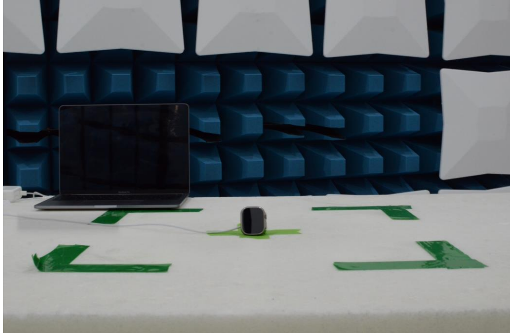
Figure 17: 30MHz-1GHz Test Setup (Front View)
