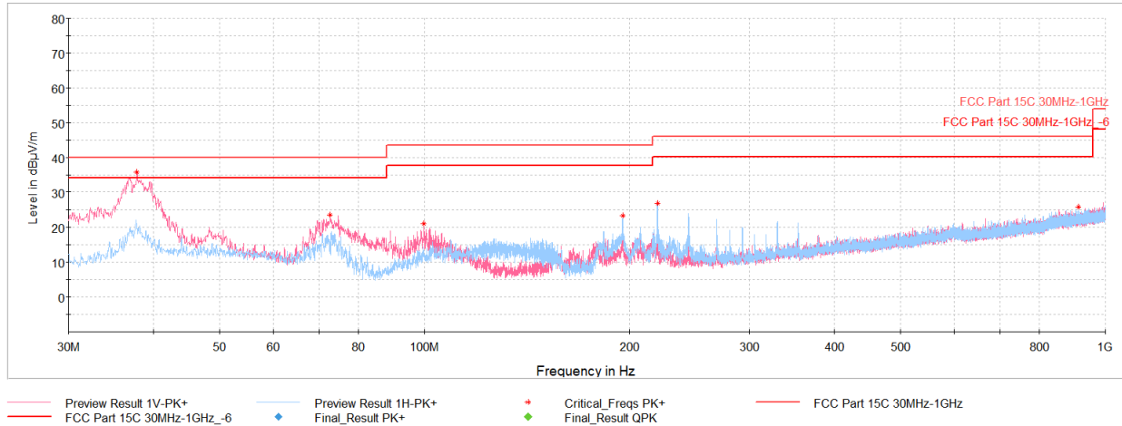
Plot 7-29. RSE 30MHz - 1GHz (O-QPSK – Ch. 24), with AC/DC Adapter & magnetic charger
