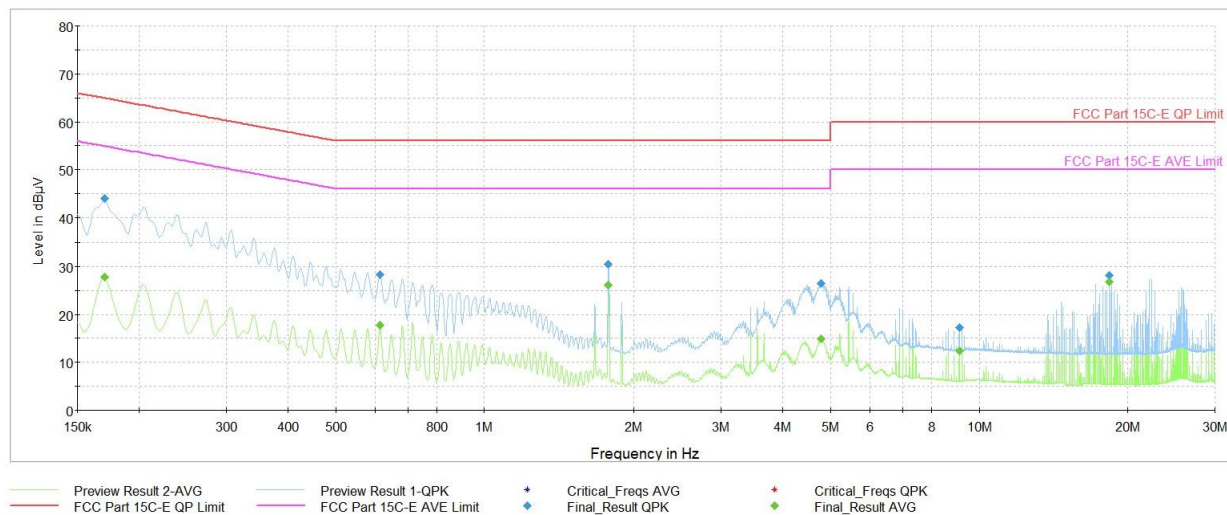
Plot 7-30. AC Line Conducted Plot (O-QPSK – Ch. 24) (L1) with AC/DC Adapter & magnetic charger
