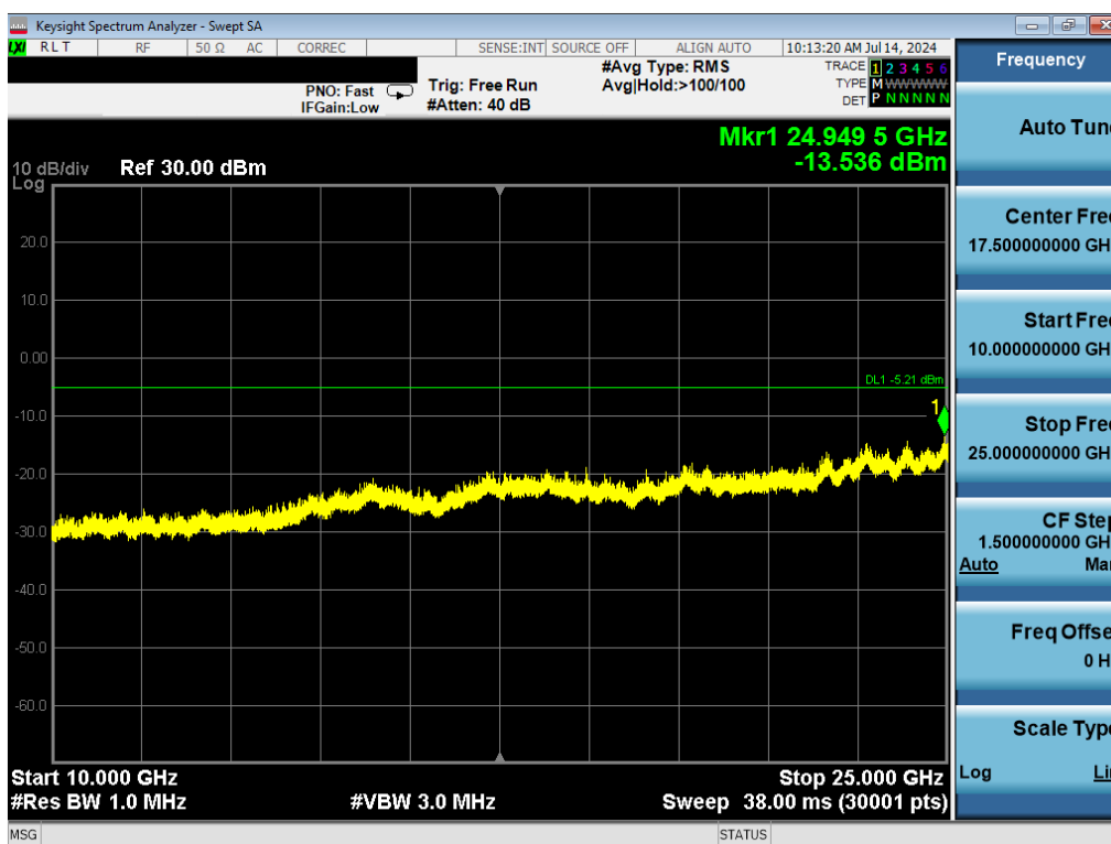
Plot 7-26. Conducted Spurious Plot (Bluetooth (HDR4), ePA – Ch. 38)
