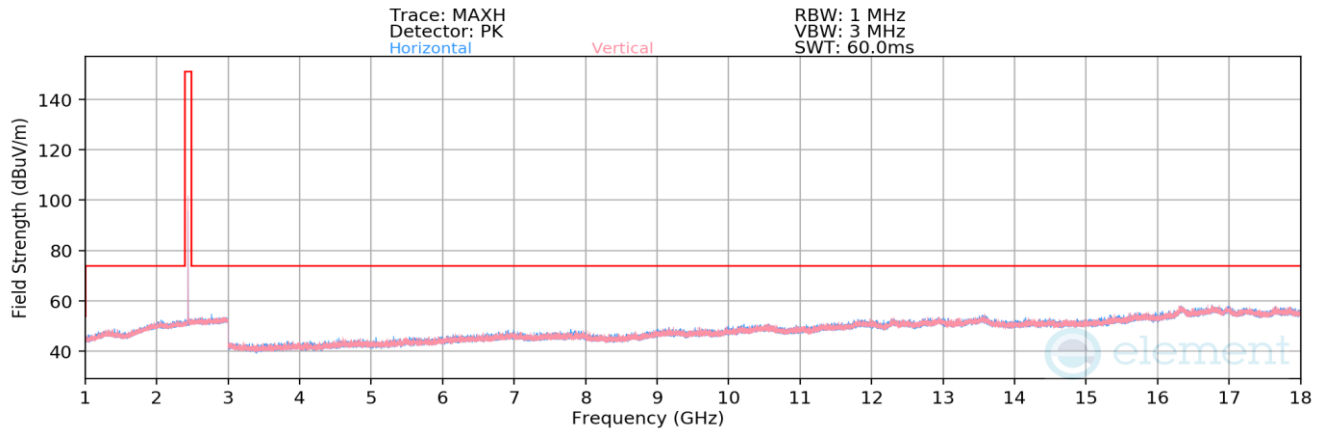
Plot 7-30. Radiated Spurious Emissions 1-18GHz (4Mbps, HDR4, ePA – Ch. 38)
