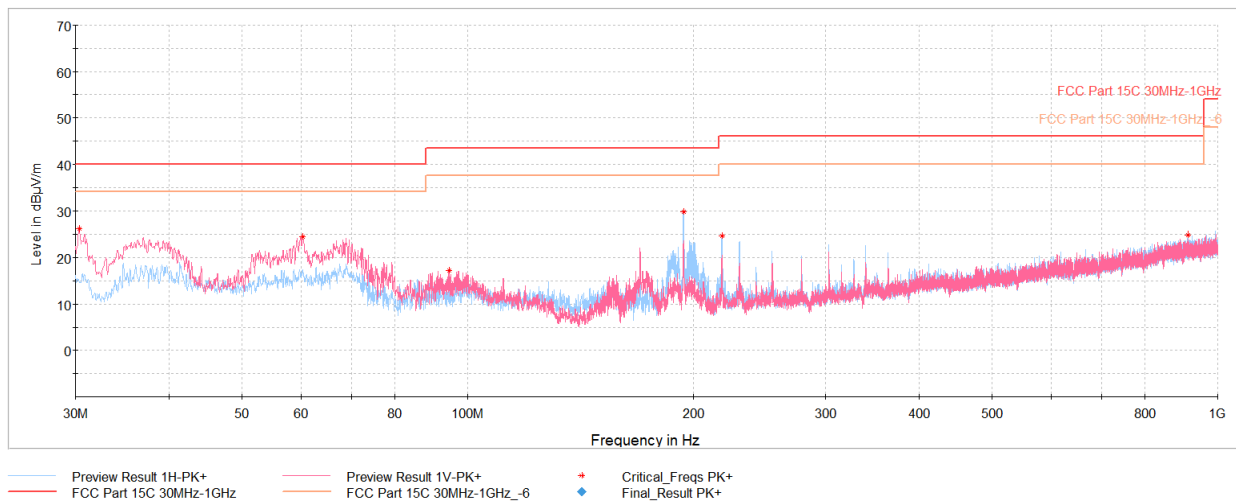
Plot 7-37. Radiated Spurious Emissions Below 1GHz (4Mbps, ePA – Ch.38 with AC/DC Adapter + Magnetic Charger)
