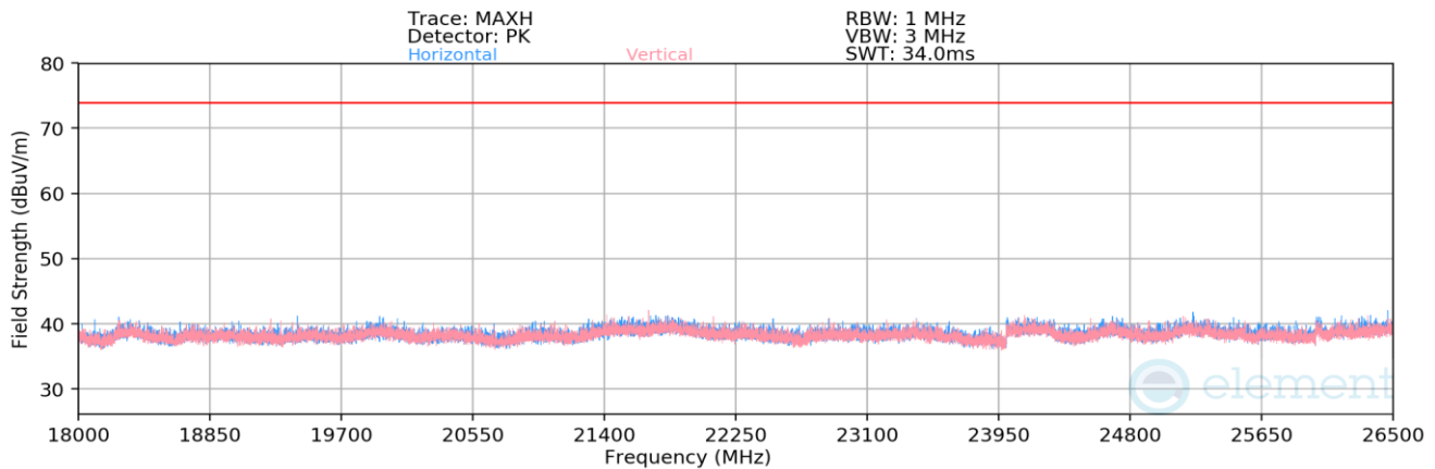
Plot 7-31. Radiated Spurious Emissions Above 18GHz (4Mbps, HDR4, ePA – Ch. 38)
