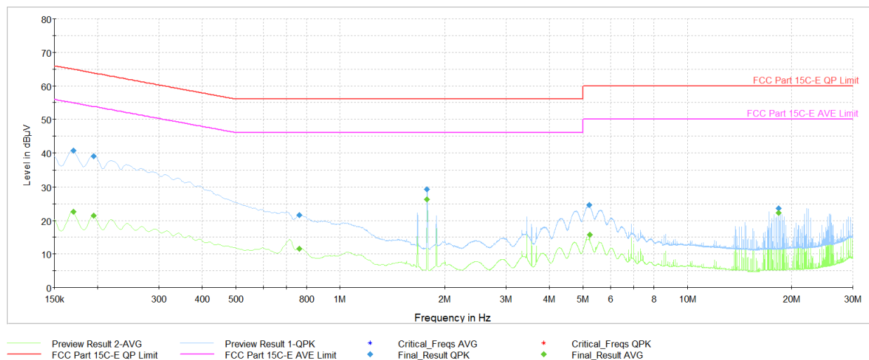
Plot 7-38. AC Line Conducted Plot with Bluetooth HDR (L1, 4Mbps ePA - Ch.38 with AC/DC Adapter + Magnetic Charger)
