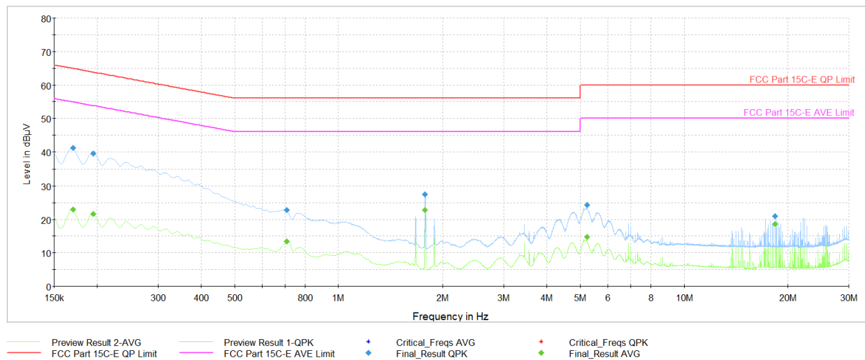
Plot 7-39. AC Line Conducted Plot with Bluetooth HDR (N, 4Mbps ePA - Ch.38 with AC/DC Adapter + Magnetic Charger)
