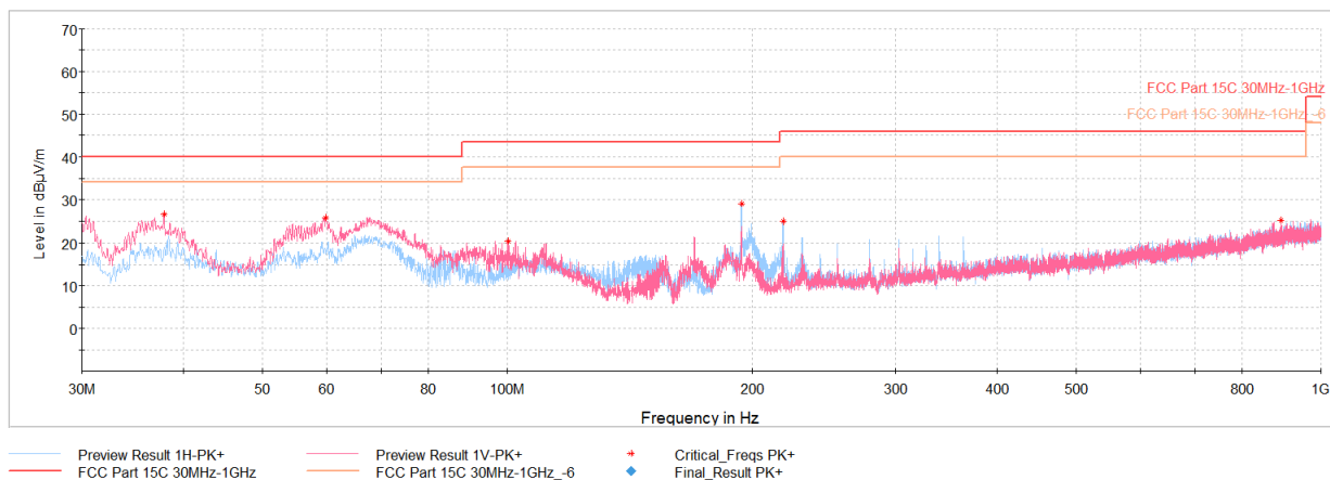
Plot 7-37. Radiated Spurious Emissions Below 1GHz (1Mbps, ePA – Ch.19, Pol. H & V, with AC/DC Adapter + Magnetic Charger)
