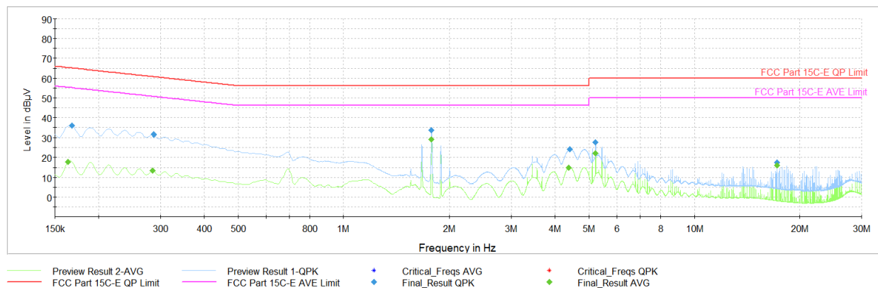
Plot 7-38. AC Line Conducted Plot with Bluetooth LE (L1, 1Mbps ePA – Ch.19 with AC/DC Adapter + Magnetic Charger)
