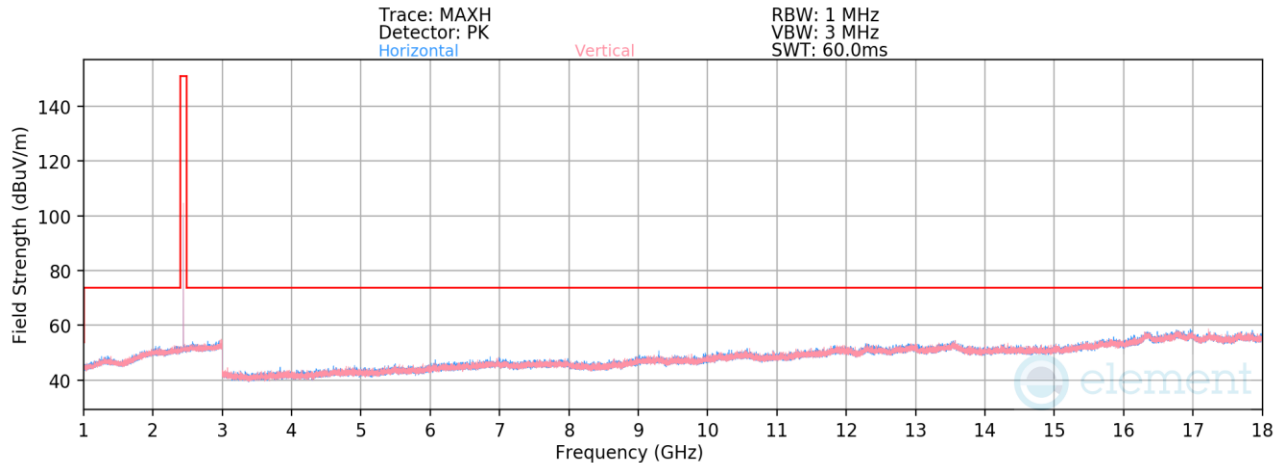
Plot 7-30. Radiated Spurious Emissions 1-18GHz (1Mbps, ePA – Ch. 19)
