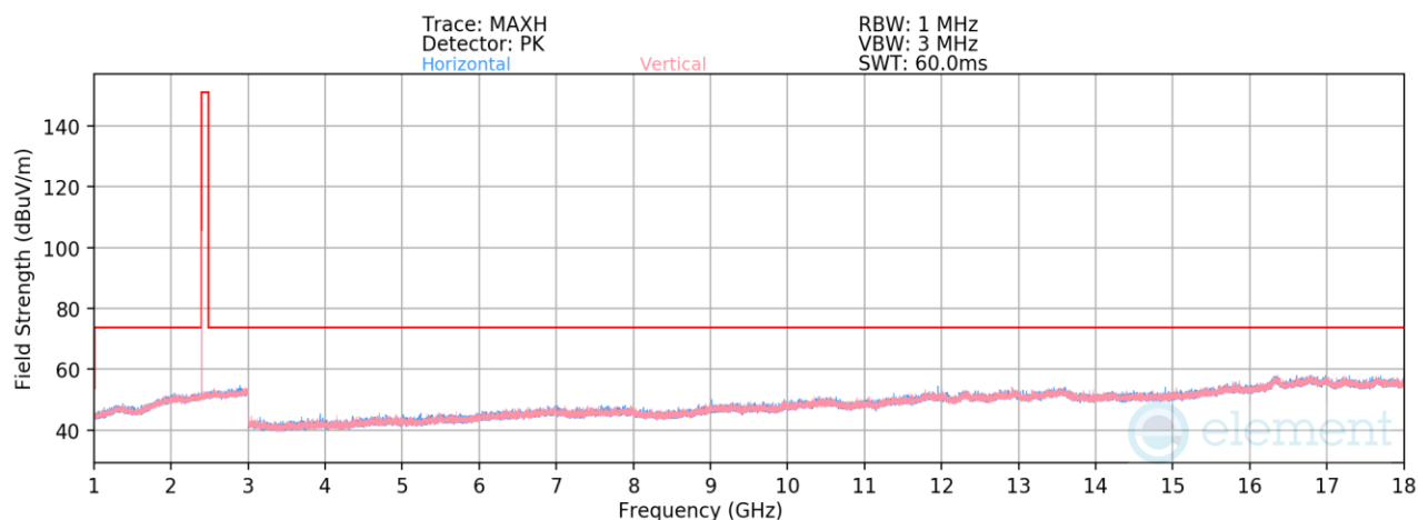
Plot 7-29. Radiated Spurious Emissions 1-18GHz (1Mbps, ePA – Ch. 0)
