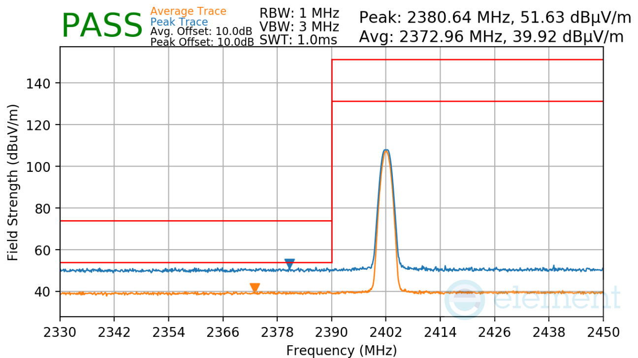
Plot 7-33. Radiated Restricted Lower Band Edge Measurement (Average & Peak)
