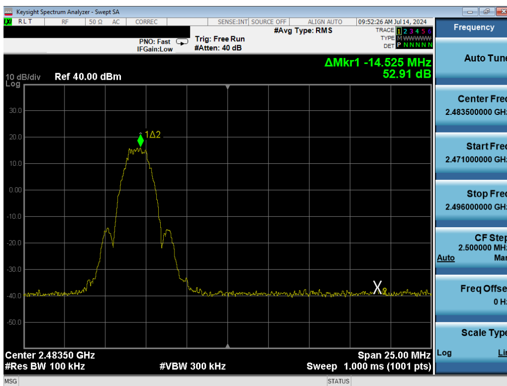
Plot 7-22. Band Edge Plot (Bluetooth (LE), 2Mbps, ePA – Ch. 38)
