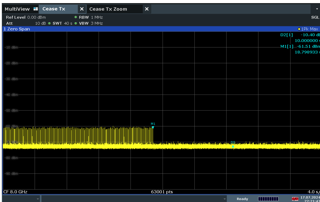
Plot 7-12. Cessation Time – Mode1 (Ch. 9, 8 GHz)
