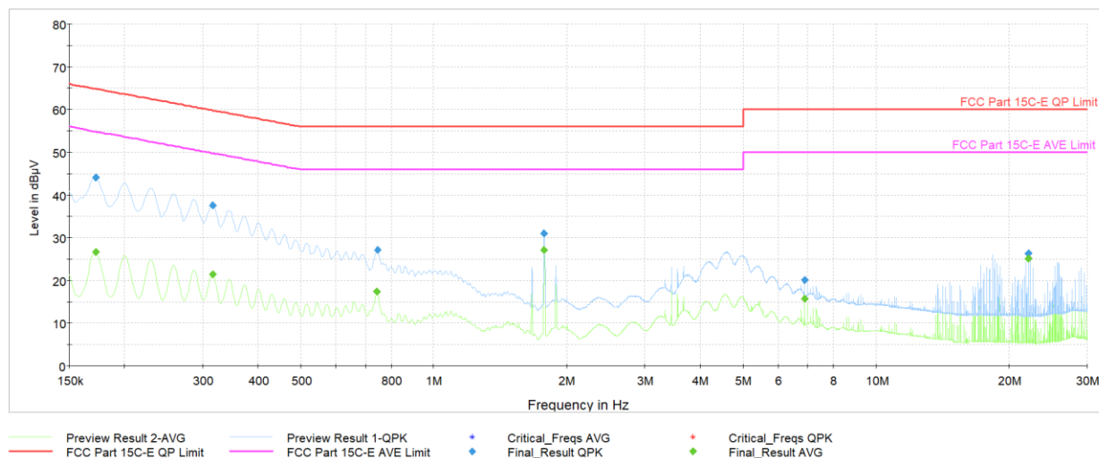
Plot 7-43. AC Line Conducted (Ch. 9, Config 409, Payload 4093 L1, with AC/DC Adapter + Magnetic Charger)
