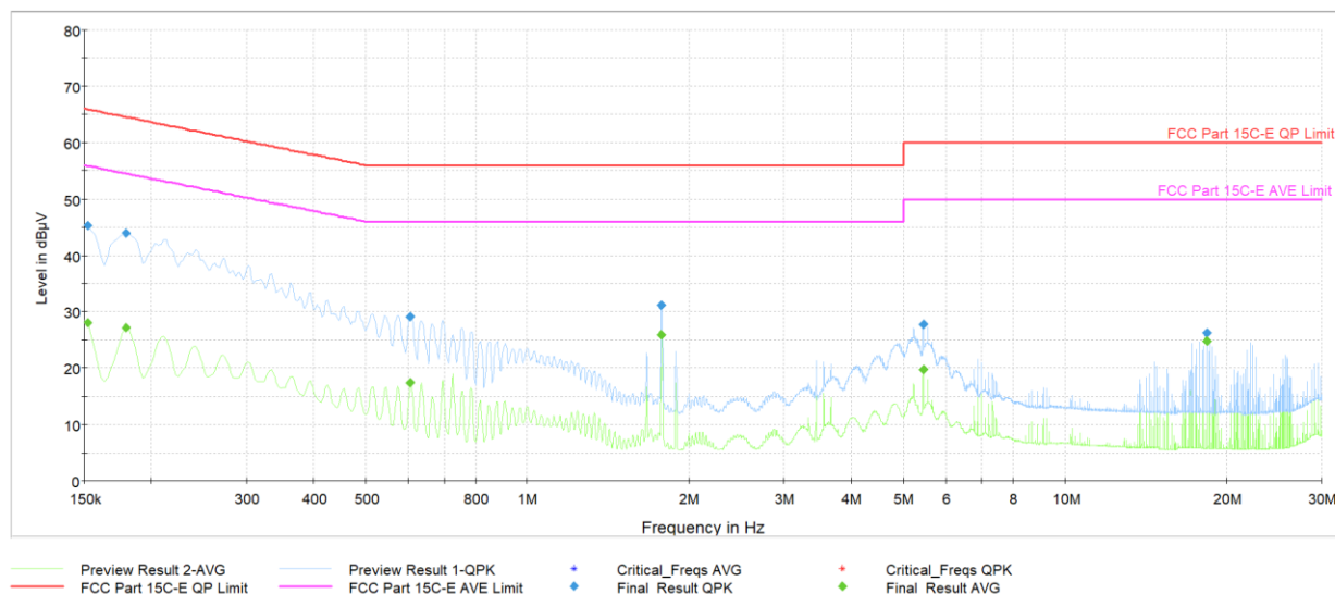
Plot 7-42. AC Line Conducted (Ch. 5, Config 409, Payload 4093 N, with AC/DC Adapter + Magnetic Charger)
