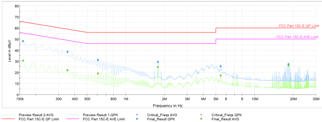
Plot 7-44. AC Line Conducted Plot (Ch. 9, Config 409, Payload 4093 N, with AC/DC Adapter + Magnetic Charger)
