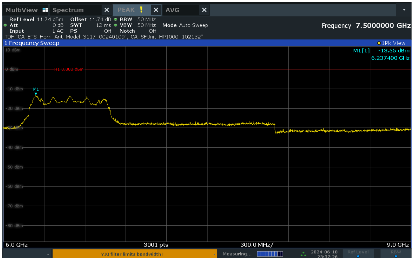
Plot 7-5. Peak Radiated Power (Ch. 5, Config 409/Payload 4093)
