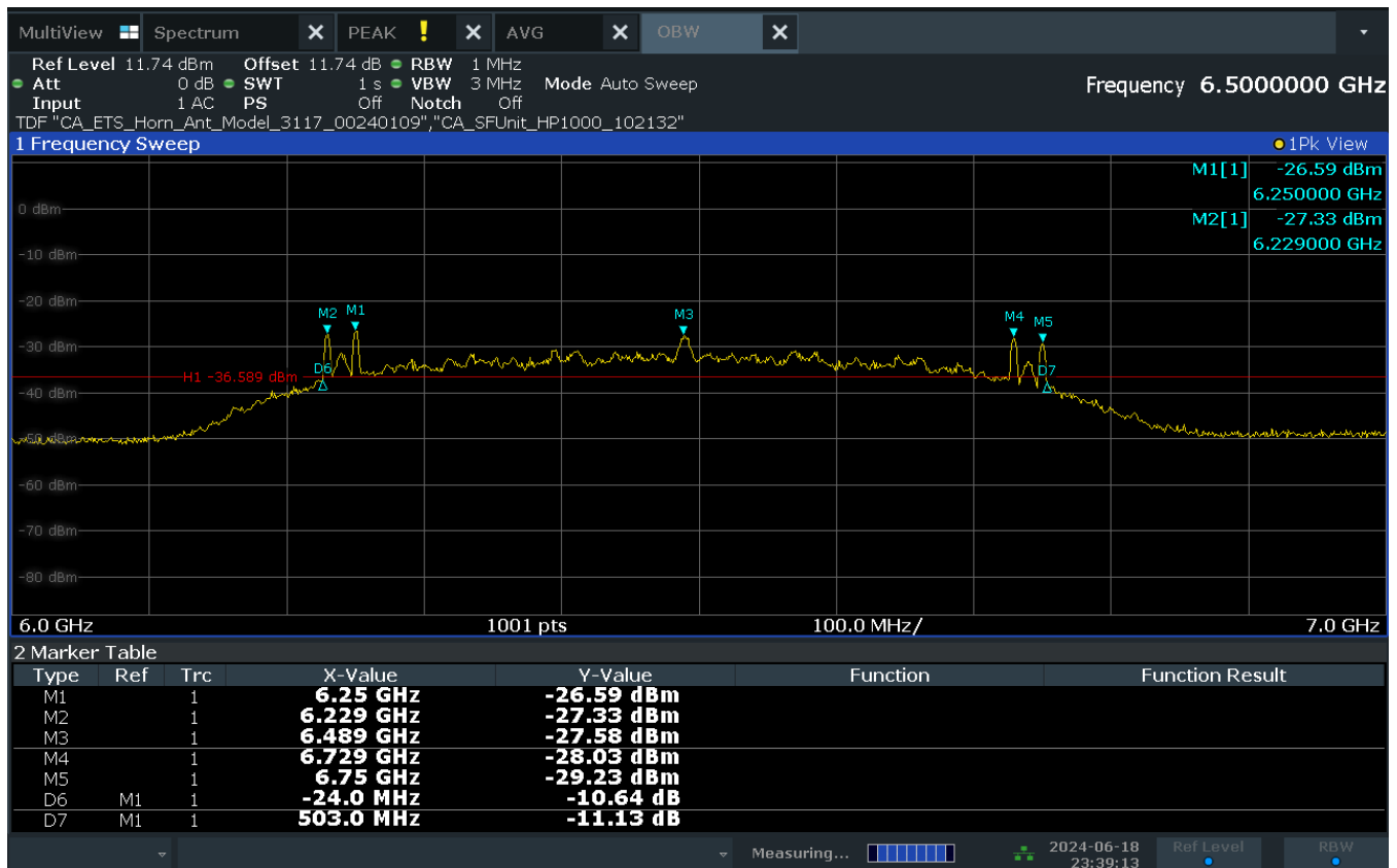
Plot 7-1. 10dBc Bandwidth (Ch. 5, Config 409/Payload 4093)
