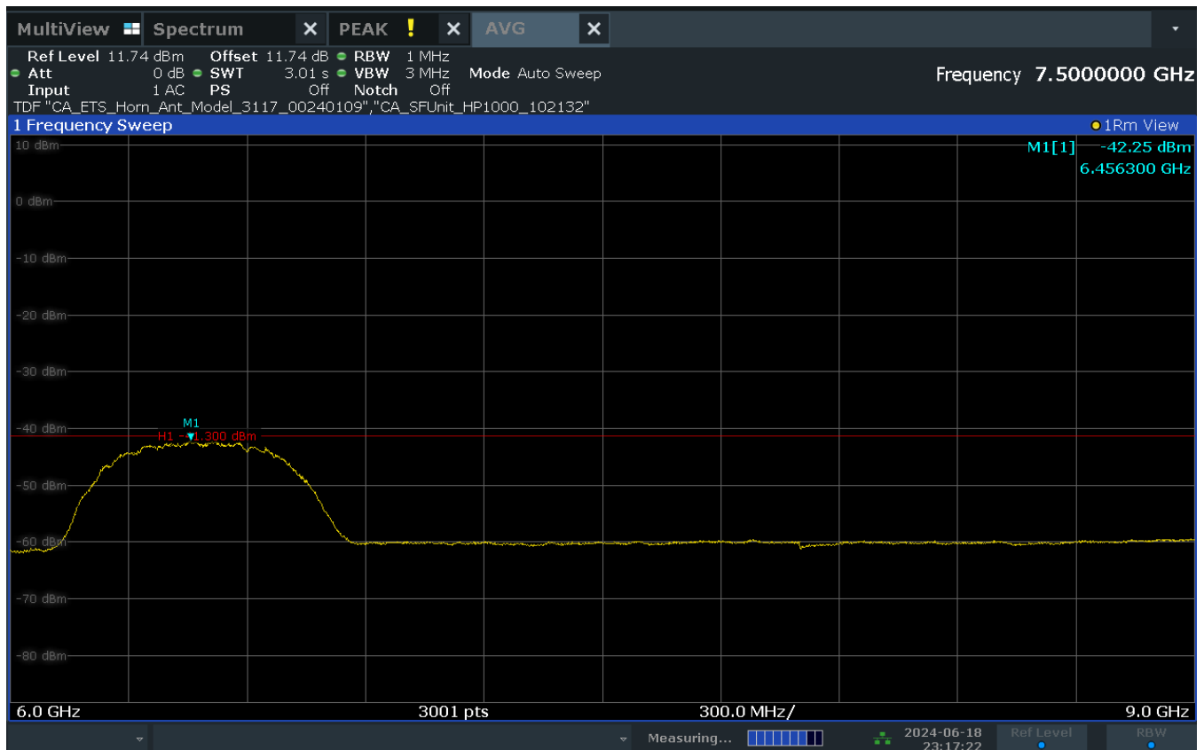
Plot 7-7. Average Radiated Power (Ch. 5, Config 409/Payload 4093)
