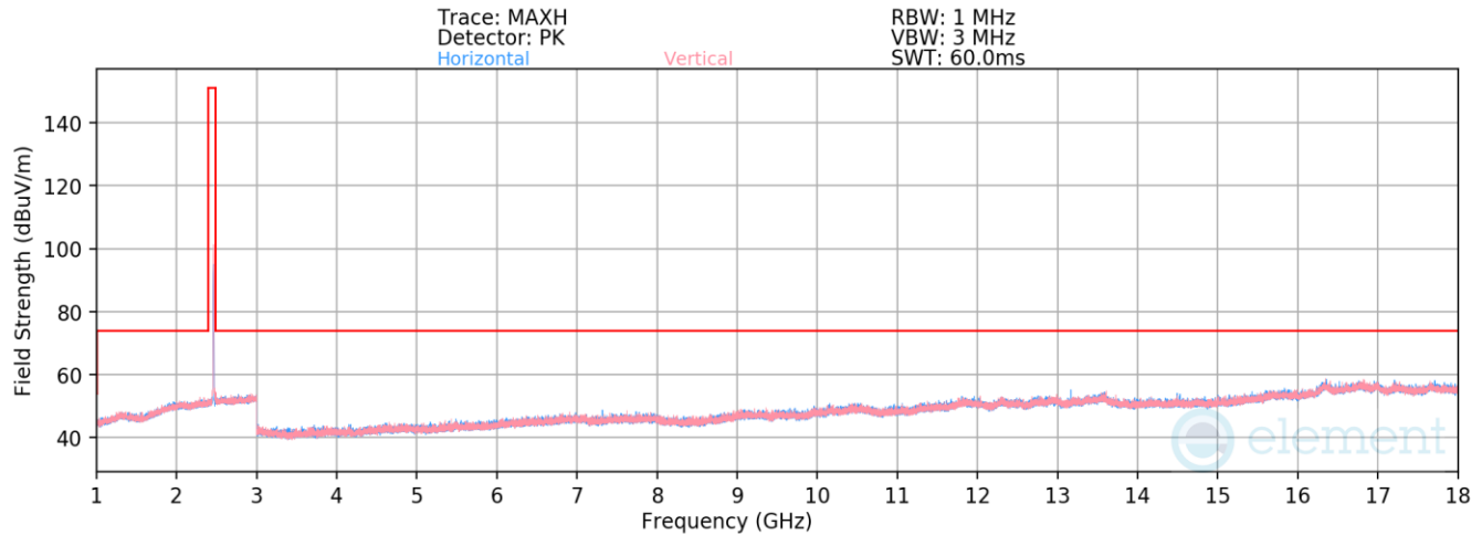
Plot 7-56. Radiated Spurious Emissions above 1GHz (802.11b – Ch. 11)
