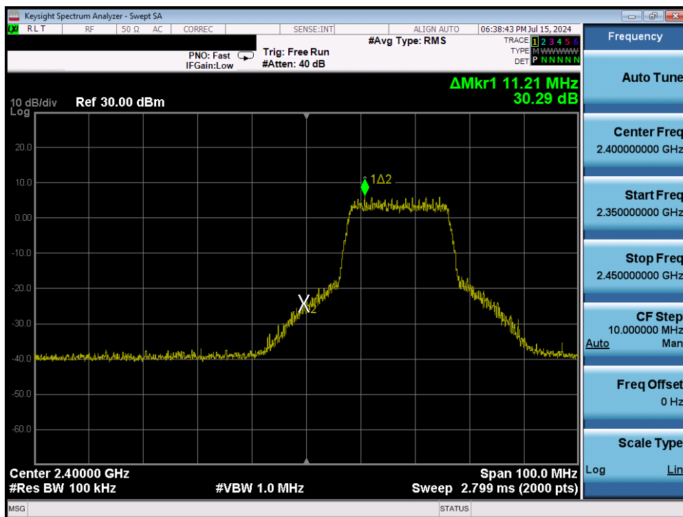
Plot 7-42. Band Edge Plot (802.11n (2.4GHz) – Ch. 2) – MCS7
