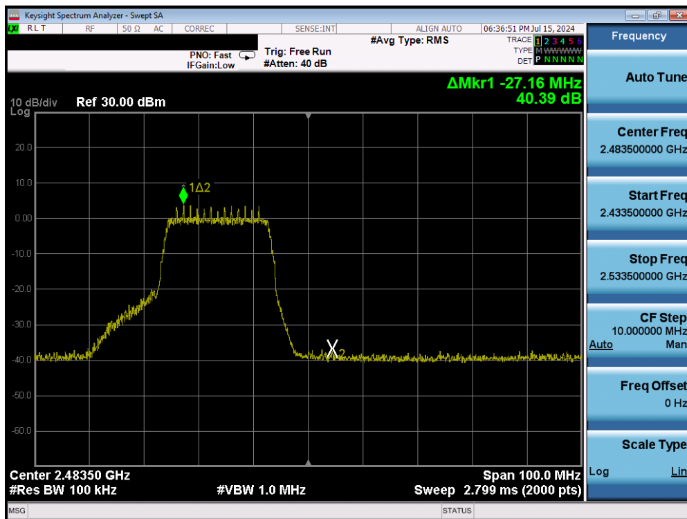
Plot 7-39. Band Edge Plot (802.11n (2.4GHz) – Ch. 12) – MCS0
