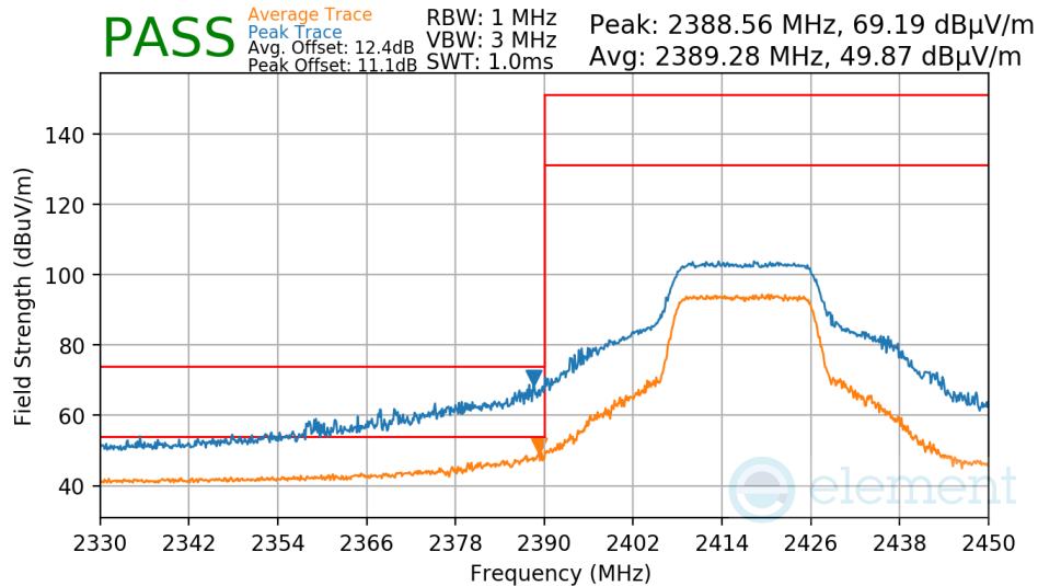
Plot 7-67. Radiated Restricted Lower Band Edge Measurement
