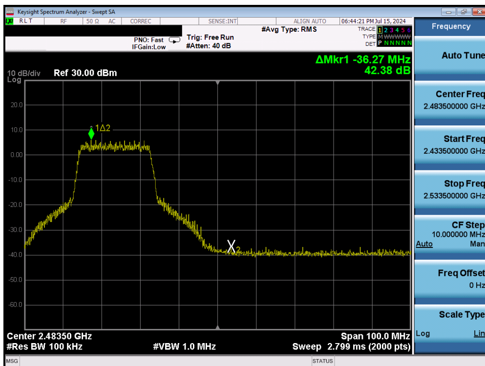
Plot 7-43. Band Edge Plot (802.11n (2.4GHz) – Ch. 10) – MCS7
