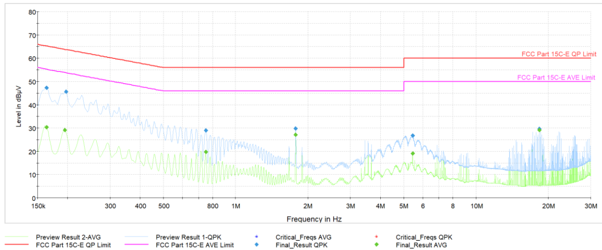
Plot 7-73. AC Line Conducted Plot 802.11b - Ch.6 (L1, with AC/DC Adapter + Magnetic charger)
