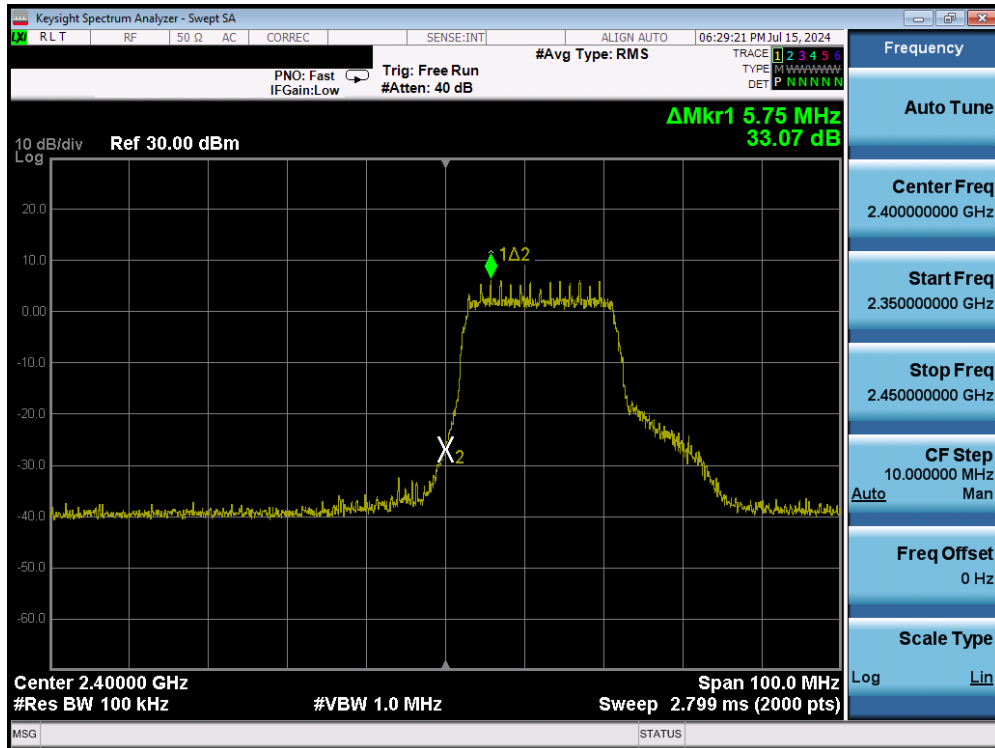
Plot 7-35. Band Edge Plot (802.11n (2.4GHz) – Ch. 1) – MCS0
