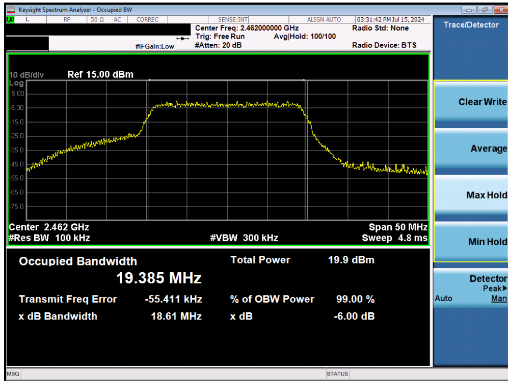
Plot 7-12. 6dB Bandwidth & 99% OBW Plot (802.11n (2.4GHz) – Ch. 11) – MCS7
