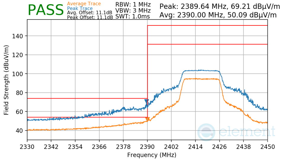
Plot 7-61. Radiated Restricted Lower Band Edge Measurement
