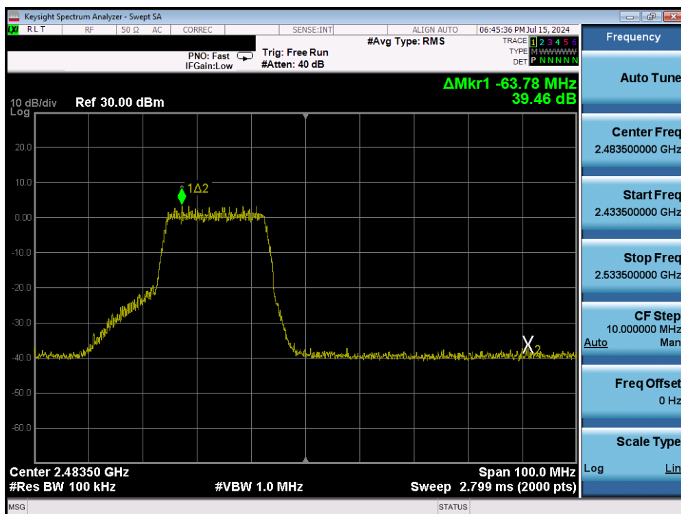
Plot 7-45. Band Edge Plot (802.11n (2.4GHz) – Ch. 12) – MCS7
