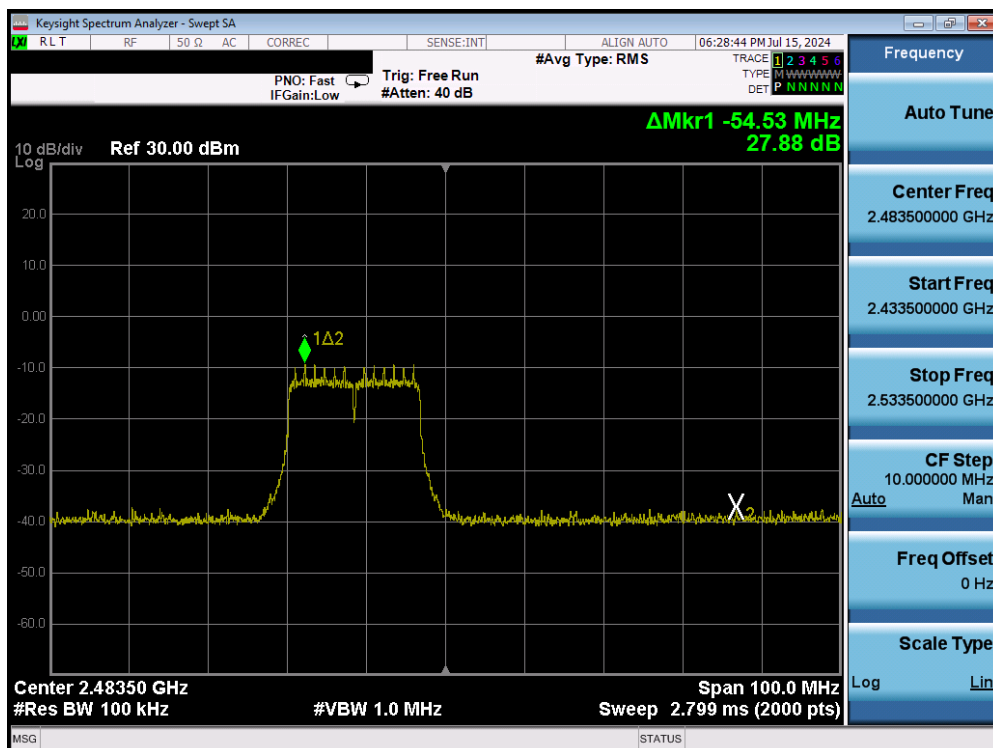
Plot 7-34. Band Edge Plot (802.11g – Ch. 13) – 6Mbps
