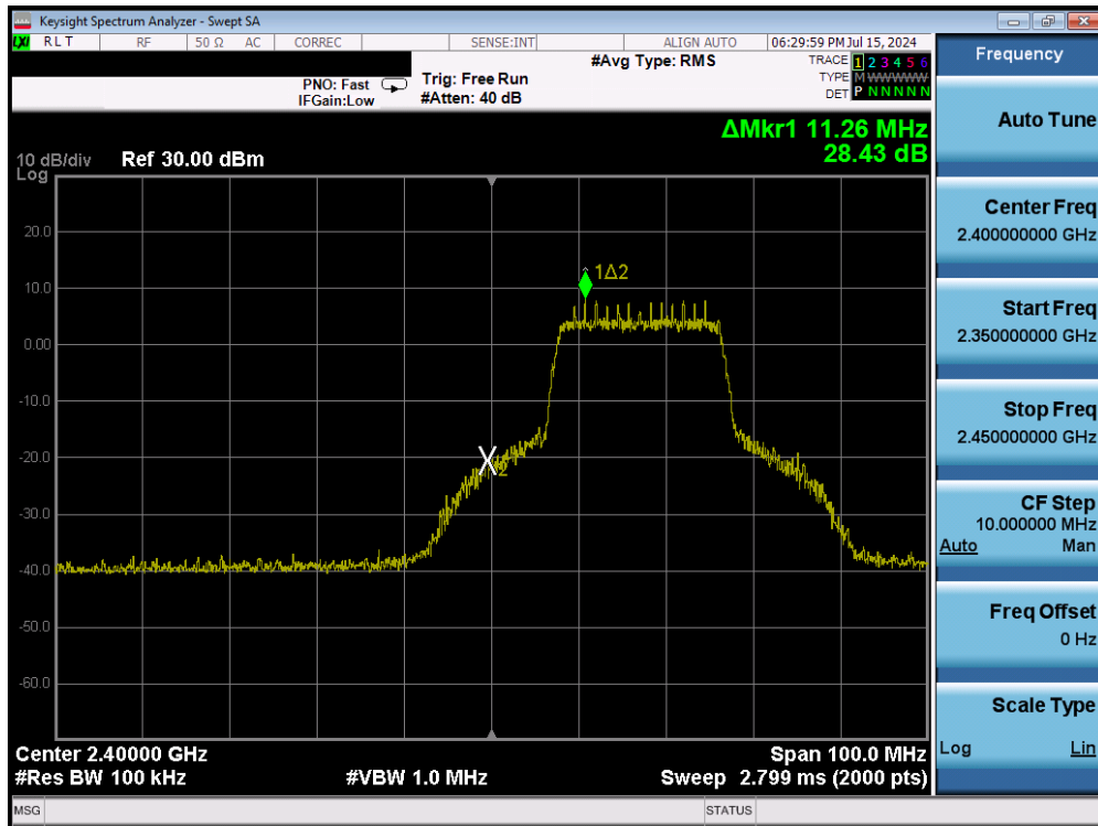
Plot 7-36. Band Edge Plot (802.11n (2.4GHz) – Ch. 2) – MCS0
