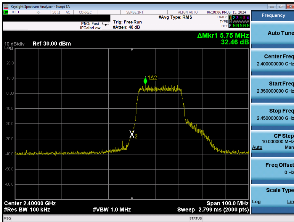
Plot 7-41. Band Edge Plot (802.11n (2.4GHz) – Ch. 1) – MCS7
