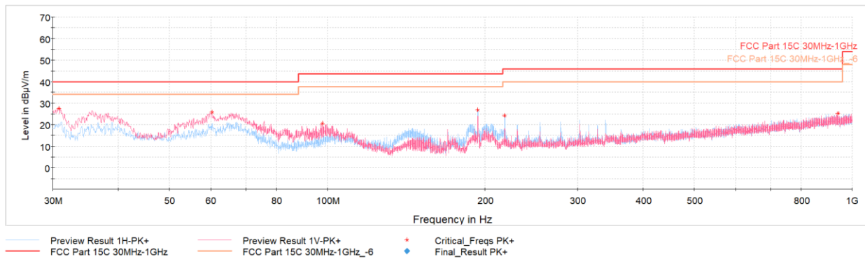
Plot 7-72. Radiated Spurious Emissions below 1GHz 11b Ch.6, with AC/DC Adapter + Magnetic Charger
