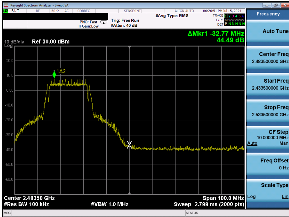
Plot 7-31. Band Edge Plot (802.11g – Ch. 10) – 6Mbps
