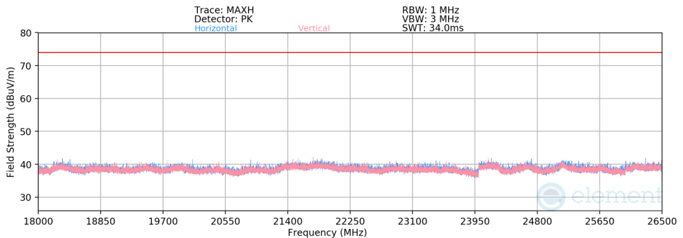
Plot 7-55. Radiated Spurious Emissions Above 18GHz (802.11b – Ch. 6)
