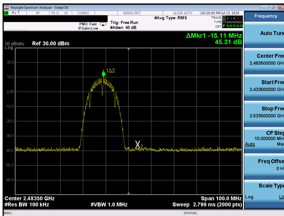
Plot 7-28. Band Edge Plot (802.11b – Ch. 13) – 1Mbps
