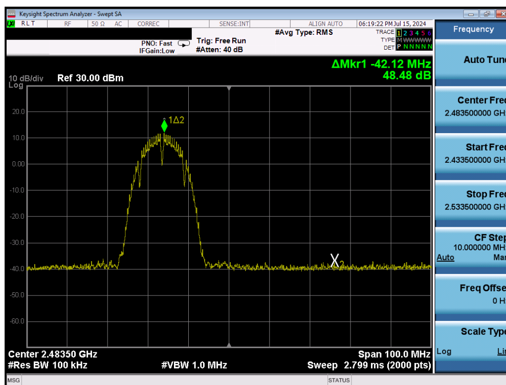
Plot 7-27. Band Edge Plot (802.11b – Ch. 12) – 1Mbps
