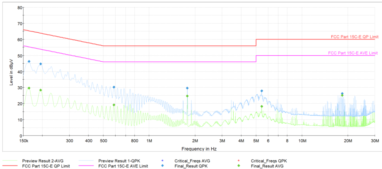
Plot 7-74. AC Line Conducted Plot 802.11b - Ch.6 (N, with AC/DC Adapter + Magnetic charger)
