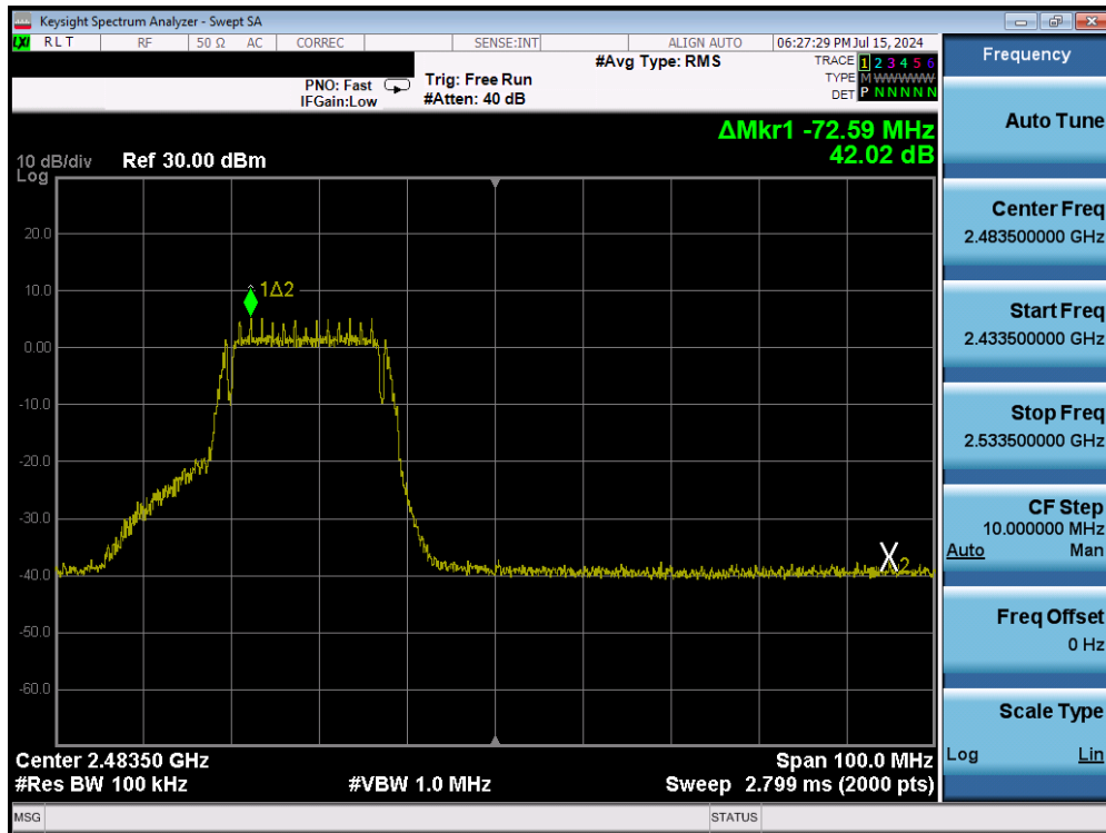
Plot 7-32. Band Edge Plot (802.11g – Ch. 11) – 6Mbps
