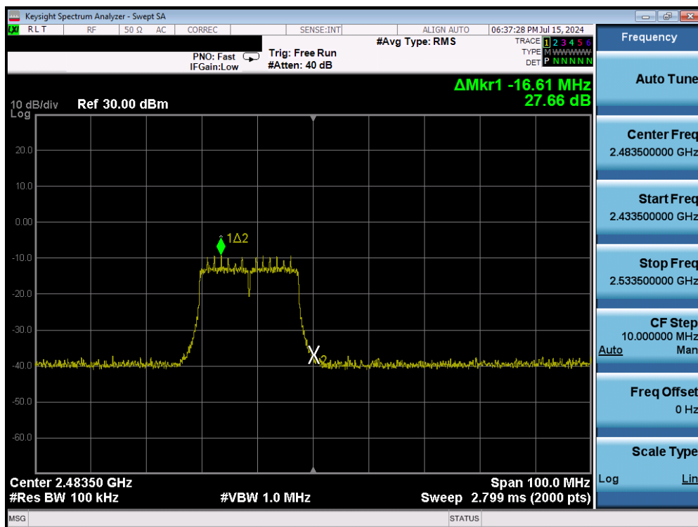
Plot 7-40. Band Edge Plot (802.11n (2.4GHz) – Ch. 13) – MCS0
