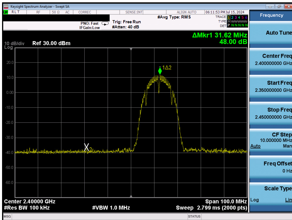
Plot 7-25. Band Edge Plot (802.11b – Ch. 1) – 1Mbps
