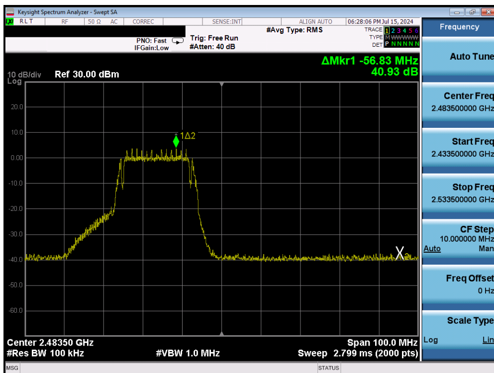
Plot 7-33. Band Edge Plot (802.11g – Ch. 12) – 6Mbps
