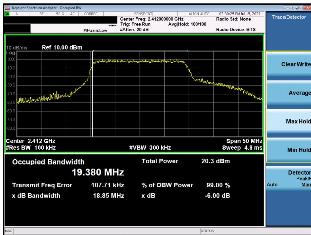
Plot 7-10. 6dB Bandwidth & 99% OBW Plot (802.11n (2.4GHz) – Ch. 1) – MCS7
