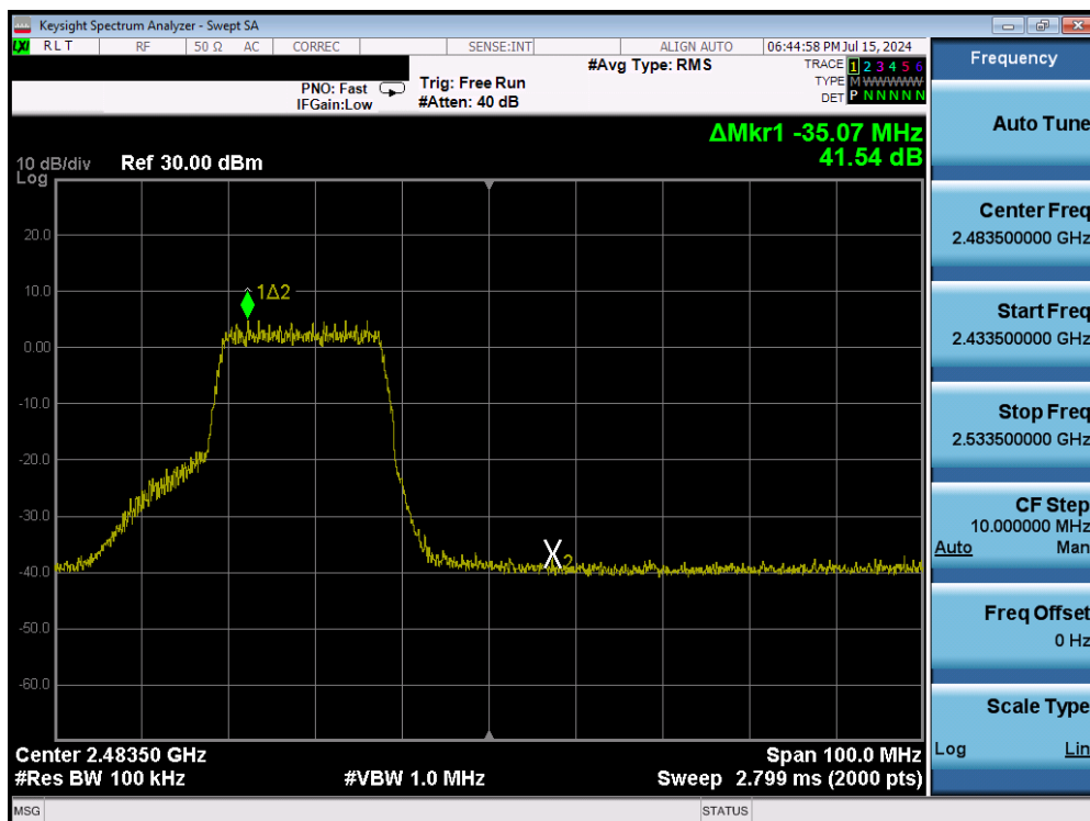
Plot 7-44. Band Edge Plot (802.11n (2.4GHz) – Ch. 11) – MCS7
