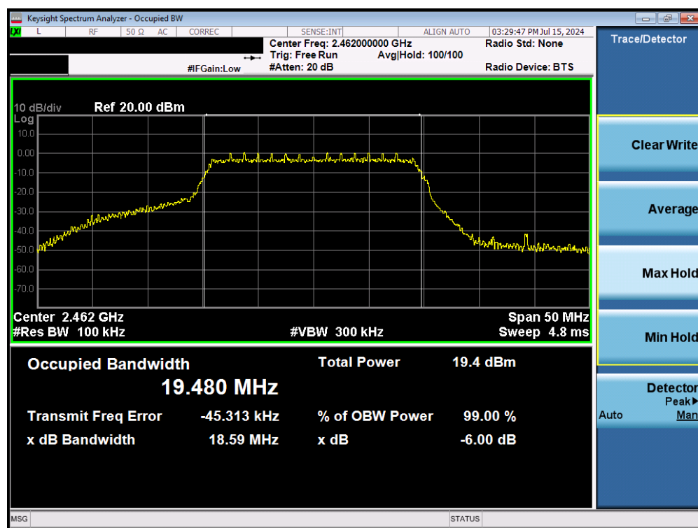
Plot 7-9. 6dB Bandwidth & 99% OBW Plot (802.11n (2.4GHz) – Ch. 11) – MCS0
