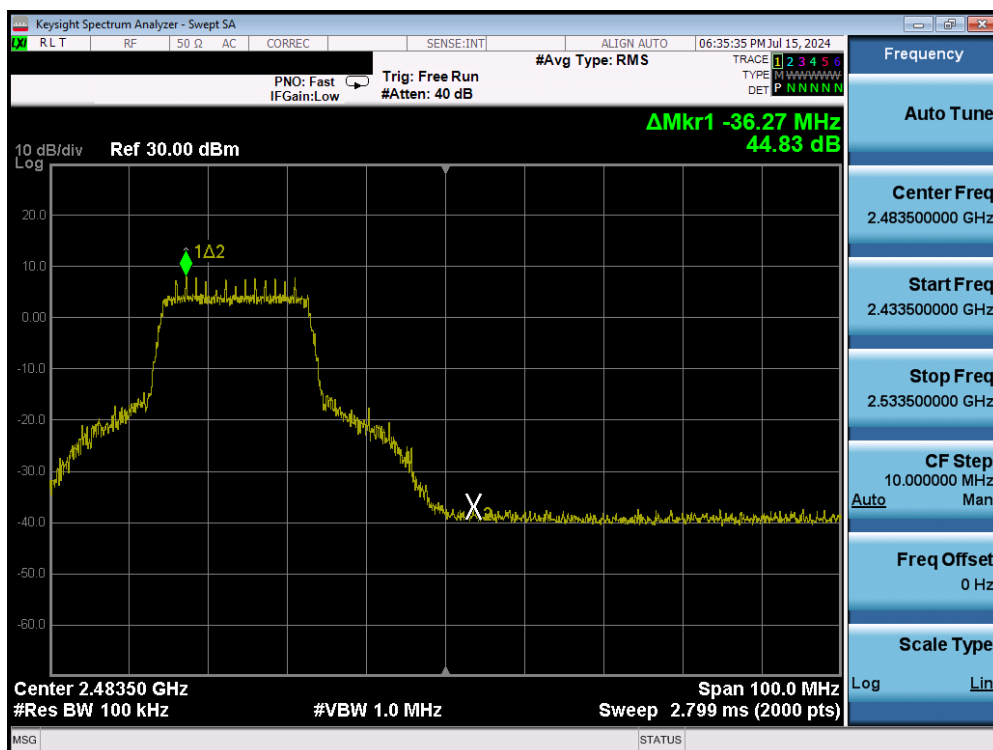
Plot 7-37. Band Edge Plot (802.11n (2.4GHz) – Ch. 10) – MCS0
