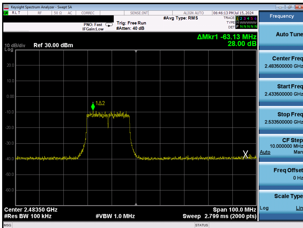
Plot 7-46. Band Edge Plot (802.11n (2.4GHz) – Ch. 13) – MCS7
