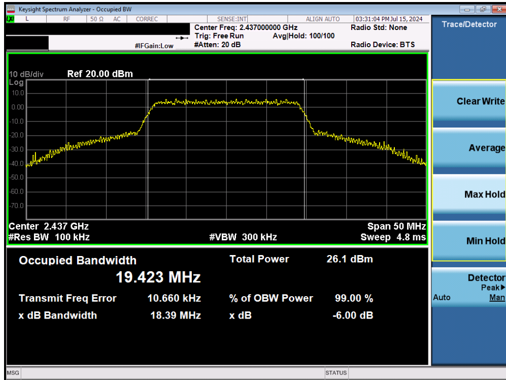
Plot 7-11. 6dB Bandwidth & 99% OBW Plot (802.11n (2.4GHz) – Ch. 6) – MCS7
