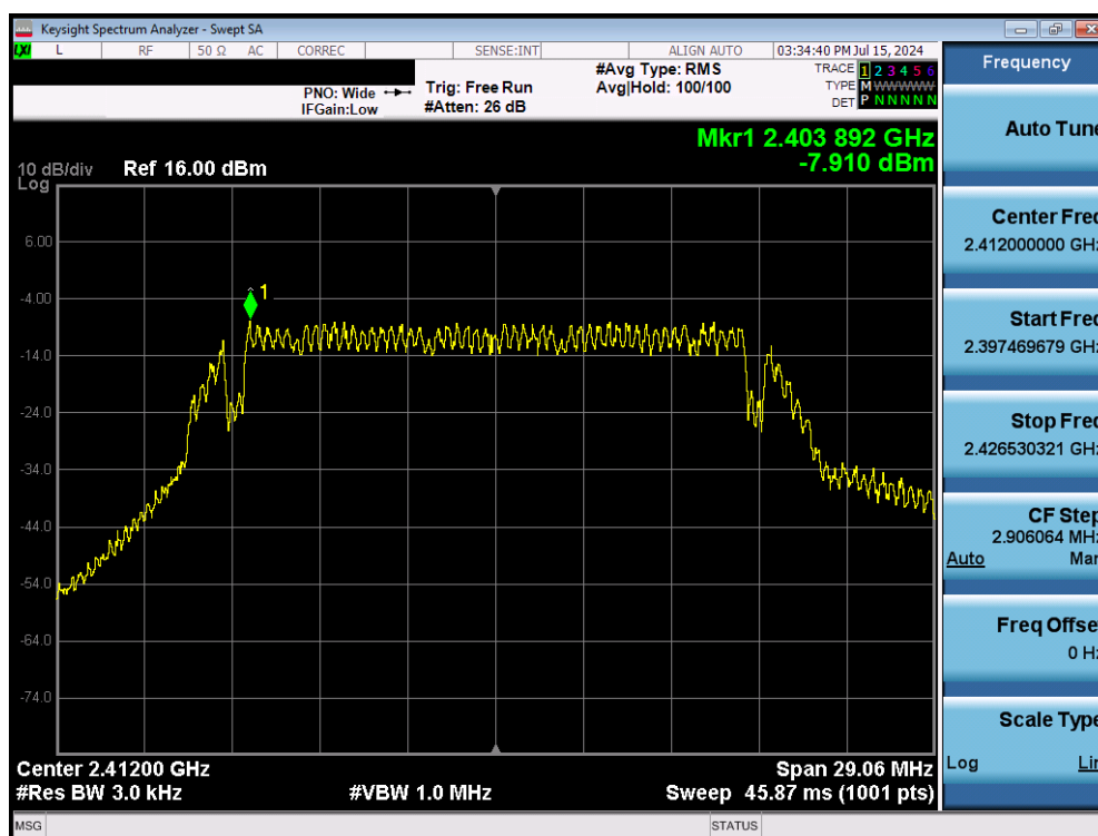
Plot 7-16. Power Spectral Density Plot (802.11g – Ch. 1) – 6Mbps
