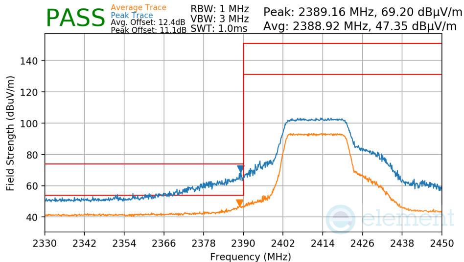
Plot 7-66. Radiated Restricted Lower Band Edge Measurement
