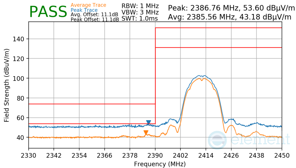
Plot 7-57. Radiated Restricted Lower Band Edge Measurement
