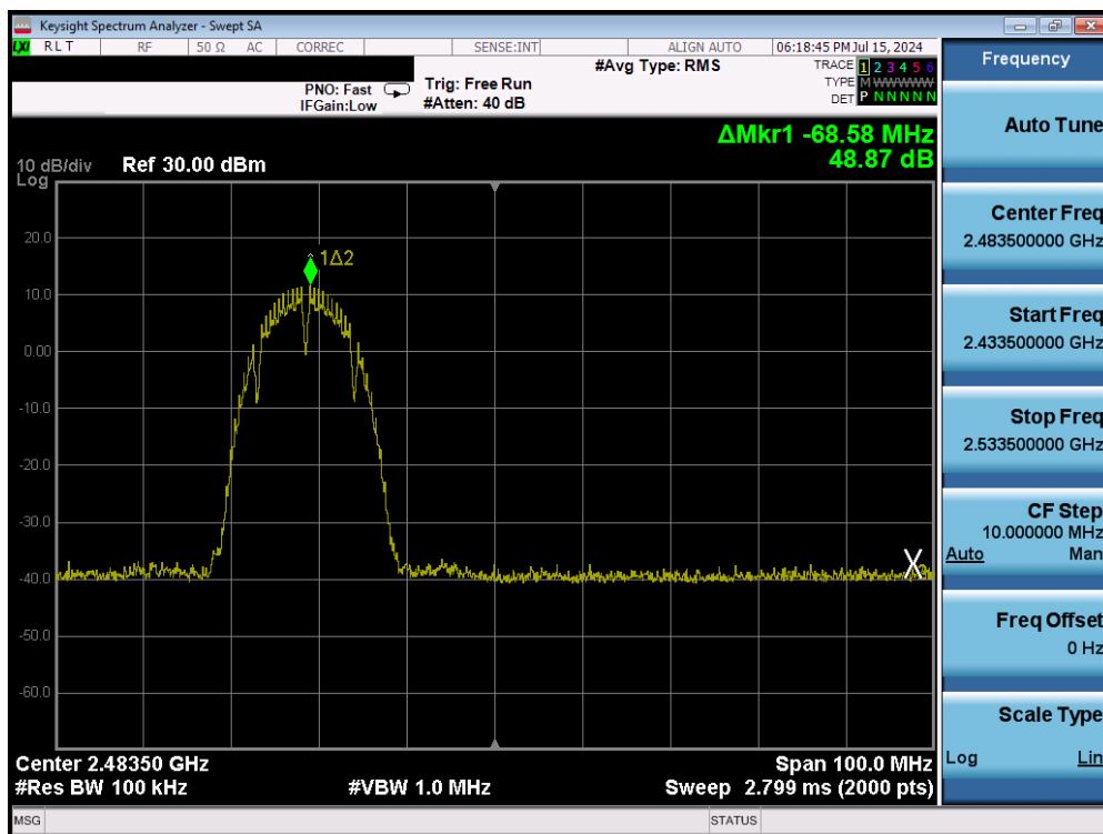
Plot 7-26. Band Edge Plot (802.11b – Ch. 11) – 1Mbps
