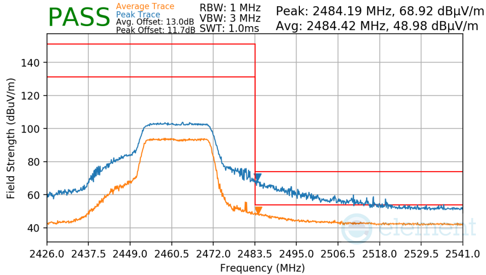
Plot 7-69. Radiated Restricted Upper Band Edge Measurement
