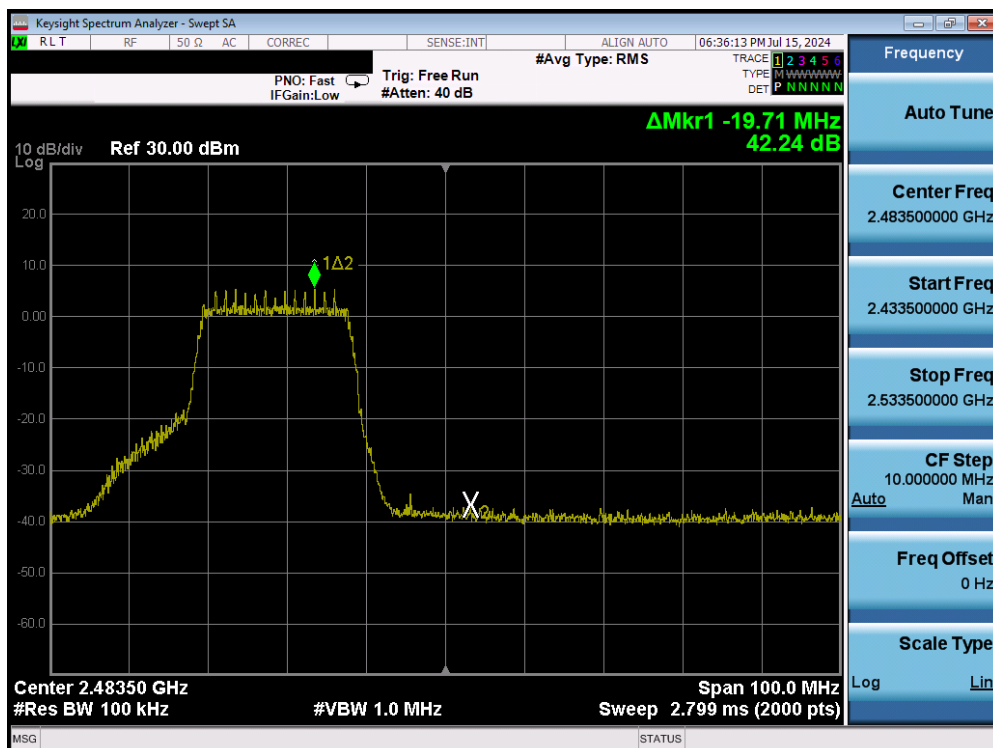
Plot 7-38. Band Edge Plot (802.11n (2.4GHz) – Ch. 11) – MCS0
