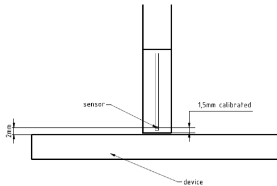
Figure F-3 EUMMWVx Probe
