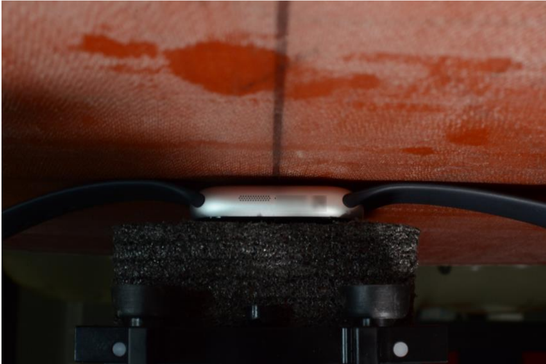
NFC SAR Test Setup Photo 7: Aluminum with Sport Wristband, Extremity, Back Side at 0.0 cm
