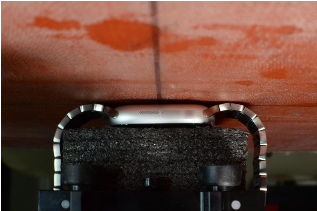
NFC SAR Test Setup Photo 8: Aluminum with Metal Links Wristband, Extremity, Back Side at 0.0 cm
