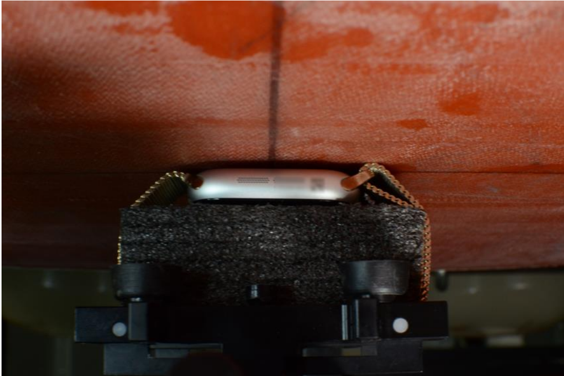
NFC SAR Test Setup Photo 9: Aluminum with Metal Loop Wristband, Extremity, Back Side at 0.0 cm
