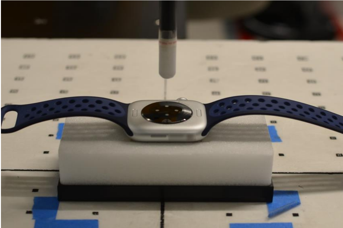
Near Field Power Density Test Setup Photo 11: Aluminum with Sport Wristband, Extremity, Back Side at 0.924 cm
