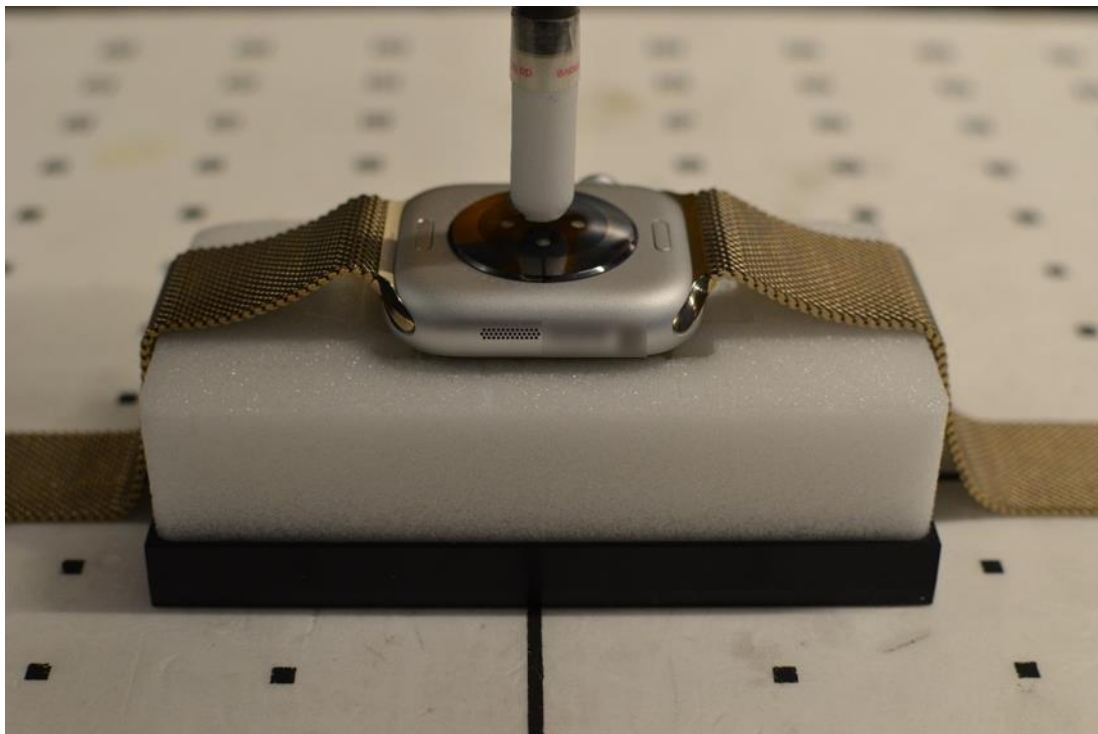
Near Field Power Density Test Setup Photo 13: Aluminum with Metal Loop Wristband, Extremity, Back Side at 0.2 cm
