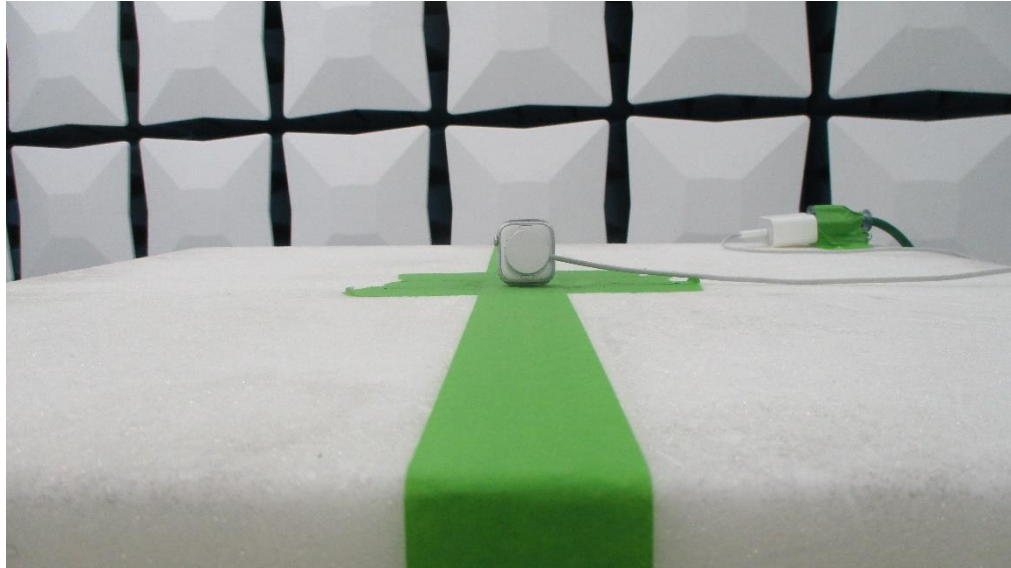
Figure 9: 1-18GHz Test Setup (Front View)
