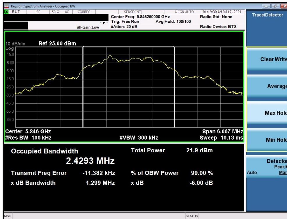
Plot 7-6. 6dB BW & 99% OBW (O-QPSK, 5846.25MHz, 500kpbs)
