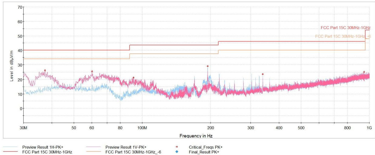
Plot 7-29. RSE 30MHz - 1GHz (O-QPSK – Ch. 24), with AC/DC Adapter & magnetic charger
