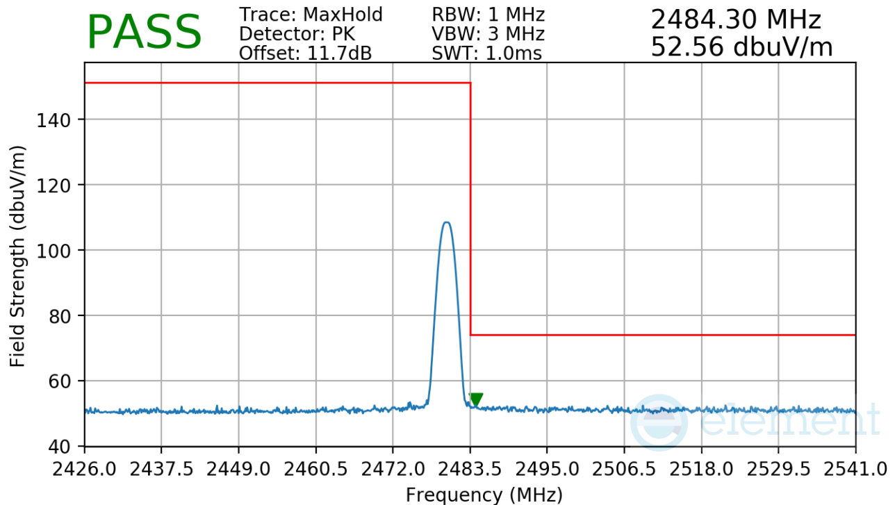
Plot 7-39. Radiated Restricted Upper Band Edge Measurement
