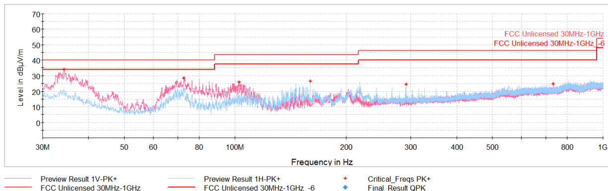
Plot 7-10. Radiated Spurious Emissions 30MHz – 1GHz (CE F 424kbps, with AC/DC Adapter and Magnetic Charger)
