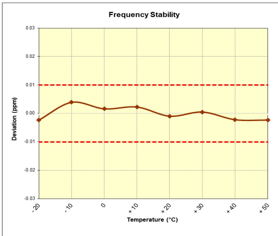
Figure 7-4. Frequency Stability Plot (Reader 10% ASK 1 out of 256)
