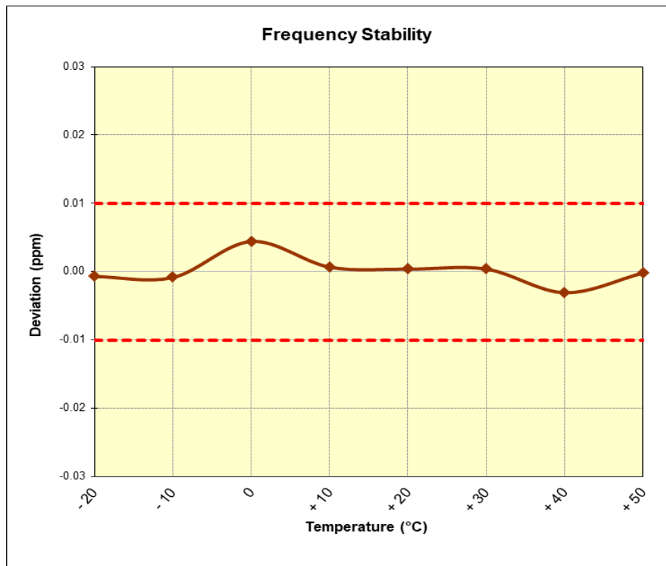
Figure 7-3. Frequency Stability Plot (CE F 212kbps)
