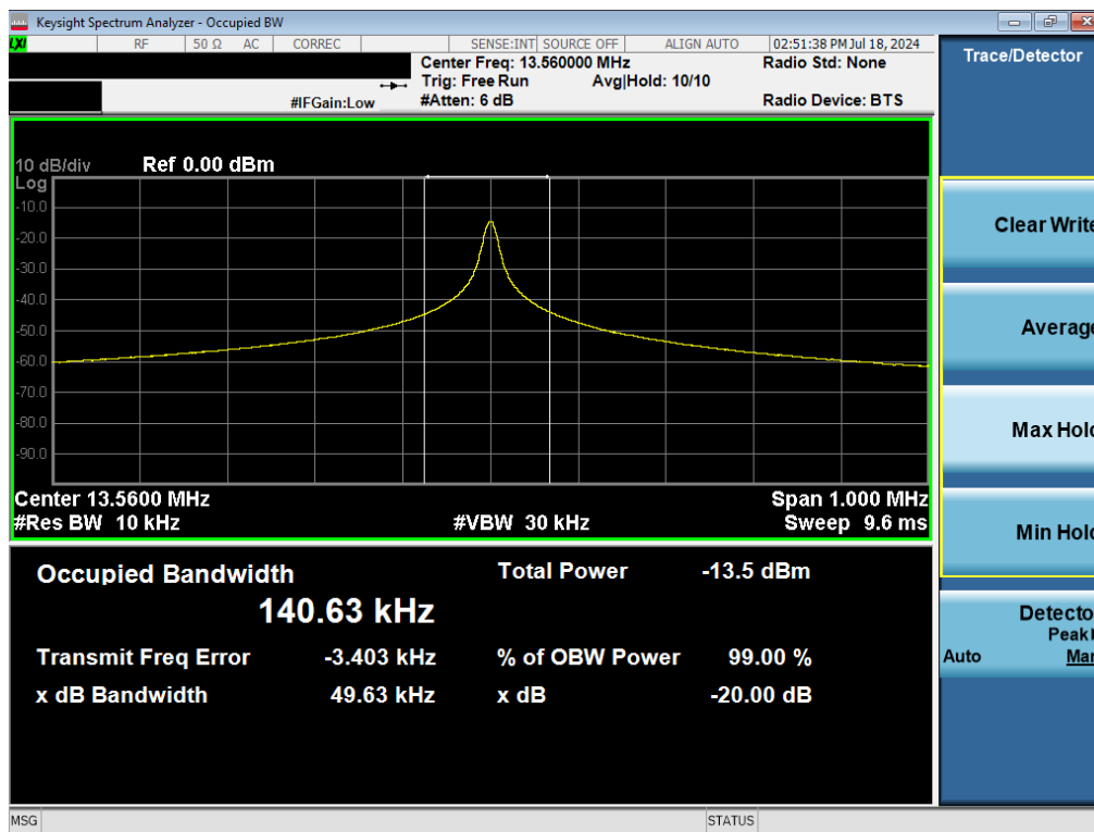
Plot 7-1. 20dB and 99% Bandwidth Plot (CE A 106kbps)
