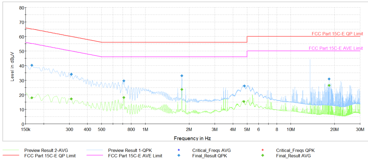
Plot 7-13. AC Line-Conducted Plot (N, CE F 424kbps, with AC/DC Adapter and Magnetic Charger)
