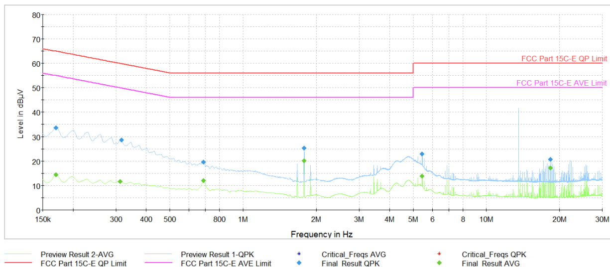
Plot 7-12. AC Line-Conducted Plot (L1, CE F 424kbps, with AC/DC Adapter and Magnetic Charger)
