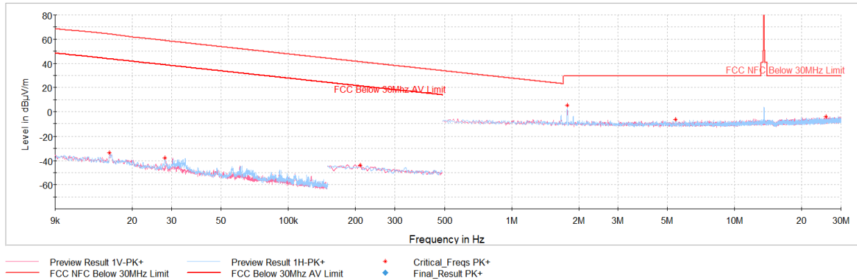
Plot 7-9. Radiated Spurious Emissions 9kHz – 30MHz (Reader A 848kbps, with AC/DC Adapter and Magnetic Charger)
