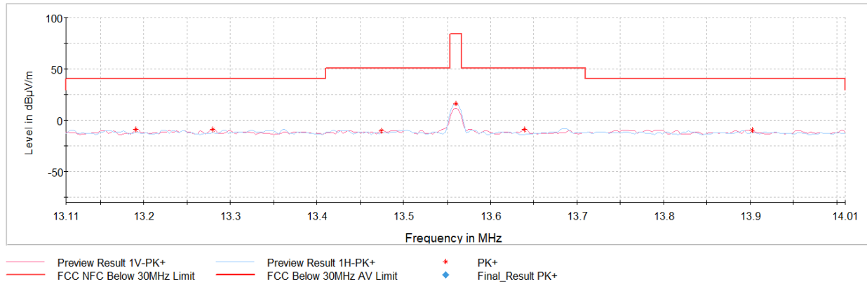
Plot 7-6. In Band Radiated Spurious Emissions (CE F 212kbps, with AC/DC Adapter and Magnetic Charger)
