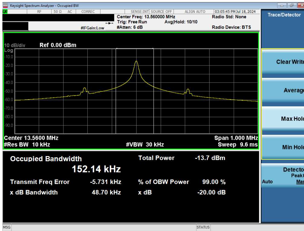
Plot 7-3. 20dB and 99% Bandwidth Plot (CE F 212kbps)
