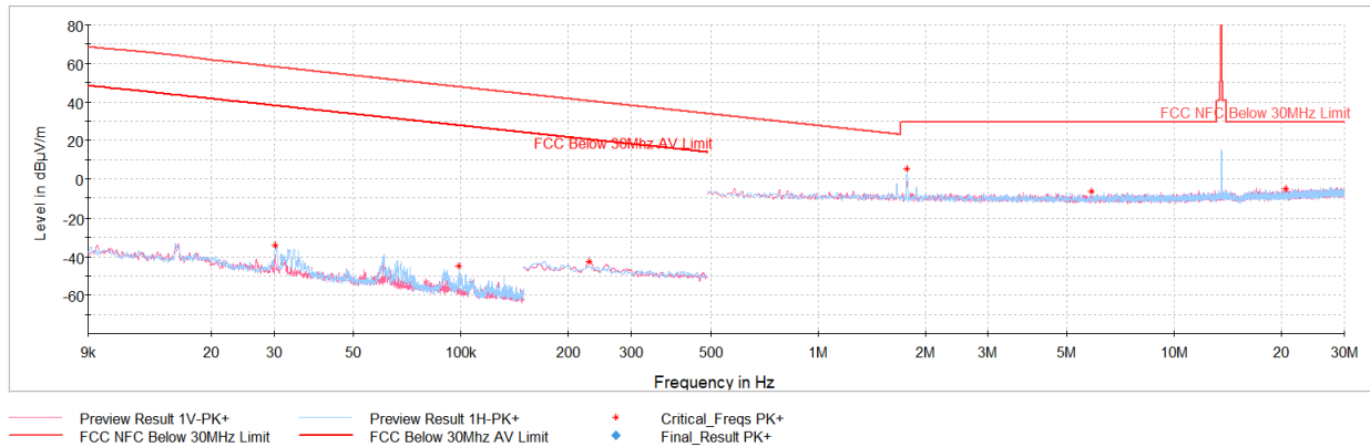
Plot 7-8. Radiated Spurious Emissions 9kHz – 30MHz (CE F 212kbps, with AC/DC Adapter and Magnetic Charger)
