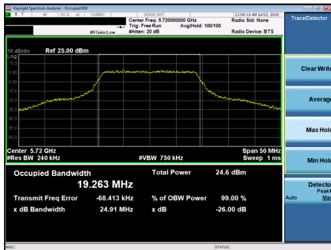
Plot 7-9. 26dB BW & 99% OBW (20MHz BW 802.11n – Ch. 144, MCS0)
