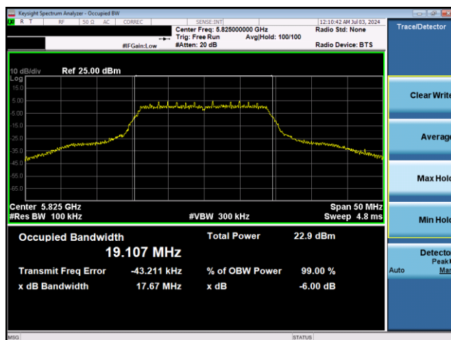
Plot 7-12. 6dB BW & 99% OBW (20MHz BW 802.11n – Ch. 165, MCS0)
