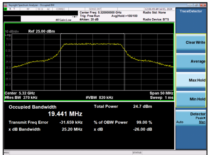
Plot 7-6. 26dB BW & 99% OBW (20MHz BW 802.11n – Ch. 64, MCS0)
