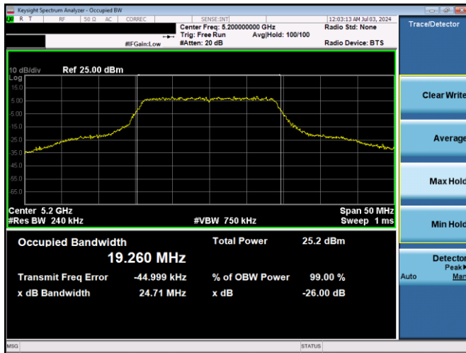
Plot 7-2. 26dB BW & 99% OBW (20MHz BW 802.11n – Ch. 40, MCS0)
