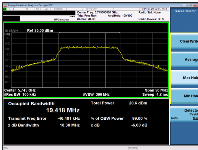
Plot 7-10. 6dB BW & 99% OBW (20MHz BW 802.11n – Ch. 149, MCS0)
