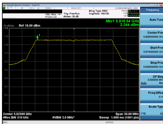
Plot 7-27. PSD (20MHz BW 802.11n - Ch. 165, MCS0)
