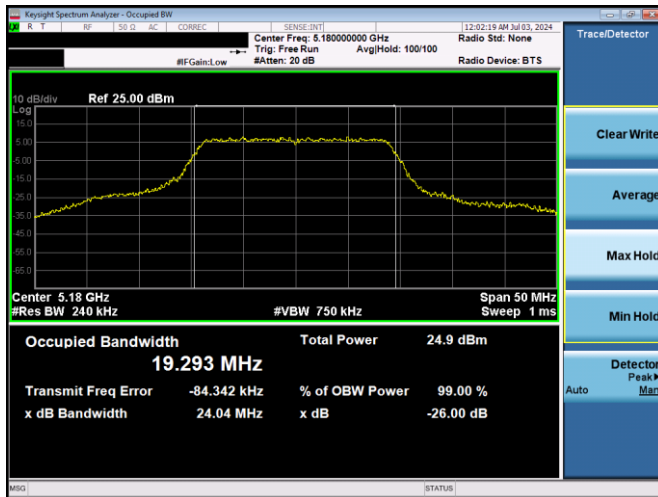
Plot 7-1. 26dB BW & 99% OBW (20MHz BW 802.11n – Ch. 36, MCS0)
