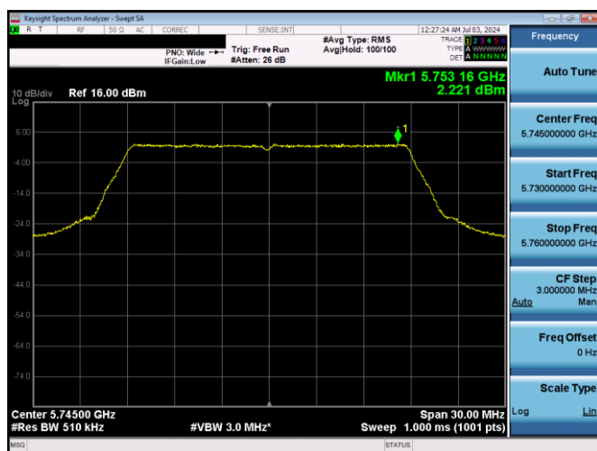
Plot 7-25. PSD (20MHz BW 802.11n - Ch. 149, MCS0)
