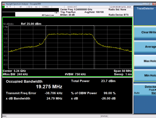
Plot 7-3. 26dB BW & 99% OBW (20MHz BW 802.11n – Ch. 48, MCS0)
