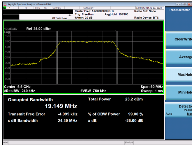
Plot 7-7. 26dB BW & 99% OBW (20MHz BW 802.11n – Ch. 100, MCS0)
