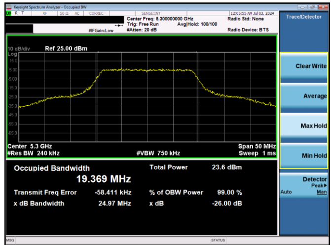
Plot 7-5. 26dB BW & 99% OBW (20MHz BW 802.11n – Ch. 60, MCS0)
