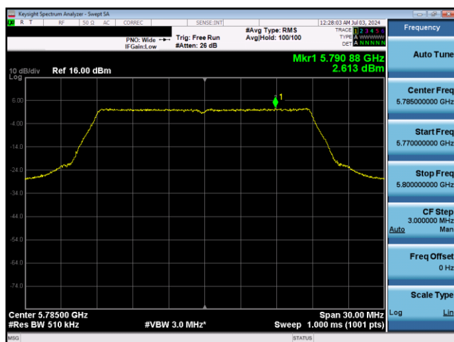
Plot 7-26. PSD (20MHz BW 802.11n - Ch. 157, MCS0)
