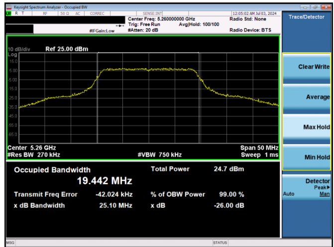
Plot 7-4. 26dB BW & 99% OBW (20MHz BW 802.11n – Ch. 52, MCS0)
