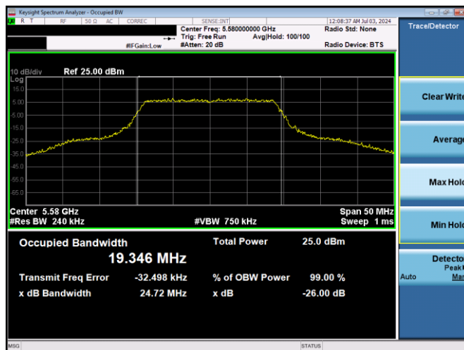
Plot 7-8. 26dB BW & 99% OBW (20MHz BW 802.11n – Ch. 116, MCS0)
