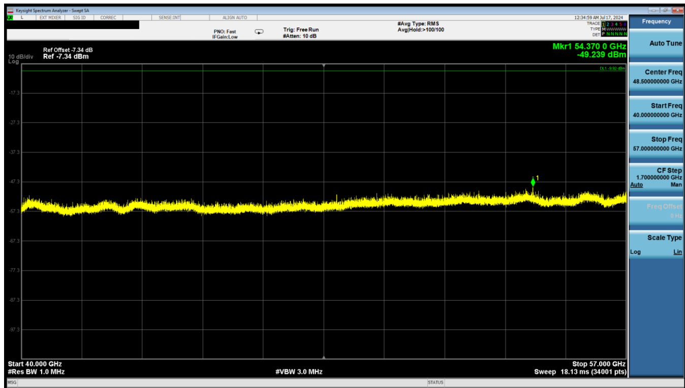
Plot 6-3. Radiated Spurious Emissions 40GHz – 57GHz (Mode 1)
