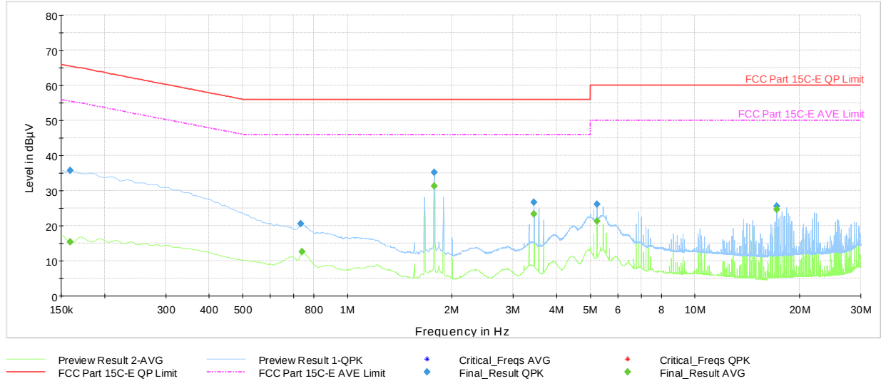
Plot 6-12. AC Line Conducted Plot (N - Mode 1, with Magnetic Charger & Laptop)
