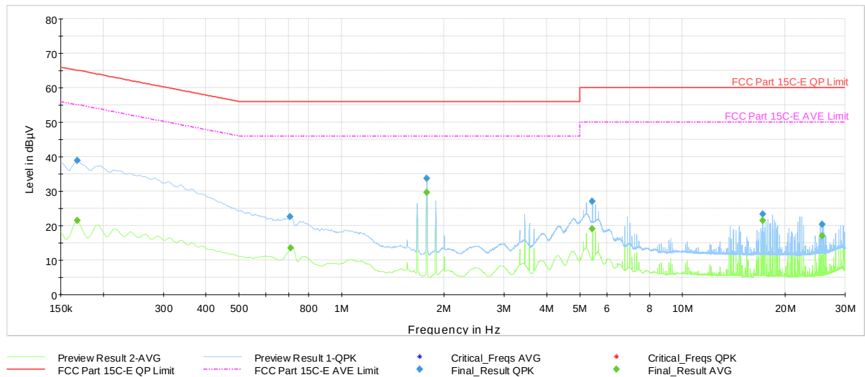
Plot 6-11. AC Line Conducted Plot (L1 - Mode 1, with Magnetic Charger & Laptop)
