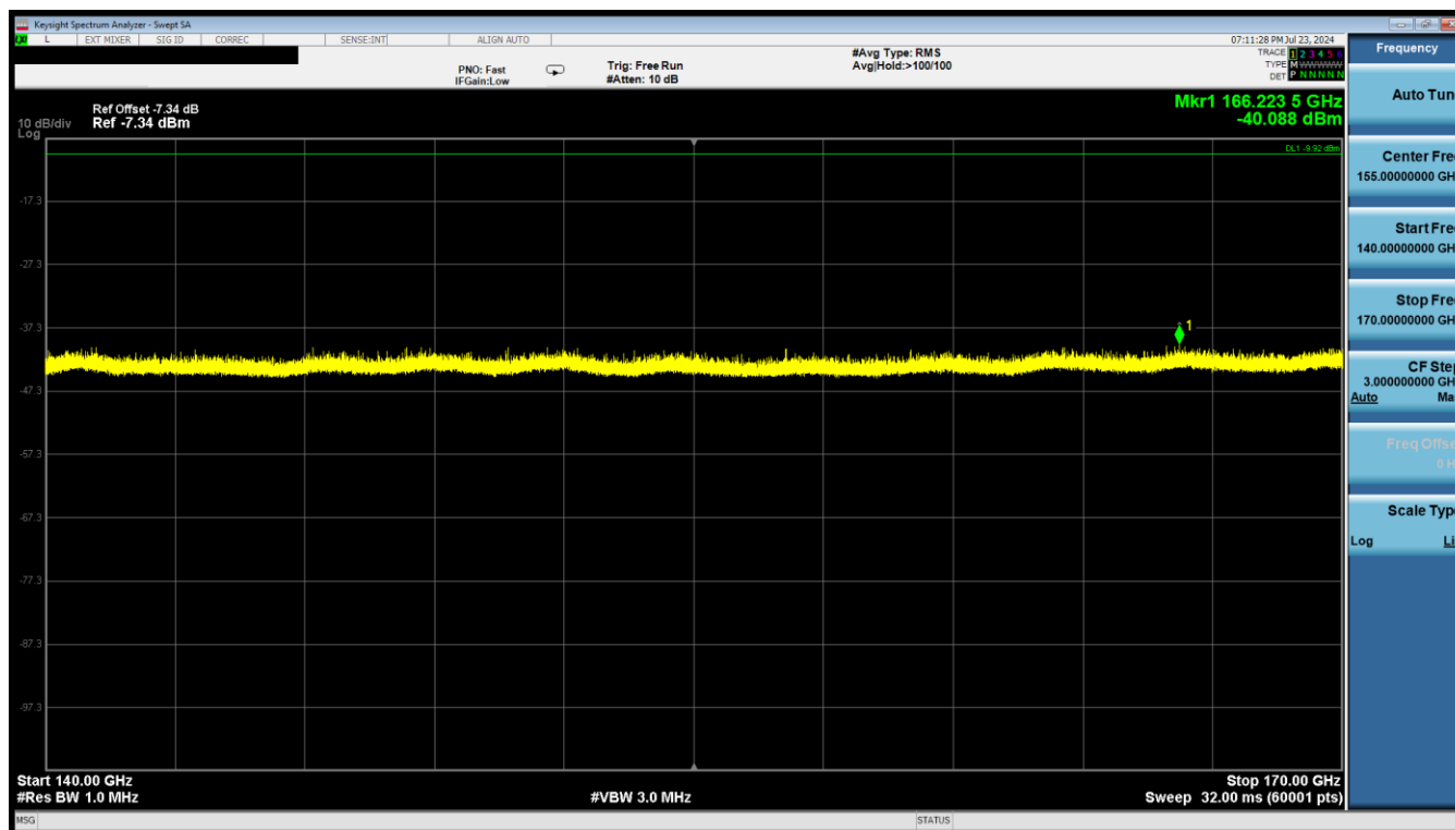
Plot 6-6. Radiated Spurious Emissions 140GHz – 170GHz (Mode1)
