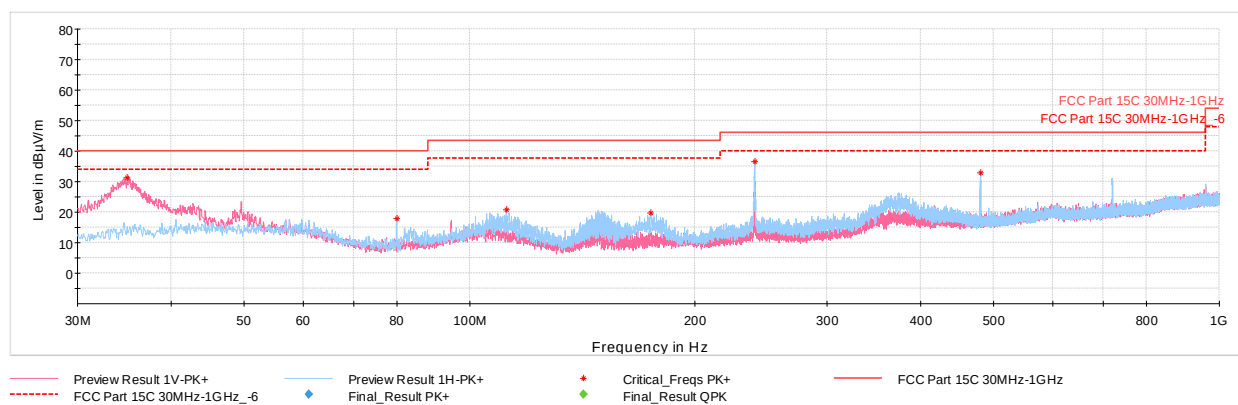
Plot 6-10. Radiated Spurious Emissions 30MHz – 1GHz (Mode 1, with Magnetic Charger & Laptop)
