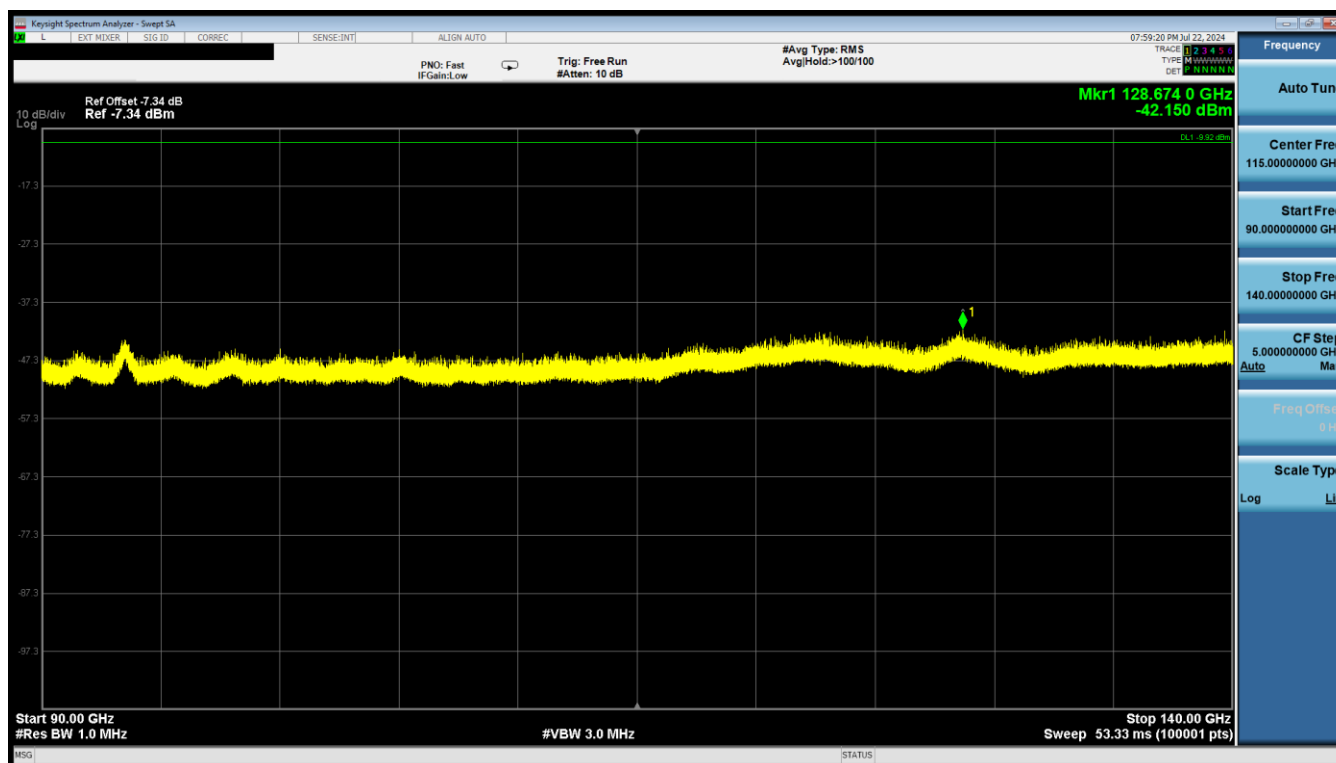
Plot 6-5. Radiated Spurious Emissions 90GHz – 140GHz (Mode 1)
