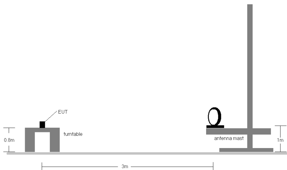
Figure 6-6. Radiated Test Setup (9kHz – 30MHz)
