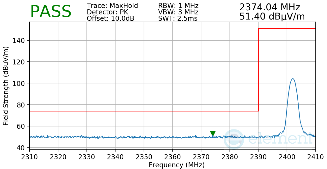
Plot 7-39. Radiated Restricted Lower Band Edge Measurement
