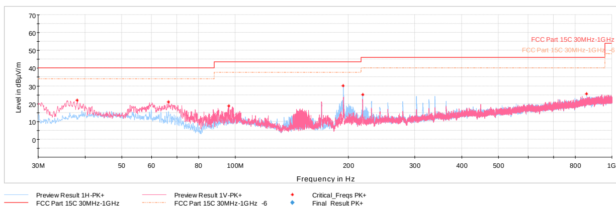
Plot 7-42. Radiated Spurious Emissions Below 1GHz (GFSK ePA – Ch.39, with AC/DC Adapter & Magnetic Charger)
