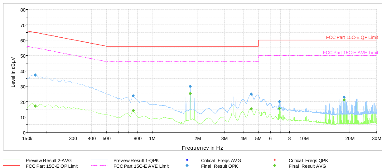
Plot 7-45. AC Line-Conducted Test Plot (N, GFSK ePA – Ch.39, with AC/DC Adapter + Magnetic Charger)
