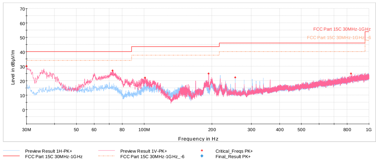
Plot 7-43. Radiated Spurious Emissions Below 1GHz – Simultaneous Transmission
