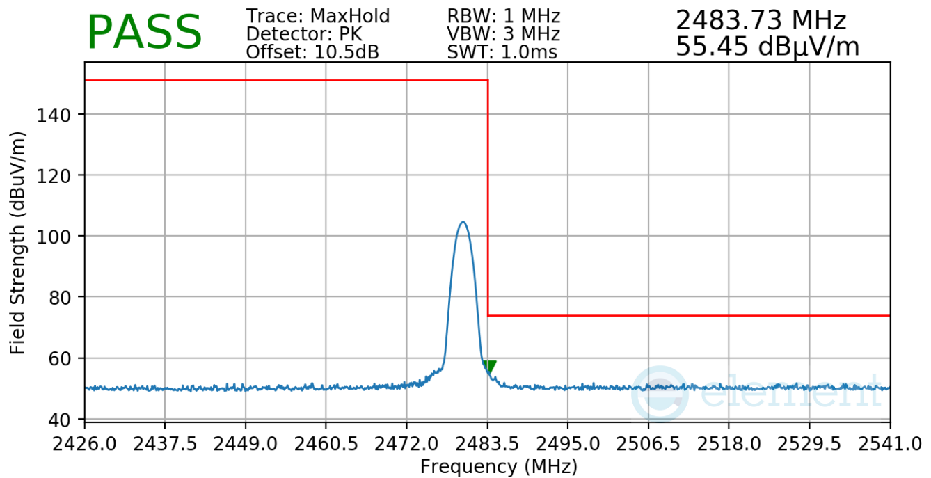
Plot 7-41. Radiated Restricted Upper Band Edge Measurement
