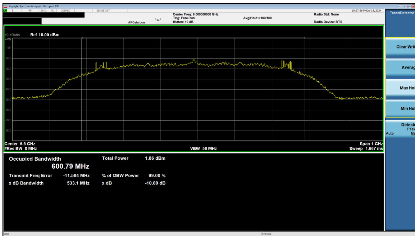
Plot 7-3. ISED 10dBc Bandwidth & 99% Occupied Bandwidth (Ch. 5, Config 409/Payload 4093)
