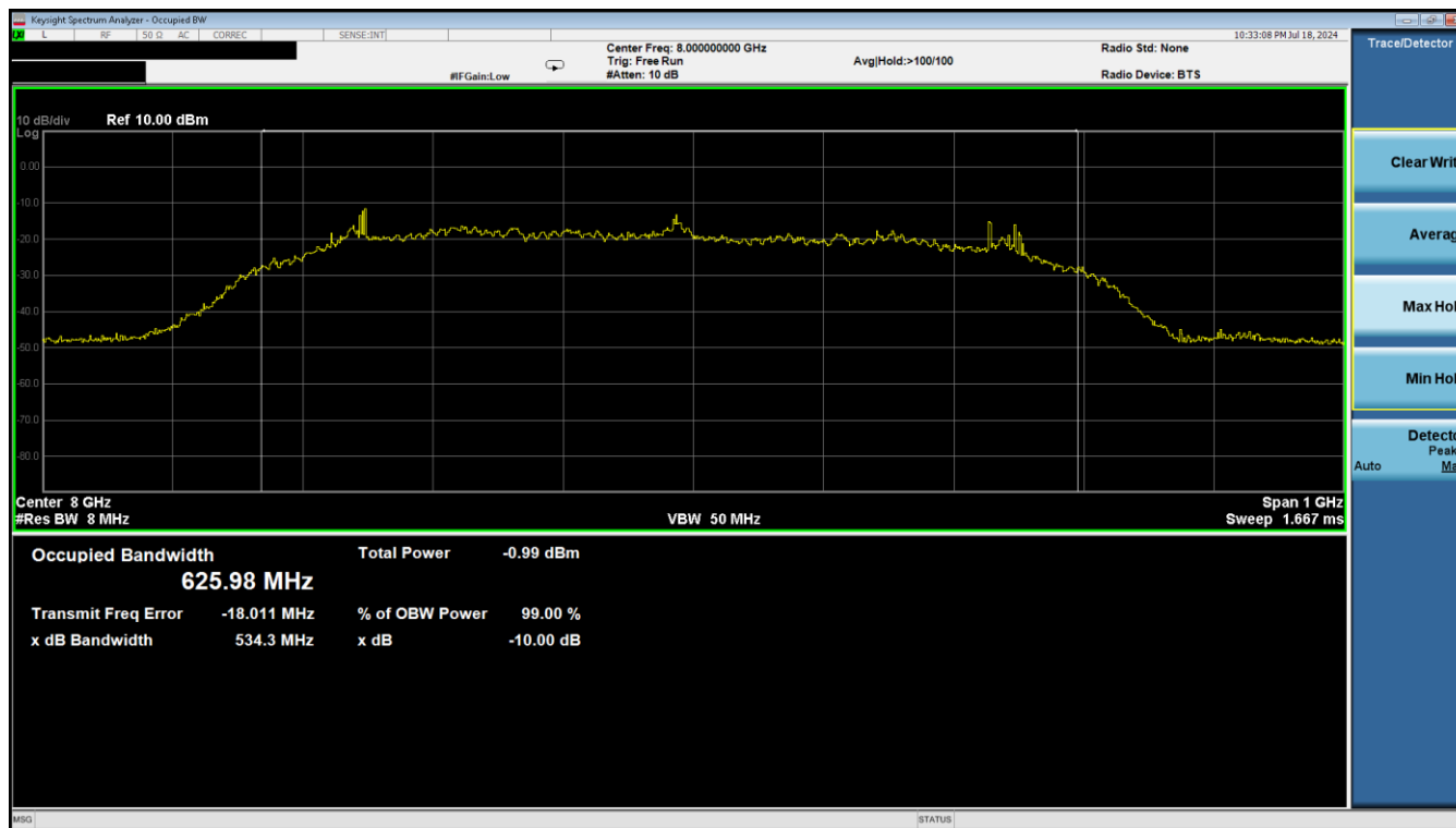
Plot 7-4. ISED 10dBc Bandwidth & 99% Occupied Bandwidth (Ch. 9, Config 409/Payload 4093)
