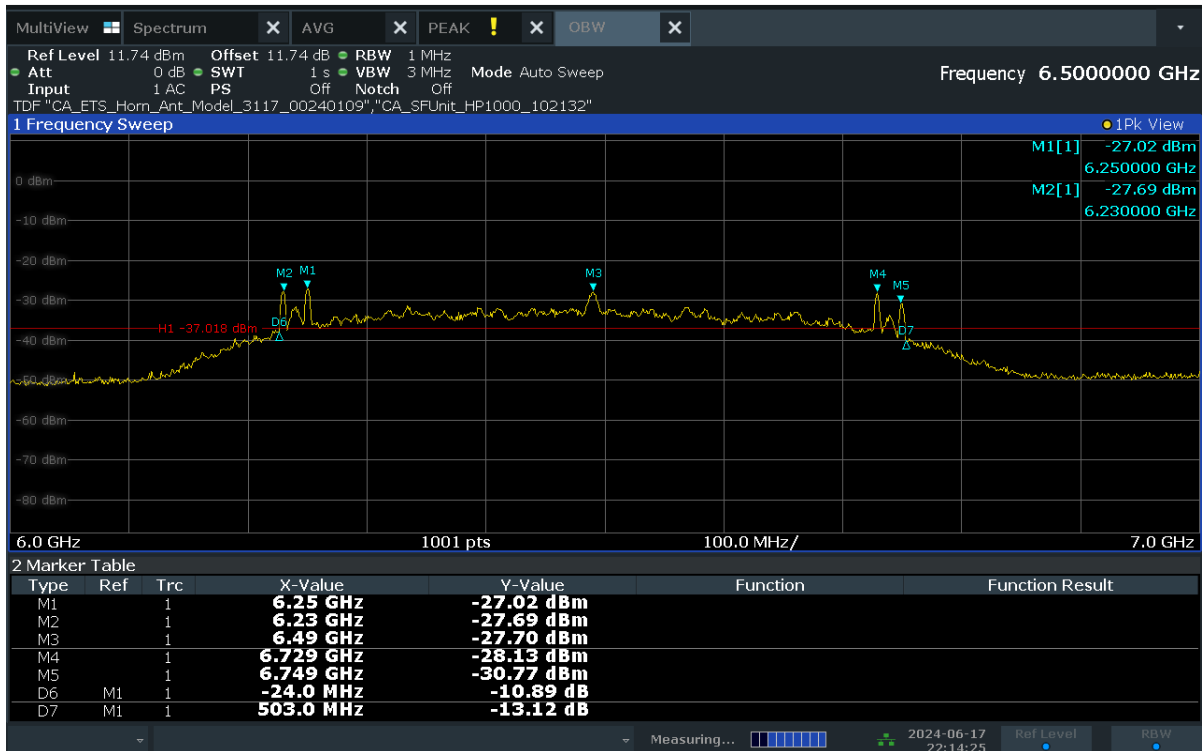
Plot 7-1. 10dBc Bandwidth (Ch. 5, Config 409/Payload 4093)
