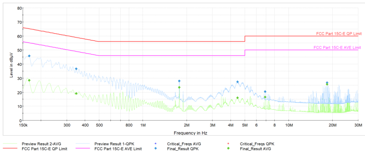
Plot 7-43. AC Line Conducted (Ch. 9, Config 409, Payload 4093 L1, with AC/DC Adapter + Magnetic Charger)
