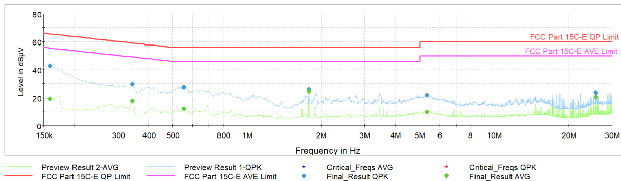
Plot 7-41. AC Line Conducted (Ch. 5, Config 409, Payload 4093 L1, with Laptop + Magnetic Charger)
