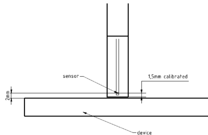
Figure G-3 EUmWVx Probe
