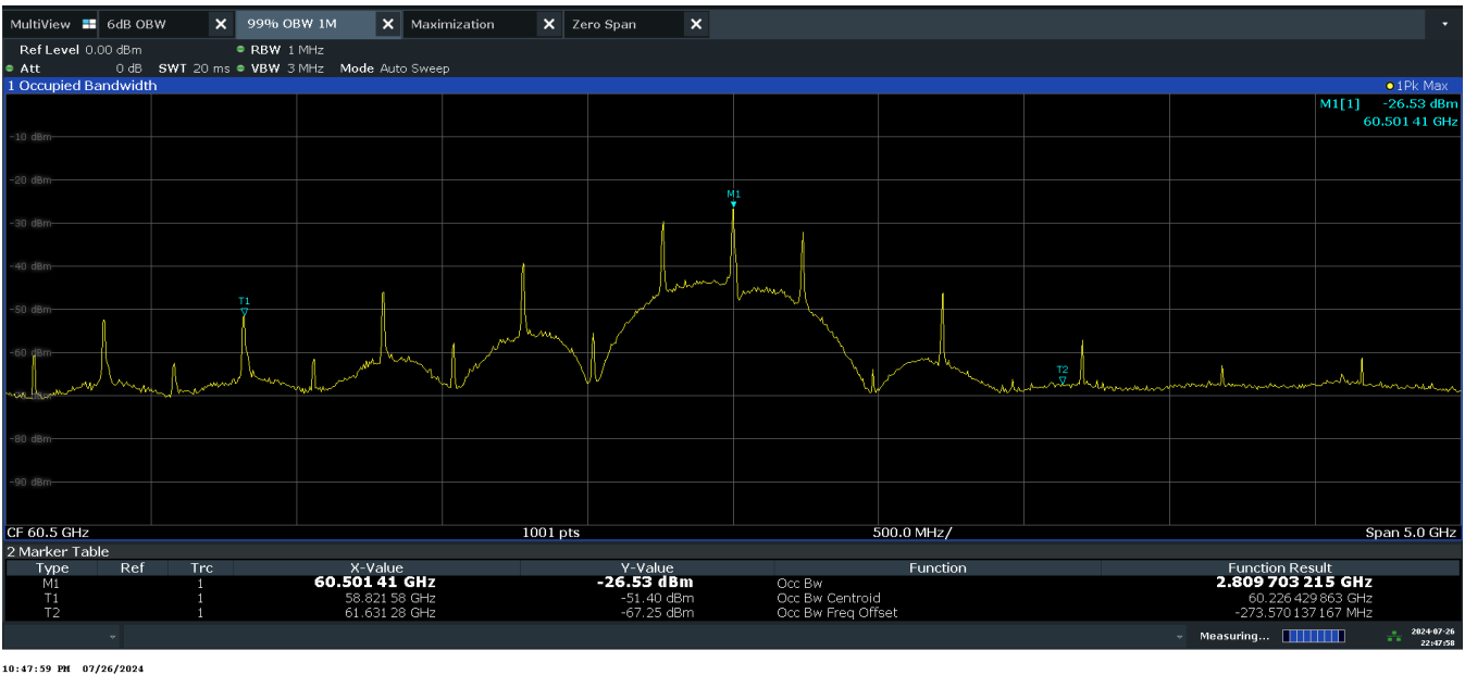
Plot 6-2. 99% Occupied Bandwidth Measurement (Mode 1)
