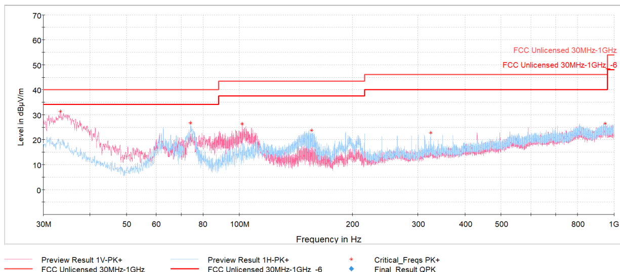
Plot 6-12. Radiated Spurious Emissions 30MHz – 1GHz (Mode 1, with Magnetic Charger & Laptop)
