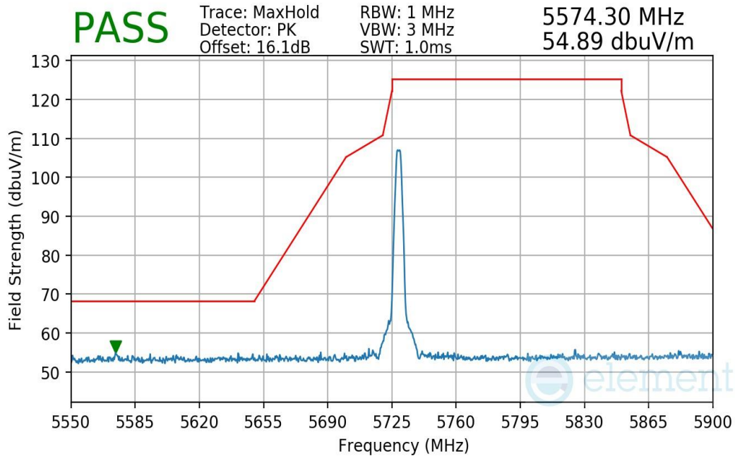
Plot 7-25. Radiated Lower Band Edge Measurement (Pk, Ch. 1, O-QPSK, 500Kbps)
