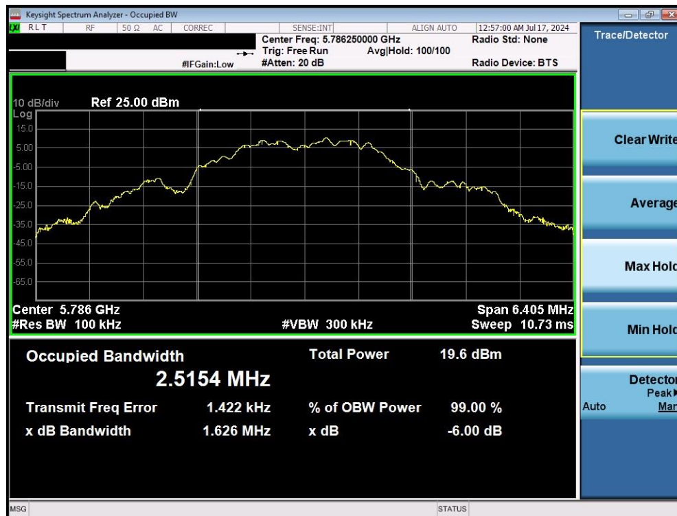
Plot 7-8. 6dB BW & 99% OBW (O-QPSK, 5786.25MHz, 1000kbps)
