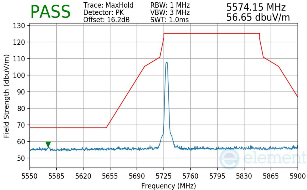
Plot 7-23. Radiated Lower Band Edge Measurement (Pk, Ch. 1, O-QPSK, 250Kbps)
