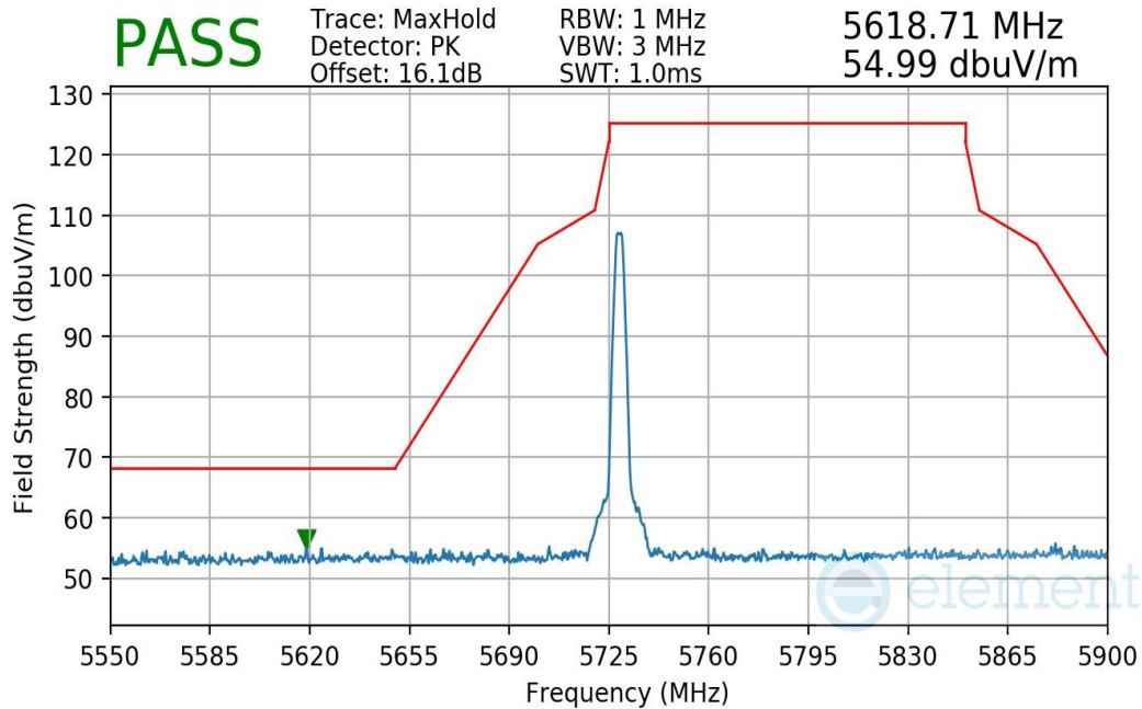
Plot 7-27. Radiated Lower Band Edge Measurement (Pk, Ch. 1, O-QPSK, 1000Kbps)
