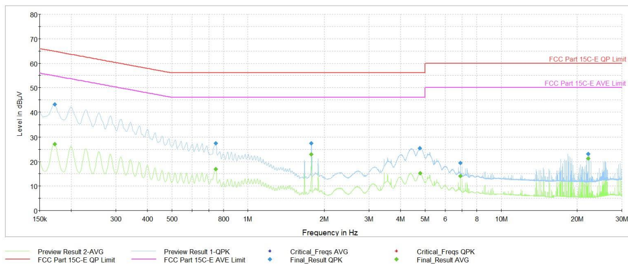
Plot 7-31. AC Line Conducted Plot (O-QPSK – Ch. 24) (N) with AC/DC Adapter & magnetic charger
