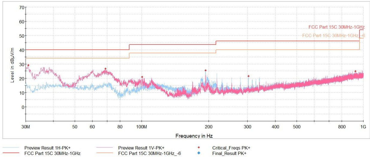
Plot 7-29. RSE 30MHz - 1GHz (O-QPSK – Ch. 24), with AC/DC Adapter & magnetic charger
