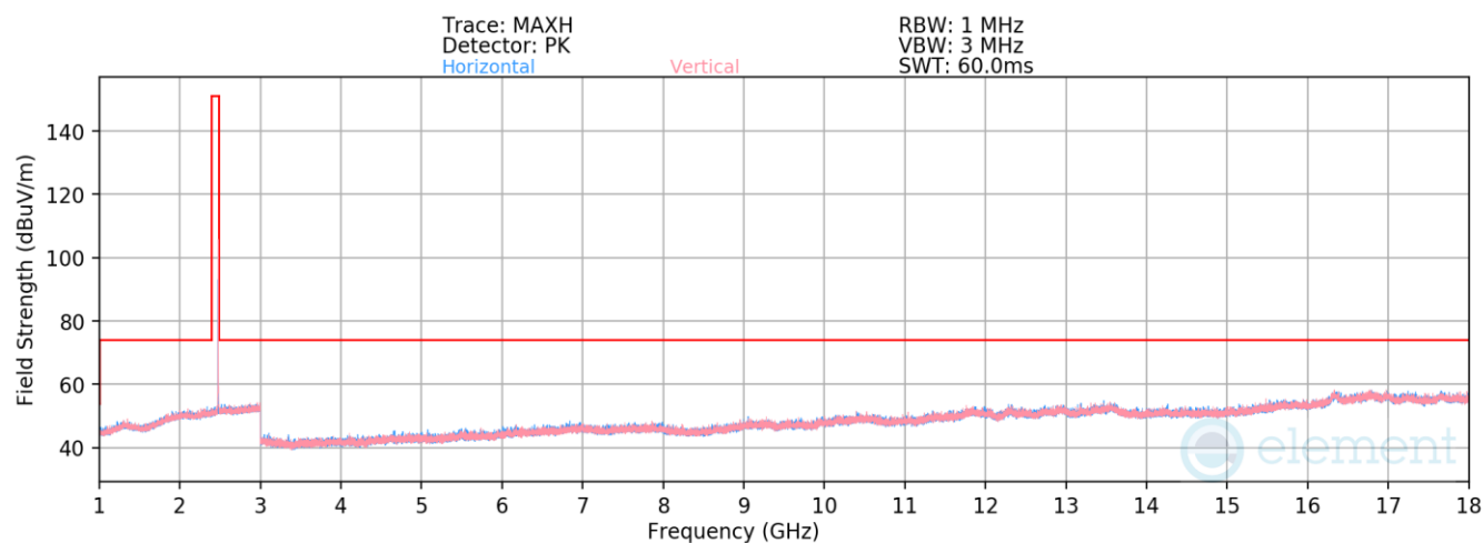
Plot 7-32. Radiated Spurious Emissions 1-18GHz (4Mbps, HDR4, ePA – Ch. 73)
