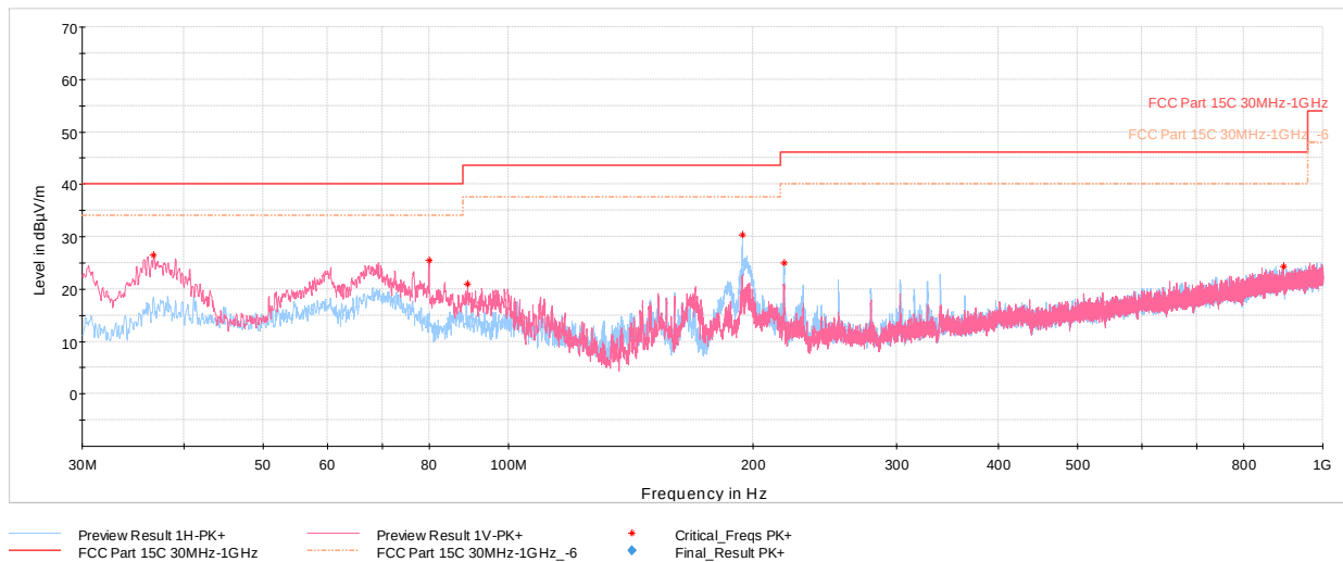
Plot 7-37. Radiated Spurious Emissions Below 1GHz (4Mbps, ePA – Ch.38 with AC/DC Adapter + Magnetic Charger)
