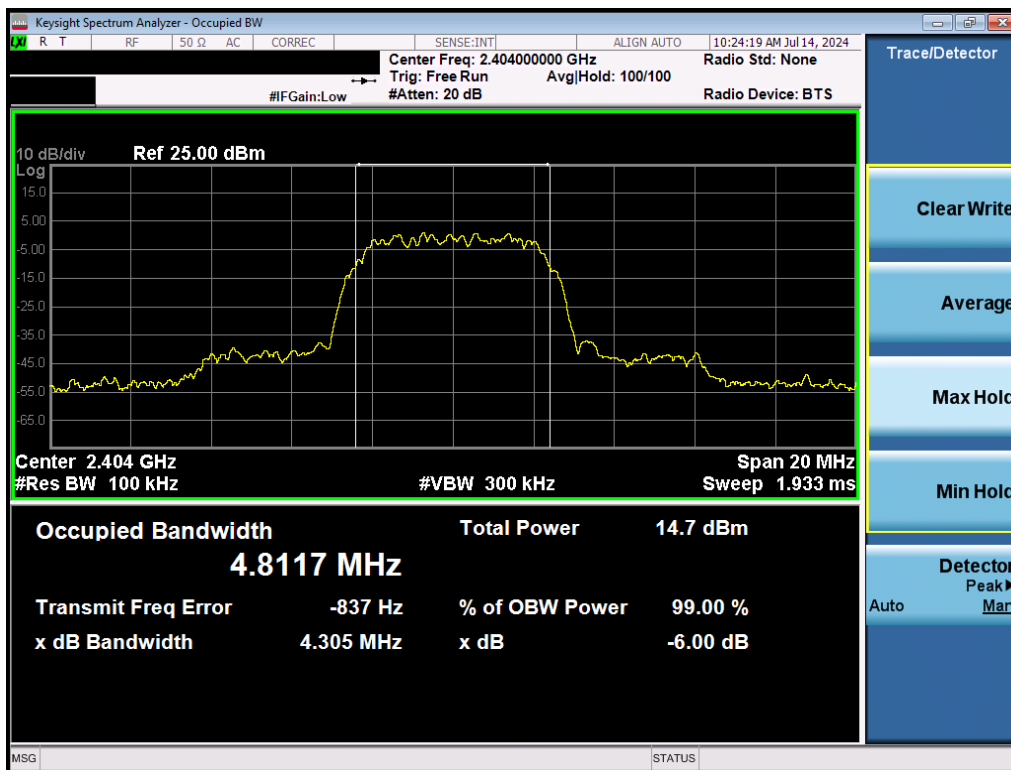
Plot 7-4. 6dB BW & 99% OBW Plot (Bluetooth (HDR8), 8Mbps, ePA – Ch. 1)
