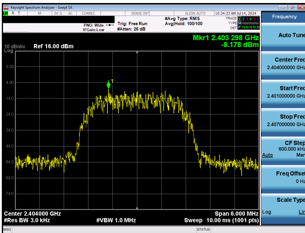
Plot 7-10. Power Spectral Density Plot (Bluetooth (HDR4), 4Mbps, iPA – Ch. 1)
