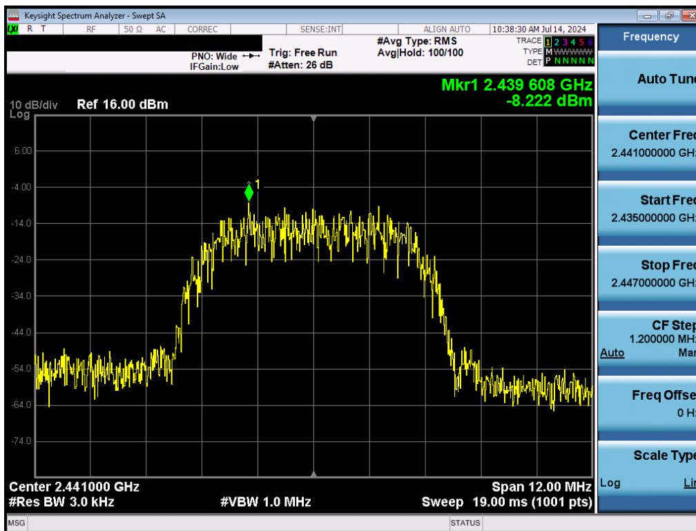
Plot 7-17. Power Spectral Density Plot (Bluetooth (HDR8), 8Mbps, iPA – Ch. 38)
