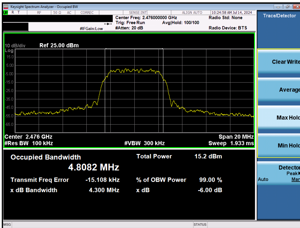
Plot 7-6. 6dB BW & 99% OBW Plot (Bluetooth (HDR8), 8Mbps, ePA – Ch. 73)
