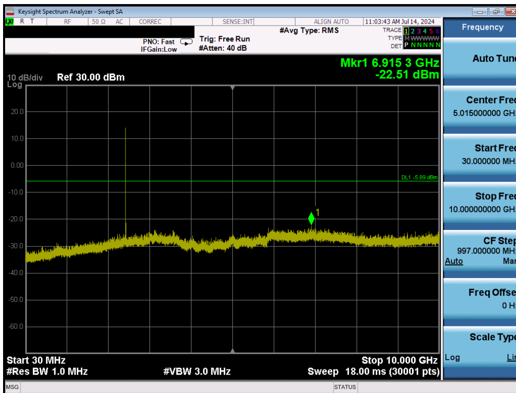
Plot 7-25. Conducted Spurious Plot (Bluetooth (HDR4), ePA – Ch. 38)
