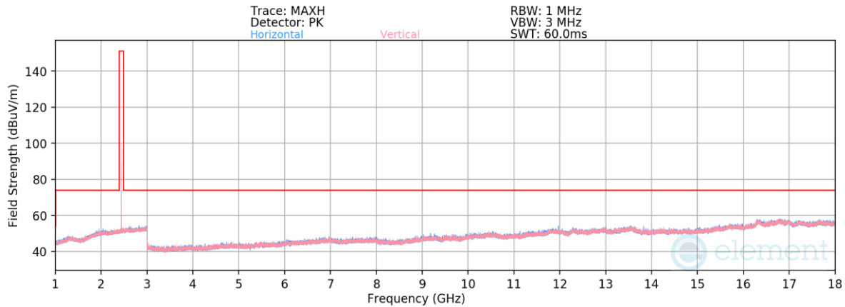
Plot 7-30. Radiated Spurious Emissions 1-18GHz (4Mbps, HDR4, ePA – Ch. 38)
