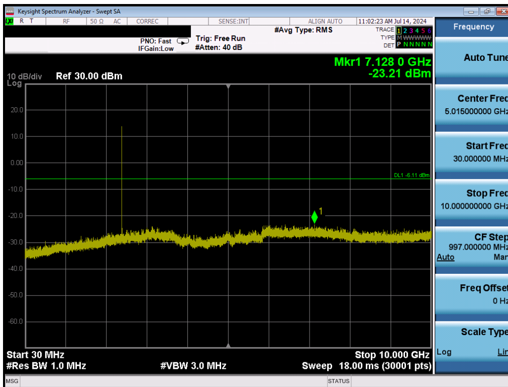
Plot 7-23. Conducted Spurious Plot (Bluetooth (HDR4), ePA – Ch. 1)
