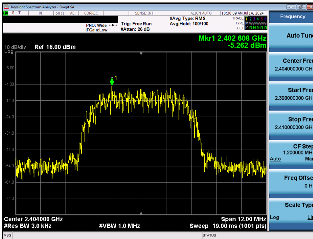
Plot 7-13. Power Spectral Density Plot (Bluetooth (HDR8), 8Mbps, ePA – Ch. 1)
