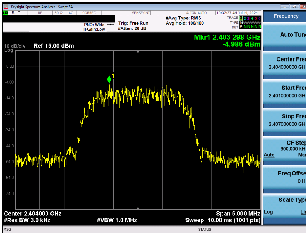
Plot 7-7. Power Spectral Density Plot (Bluetooth (HDR4), 4Mbps, ePA – Ch. 1)
