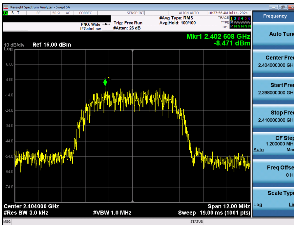
Plot 7-16. Power Spectral Density Plot (Bluetooth (HDR8), 8Mbps, iPA – Ch. 1)
