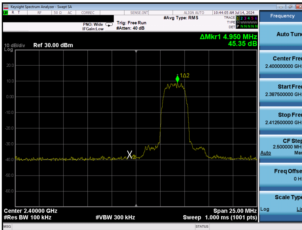
Plot 7-19. Band Edge Plot (Bluetooth (HDR4), ePA – Ch. 1)
