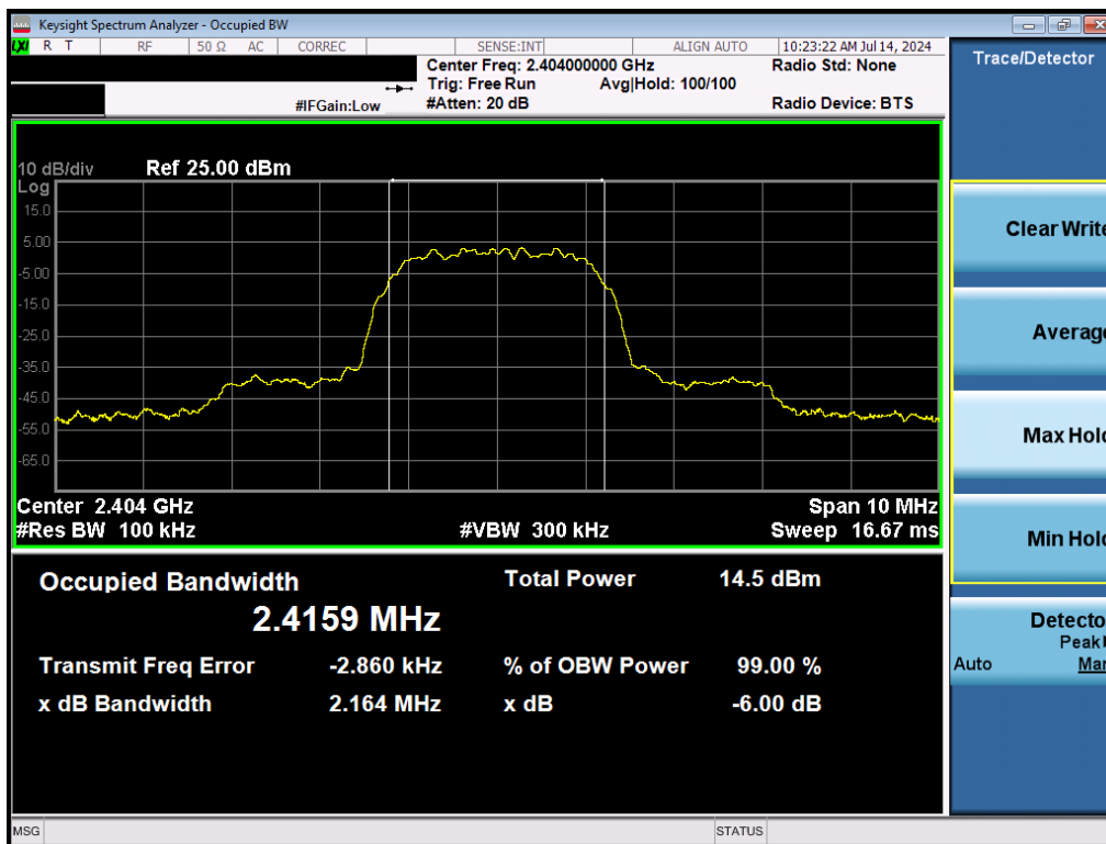
Plot 7-1. 6dB BW & 99% OBW Plot (Bluetooth (HDR4), 4Mbps, ePA – Ch. 1)
