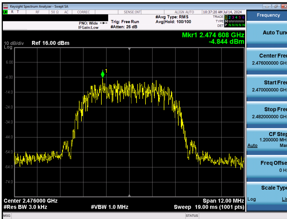
Plot 7-15. Power Spectral Density Plot (Bluetooth (HDR8), 8Mbps, ePA – Ch. 73)
