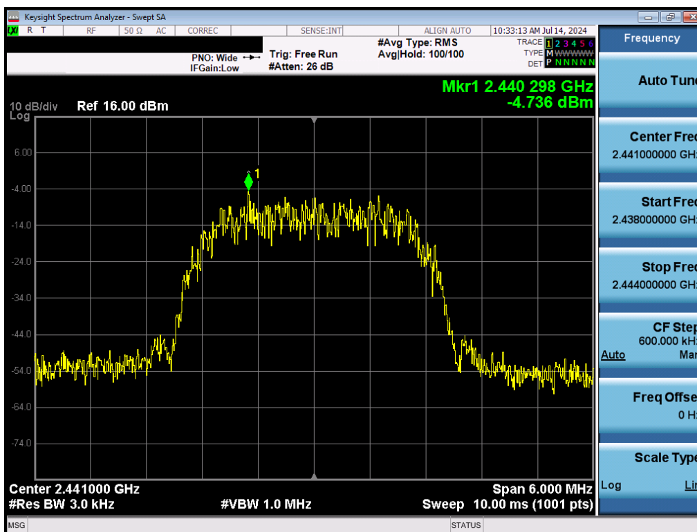
Plot 7-8. Power Spectral Density Plot (Bluetooth (HDR4), 4Mbps, ePA – Ch. 38)
