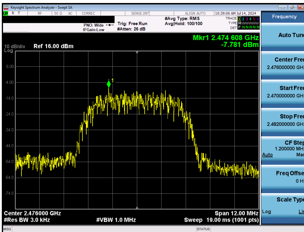
Plot 7-18. Power Spectral Density Plot (Bluetooth (HDR8), 8Mbps, iPA – Ch. 73)
