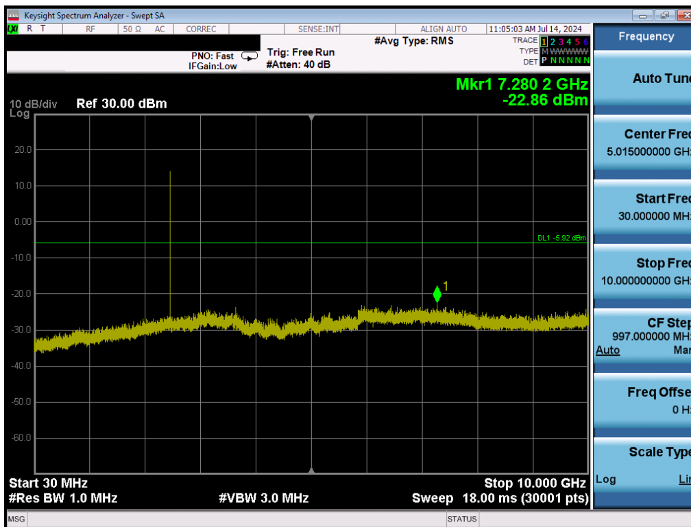
Plot 7-27. Conducted Spurious Plot (Bluetooth (HDR4), ePA – Ch. 73)
