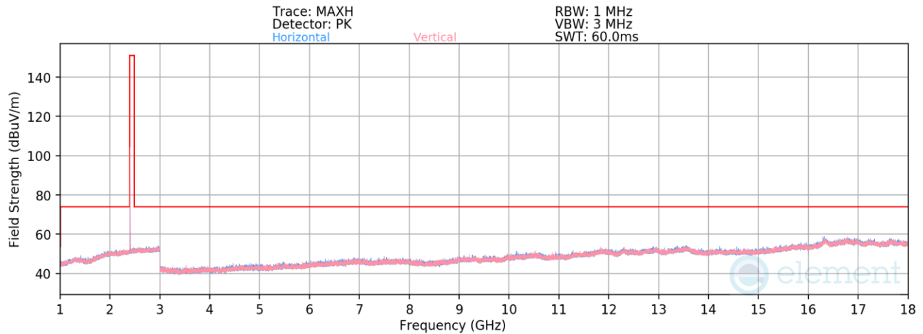
Plot 7-29. Radiated Spurious Emissions 1-18GHz (4Mbps, HDR4, ePA – Ch. 1)
