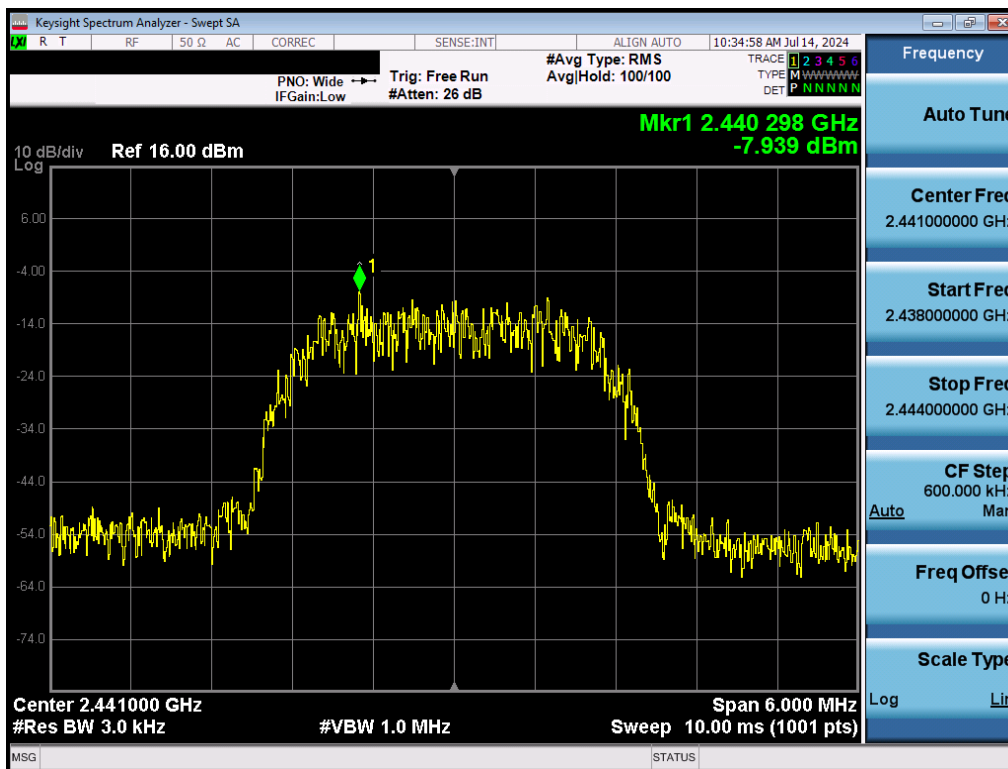
Plot 7-11. Power Spectral Density Plot (Bluetooth (HDR4), 4Mbps, iPA – Ch. 38)
