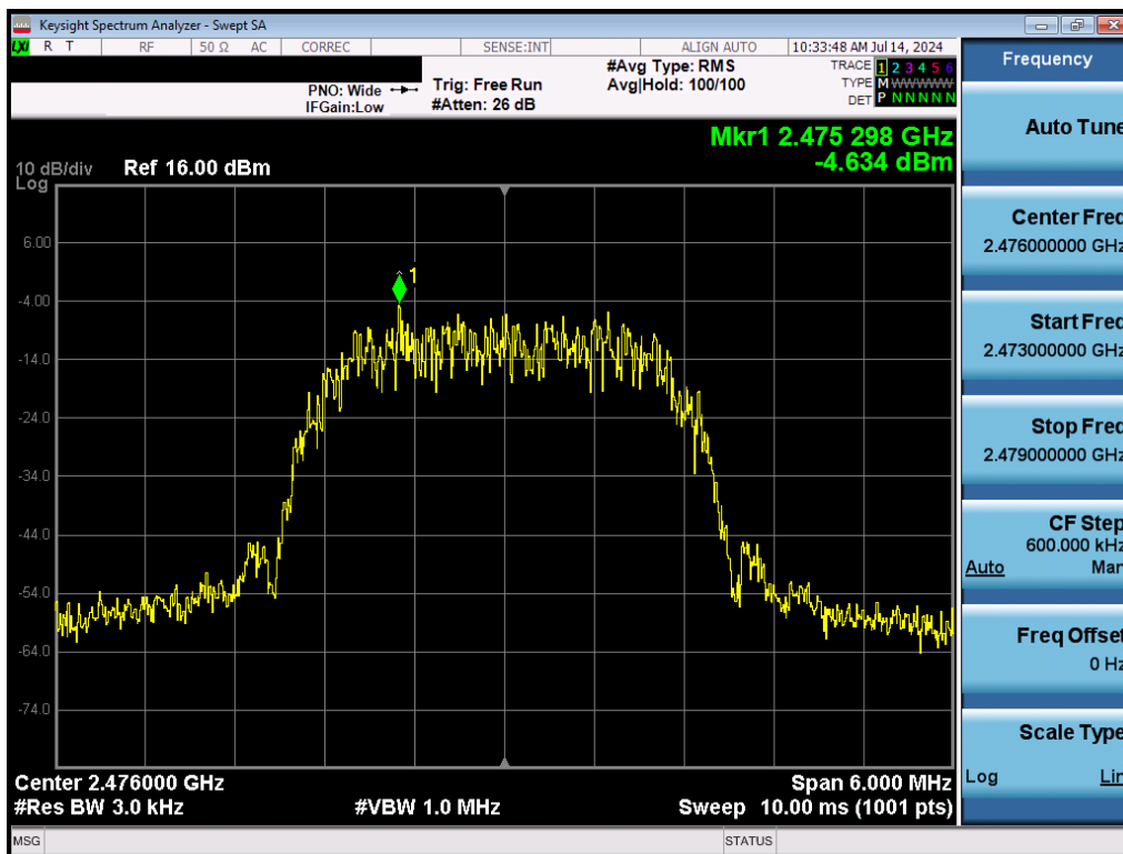
Plot 7-9. Power Spectral Density Plot (Bluetooth (HDR4), 4Mbps, ePA – Ch. 73)
