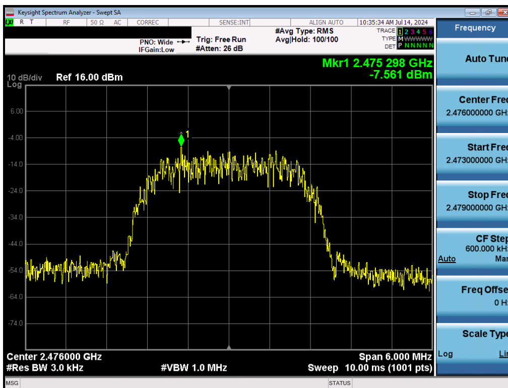
Plot 7-12. Power Spectral Density Plot (Bluetooth (HDR4), 4Mbps, iPA – Ch. 73)
