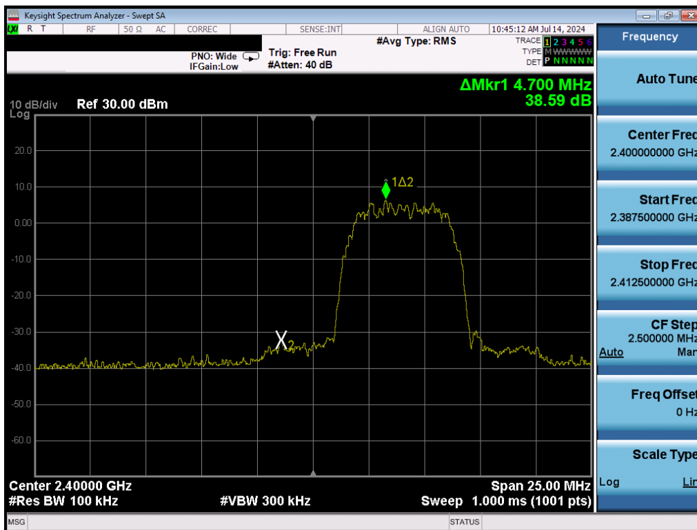
Plot 7-21. Band Edge Plot (Bluetooth (HDR8), ePA – Ch. 1)
