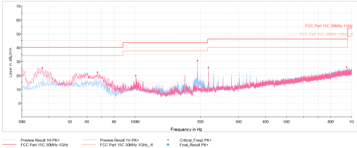
Plot 7-37. Radiated Spurious Emissions Below 1GHz (1Mbps, ePA – Ch.19, Pol. H & V, with AC/DC Adapter + Magnetic Charger)
