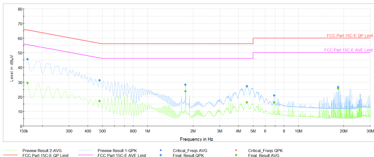
Plot 7-38. AC Line Conducted Plot with Bluetooth LE (L1, 1Mbps ePA – Ch.19 with AC/DC Adapter + Magnetic Charger)
