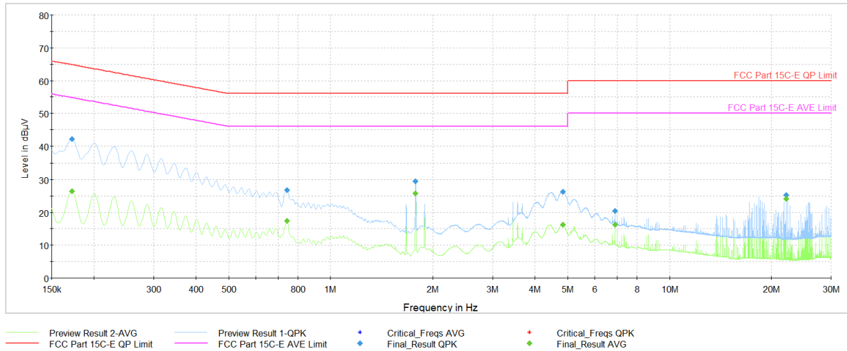
Plot 7-39. AC Line Conducted Plot with Bluetooth LE (N, 1Mbps ePA – Ch.19, with AC/DC Adapter + Magnetic Charger)
