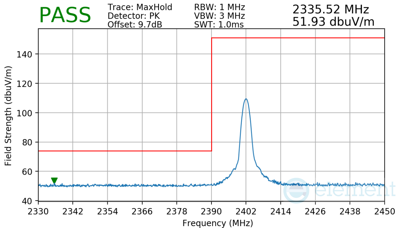
Plot 7-39. Radiated Restricted Lower Band Edge Measurement
