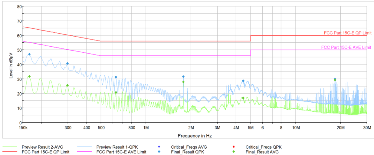
Plot 7-45. AC Line-Conducted Test Plot (N, GFSK ePA – Ch.39, with AC/DC Adapter + Magnetic Charger)
