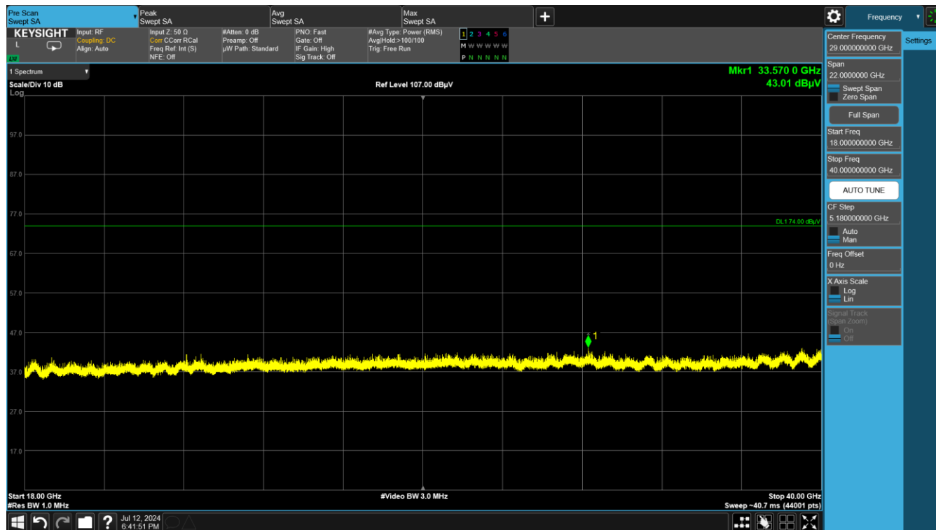
Plot 7-36. Radiated Spurious Emissions above 18GHz Simultaneous Transmission (Pol. H)
