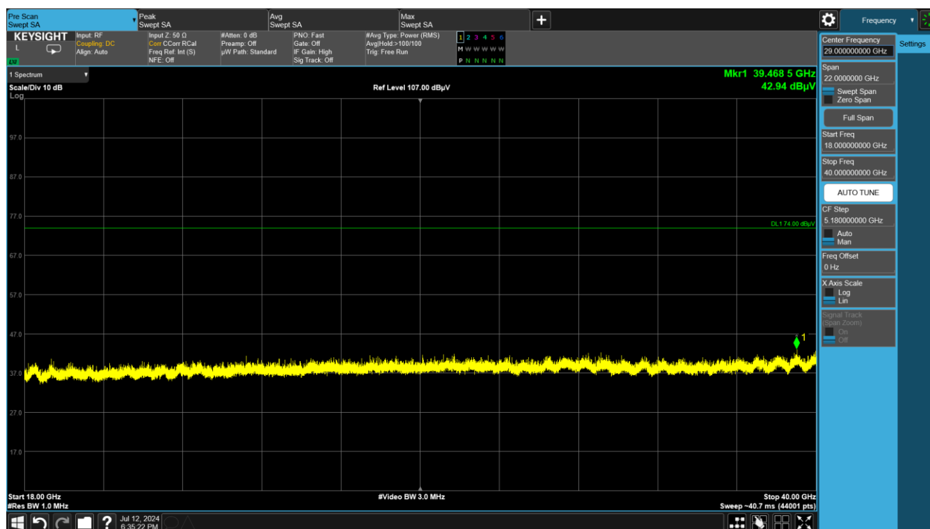
Plot 7-37. Radiated Spurious Emissions above 18GHz Simultaneous Transmission (Pol. V)
