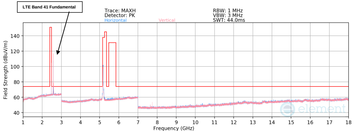
Plot 7-35. Radiated Spurious Emissions 1 - 18GHz – Simultaneous Transmission
