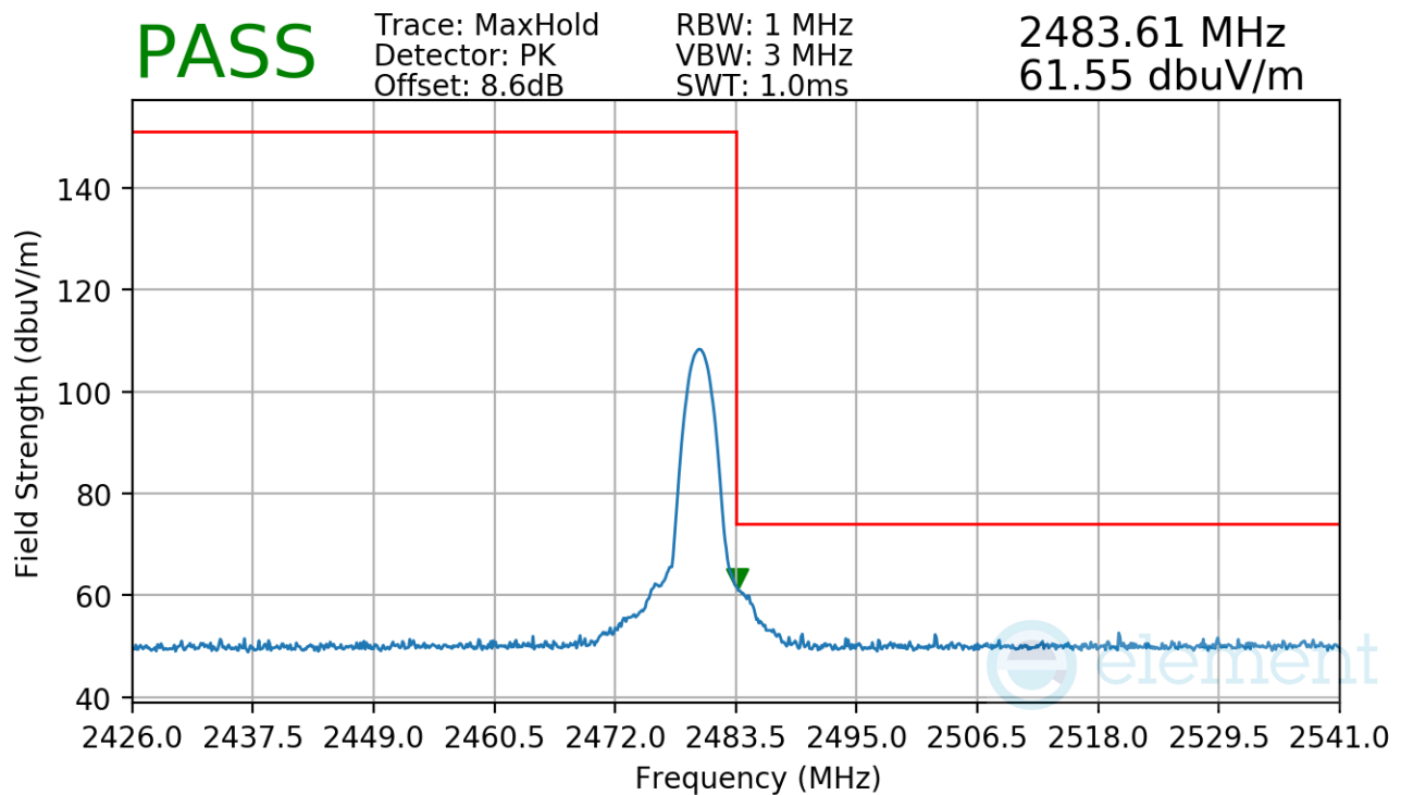
Plot 7-41. Radiated Restricted Upper Band Edge Measurement
