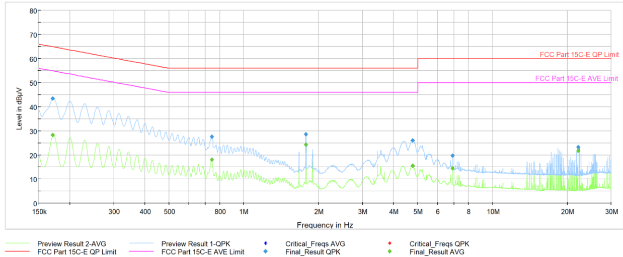
Plot 7-44. AC Line-Conducted Test Plot (L1, GFSK ePA – Ch.39, with AC/DC Adapter + Magnetic Charger)
