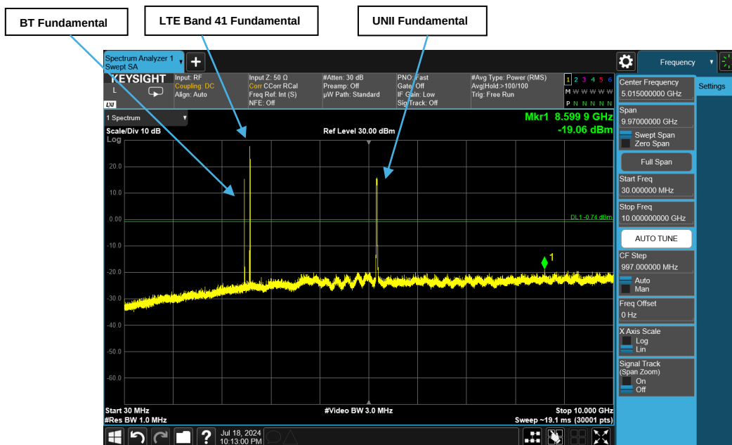
Plot 7-29. Conducted Simultaneous Tx Spurious Plot
