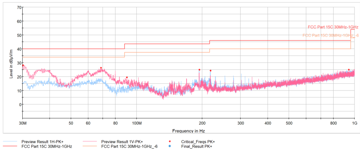
Plot 7-42. Radiated Spurious Emissions Below 1GHz (GFSK ePA – Ch.39, with AC/DC Adapter & Magnetic Charger)
