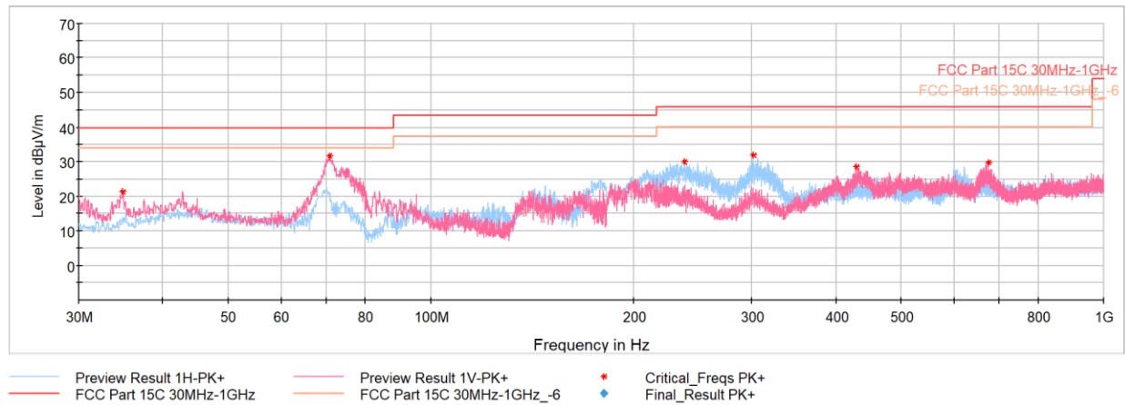
Plot 7-43. Radiated Spurious Emissions Below 1GHz – Simultaneous Transmission
