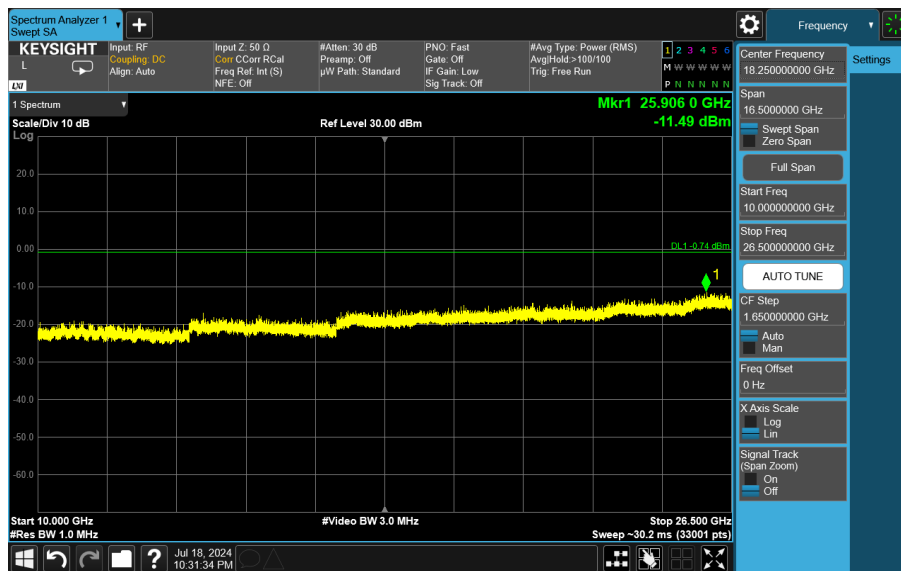
Plot 7-30. Conducted Simultaneous Tx Spurious Plot
