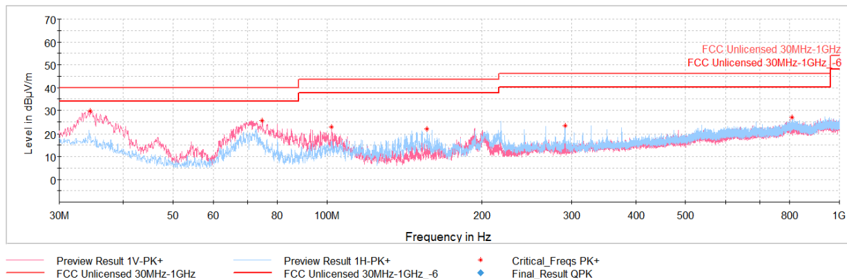
Plot 7-11. Radiated Spurious Emissions 30MHz – 1GHz (Reader B 848kbps, with AC/DC Adapter and Magnetic Charger)
