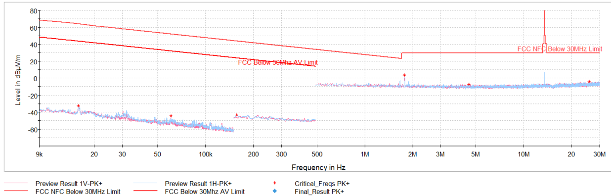
Plot 7-9. Radiated Spurious Emissions 9kHz – 30MHz (Reader B 848kbps, with AC/DC Adapter and Magnetic Charger)
