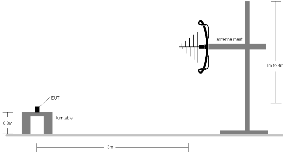
Figure 7-7. Radiated Test Setup > 30MHz
