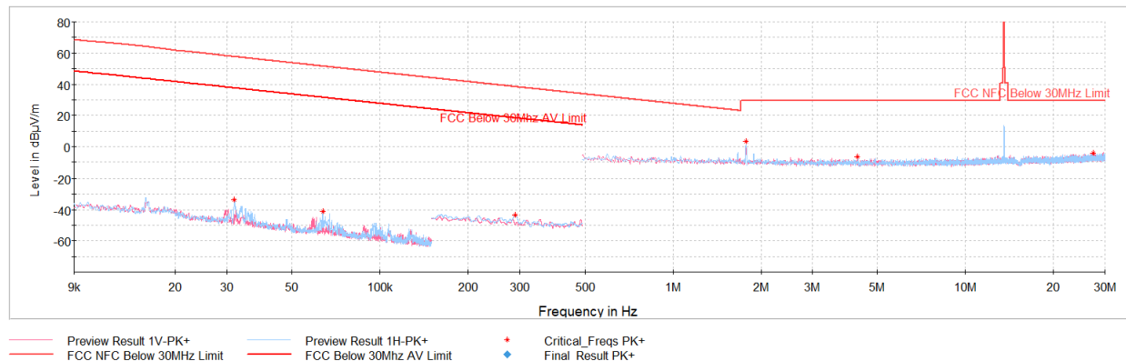
Plot 7-8. Radiated Spurious Emissions 9kHz – 30MHz (CE F 424kbps, with AC/DC Adapter and Magnetic Charger)
