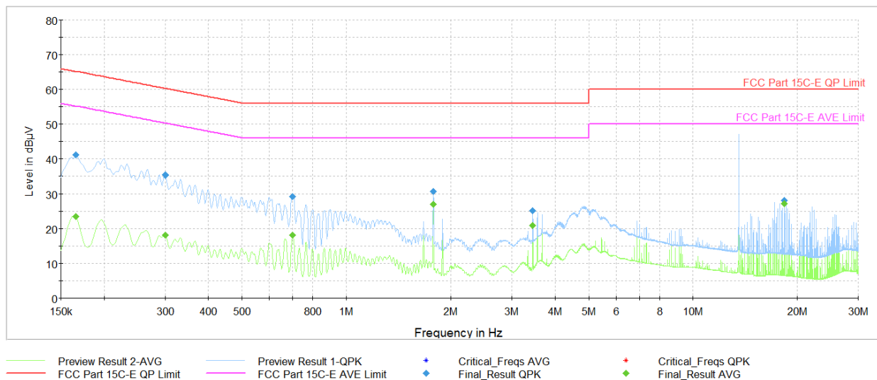
Plot 7-15. AC Line-Conducted Plot (N, Reader B 848kbps, with AC/DC Adapter and Magnetic Charger)
