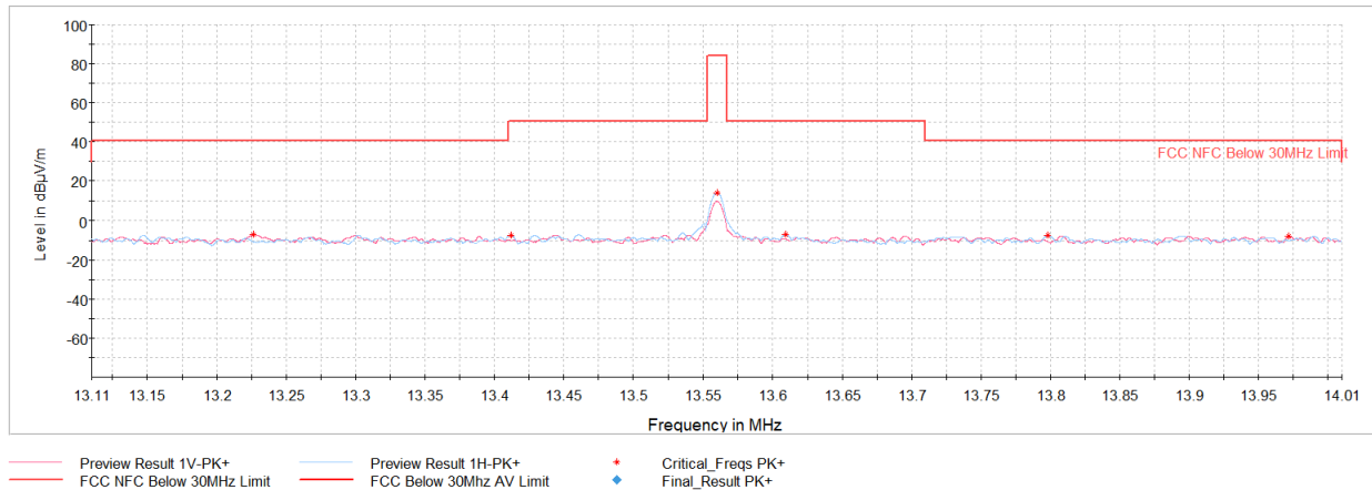
Plot 7-7. In Band Radiated Spurious Emissions (Reader B 848kbps, with AC/DC Adapter and Magnetic Charger)
