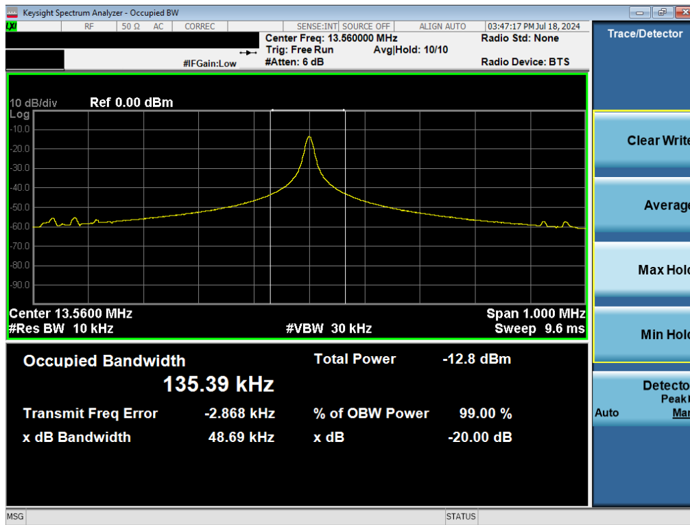
Plot 7-1. 20dB and 99% Bandwidth Plot (CE A 848kbps)
