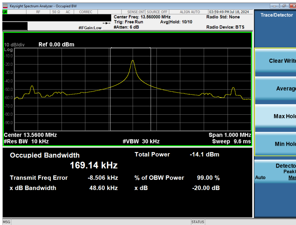
Plot 7-3. 20dB and 99% Bandwidth Plot (CE F 424kbps)
