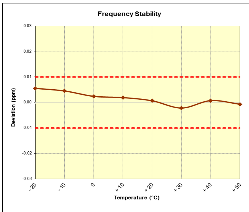
Figure 7-3. Frequency Stability Plot (CE F 424kbps)
