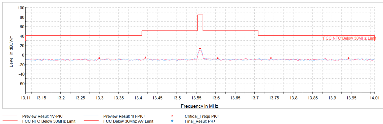
Plot 7-6. In Band Radiated Spurious Emissions (CE F 424kbps, with AC/DC Adapter and Magnetic Charger)
