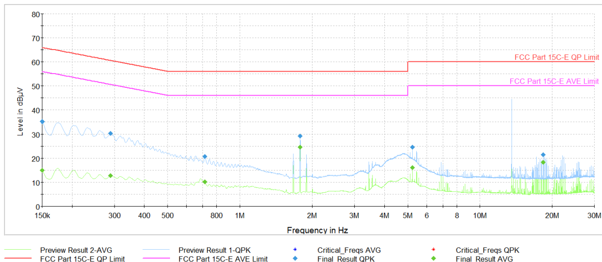
Plot 7-14. AC Line-Conducted Plot (L1, Reader B 848kbps, with AC/DC Adapter and Magnetic Charger)
