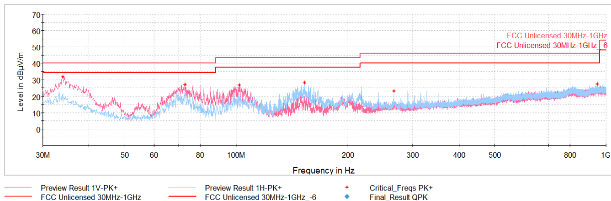
Plot 7-10. Radiated Spurious Emissions 30MHz – 1GHz (CE F 424kbps, with AC/DC Adapter and Magnetic Charger)
