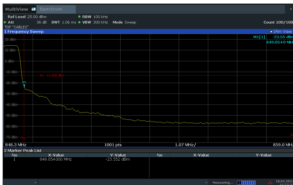
Plot 7-37. Upper BE Plot (LTE Band 5 – 1.4MHz QPSK – Full RB Configuration)
