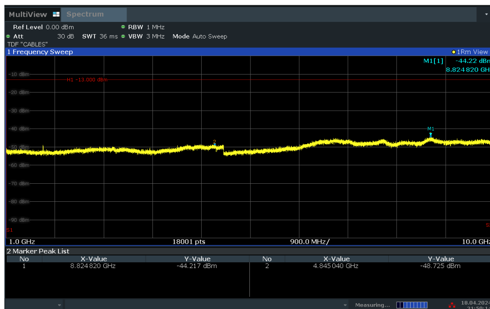
Plot 7-18. Conducted Spurious Plot (LTE Band 26/5 - 10MHz QPSK - RB Size 1, RB Offset 0 - High Channel)
