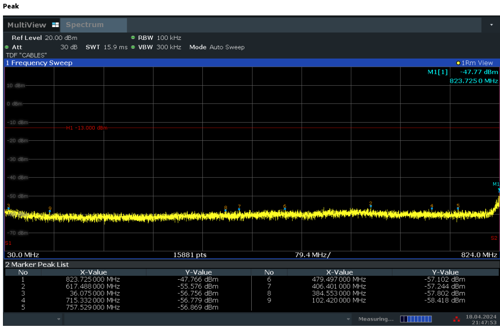
Plot 7-12. Conducted Spurious Plot (LTE Band 26/5 - 10MHz QPSK - RB Size 1, RB Offset 0 - Low Channel)
