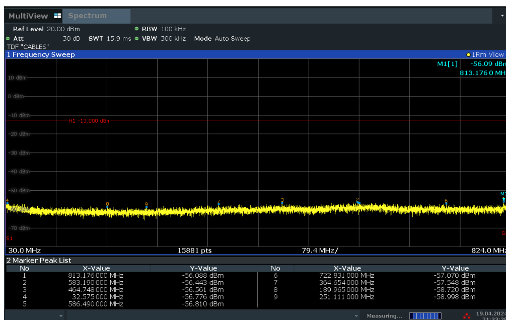
Plot 7-25. Conducted Spurious Plot (WCDMA Ch. 4233)
