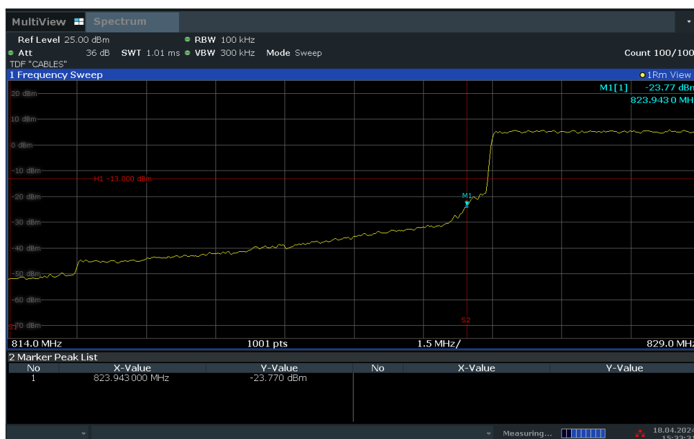
Plot 7-42. Lower BE Plot (LTE Band 5 - 10MHz QPSK – Full RB Configuration)
