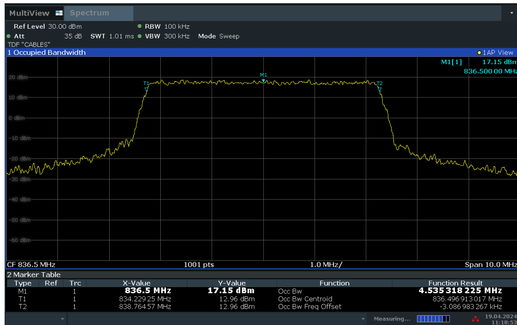
Plot 7-5. Occupied Bandwidth Plot (LTE Band 26/5 - 5MHz QPSK - Full RB Configuration)
