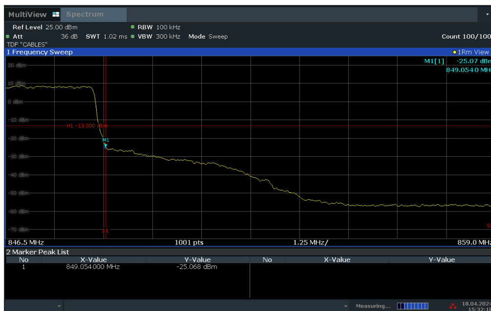
Plot 7-41. Upper BE Plot (LTE Band 5 - 5MHz QPSK – Full RB Configuration)
