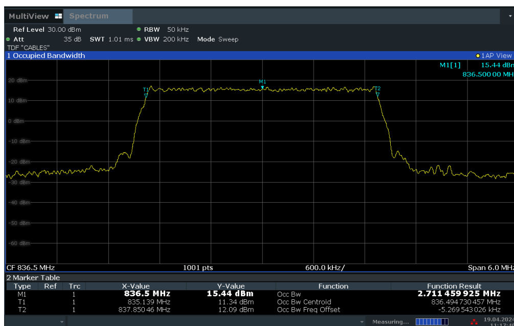
Plot 7-4. Occupied Bandwidth Plot (LTE Band 26/5 - 3MHz 16-QAM - Full RB Configuration)
