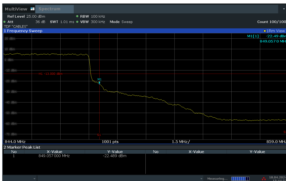
Plot 7-35. Upper BE Plot (LTE Band 26 - 10MHz QPSK – Full RB Configuration)
