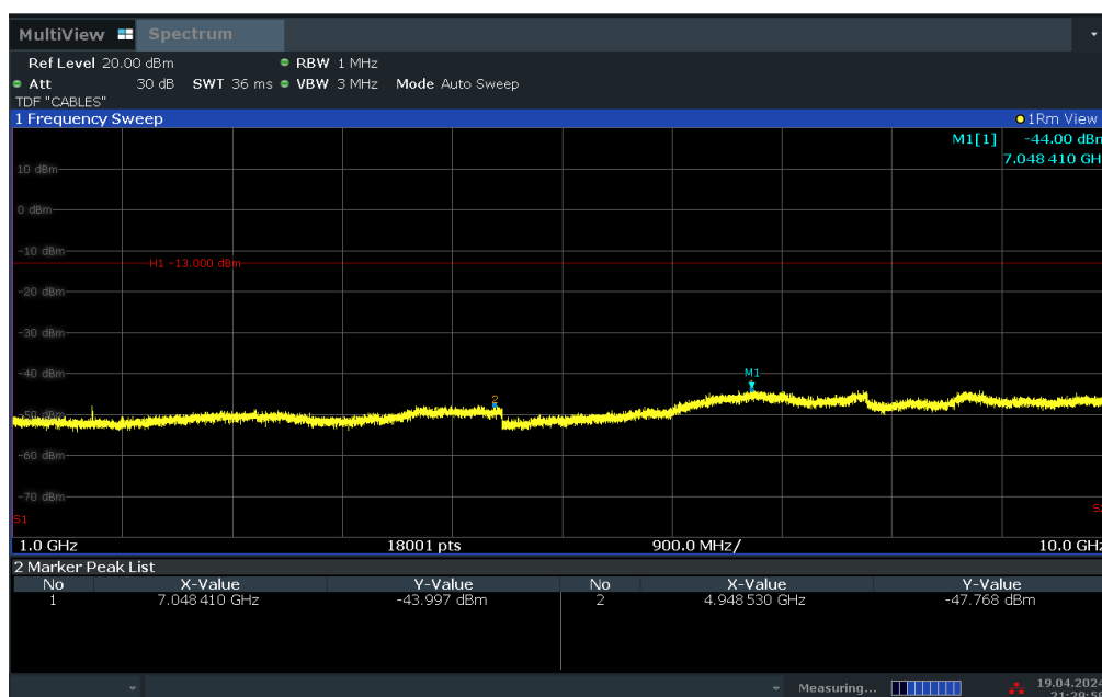
Plot 7-21. Conducted Spurious Plot (WCDMA Ch. 4132)
