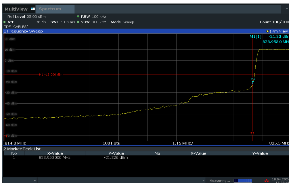
Plot 7-30. Lower BE Plot (LTE Band 26 - 3MHz QPSK – Full RB Configuration)
