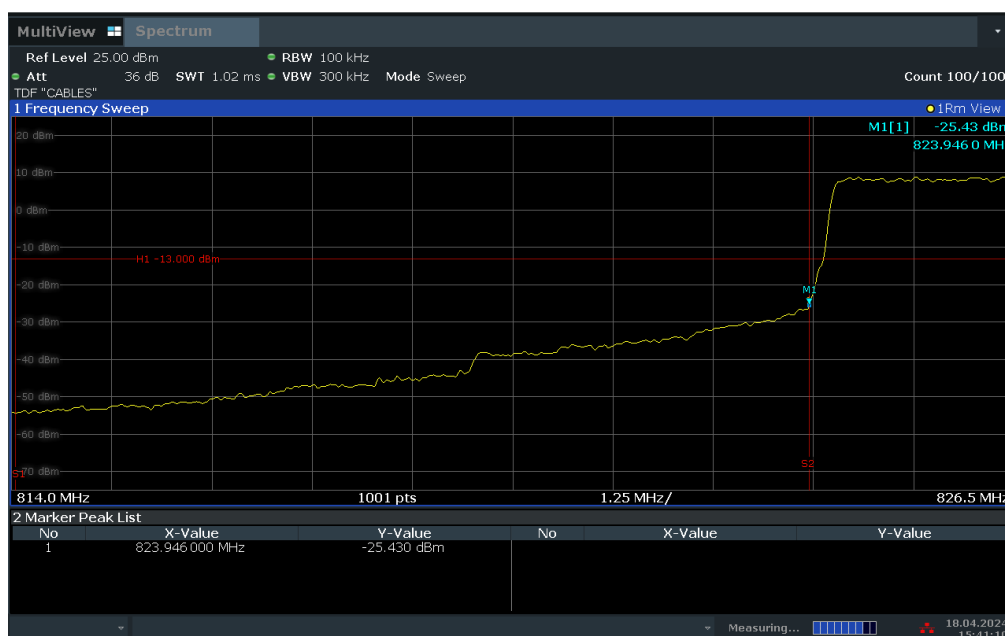
Plot 7-32. Lower BE Plot (LTE Band 26 - 5MHz QPSK – Full RB Configuration)
