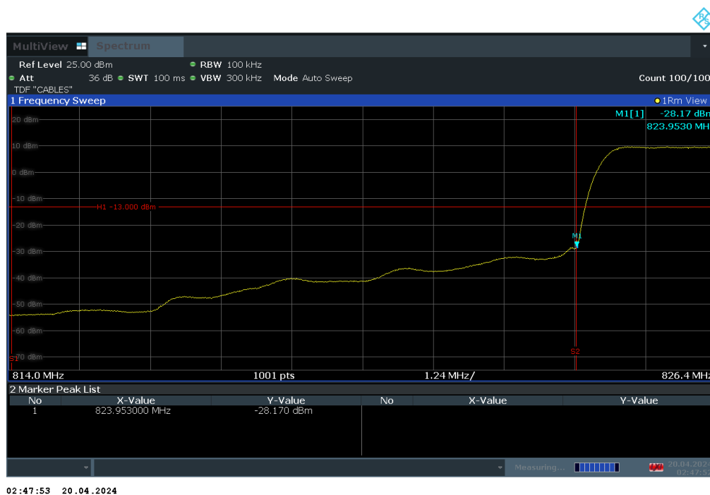
Plot 7-44. Lower BE Plot (WCDMA Cell – Ch. 4132)
