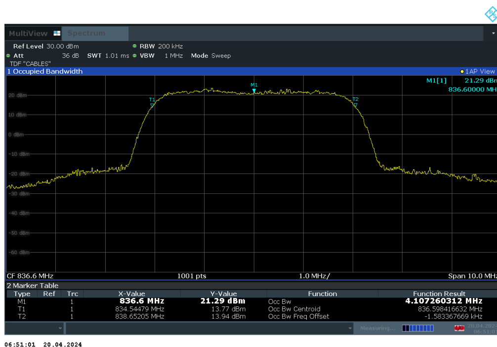
Plot 7-9. Occupied Bandwidth Plot (WCDMA, Ch. 4183)
