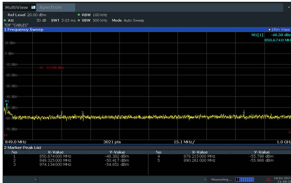
Plot 7-14. Conducted Spurious Plot (LTE Band 26/5 - 10MHz QPSK - RB Size 1, RB Offset 0 - Mid Channel)
