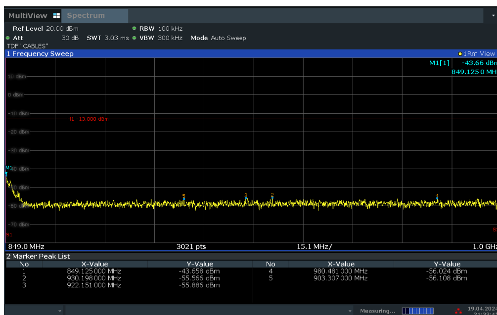
Plot 7-26. Conducted Spurious Plot (WCDMA Ch. 4233)
