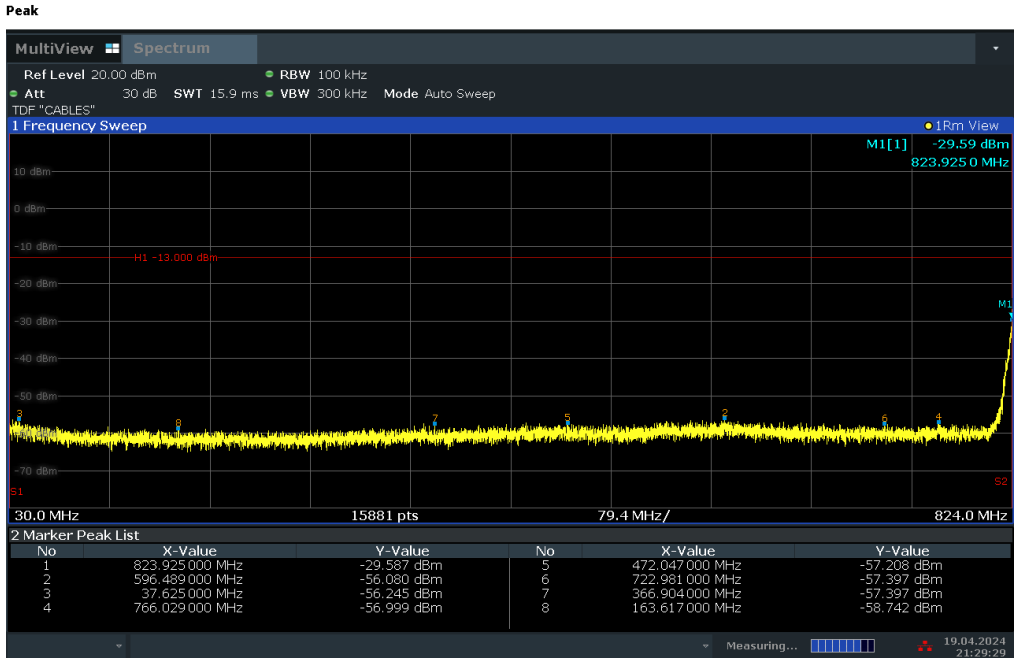
Plot 7-19. Conducted Spurious Plot (WCDMA Ch. 4132)
