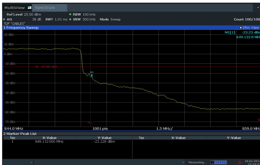
Plot 7-43. Upper BE Plot (LTE Band 5 - 10MHz QPSK – Full RB Configuration)
