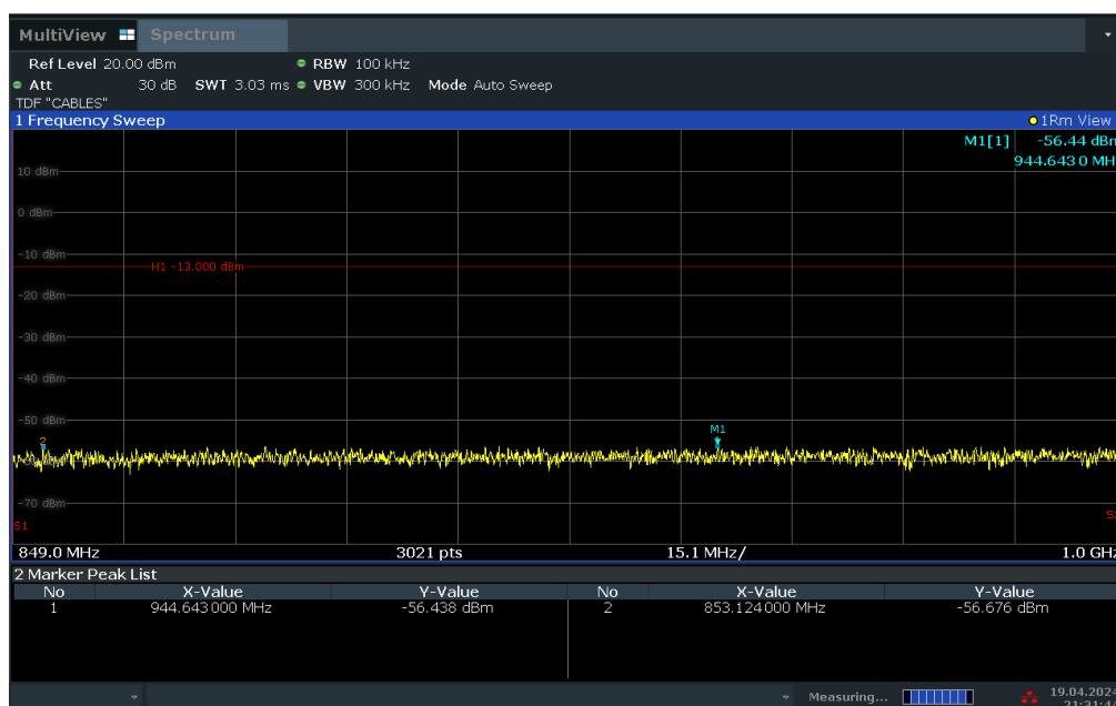
Plot 7-23. Conducted Spurious Plot (WCDMA Ch. 4183)
