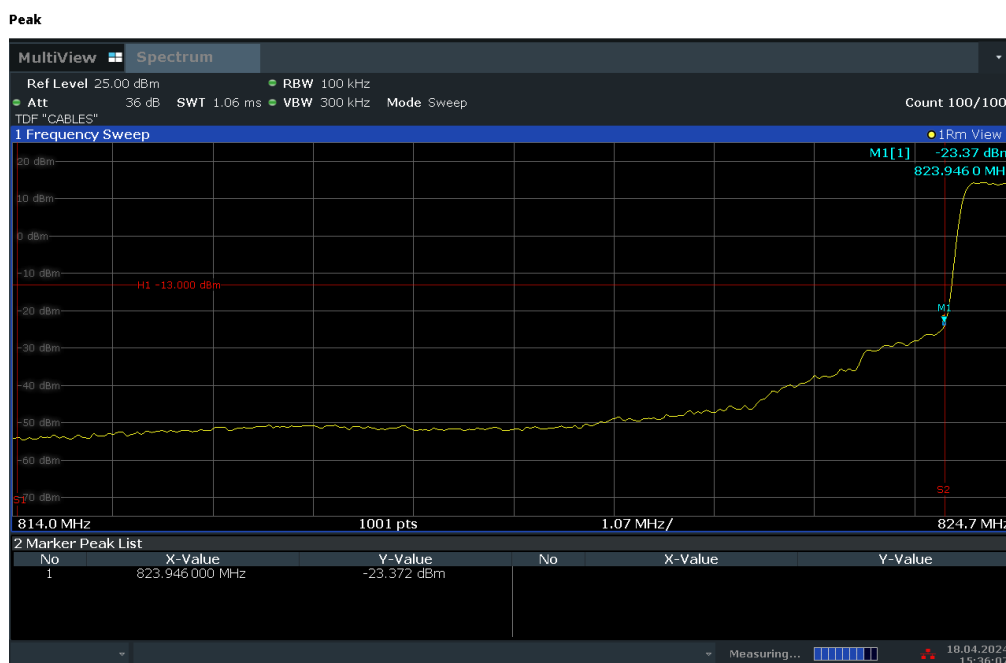
Plot 7-28. Lower BE Plot (LTE Band 26 – 1.4MHz QPSK – Full RB Configuration)
