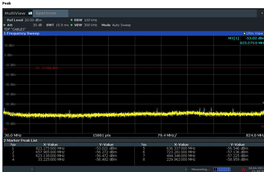
Plot 7-16. Conducted Spurious Plot (LTE Band 26/5 - 10MHz QPSK - RB Size 1, RB Offset 0 - High Channel)
