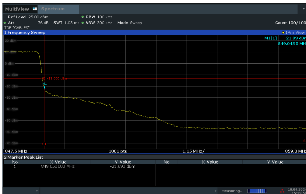
Plot 7-31. Upper BE Plot (LTE Band 26 - 3MHz QPSK – Full RB Configuration)
