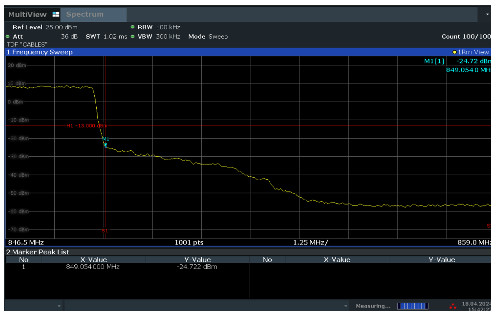
Plot 7-33. Upper BE Plot (LTE Band 26 - 5MHz QPSK – Full RB Configuration)
