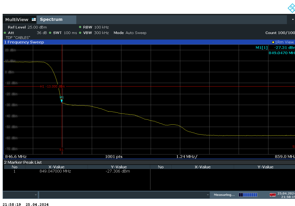
Plot 7-45. Upper BE Plot (WCDMA Cell – Ch. 4233)
