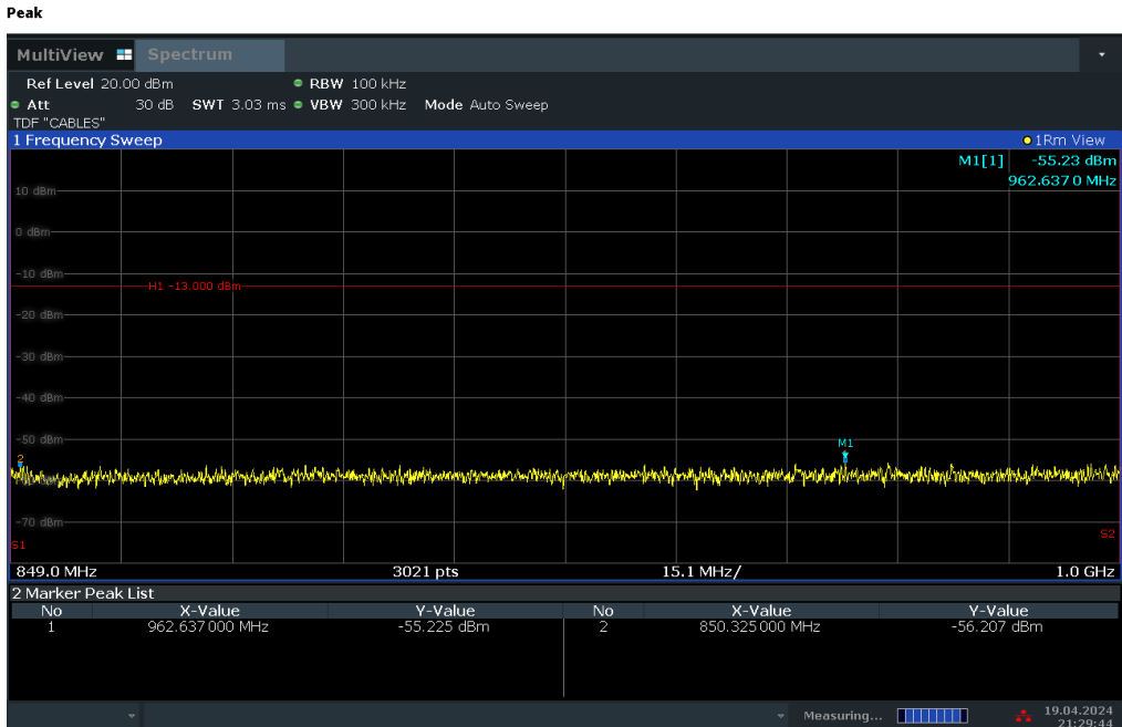
Plot 7-20. Conducted Spurious Plot (WCDMA Ch. 4132)
