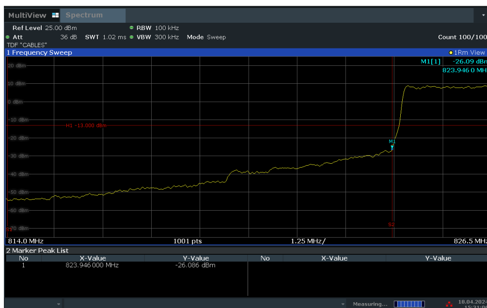
Plot 7-40. Lower BE Plot (LTE Band 5 - 5MHz QPSK – Full RB Configuration)
