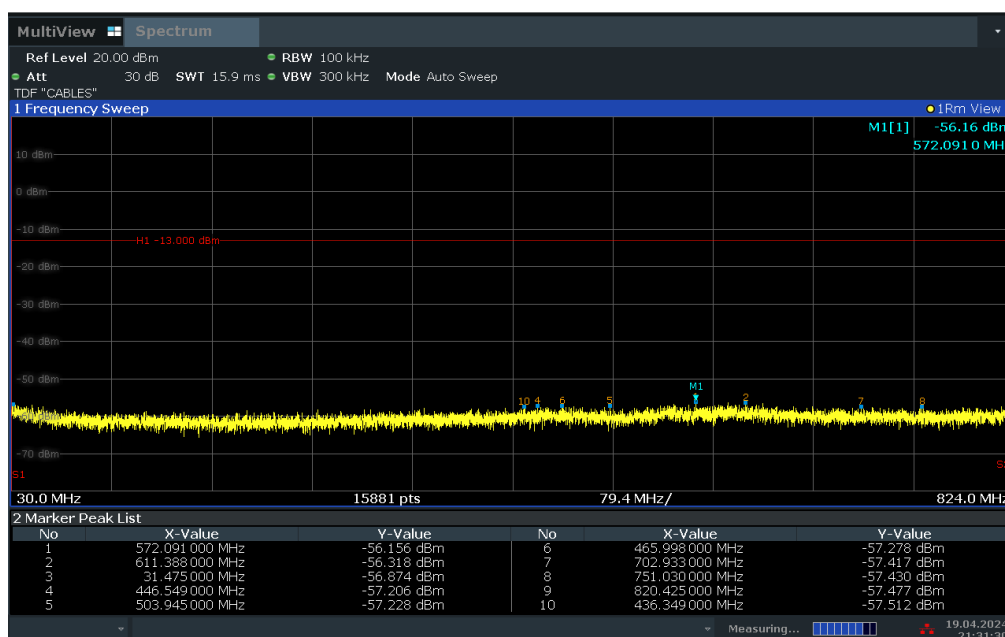
Plot 7-22. Conducted Spurious Plot (WCDMA Ch. 4183)
