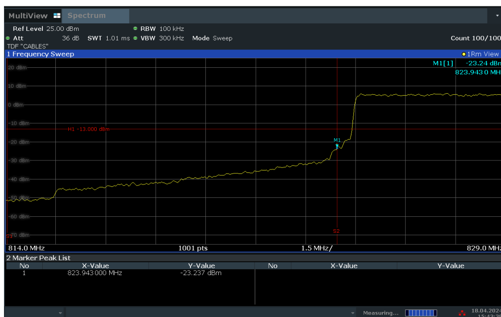
Plot 7-34. Lower BE Plot (LTE Band 26 - 10MHz QPSK – Full RB Configuration)
