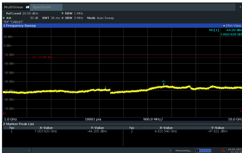
Plot 7-24. Conducted Spurious Plot (WCDMA Ch. 4183)
