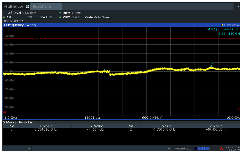
Plot 7-15. Conducted Spurious Plot (LTE Band 26/5 - 10MHz QPSK - RB Size 1, RB Offset 0 - Mid Channel)
