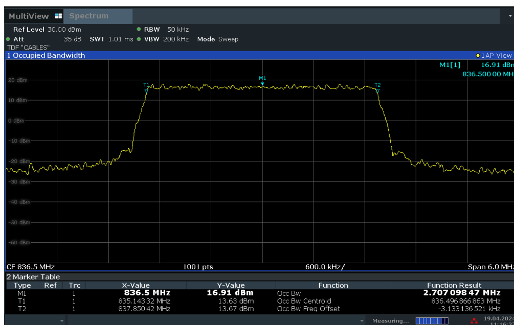
Plot 7-3. Occupied Bandwidth Plot (LTE Band 26/5 - 3MHz QPSK - Full RB Configuration)
