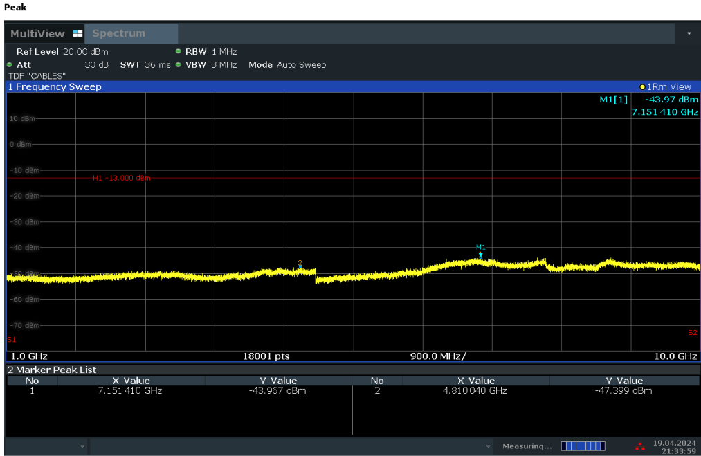
Plot 7-27. Conducted Spurious Plot (WCDMA Ch. 4233)
