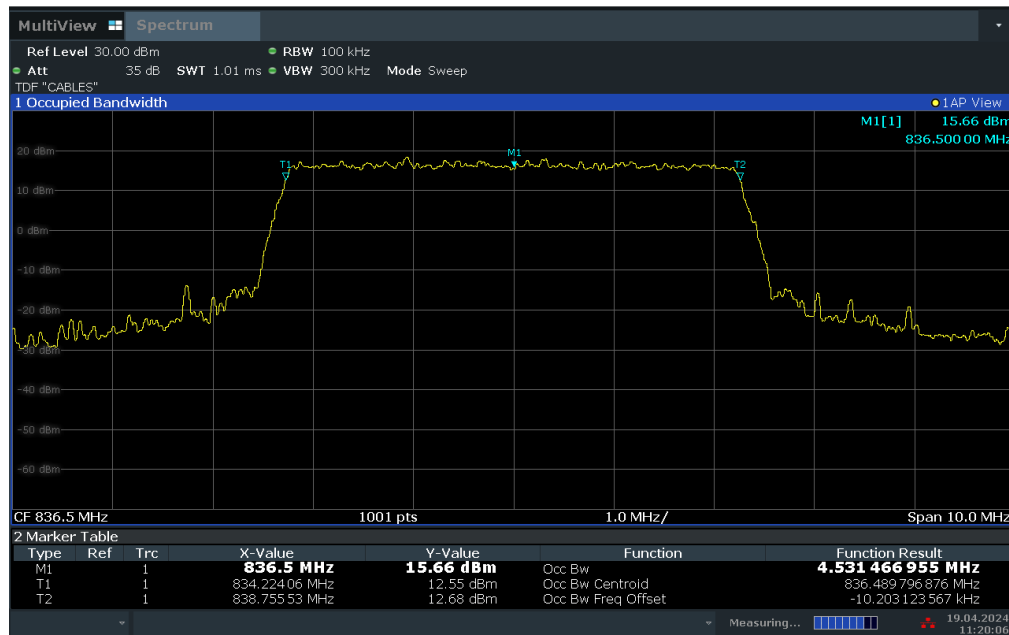
Plot 7-6. Occupied Bandwidth Plot (LTE Band 26/5 - 5MHz 16-QAM - Full RB Configuration)
