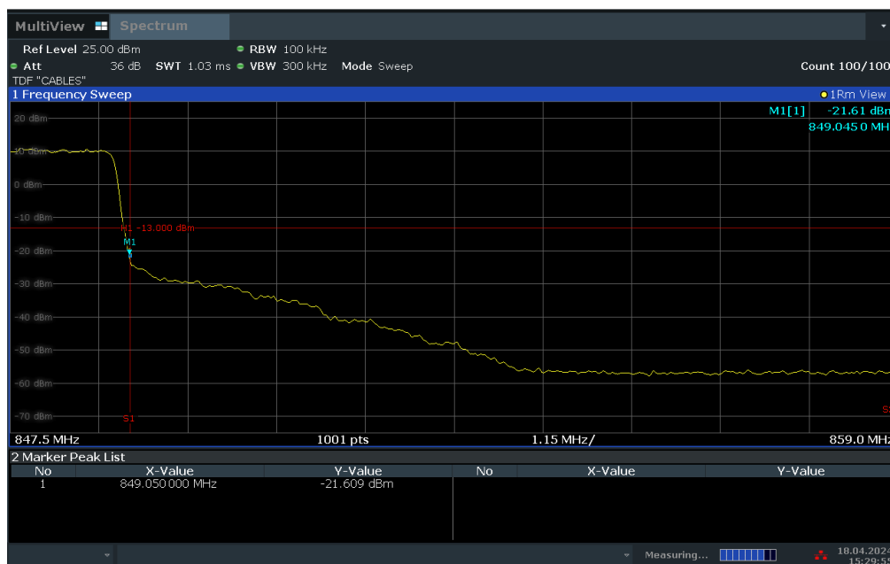
Plot 7-39. Upper BE Plot (LTE Band 5 - 3MHz QPSK – Full RB Configuration)
