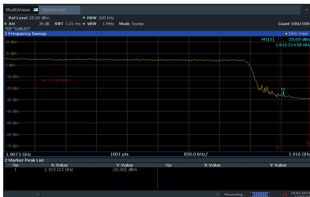
Plot 7-56. Upper Band Edge Plot (LTE Band 25 – 15MHz QPSK – Full RB Configuration)
