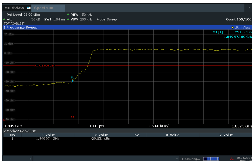
Plot 7-70. Lower Band Edge Plot (LTE Band 2 – 5MHz QPSK – Full RB Configuration)
