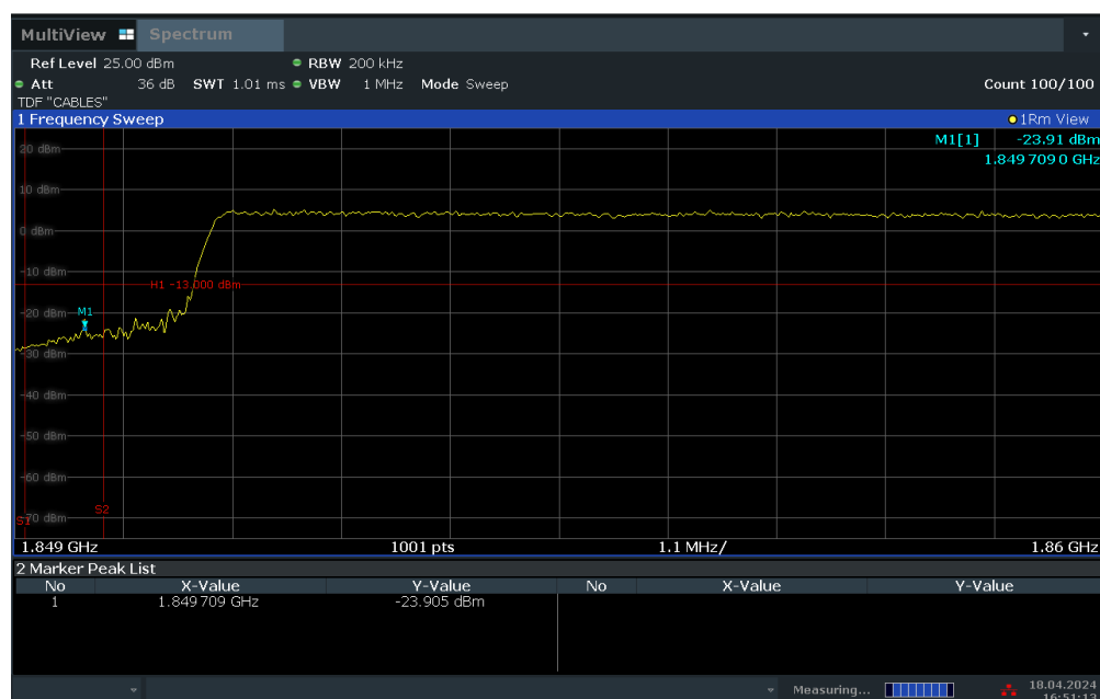
Plot 7-82. Lower Band Edge Plot (LTE Band 2 – 20MHz QPSK – Full RB Configuration)
