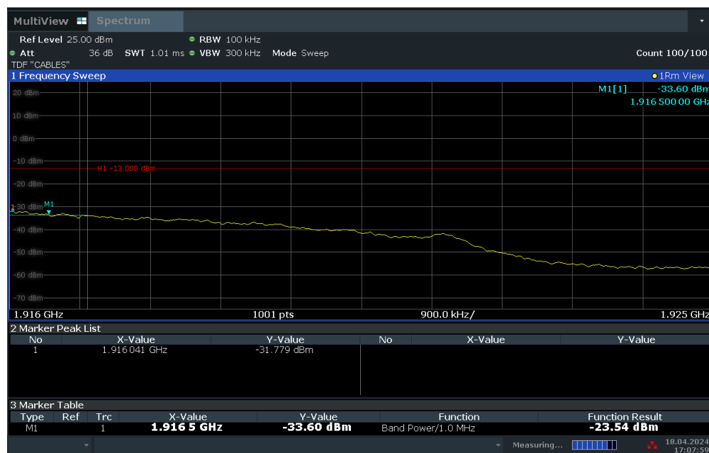
Plot 7-57. Extended Upper Band Edge Plot (LTE Band 25 – 15MHz QPSK – Full RB Configuration)
