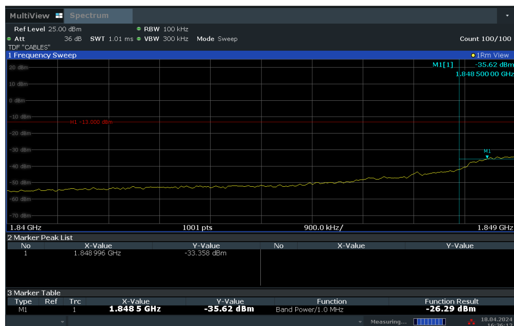
Plot 7-63. Extended Lower Band Edge Plot (LTE Band 2 – 1.4MHz QPSK – Full RB Configuration)
