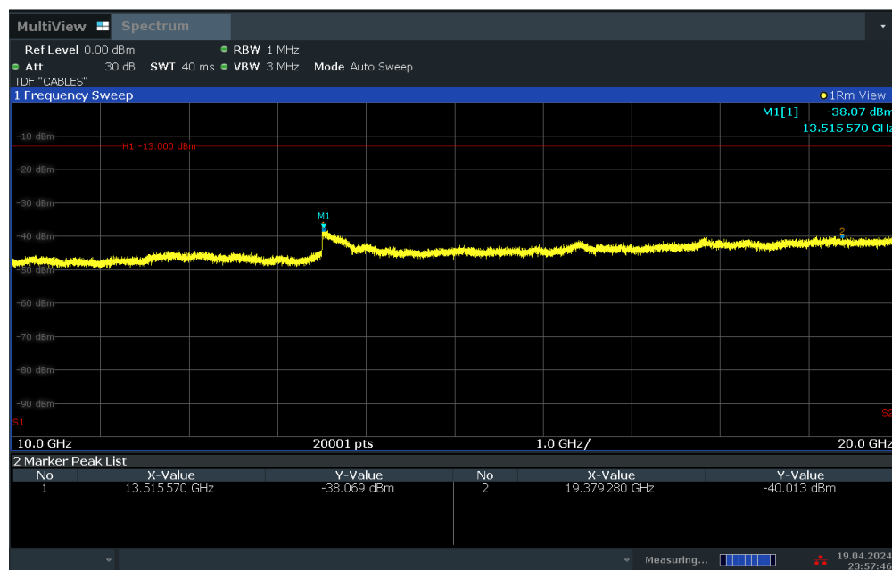
Plot 7-37. Conducted Spurious Plot (WCDMA Ch. 9538)
