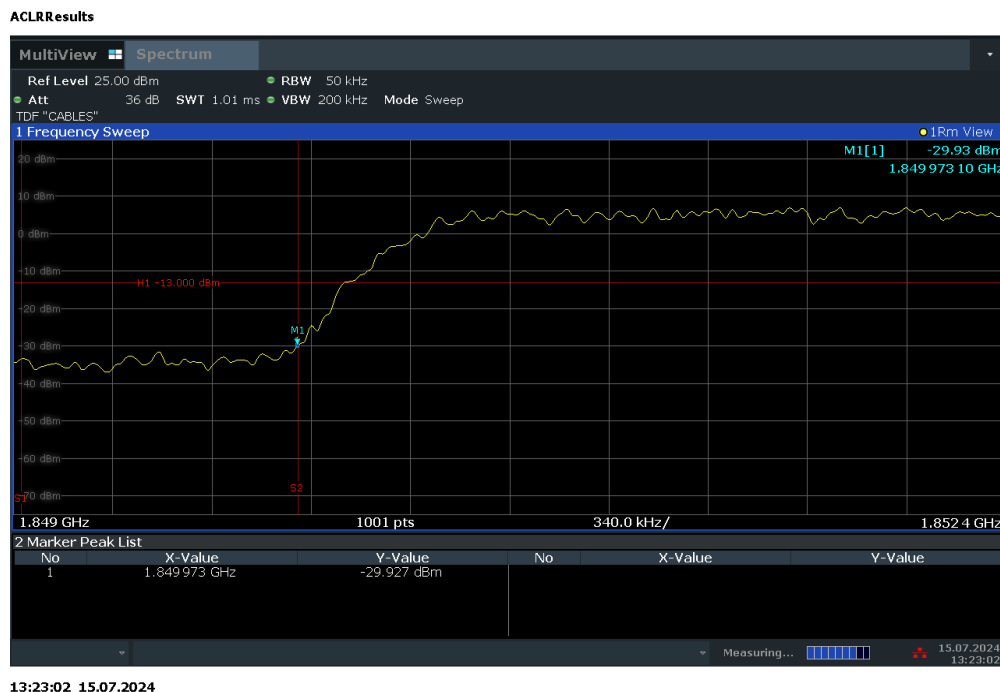
Plot 7-86. Lower Band Edge Plot (WCDMA PCS – Ch. 9262)
