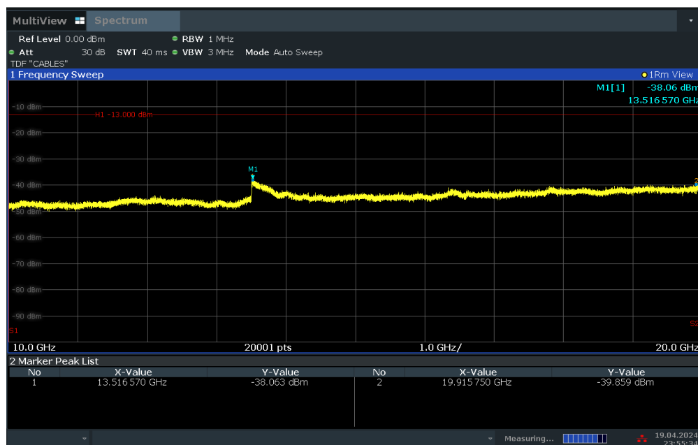
Plot 7-33. Conducted Spurious Plot (WCDMA Ch. 9400)
