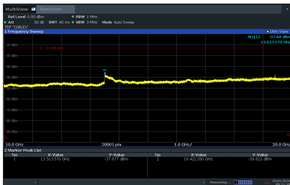
Plot 7-25. Conducted Spurious Plot (LTE Band 25/2 - 20MHz QPSK - RB Size 1, RB Offset 0 - High Channel)
