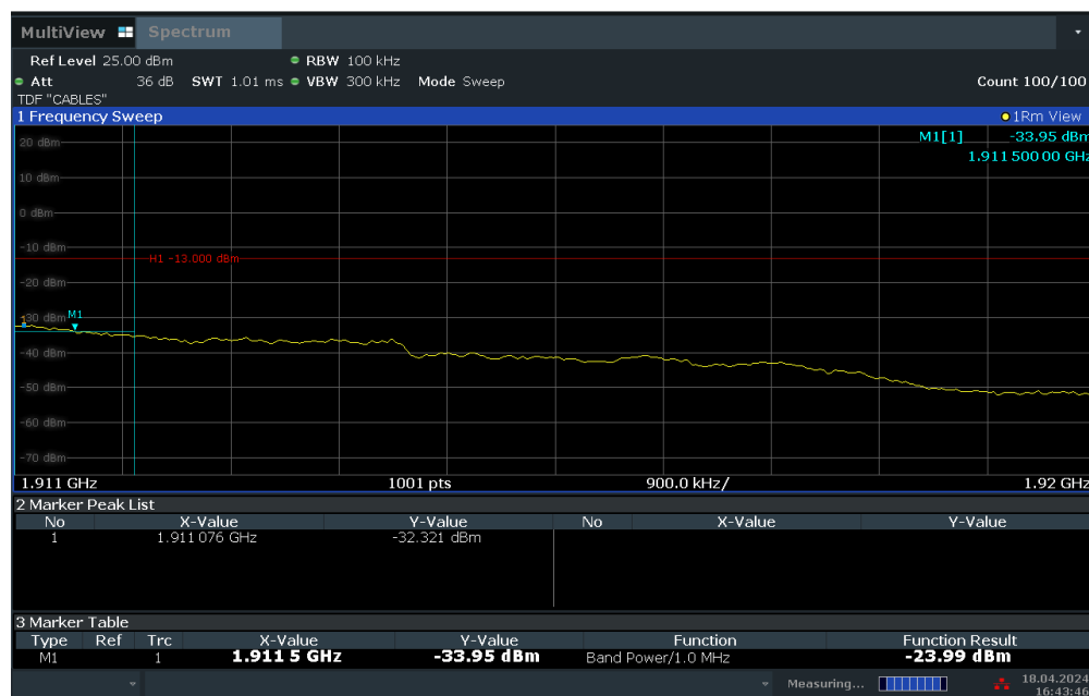
Plot 7-73. Extended Upper Band Edge Plot (LTE Band 2 – 5MHz QPSK – Full RB Configuration)
