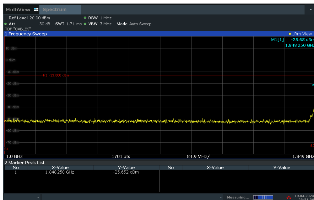
Plot 7-27. Conducted Spurious Plot (WCDMA Ch. 9262)
