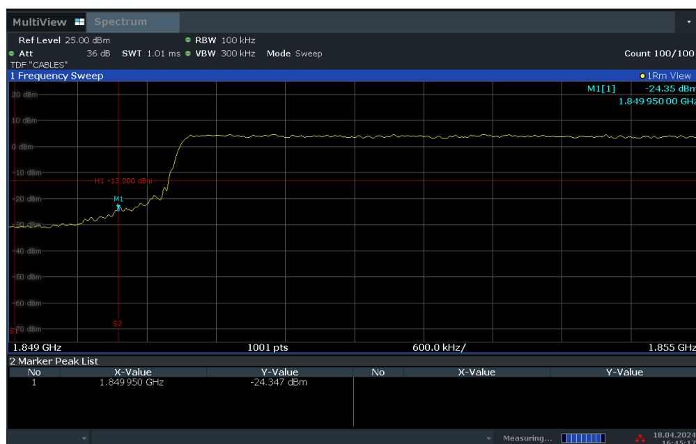
Plot 7-74. Lower Band Edge Plot (LTE Band 2 – 10MHz QPSK – Full RB Configuration)
