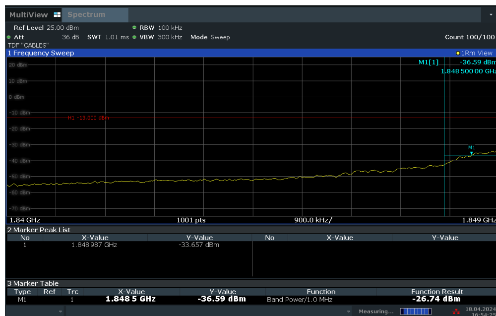
Plot 7-39. Extended Lower Band Edge Plot (LTE Band 25 – 1.4MHz QPSK – Full RB Configuration)
