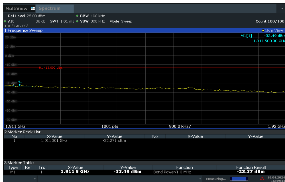
Plot 7-81. Extended Upper Band Edge Plot (LTE Band 2 – 15MHz QPSK – Full RB Configuration)
