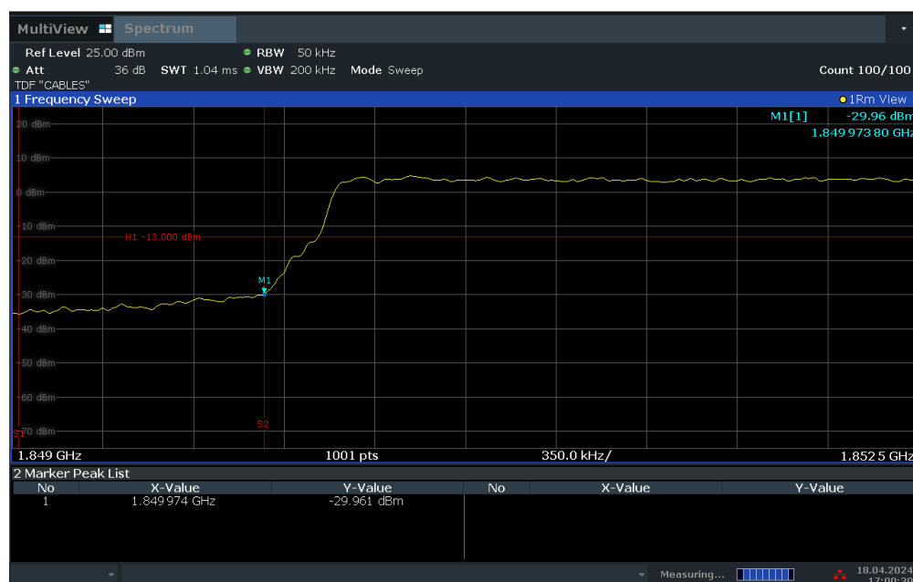
Plot 7-46. Lower Band Edge Plot (LTE Band 25 – 5MHz QPSK – Full RB Configuration)
