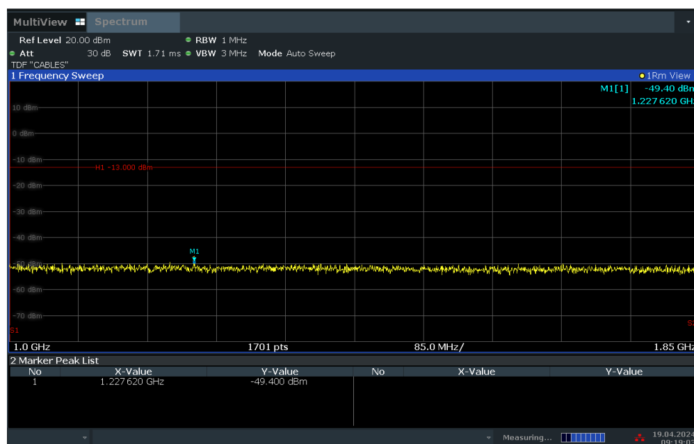
Plot 7-19. Conducted Spurious Plot (LTE Band 25/2 - 20MHz QPSK - RB Size 1, RB Offset 0 - Mid Channel)
