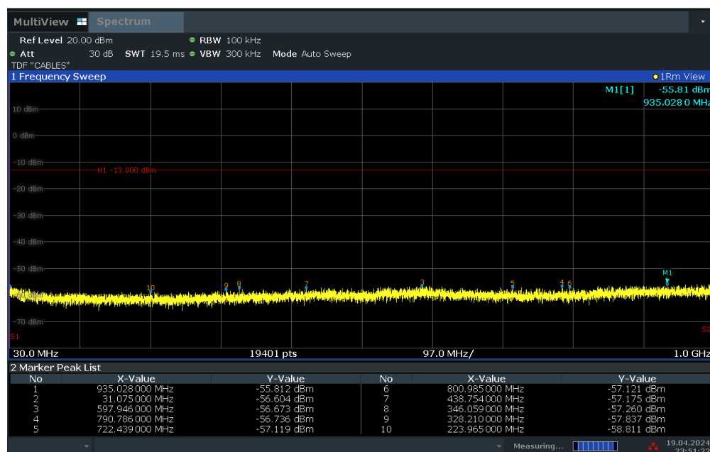
Plot 7-26. Conducted Spurious Plot (WCDMA Ch. 9262)
