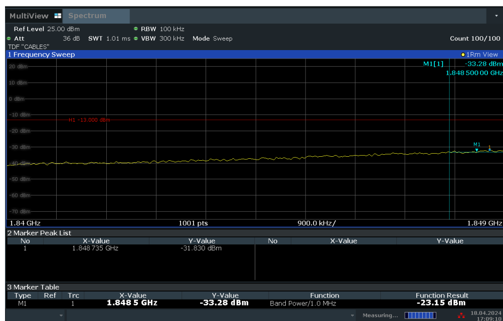
Plot 7-59. Extended Lower Band Edge Plot (LTE Band 25 – 20MHz QPSK – Full RB Configuration)
