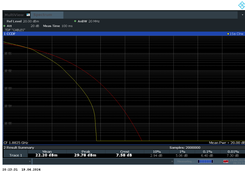
Plot 7-99. PAR Plot (LTE Band 25 - 15MHz 16-QAM - Full RB Configuration)
