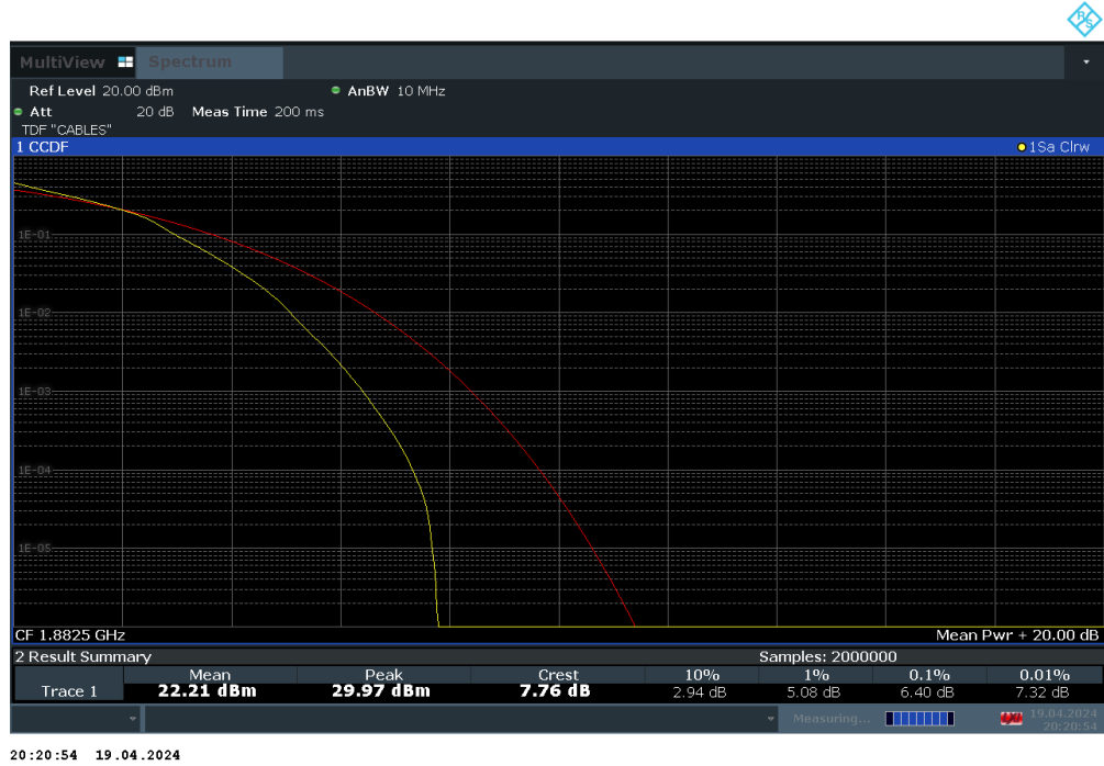
Plot 7-97. PAR Plot (LTE Band 25 - 10MHz 16-QAM - Full RB Configuration)
