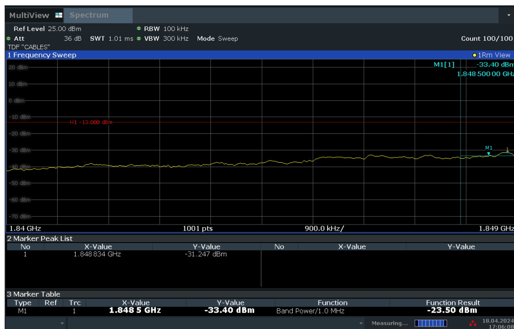
Plot 7-55. Extended Lower Band Edge Plot (LTE Band 25 – 15MHz QPSK – Full RB Configuration)
