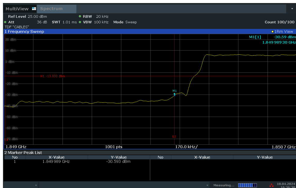
Plot 7-62. Lower Band Edge Plot (LTE Band 2 – 1.4MHz QPSK – Full RB Configuration)
