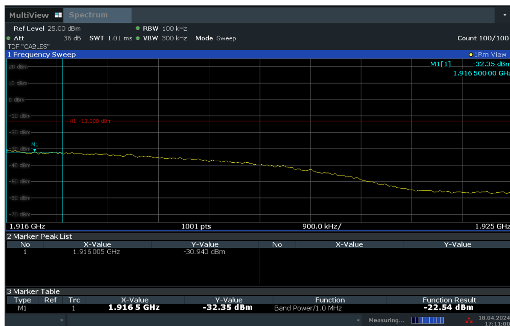
Plot 7-61. Extended Upper Band Edge Plot (LTE Band 25 – 20MHz QPSK – Full RB Configuration)
