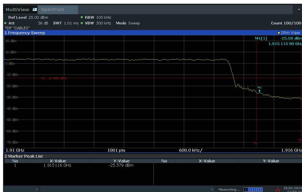
Plot 7-52. Upper Band Edge Plot (LTE Band 25 – 10MHz QPSK – Full RB Configuration)
