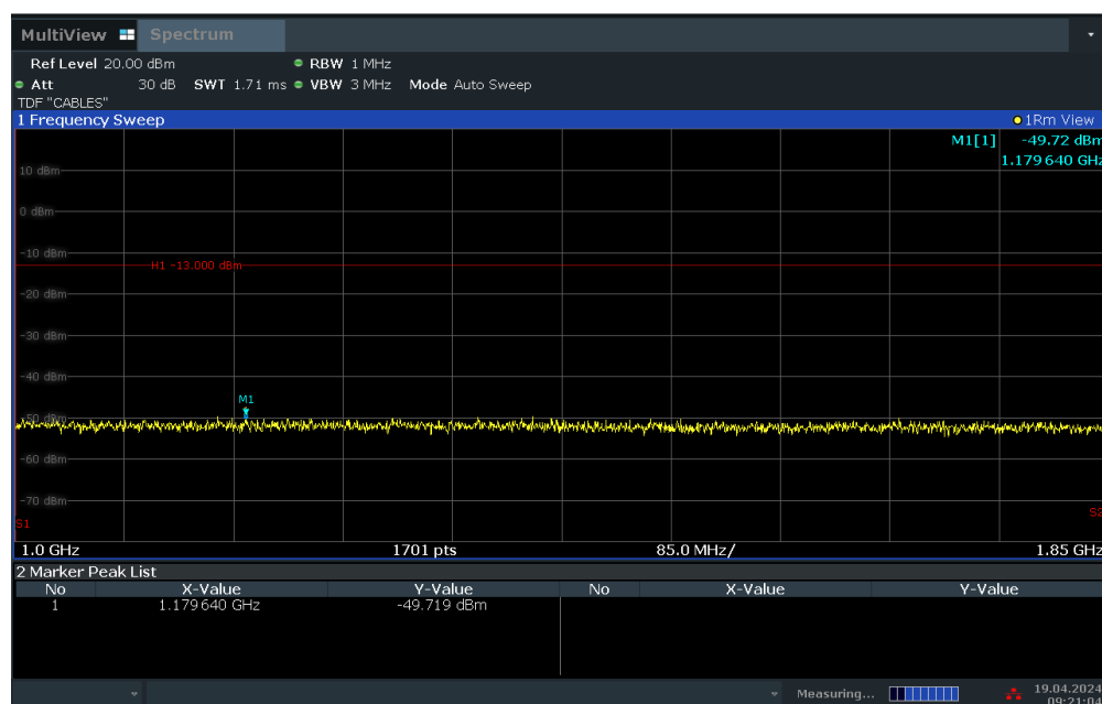
Plot 7-23. Conducted Spurious Plot (LTE Band 25/2 - 20MHz QPSK - RB Size 1, RB Offset 0 - High Channel)
