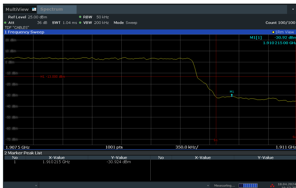
Plot 7-72. Upper Band Edge Plot (LTE Band 2 – 5MHz QPSK – Full RB Configuration)
