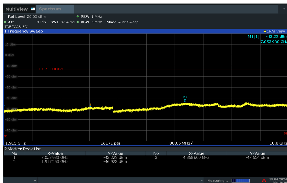
Plot 7-20. Conducted Spurious Plot (LTE Band 25/2 - 20MHz QPSK - RB Size 1, RB Offset 0 - Mid Channel)
