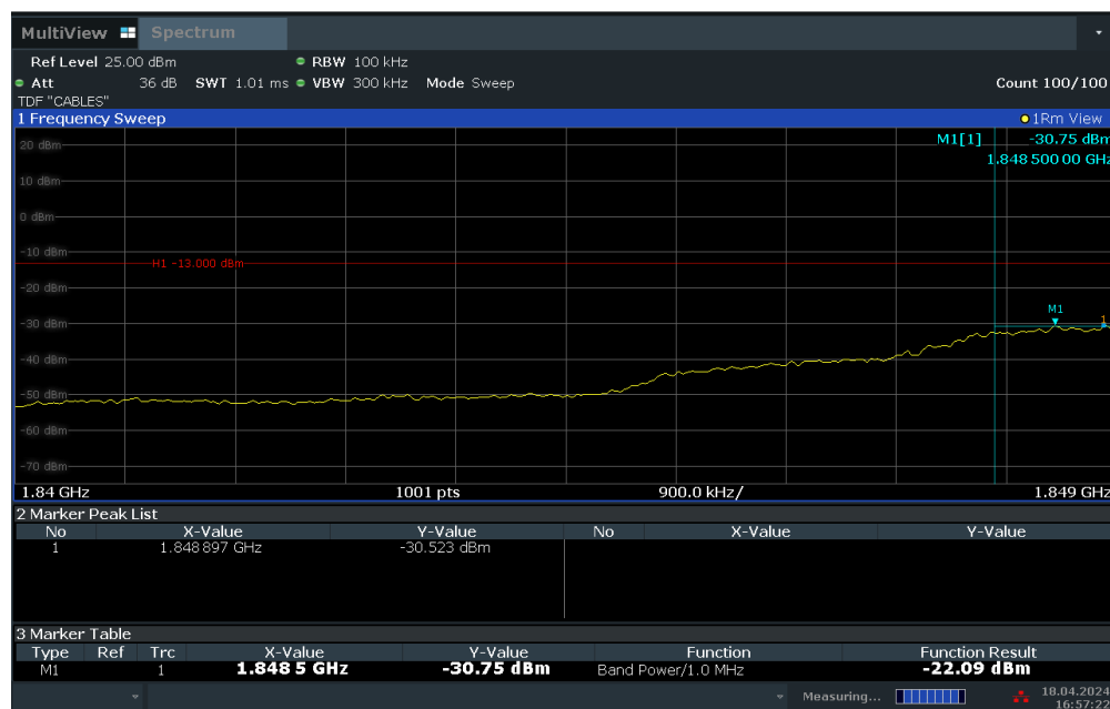
Plot 7-43. Extended Lower Band Edge Plot (LTE Band 25 – 3MHz QPSK – Full RB Configuration)
