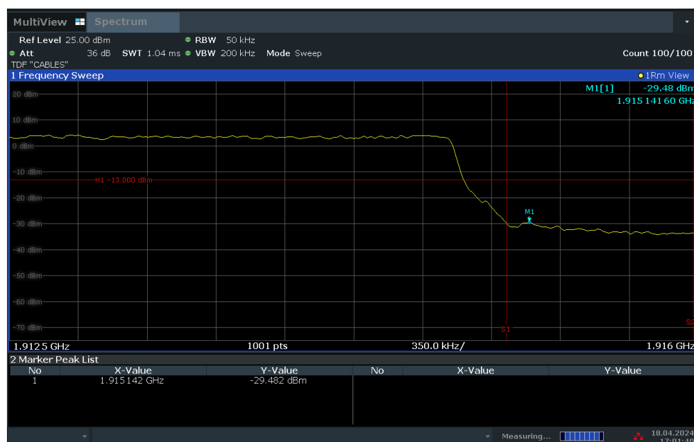
Plot 7-48. Upper Band Edge Plot (LTE Band 25 – 5MHz QPSK – Full RB Configuration)
