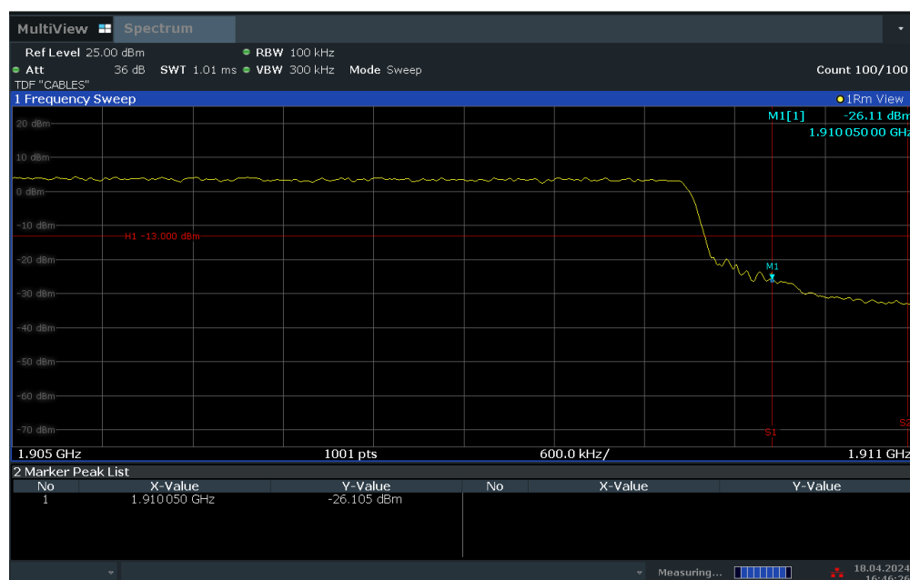
Plot 7-76. Upper Band Edge Plot (LTE Band 2 – 10MHz QPSK – Full RB Configuration)
