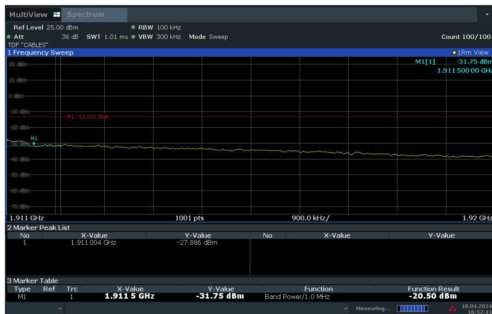
Plot 7-85. Extended Upper Band Edge Plot (LTE Band 2 – 20MHz QPSK – Full RB Configuration)
