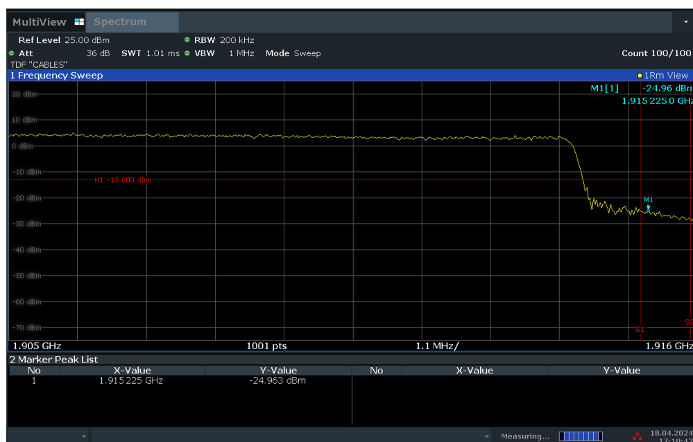
Plot 7-60. Upper Band Edge Plot (LTE Band 25 – 20MHz QPSK – Full RB Configuration)
