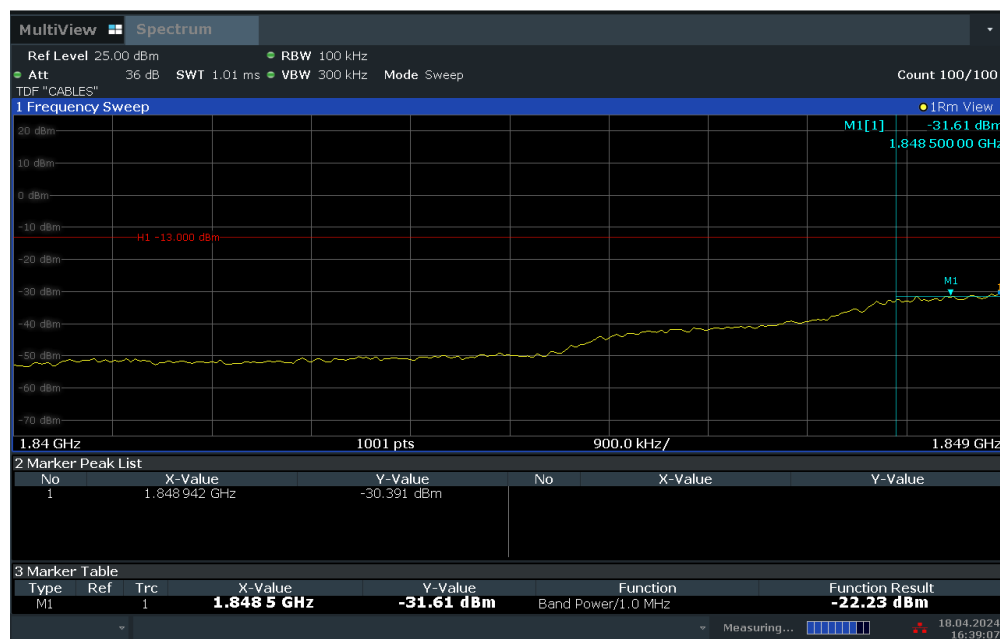
Plot 7-67. Extended Lower Band Edge Plot (LTE Band 2 – 3MHz QPSK – Full RB Configuration)
