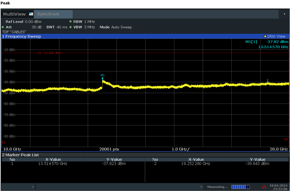
Plot 7-29. Conducted Spurious Plot (WCDMA Ch. 9262)
