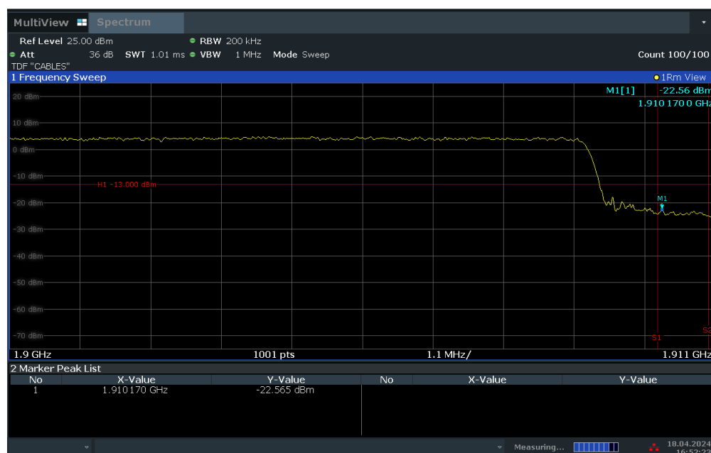
Plot 7-84. Upper Band Edge Plot (LTE Band 2 – 20MHz QPSK – Full RB Configuration)
