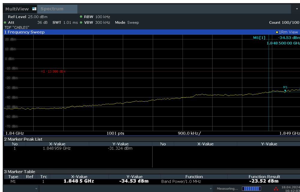
Plot 7-71. Extended Lower Band Edge Plot (LTE Band 2 – 5MHz QPSK – Full RB Configuration)
