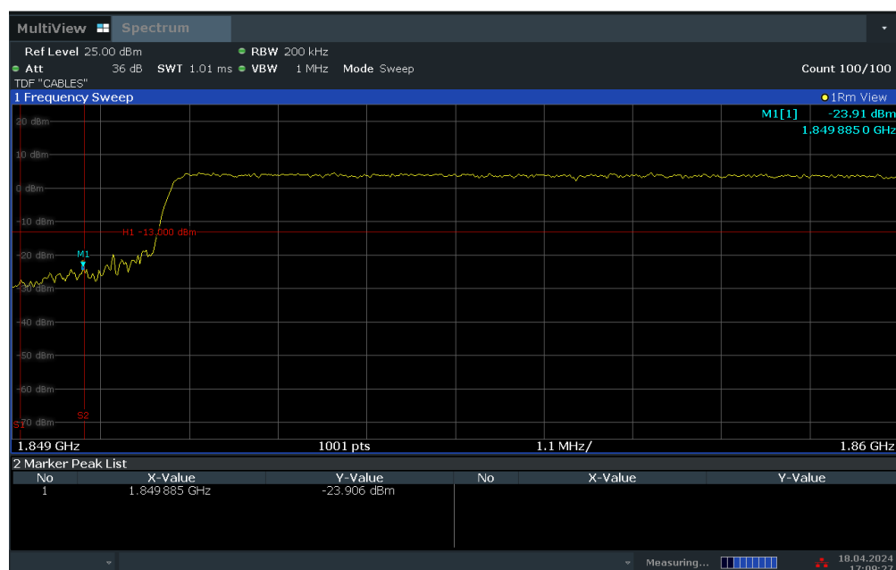
Plot 7-58. Lower Band Edge Plot (LTE Band 25 – 20MHz QPSK – Full RB Configuration)
