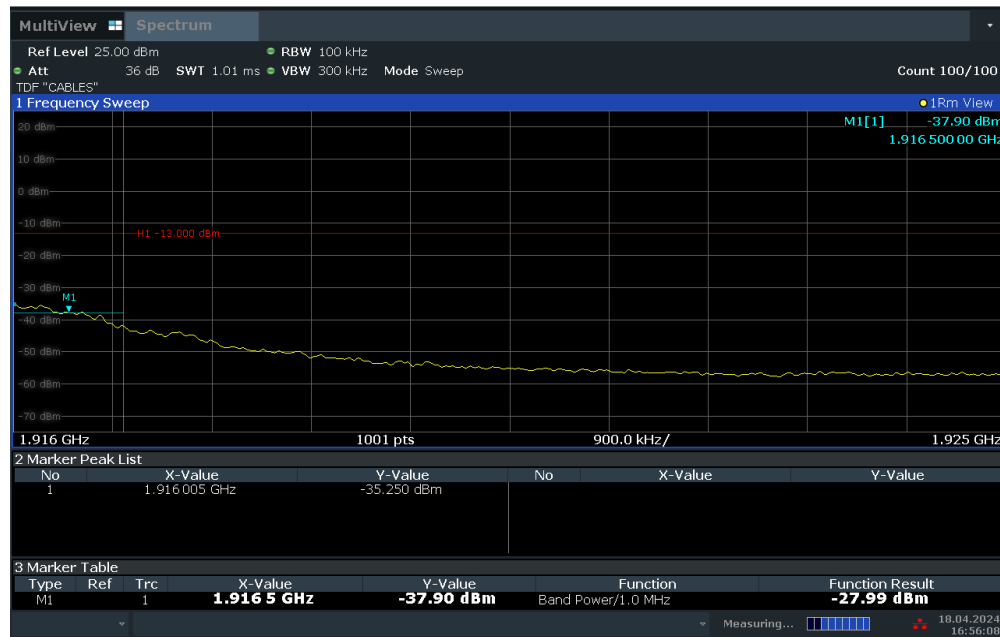
Plot 7-41. Extended Upper Band Edge Plot (LTE Band 25 – 1.4MHz QPSK – Full RB Configuration)
