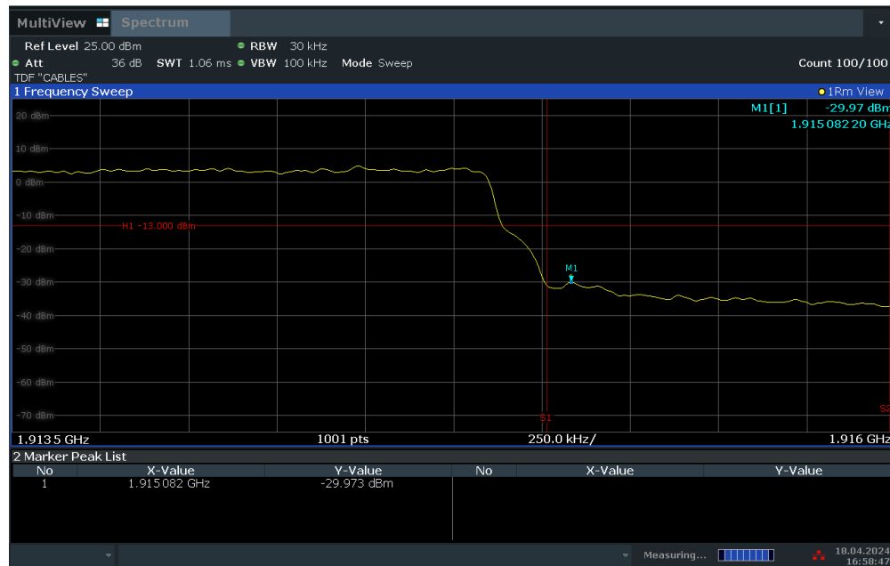
Plot 7-44. Upper Band Edge Plot (LTE Band 25 – 3MHz QPSK – Full RB Configuration)
