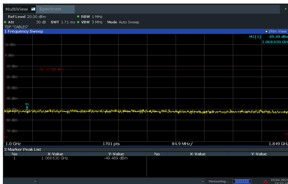
Plot 7-35. Conducted Spurious Plot (WCDMA Ch. 9538)
