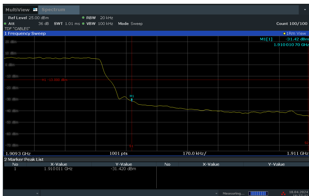
Plot 7-64. Upper Band Edge Plot (LTE Band 2 – 1.4MHz QPSK – Full RB Configuration)
