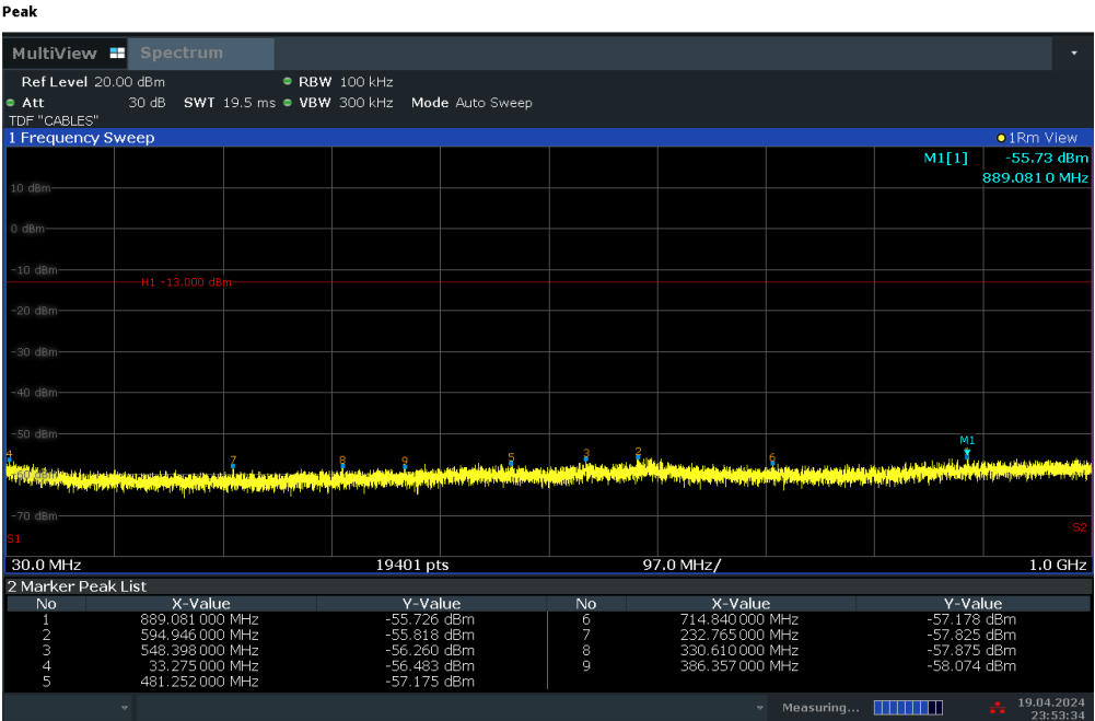
Plot 7-30. Conducted Spurious Plot (WCDMA Ch. 9400)
