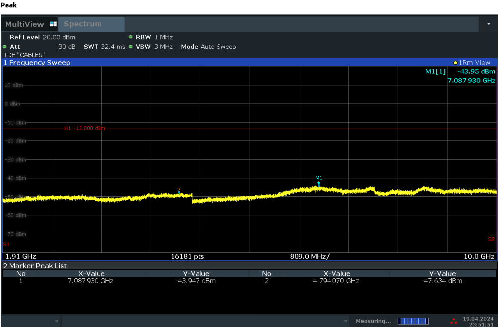
Plot 7-28. Conducted Spurious Plot (WCDMA Ch. 9262)
