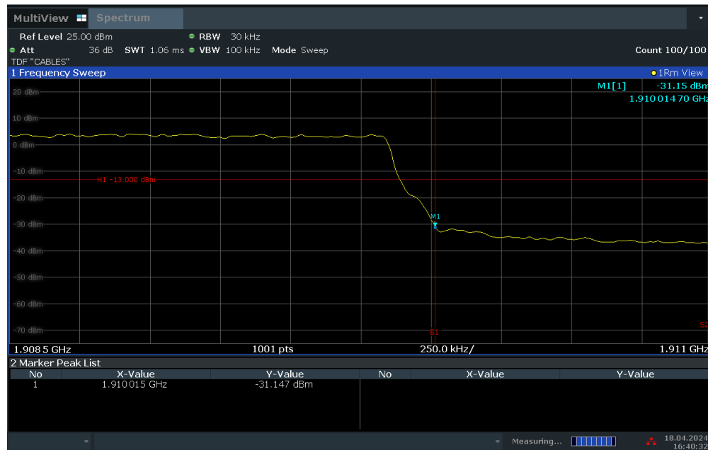
Plot 7-68. Upper Band Edge Plot (LTE Band 2 – 3MHz QPSK – Full RB Configuration)
