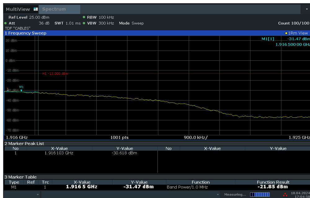
Plot 7-53. Extended Upper Band Edge Plot (LTE Band 25 – 10MHz QPSK – Full RB Configuration)
