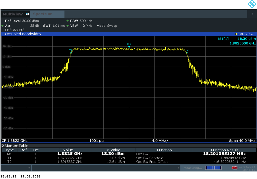
Plot 7-11. Occupied Bandwidth Plot (LTE Band 25/2 - 20MHz QPSK - Full RB Configuration)
