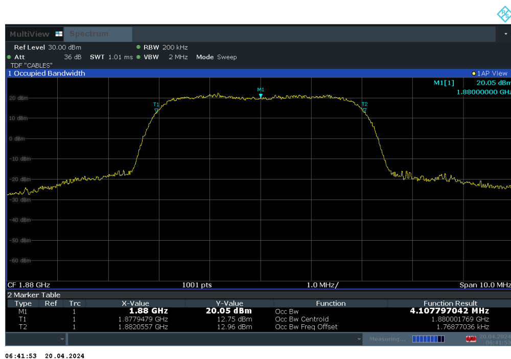
Plot 7-13. Occupied Bandwidth Plot (WCDMA, Ch. 9400)
