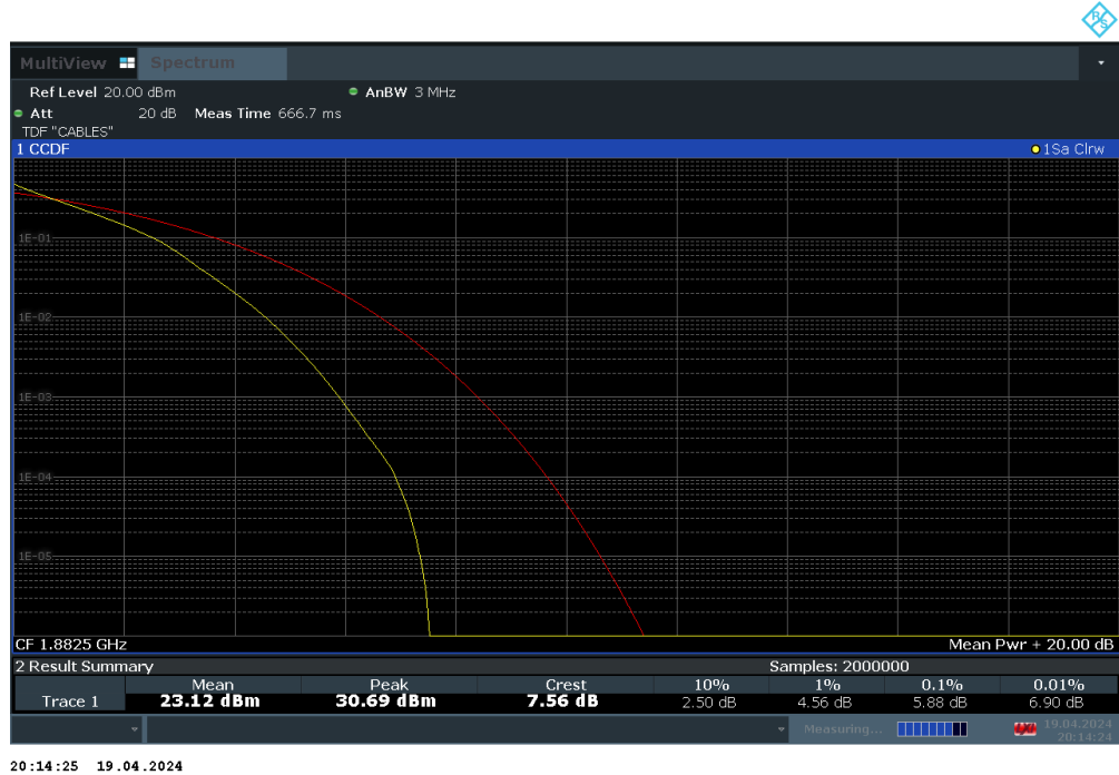
Plot 7-92. PAR Plot (LTE Band 25 - 3MHz QPSK - Full RB Configuration)
