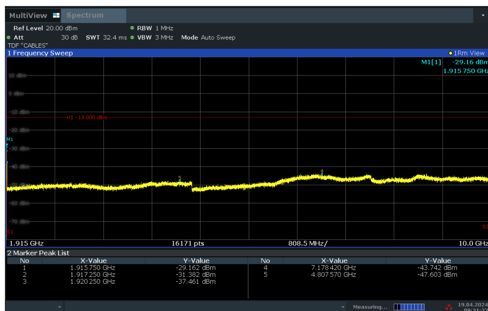
Plot 7-24. Conducted Spurious Plot (LTE Band 25/2 - 20MHz QPSK - RB Size 1, RB Offset 0 - High Channel)
