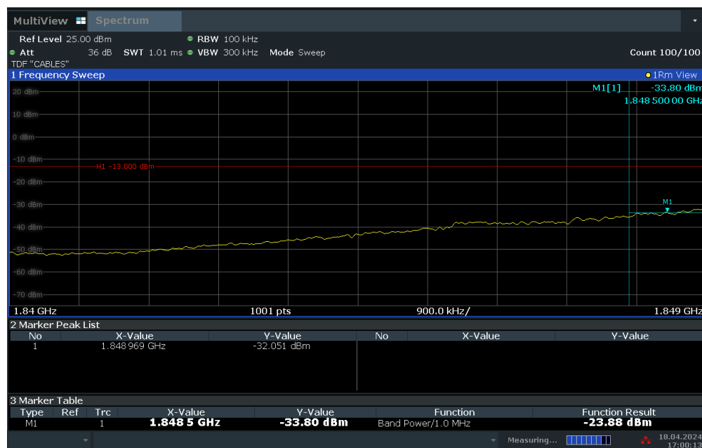
Plot 7-47. Extended Lower Band Edge Plot (LTE Band 25 – 5MHz QPSK – Full RB Configuration)
