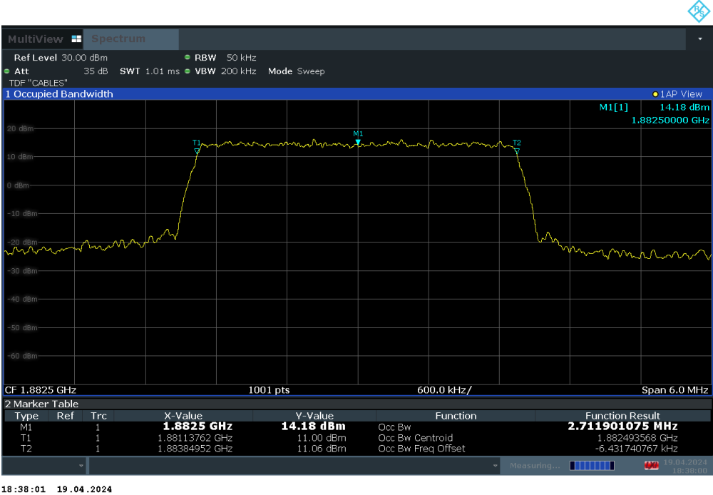
Plot 7-4. Occupied Bandwidth Plot (LTE Band 25/2 - 3MHz 16-QAM - Full RB Configuration)
