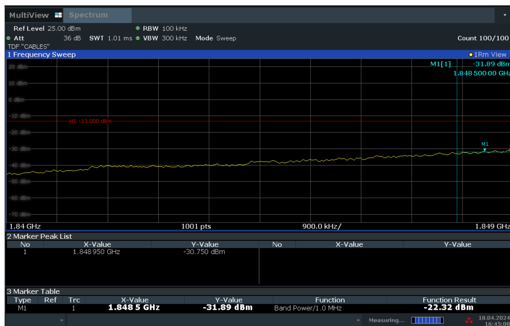
Plot 7-75. Extended Lower Band Edge Plot (LTE Band 2 – 10MHz QPSK – Full RB Configuration)
