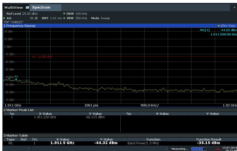
Plot 7-89. Extended Upper Band Edge Plot (WCDMA PCS – Ch. 9538)
