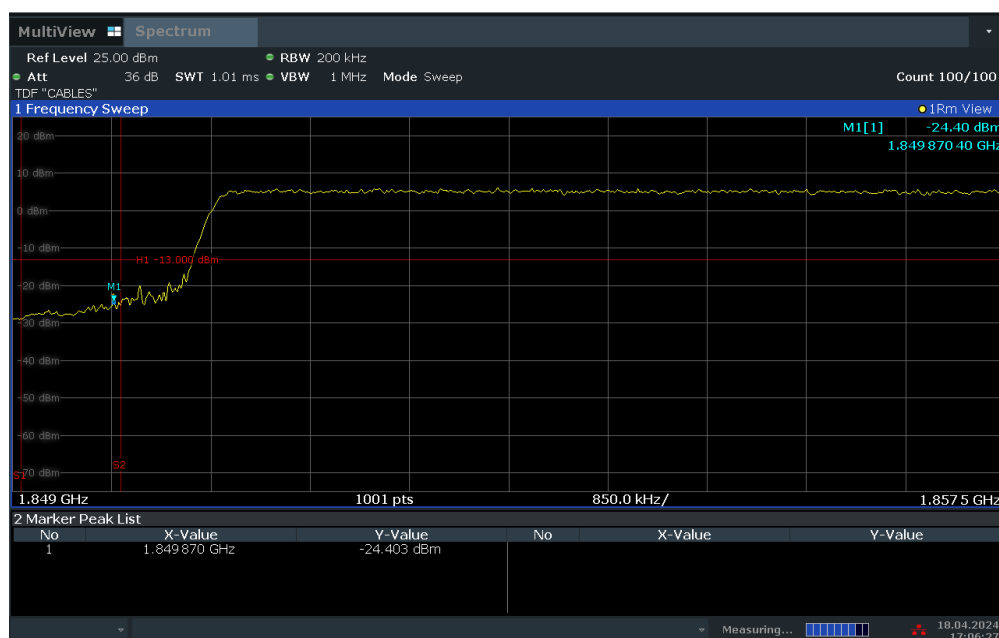
Plot 7-54. Lower Band Edge Plot (LTE Band 25 – 15MHz QPSK – Full RB Configuration)
