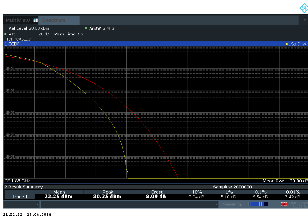
Plot 7-103. PAR Plot (LTE Band 2 - 1.4MHz 16-QAM - Full RB Configuration)
