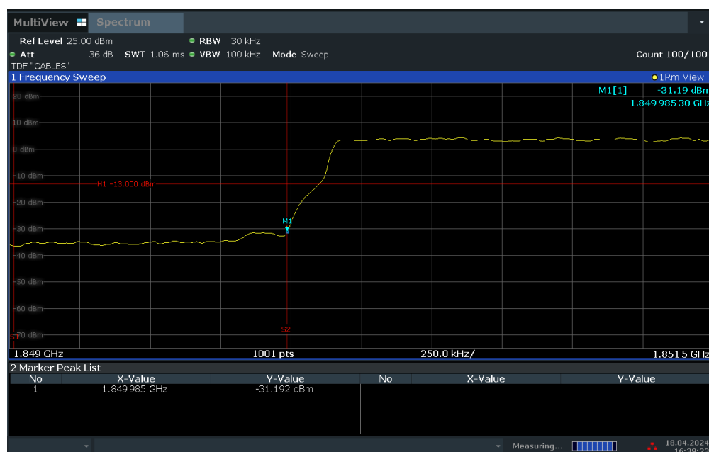
Plot 7-66. Lower Band Edge Plot (LTE Band 2 – 3MHz QPSK – Full RB Configuration)
