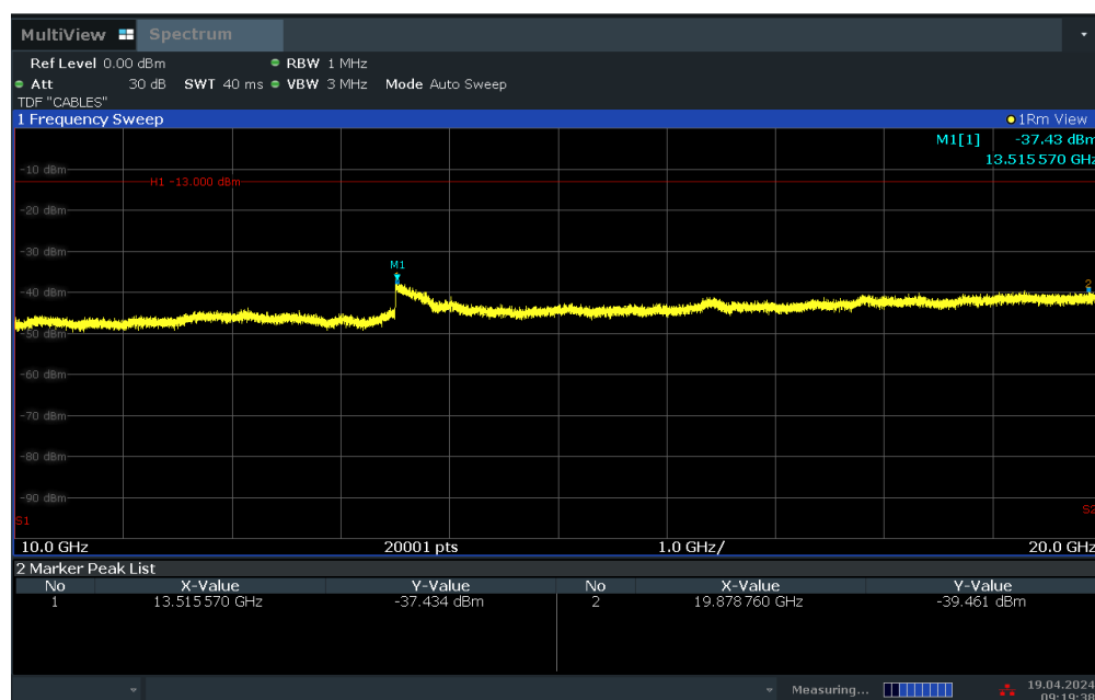
Plot 7-21. Conducted Spurious Plot (LTE Band 25/2 - 20MHz QPSK - RB Size 1, RB Offset 0 - Mid Channel)
