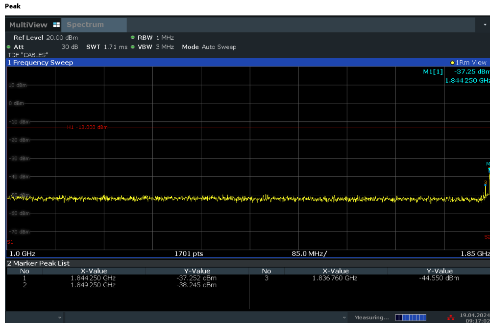
Plot 7-15. Conducted Spurious Plot (LTE Band 25/2 - 20MHz QPSK - RB Size 1, RB Offset 0 - Low Channel)
