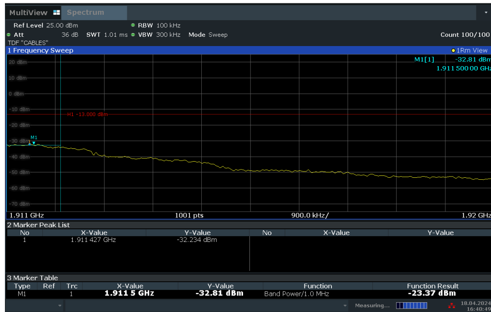
Plot 7-69. Extended Upper Band Edge Plot (LTE Band 2 – 3MHz QPSK – Full RB Configuration)
