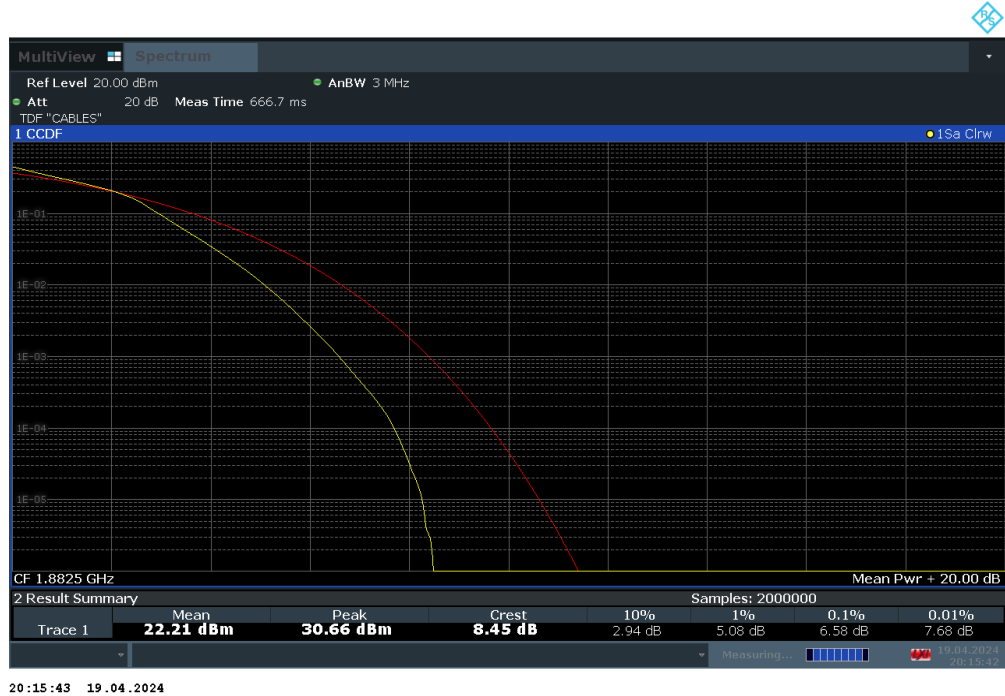
Plot 7-93. PAR Plot (LTE Band 25 - 3MHz 16-QAM - Full RB Configuration)
