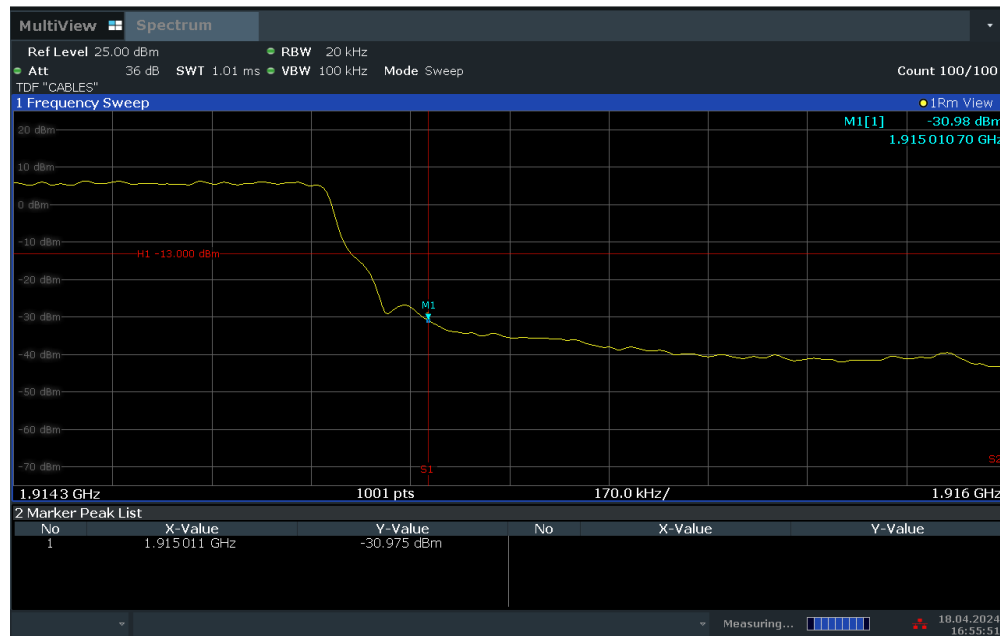
Plot 7-40. Upper Band Edge Plot (LTE Band 25 – 1.4MHz QPSK – Full RB Configuration)
