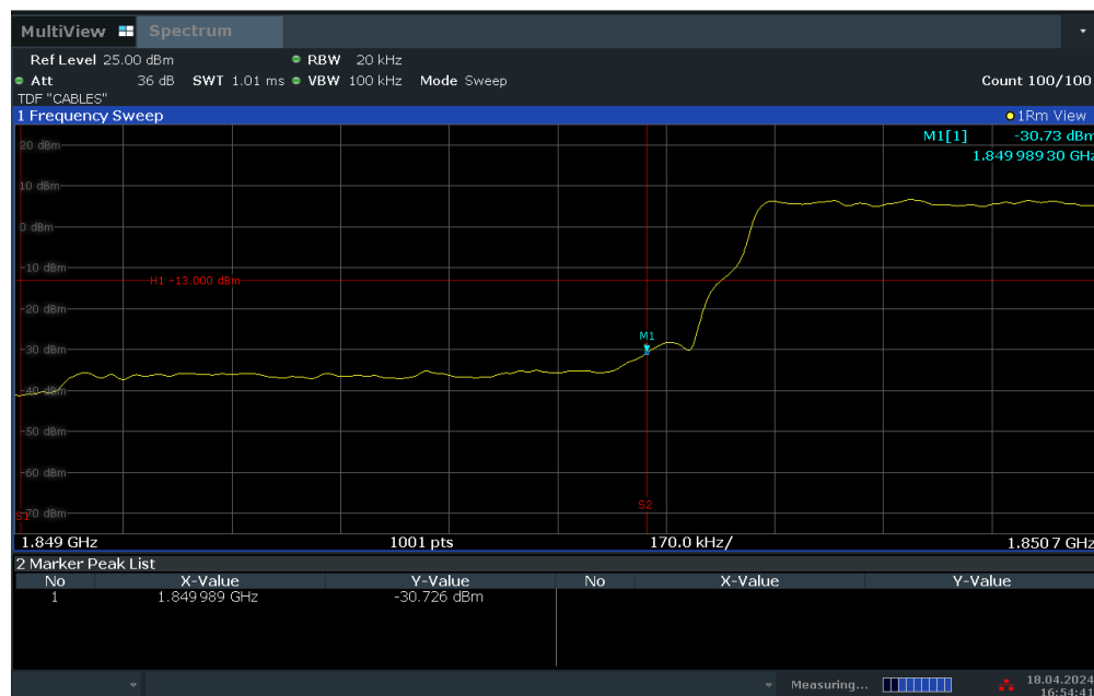
Plot 7-38. Lower Band Edge Plot (LTE Band 25 – 1.4MHz QPSK – Full RB Configuration)
