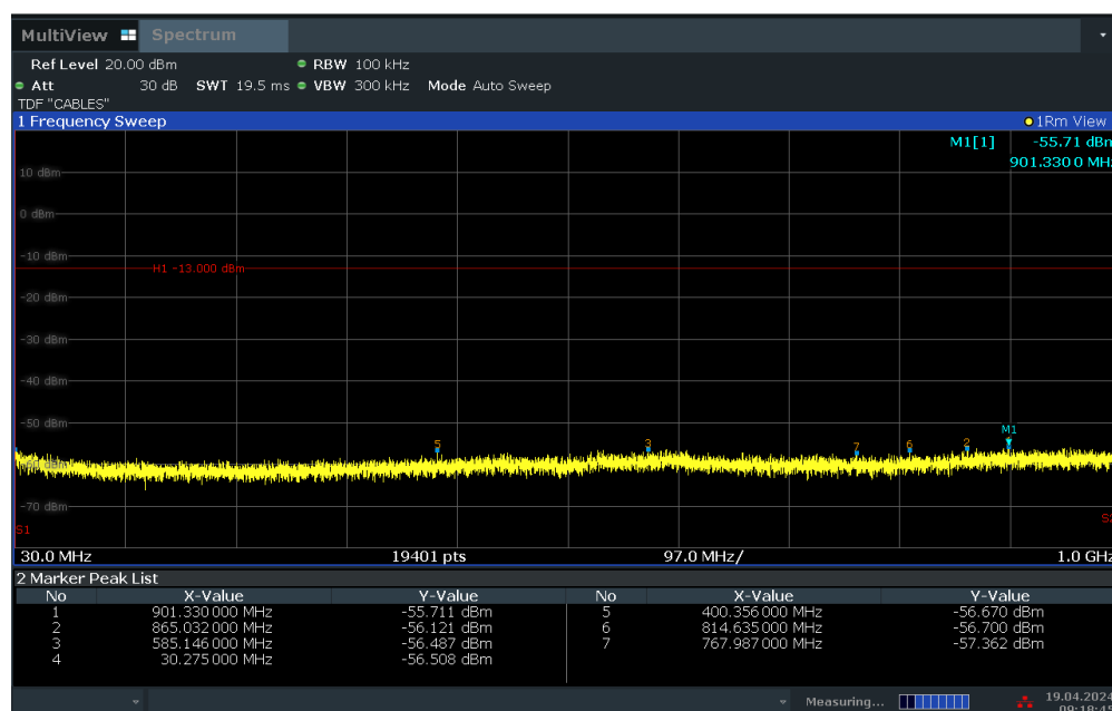
Plot 7-18. Conducted Spurious Plot (LTE Band 25/2 - 20MHz QPSK - RB Size 1, RB Offset 0 - Mid Channel)
