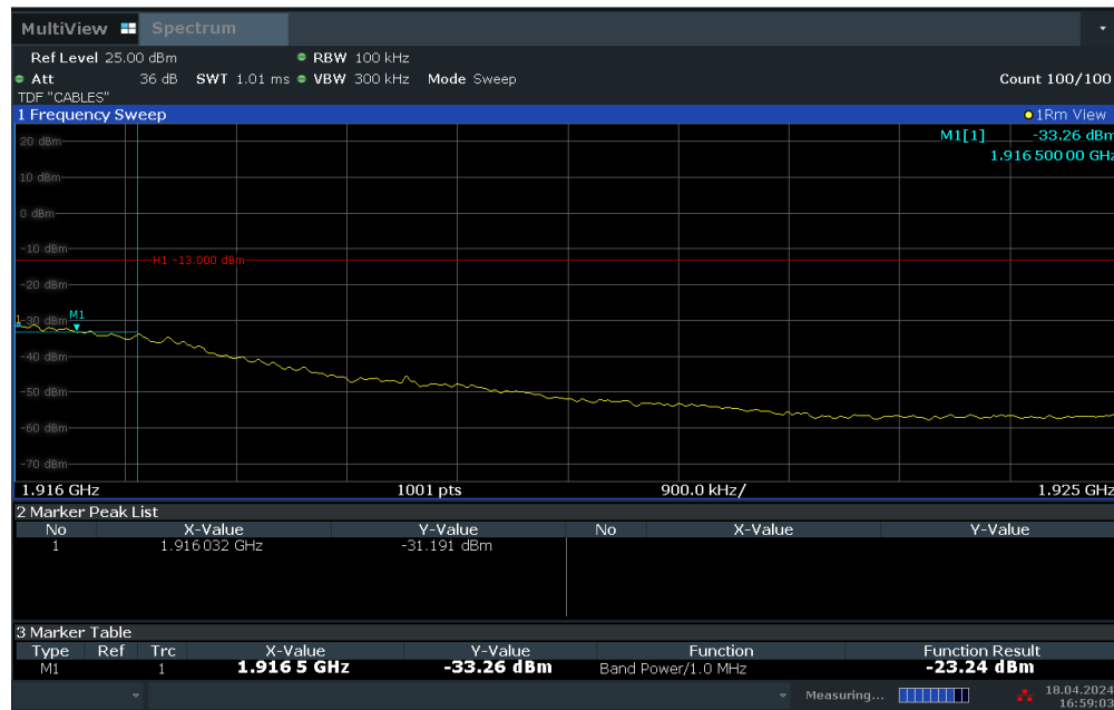
Plot 7-45. Extended Upper Band Edge Plot (LTE Band 25 – 3MHz QPSK – Full RB Configuration)
