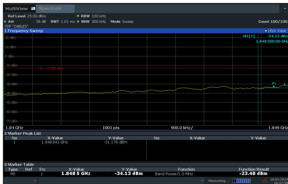
Plot 7-79. Extended Lower Band Edge Plot (LTE Band 2 – 15MHz QPSK – Full RB Configuration)
