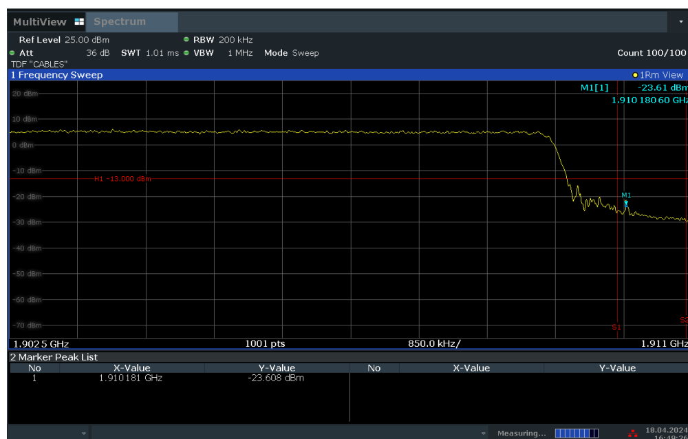
Plot 7-80. Upper Band Edge Plot (LTE Band 2 – 15MHz QPSK – Full RB Configuration)
