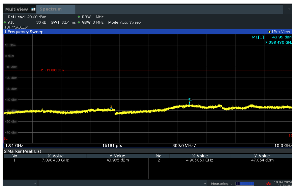
Plot 7-32. Conducted Spurious Plot (WCDMA Ch. 9400)
