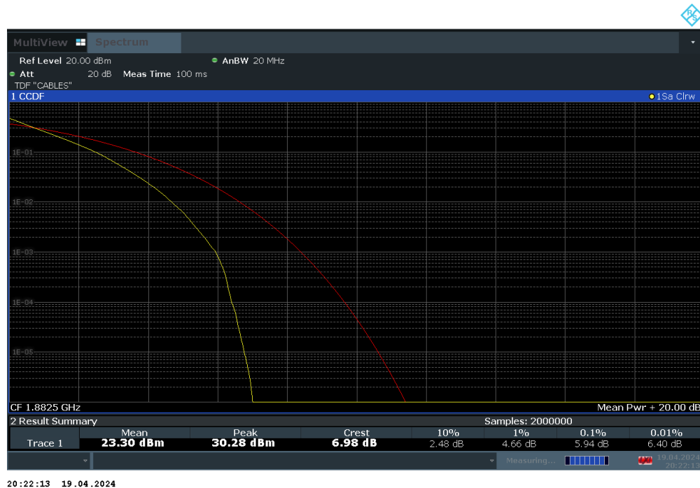
Plot 7-98. PAR Plot (LTE Band 25 - 15MHz QPSK - Full RB Configuration)
