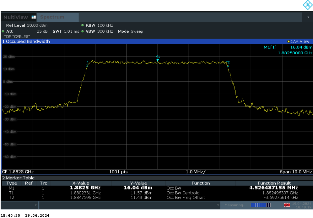
Plot 7-6. Occupied Bandwidth Plot (LTE Band 25/2 - 5MHz 16-QAM - Full RB Configuration)
