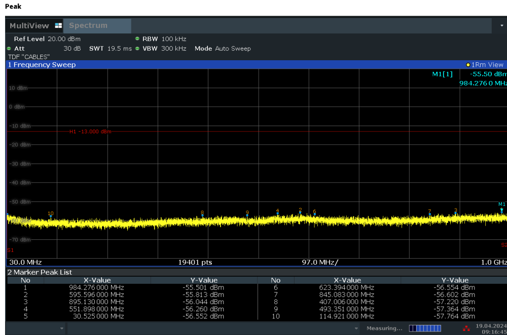
Plot 7-14. Conducted Spurious Plot (LTE Band 25/2 - 20MHz QPSK - RB Size 1, RB Offset 0 - Low Channel)
