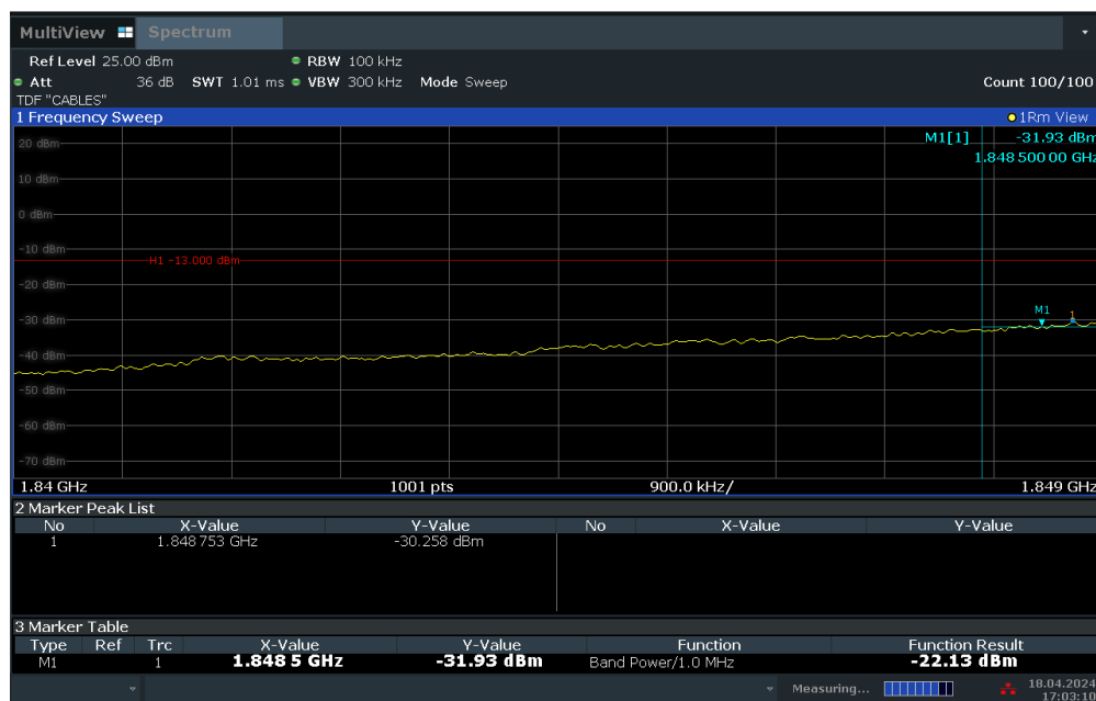
Plot 7-51. Extended Lower Band Edge Plot (LTE Band 25 – 10MHz QPSK – Full RB Configuration)
