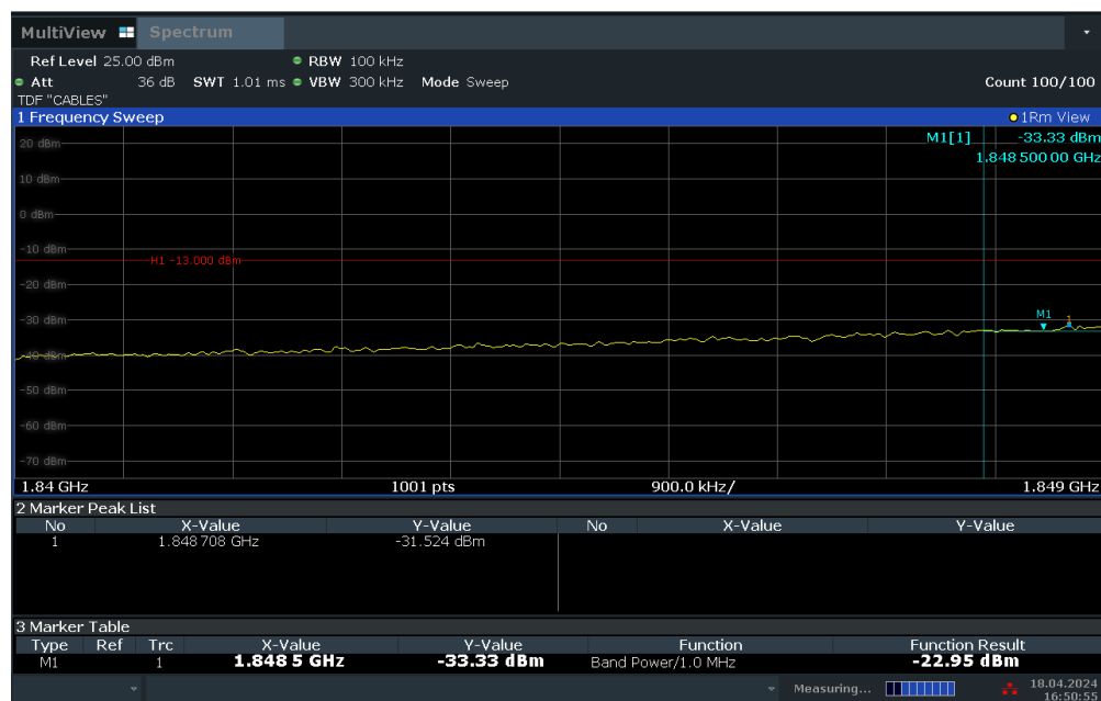
Plot 7-83. Extended Lower Band Edge Plot (LTE Band 2 – 20MHz QPSK – Full RB Configuration)
