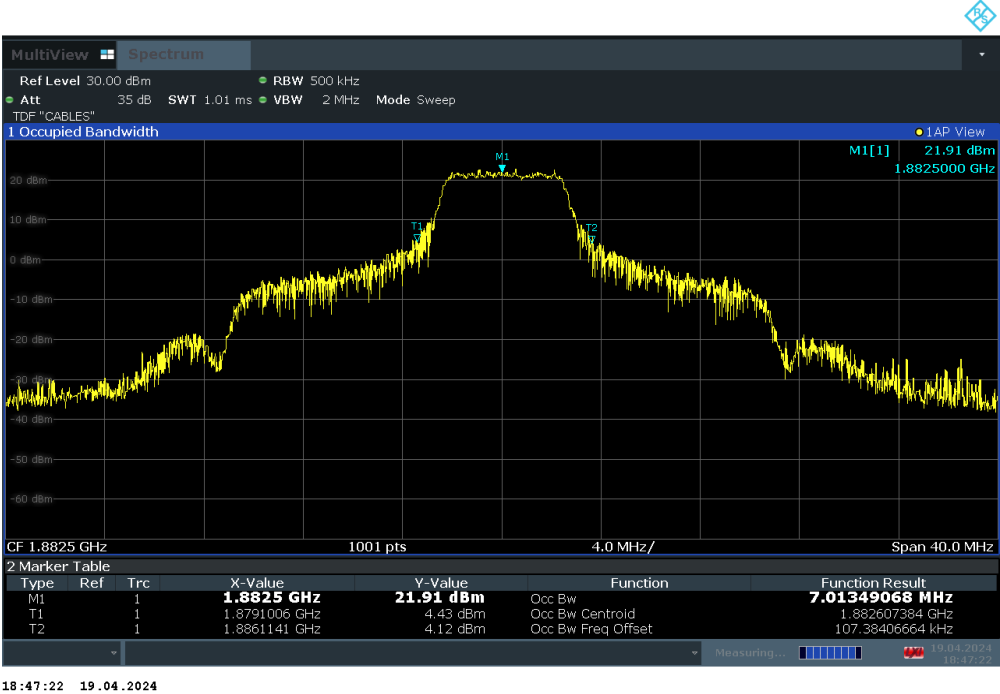
Plot 7-12. Occupied Bandwidth Plot (LTE Band 25/2 - 20MHz 16-QAM - Full RB Configuration)
