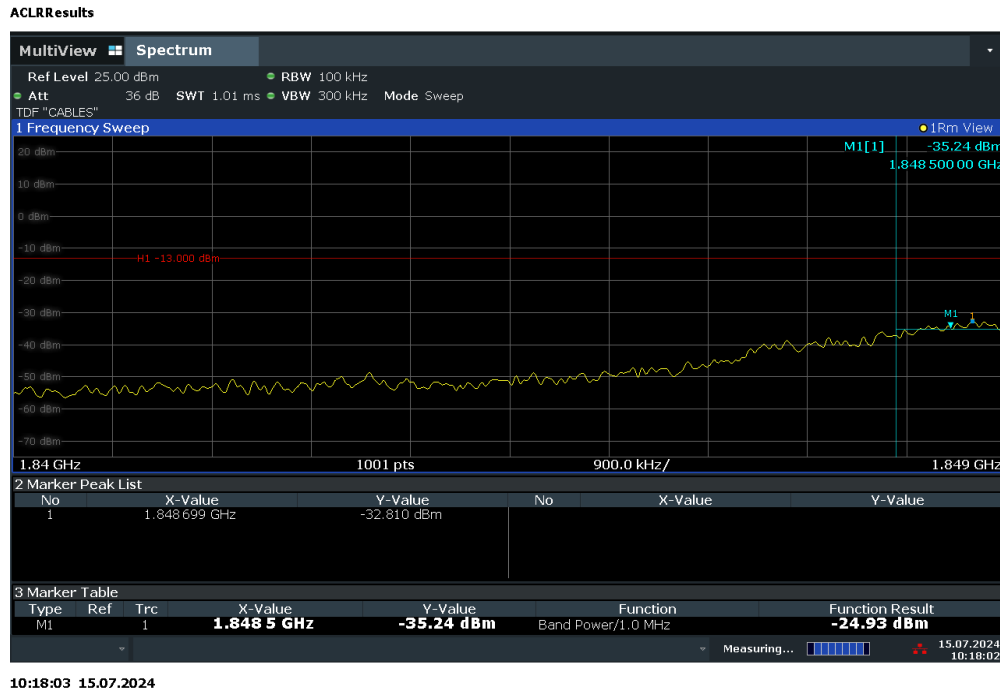
Plot 7-87. Extended Lower Band Edge Plot (WCDMA PCS – Ch. 9262)
