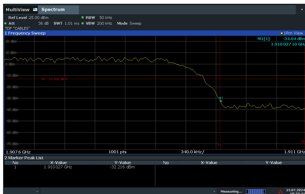
Plot 7-88. Upper Band Edge Plot (WCDMA PCS – Ch. 9538)
