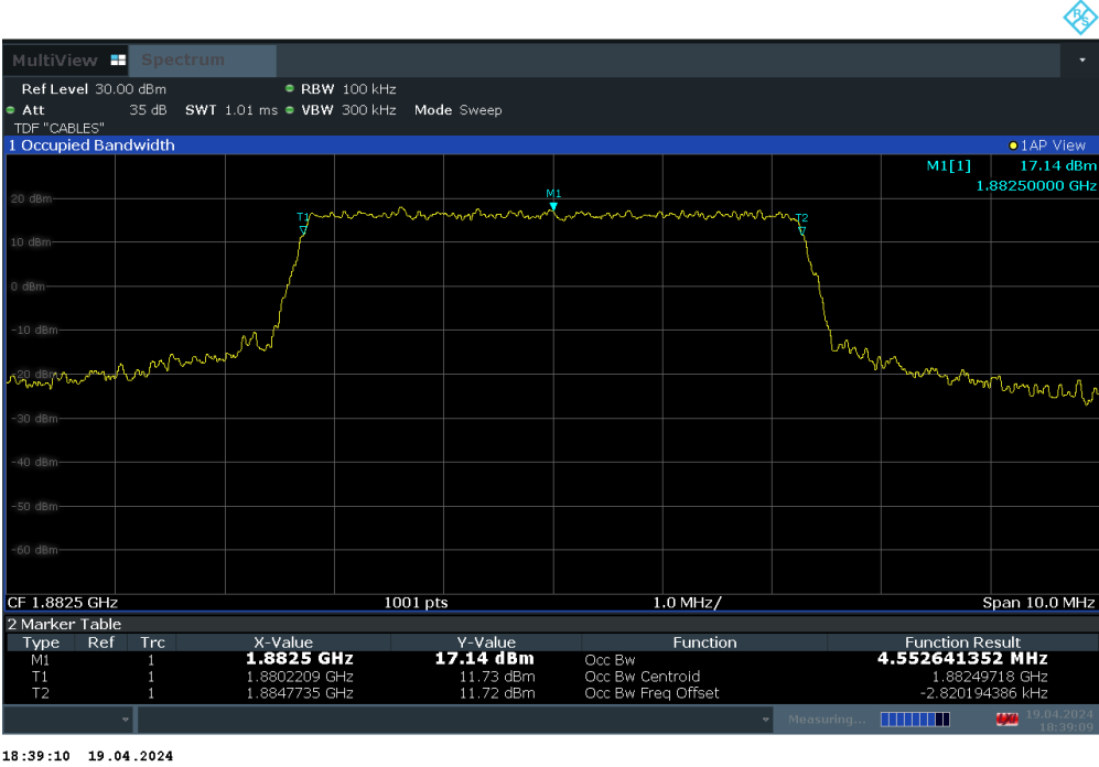
Plot 7-5. Occupied Bandwidth Plot (LTE Band 25/2 - 5MHz QPSK - Full RB Configuration)
