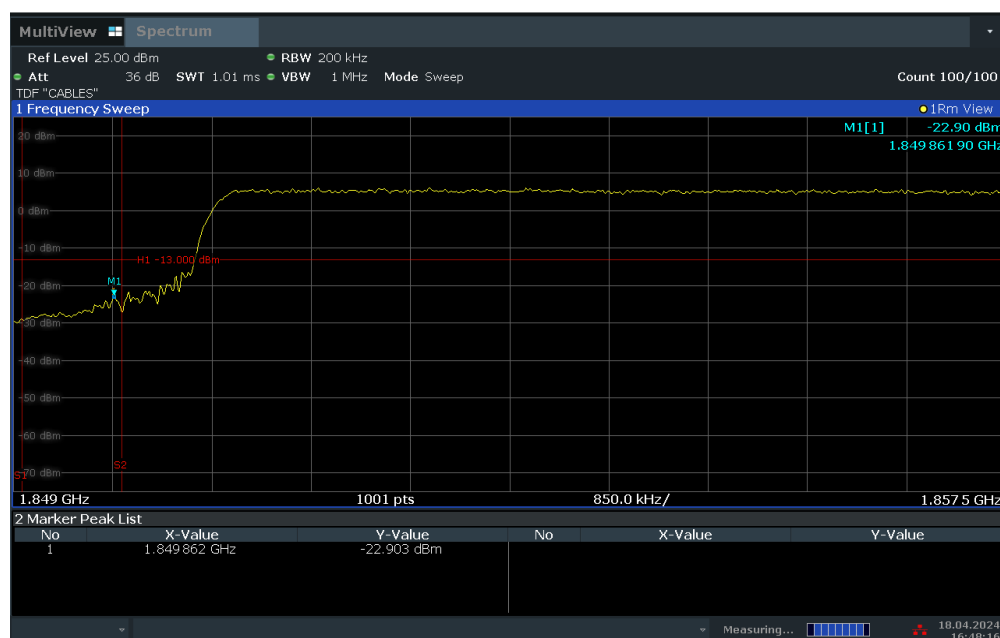
Plot 7-78. Lower Band Edge Plot (LTE Band 2 – 15MHz QPSK – Full RB Configuration)
