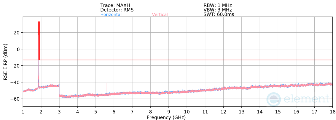
Plot 7-115. Radiated Spurious Plot (LTE Band 25/2)
