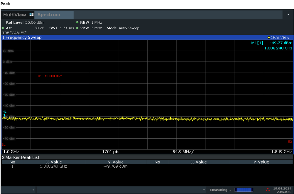
Plot 7-31. Conducted Spurious Plot (WCDMA Ch. 9400)
