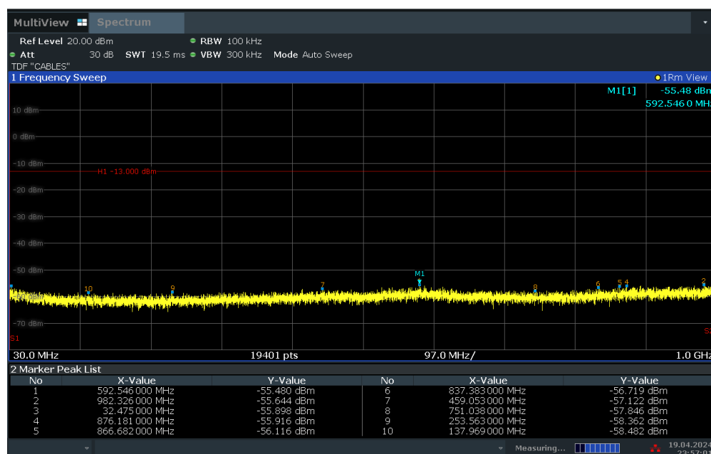
Plot 7-34. Conducted Spurious Plot (WCDMA Ch. 9538)
