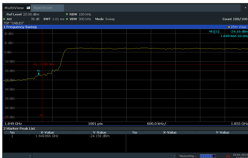
Plot 7-50. Lower Band Edge Plot (LTE Band 25 – 10MHz QPSK – Full RB Configuration)
