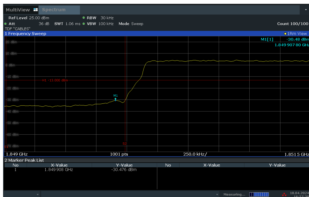
Plot 7-42. Lower Band Edge Plot (LTE Band 25 – 3MHz QPSK – Full RB Configuration)
