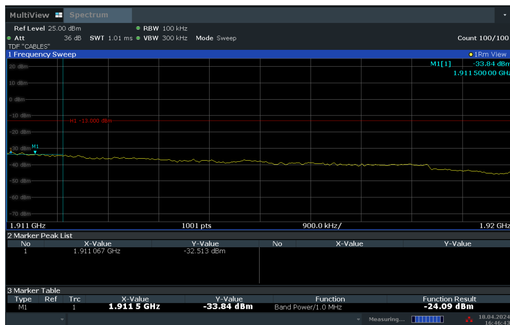
Plot 7-77. Extended Upper Band Edge Plot (LTE Band 2 – 10MHz QPSK – Full RB Configuration)
