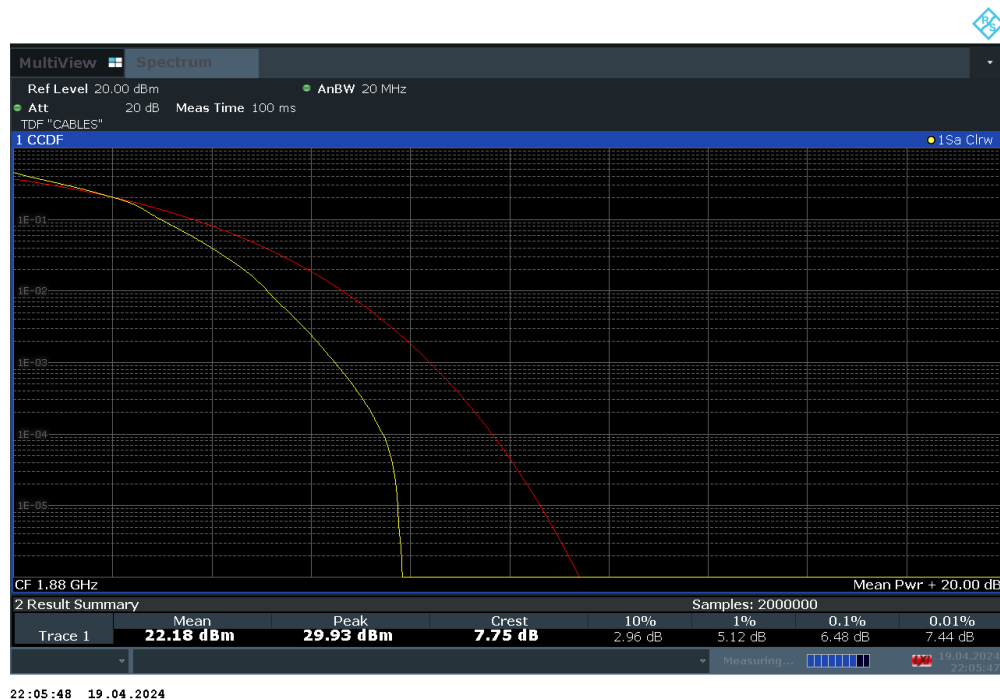
Plot 7-113. PAR Plot (LTE Band 2 - 20MHz 16-QAM - Full RB Configuration)
