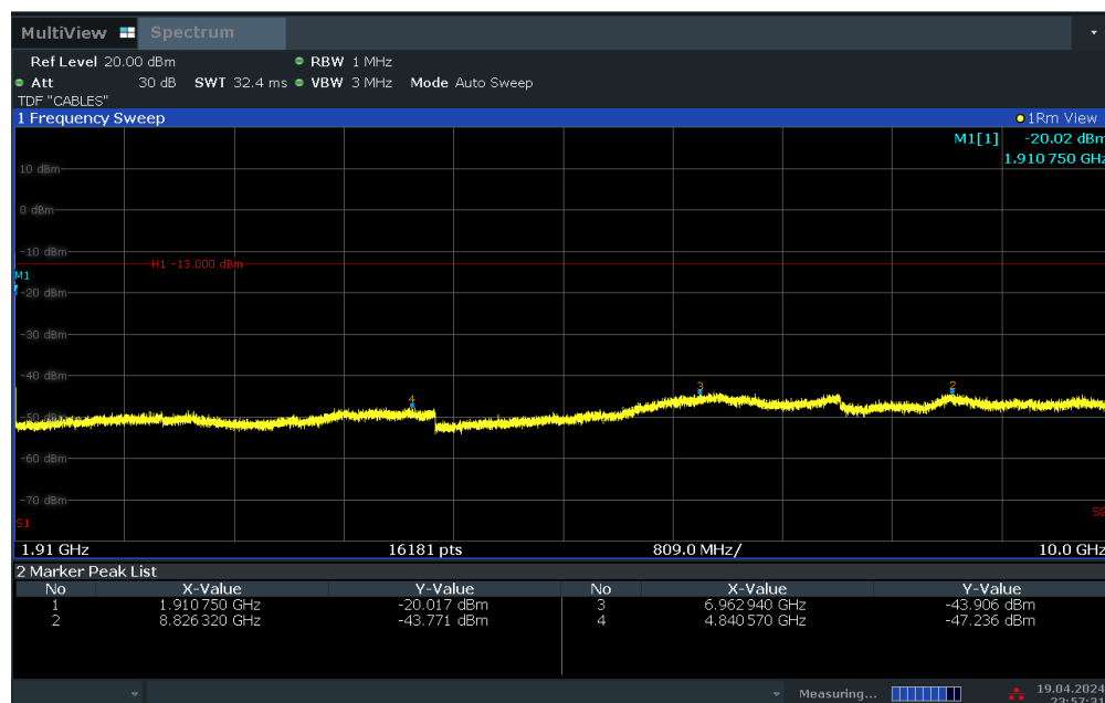
Plot 7-36. Conducted Spurious Plot (WCDMA Ch. 9538)
