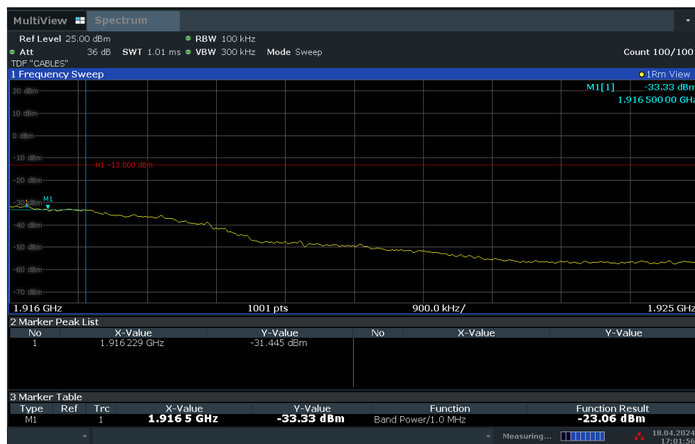
Plot 7-49. Extended Upper Band Edge Plot (LTE Band 25 – 5MHz QPSK – Full RB Configuration)
