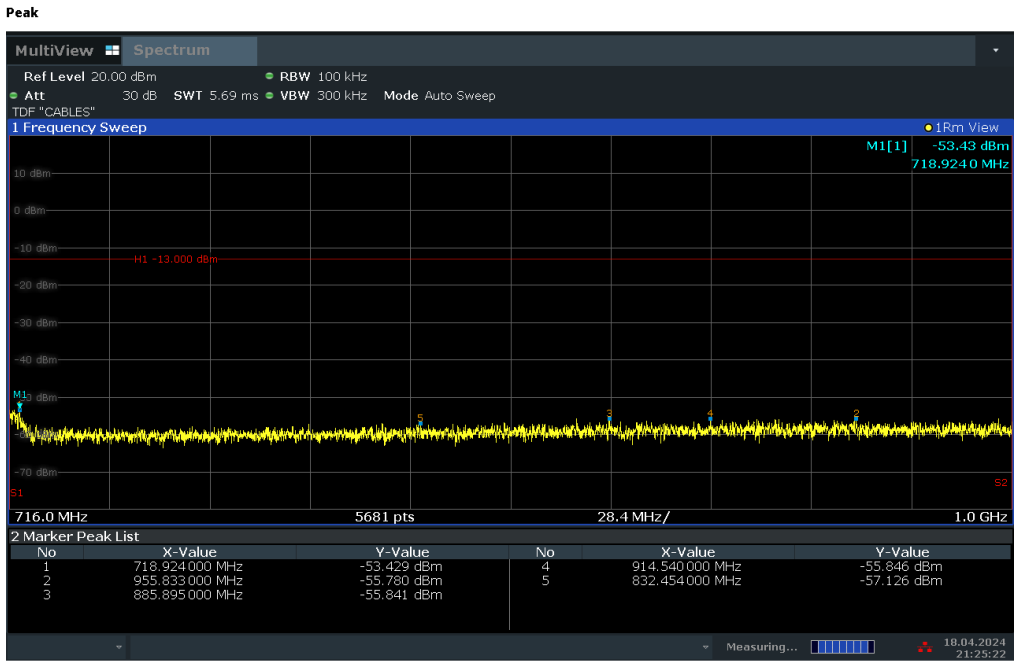
Plot 7-39. Conducted Spurious Plot (LTE Band 12/17 - 10MHz QPSK - RB Size 1, RB Offset 0 - Low Channel)
