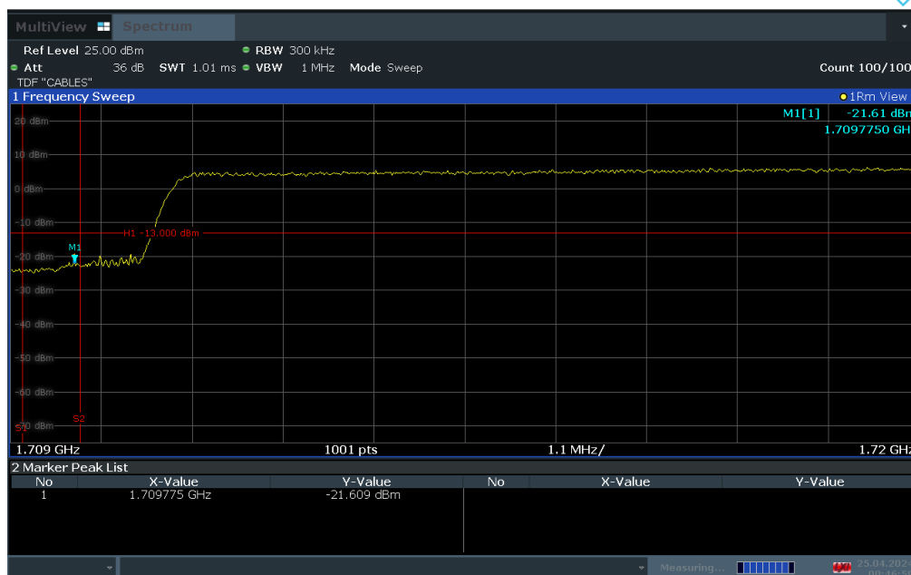
Plot 7-87. Lower Band Edge Plot (LTE Band 66 - 20MHz QPSK – Full RB)
