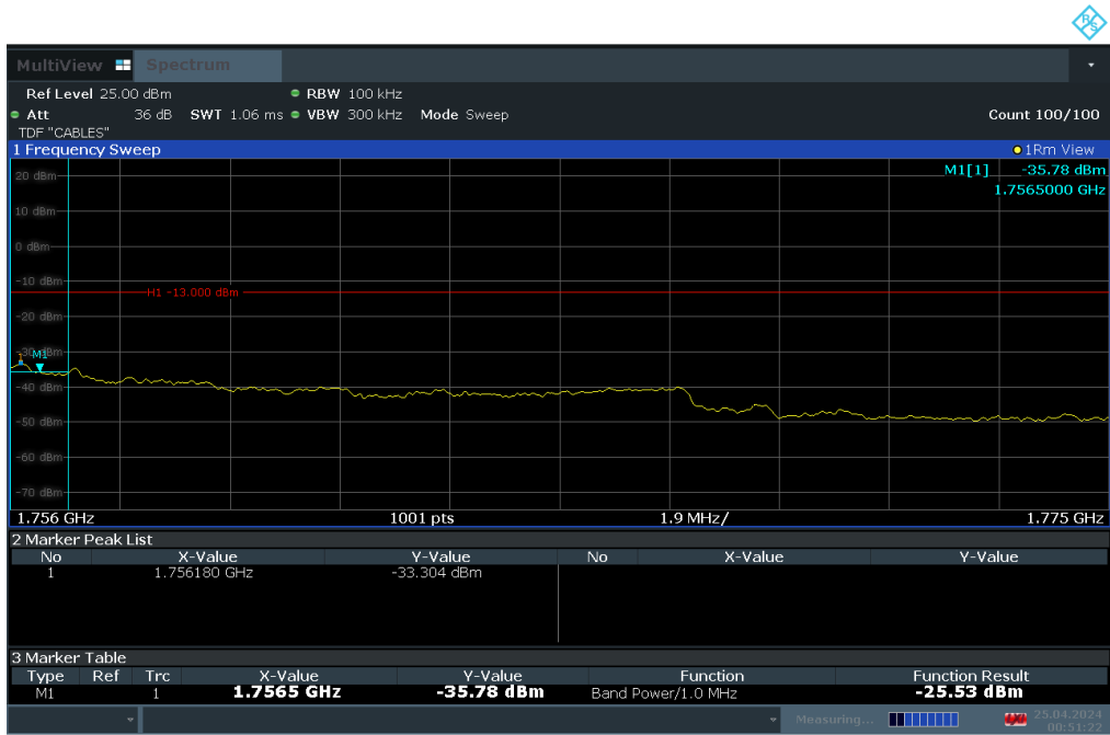
Plot 7-110. Upper Extended Band Edge Plot (LTE Band 4 - 15MHz QPSK – Full RB)
