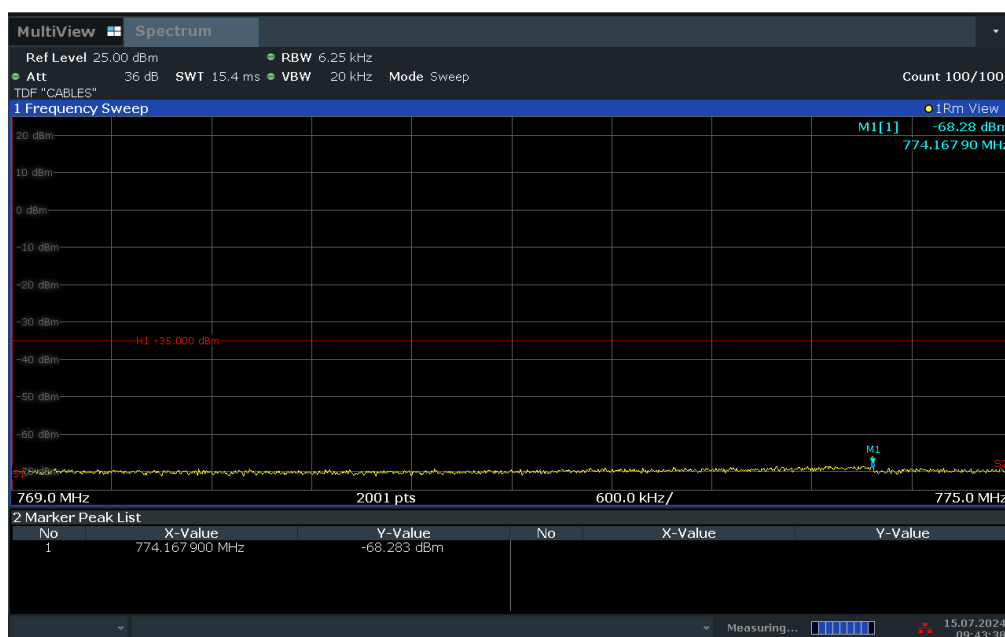
Plot 7-44. Lower Emission Mask Plot (LTE Band 14 - 10MHz QPSK – RB Size 50)
