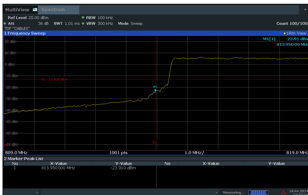
Plot 7-37. Channel Edge Plot (LTE Band 26 - 10MHz QPSK – Low Channel)
