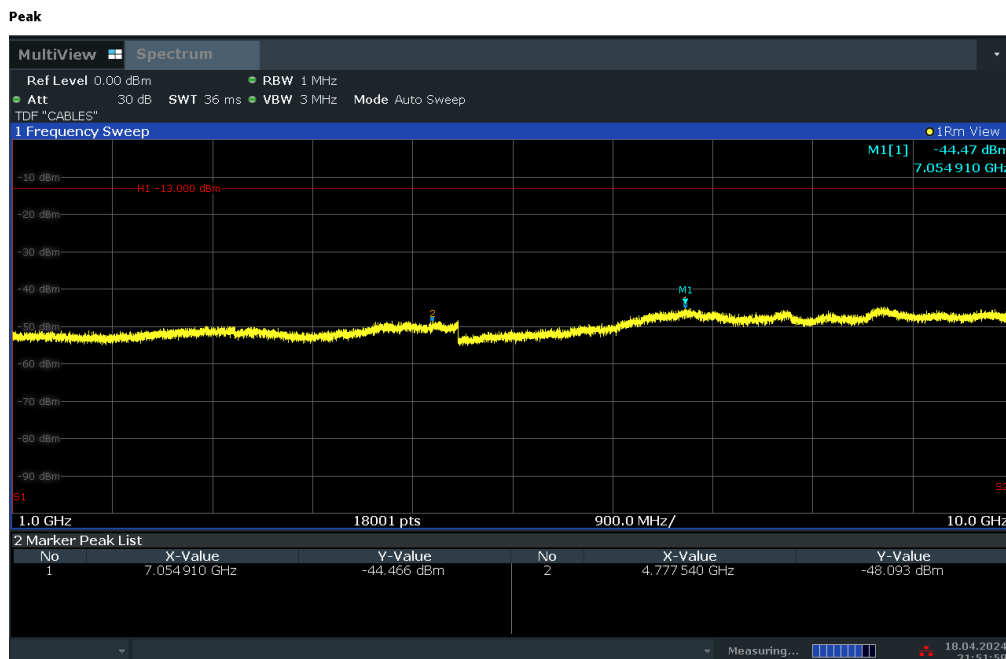
Plot 7-15. Conducted Spurious Plot (LTE Band 26 - 5MHz QPSK - RB Size 1, RB Offset 0 - Low Channel)
