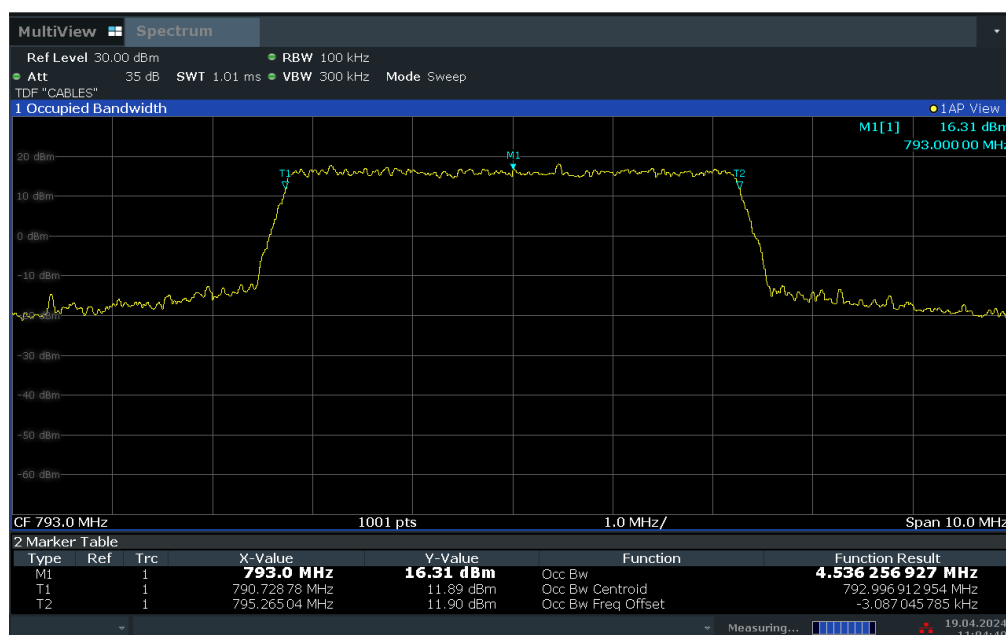
Plot 7-10. Occupied Bandwidth Plot (LTE Band 14 - 5MHz 16-QAM - Full RB)
