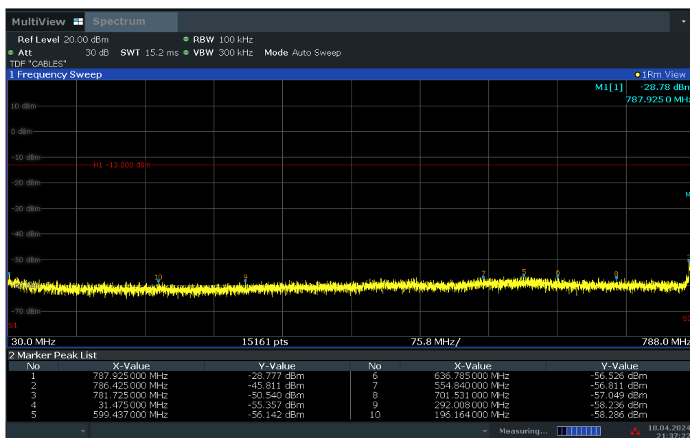
Plot 7-25. Conducted Spurious Plot (LTE Band 14 - 10MHz QPSK - RB Size 1, RB Offset 0 - Mid Channel)
