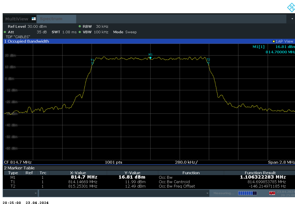
Plot 7-2. Occupied Bandwidth Plot (LTE Band 26 - 1.4MHz 16-QAM - Full RB)
