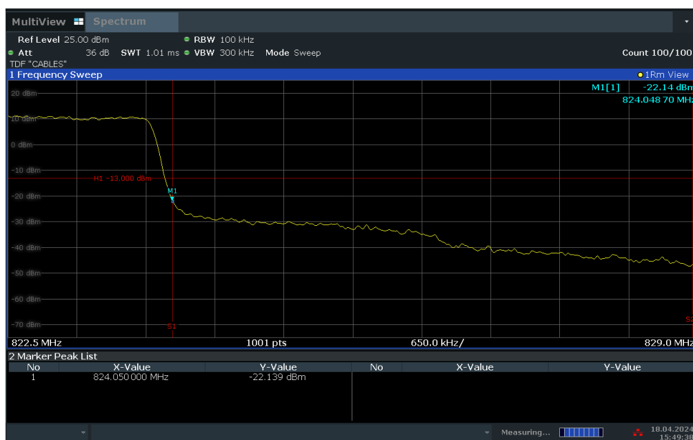
Plot 7-34. Channel Edge Plot (LTE Band 26 - 3MHz QPSK – High Channel)
