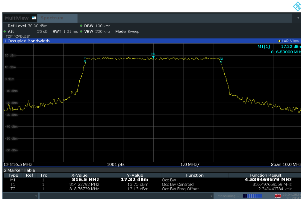
Plot 7-5. Occupied Bandwidth Plot (LTE Band 26 - 5MHz QPSK - Full RB)
