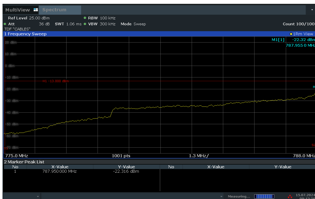
Plot 7-43. Lower Band Edge Plot (LTE Band 14 - 10MHz QPSK – RB Size 50)
