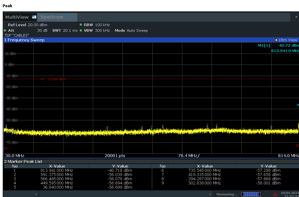
Plot 7-13. Conducted Spurious Plot (LTE Band 26 - 5MHz QPSK - RB Size 1, RB Offset 0 - Low Channel)
