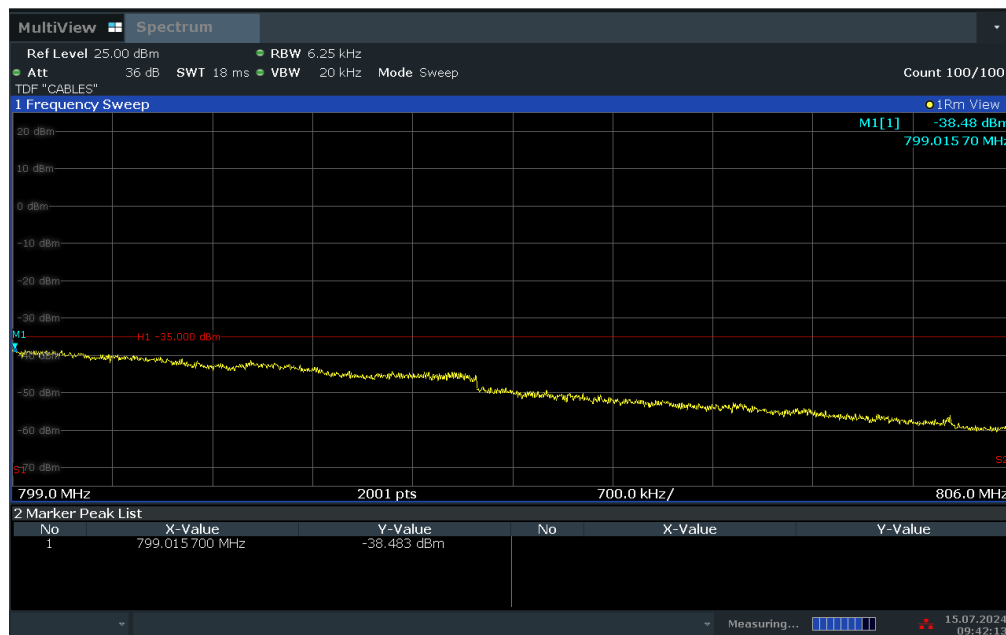
Plot 7-42. Upper Emission Mask Plot (LTE Band 14 - 5MHz QPSK – RB Size 25)
