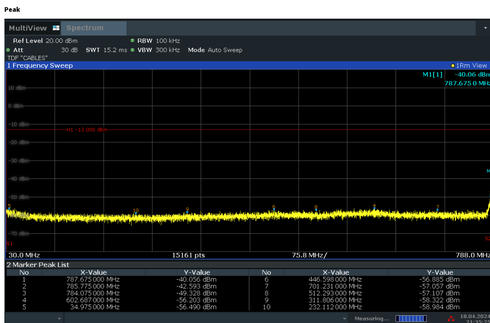
Plot 7-22. Conducted Spurious Plot (LTE Band 14 - 5MHz QPSK - RB Size 1, RB Offset 0 - Low Channel)
