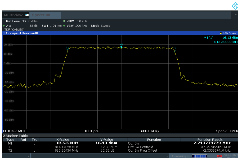
Plot 7-3. Occupied Bandwidth Plot (LTE Band 26 - 3MHz QPSK - Full RB)
