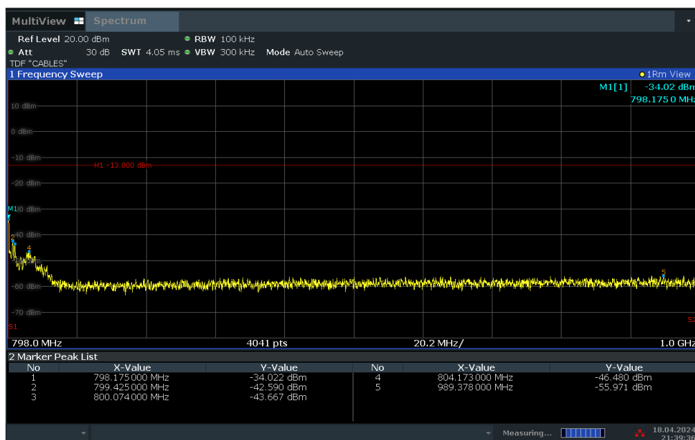
Plot 7-29. Conducted Spurious Plot (LTE Band 14 - 5MHz QPSK - RB Size 1, RB Offset 0 - High Channel)
