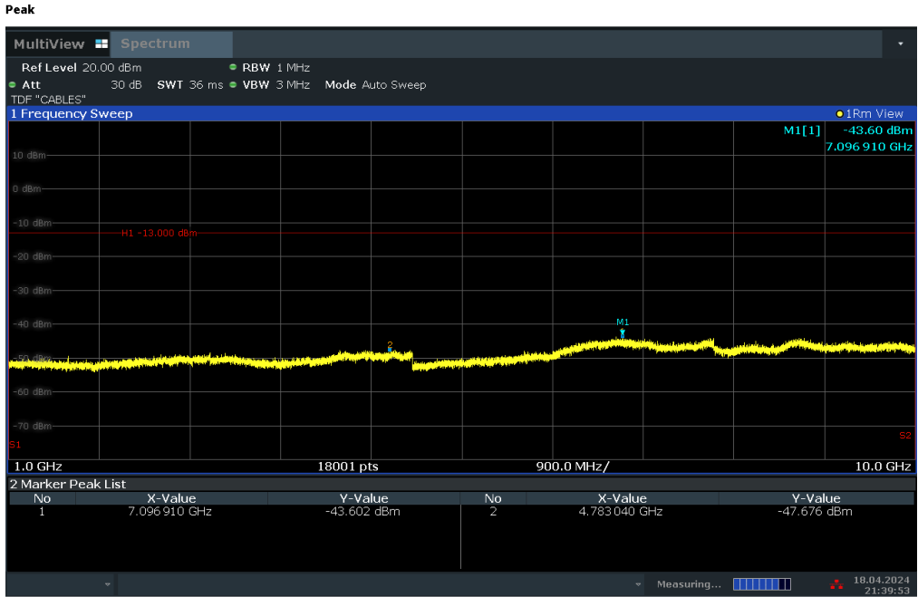
Plot 7-30. Conducted Spurious Plot (LTE Band 14 - 5MHz QPSK - RB Size 1, RB Offset 0 - High Channel)
