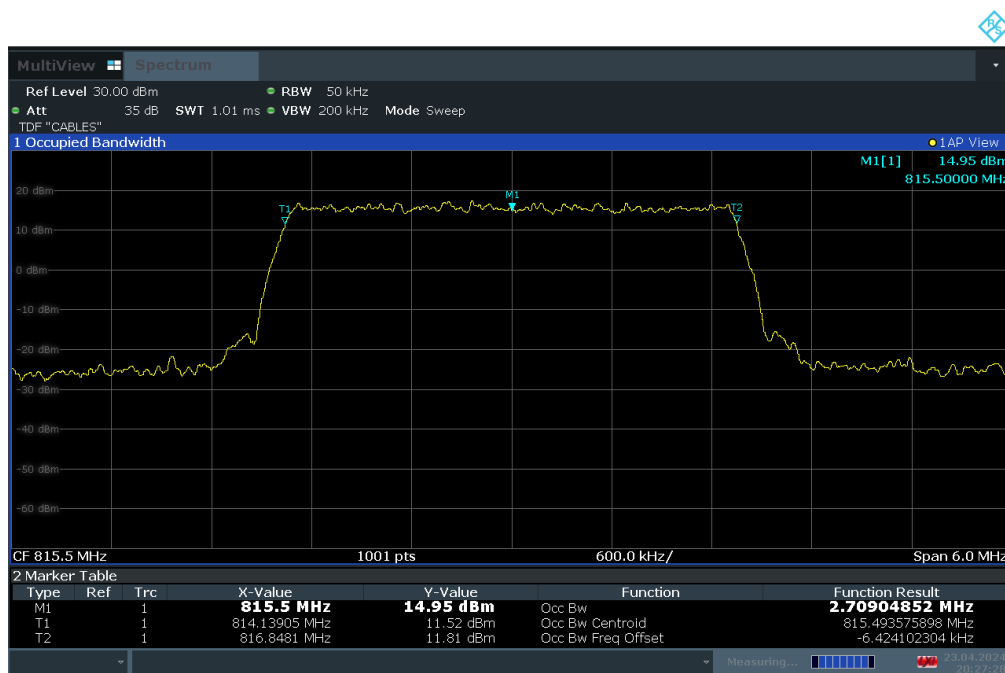
Plot 7-4. Occupied Bandwidth Plot (LTE Band 26 - 3MHz 16-QAM - Full RB)
