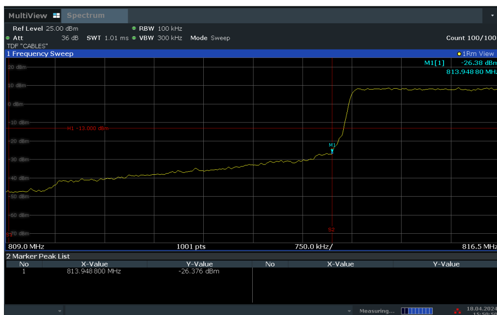
Plot 7-35. Channel Edge Plot (LTE Band 26 - 5MHz QPSK – Low Channel)
