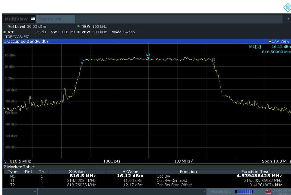
Plot 7-6. Occupied Bandwidth Plot (LTE Band 26 - 5MHz 16-QAM - Full RB)
