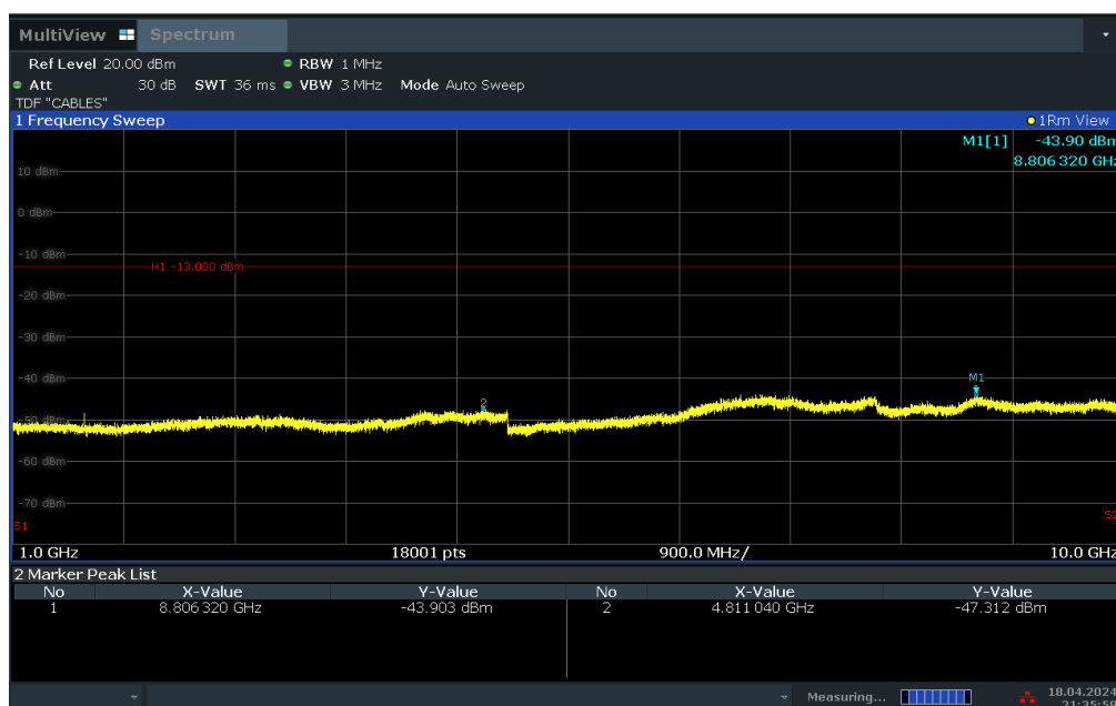
Plot 7-24. Conducted Spurious Plot (LTE Band 14 - 5MHz QPSK - RB Size 1, RB Offset 0 - Low Channel)
