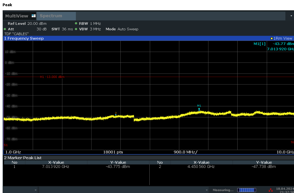
Plot 7-27. Conducted Spurious Plot (LTE Band 14 - 10MHz QPSK - RB Size 1, RB Offset 0 - Mid Channel)
