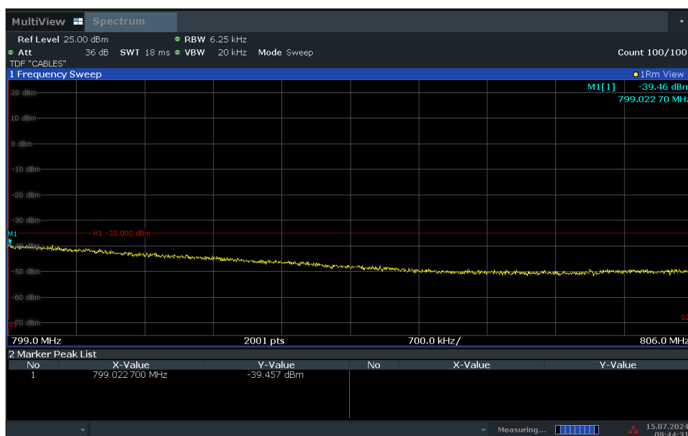
Plot 7-46. Upper Emission Mask Plot (LTE Band 14 - 10MHz QPSK – RB Size 50)
