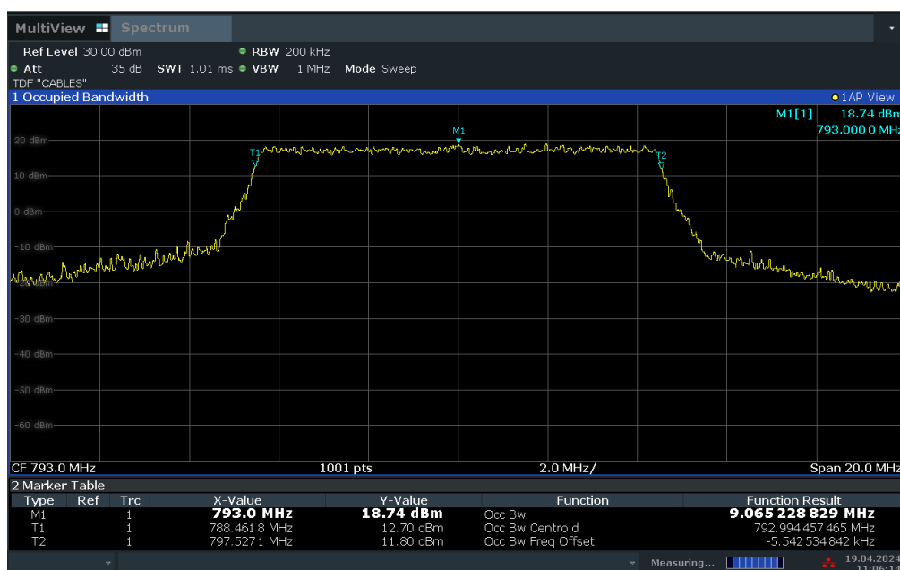
Plot 7-11. Occupied Bandwidth Plot (LTE Band 14 - 10MHz QPSK - Full RB)
