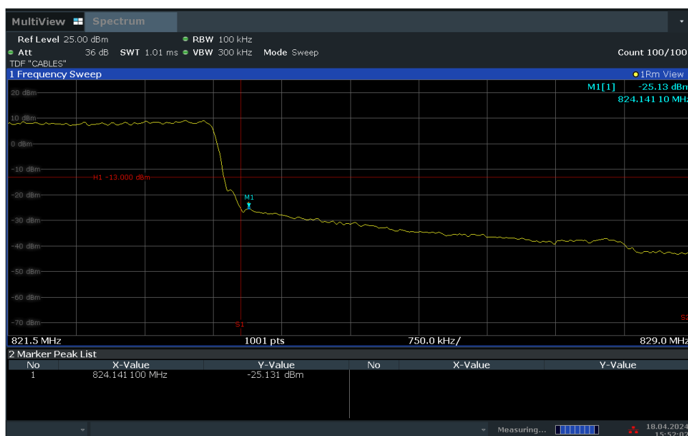
Plot 7-36. Channel Edge Plot (LTE Band 26 - 5MHz QPSK – High Channel)
