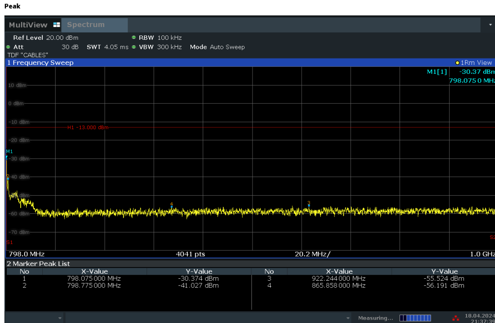
Plot 7-26. Conducted Spurious Plot (LTE Band 14 - 10MHz QPSK - RB Size 1, RB Offset 0 - Mid Channel)
