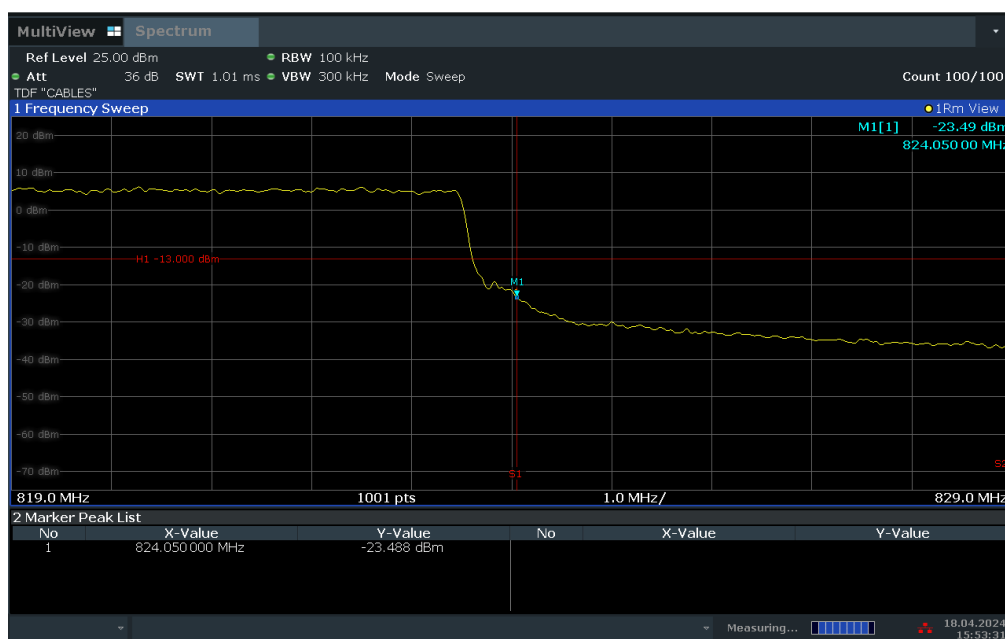
Plot 7-38. Channel Edge Plot (LTE Band 26 - 10MHz QPSK – High Channel)
