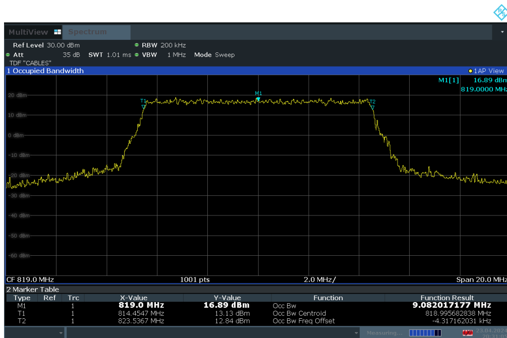
Plot 7-7. Occupied Bandwidth Plot (LTE Band 26 - 10MHz QPSK - Full RB)
