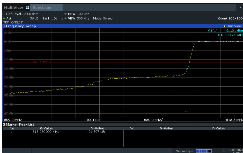
Plot 7-33. Channel Edge Plot (LTE Band 26 - 3MHz QPSK – Low Channel)
