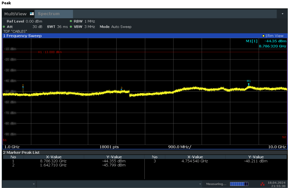
Plot 7-21. Conducted Spurious Plot (LTE Band 26 - 5MHz QPSK - RB Size 1, RB Offset 0 - High Channel)
