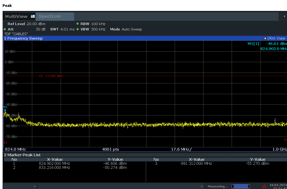
Plot 7-14. Conducted Spurious Plot (LTE Band 26 - 5MHz QPSK - RB Size 1, RB Offset 0 - Low Channel)
