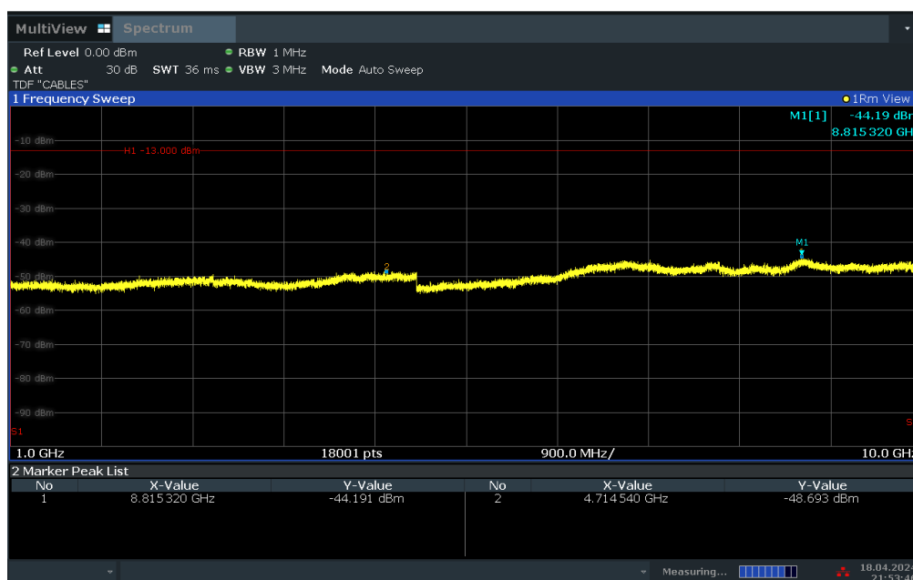
Plot 7-18. Conducted Spurious Plot (LTE Band 26 - 10MHz QPSK - RB Size 1, RB Offset 0 - Mid Channel)
