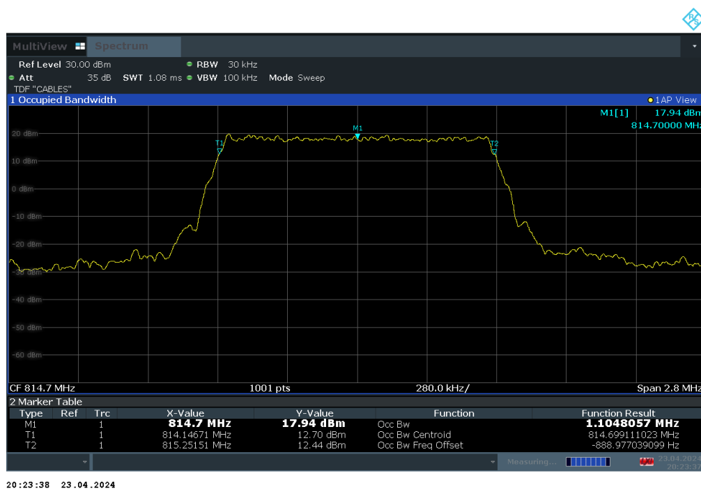
Plot 7-1. Occupied Bandwidth Plot (LTE Band 26 - 1.4MHz QPSK - Full RB)
