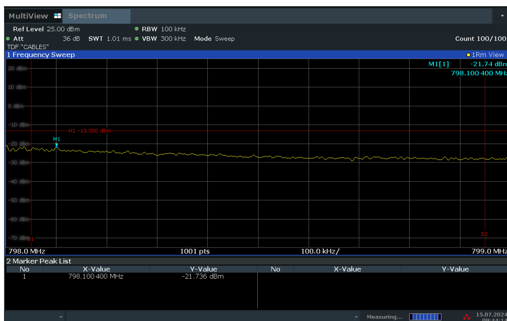
Plot 7-45. Upper Band Edge Plot (LTE Band 14 - 10MHz QPSK – RB Size 50)
