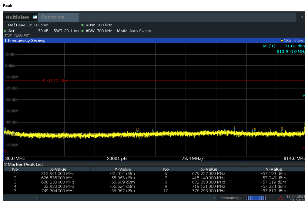
Plot 7-16. Conducted Spurious Plot (LTE Band 26 - 10MHz QPSK - RB Size 1, RB Offset 0 - Mid Channel)
