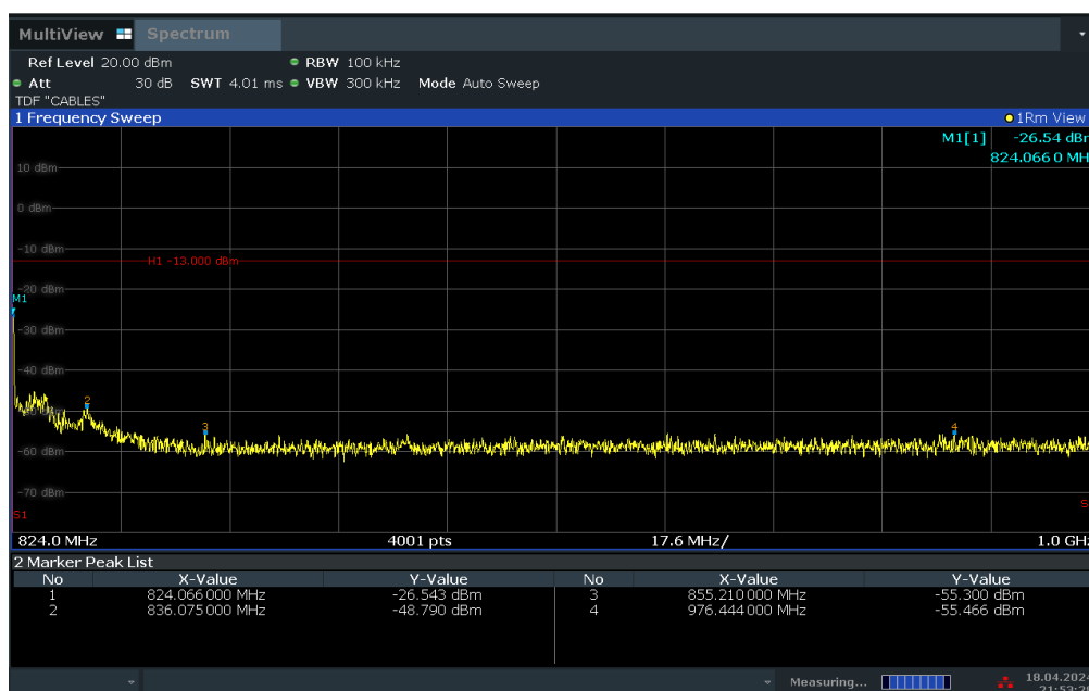
Plot 7-17. Conducted Spurious Plot (LTE Band 26 - 10MHz QPSK - RB Size 1, RB Offset 0 - Mid Channel)
