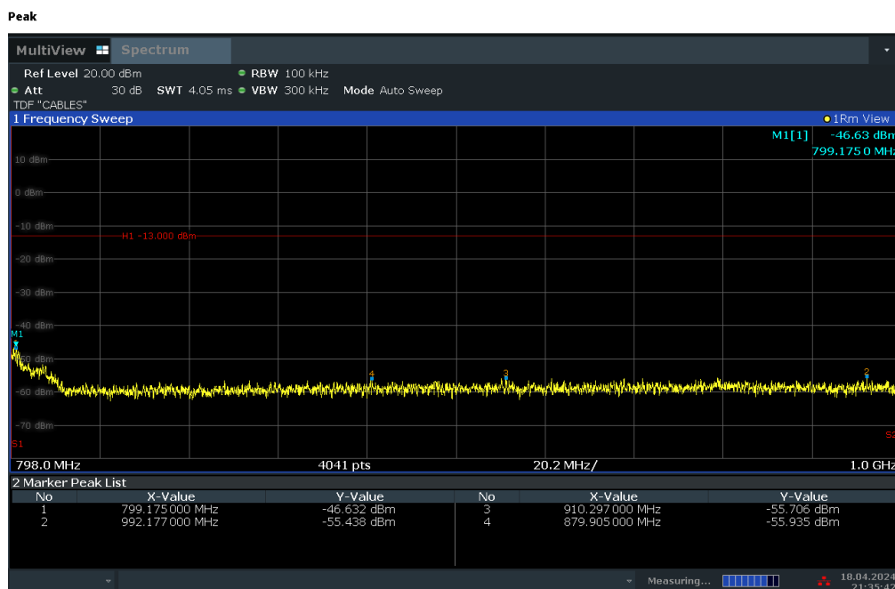
Plot 7-23. Conducted Spurious Plot (LTE Band 14 - 5MHz QPSK - RB Size 1, RB Offset 0 - Low Channel)
