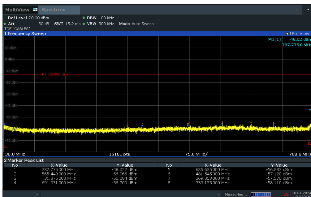
Plot 7-28. Conducted Spurious Plot (LTE Band 14 - 5MHz QPSK - RB Size 1, RB Offset 0 - High Channel)
