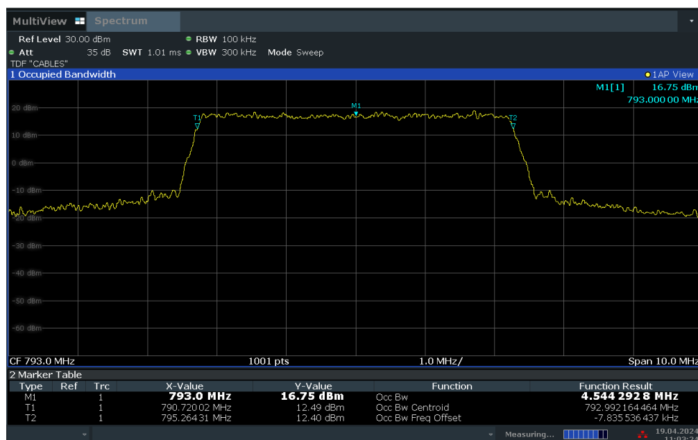
Plot 7-9. Occupied Bandwidth Plot (LTE Band 14 - 5MHz QPSK - Full RB)
