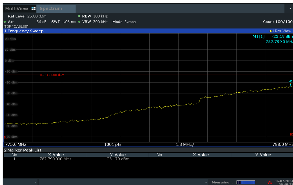
Plot 7-39. Lower Band Edge Plot (LTE Band 14 - 5MHz QPSK – RB Size 25)
