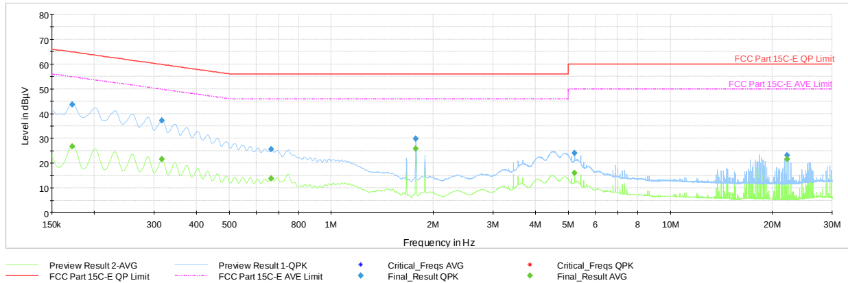
Plot 7-62. AC Line Conducted Plot with 802.11n- Ch.157 (N), with AC/DC Adapter & magnetic charger
