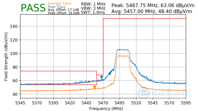
Plot 7-49. (Pk & Avg, Ch.100, 802.11n, MCS7)
