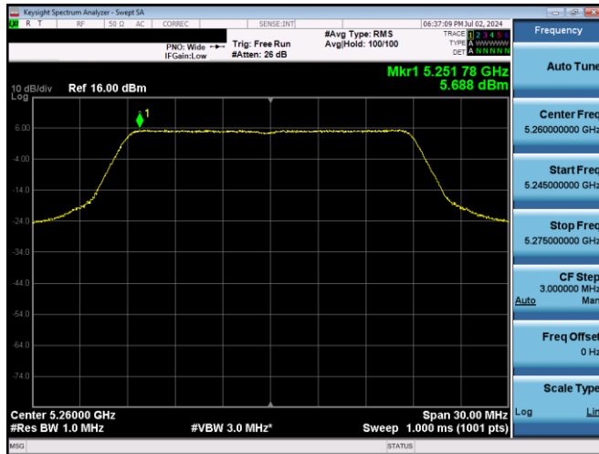
Plot 7-19. PSD (20MHz BW 802.11n - Ch. 52, MCS0)
