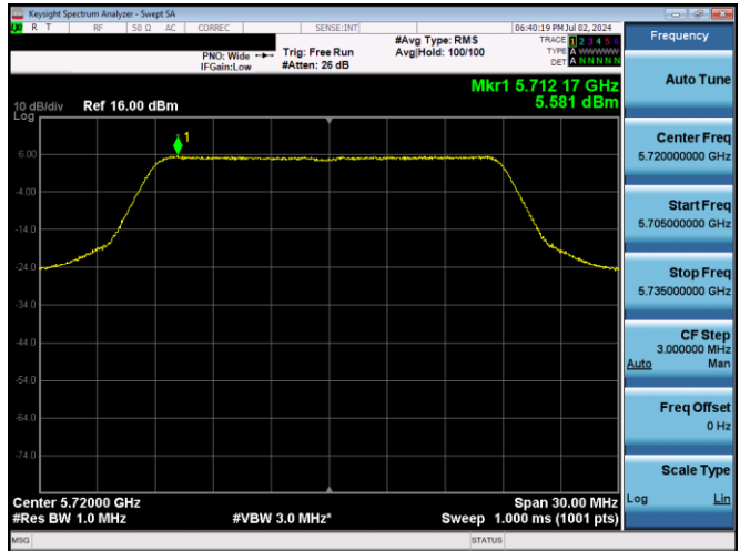
Plot 7-24. PSD (20MHz BW 802.11n - Ch. 144, MCS0)
