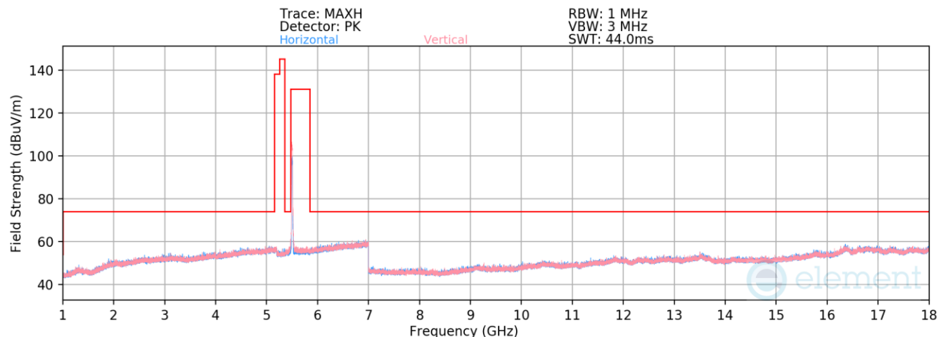
Plot 7-34. Radiated Spurious Emissions above 1GHz (802.11n – Ch. 100)
