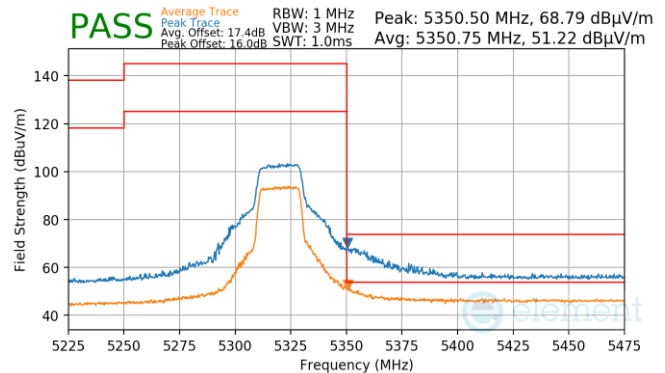
Plot 7-47. (Pk & Avg, Ch.64, 802.11n, MCS7)
