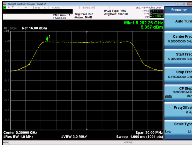
Plot 7-20. PSD (20MHz BW 802.11n - Ch. 60, MCS0)
