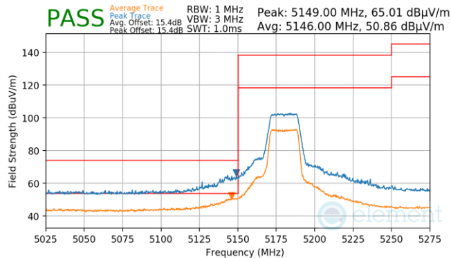
Plot 7-44. (Pk & Avg, Ch.36, 802.11n, MCS0)
