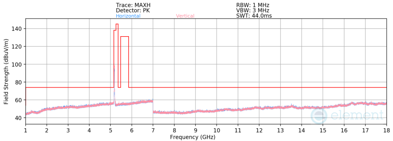
Plot 7-28. Radiated Spurious Emissions above 1GHz (802.11n – Ch. 36)
