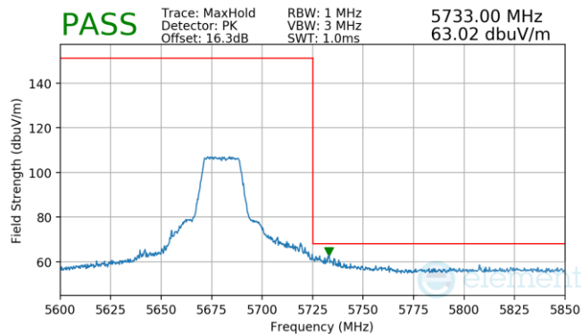
Plot 7-51. (Pk, Ch.136, 802.11n, MCS0)
