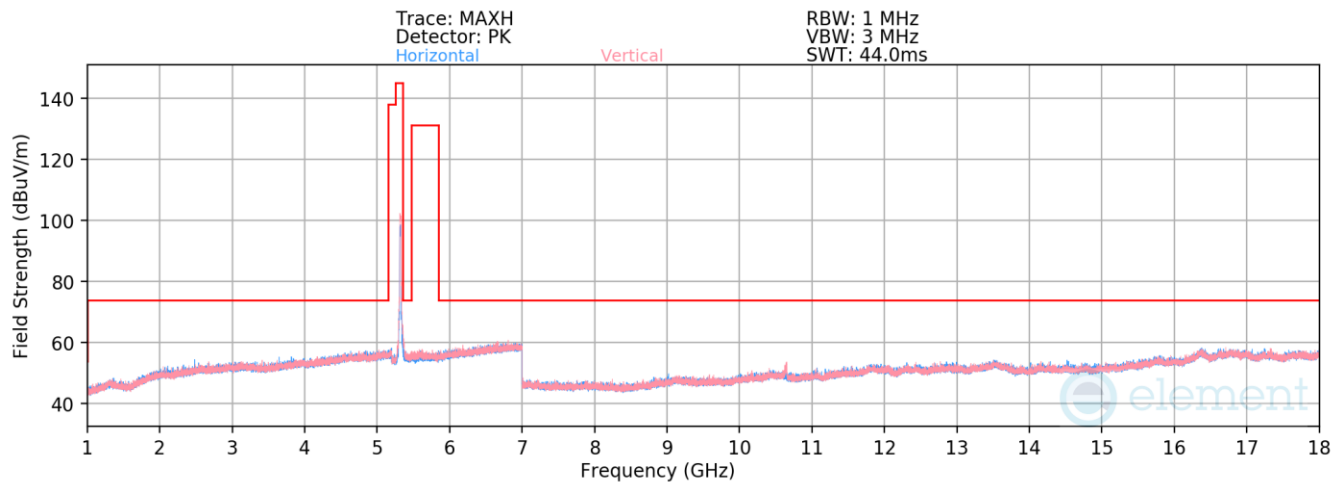
Plot 7-33. Radiated Spurious Emissions above 1GHz (802.11n – Ch. 64)
