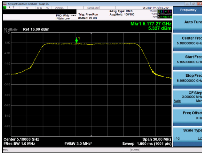
Plot 7-13. PSD (20MHz BW 802.11n - Ch. 36, MCS0)
