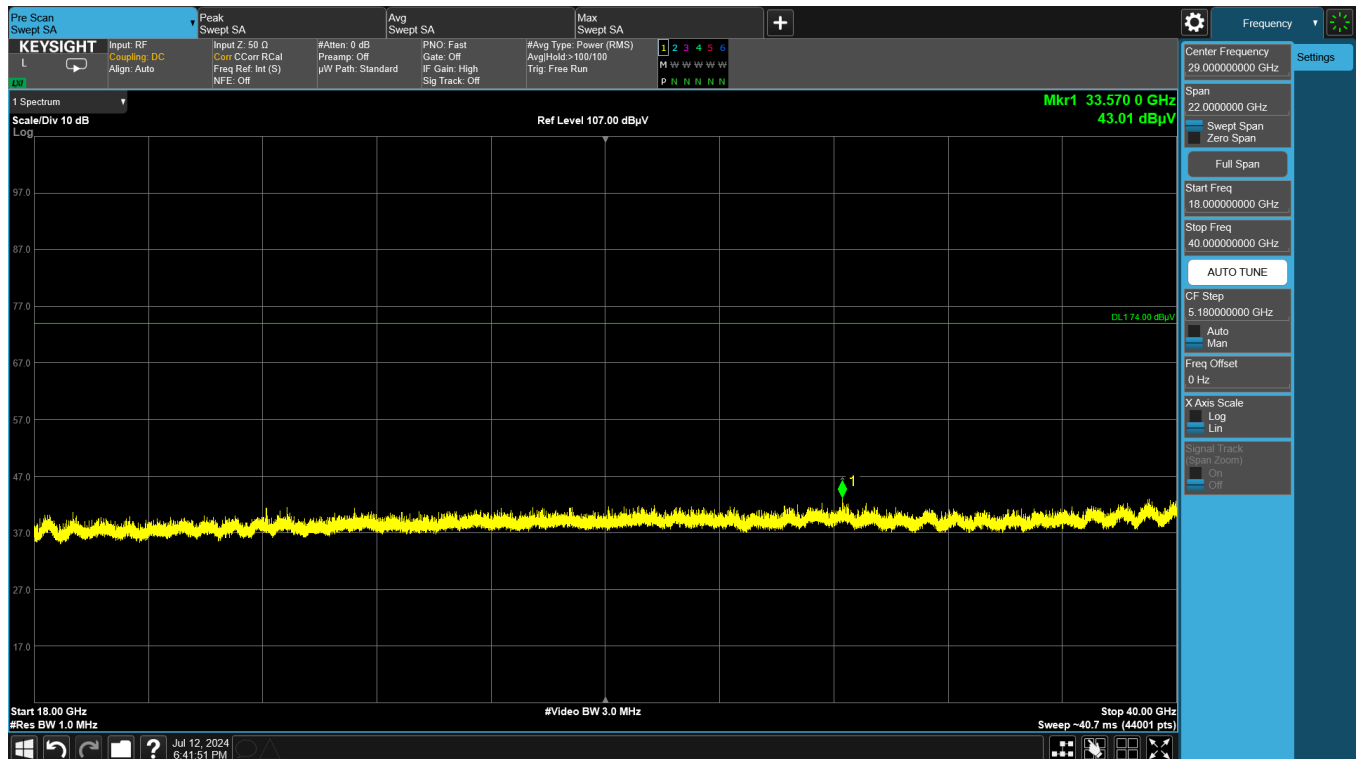
Plot 7-42. Radiated Spurious Emissions Simultaneous Transmission 18GHz – 40GHz Pol H
