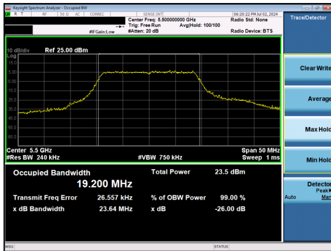
Plot 7-7. 26dB BW & 99% OBW (20MHz BW 802.11n – Ch. 100, MCS0)
