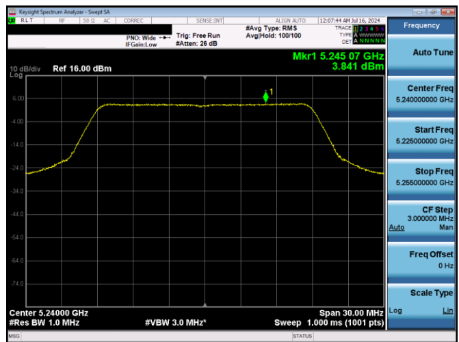
Plot 7-18. ISED PSD (20MHz BW 802.11n - Ch. 48, MCS0)
