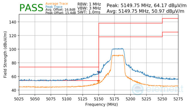
Plot 7-45. (Pk & Avg, Ch.36, 802.11n, MCS7)
