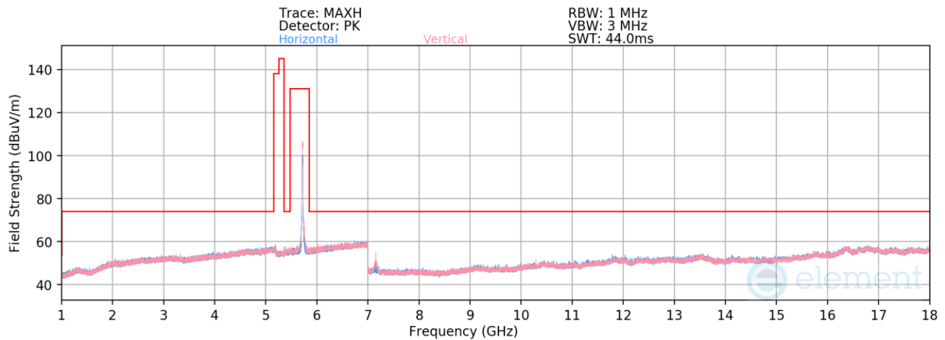
Plot 7-36. Radiated Spurious Emissions above 1GHz (802.11n – Ch. 144)
