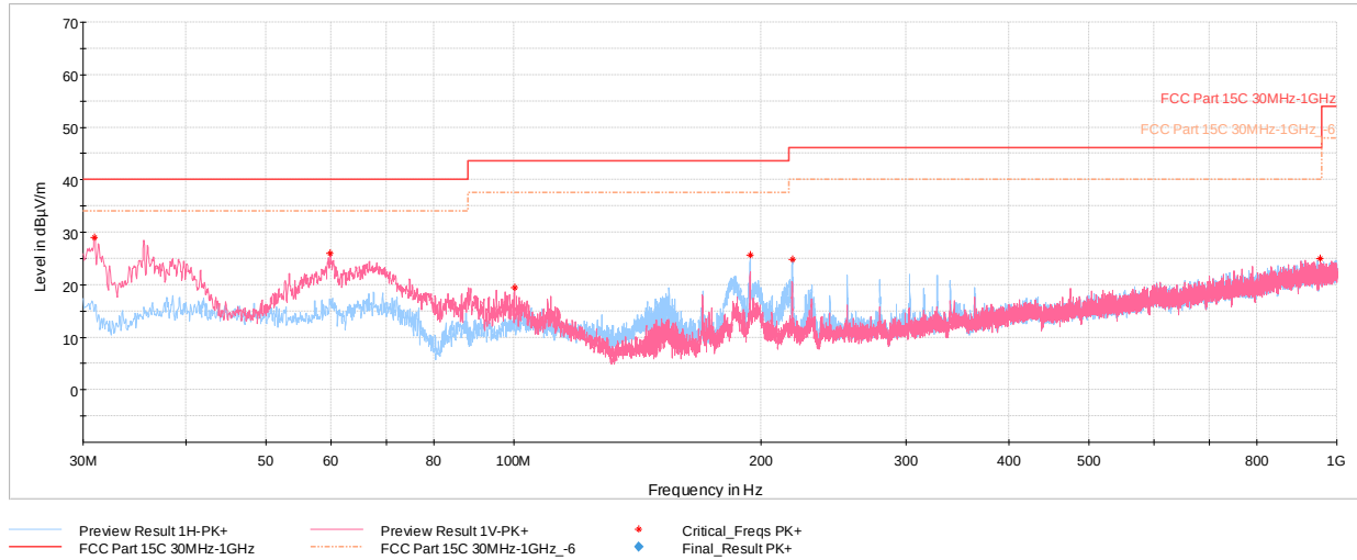
Plot 7-59. Radiated Spurious Emissions below 1GHz, 802.11n, Ch.157 with AC/DC Adapter & magnetic charger
