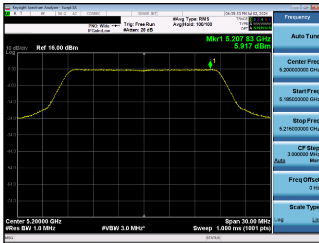
Plot 7-14. PSD (20MHz BW 802.11n - Ch. 40, MCS0)
