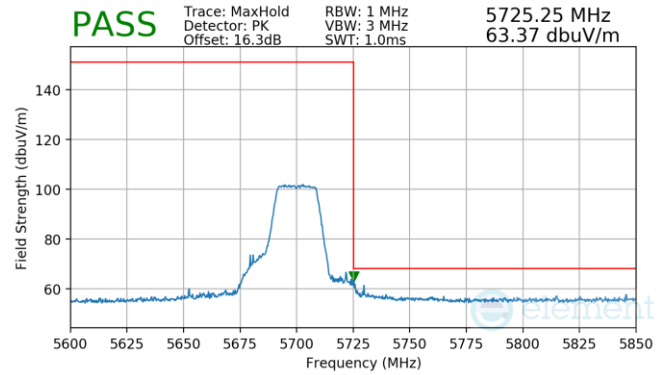
Plot 7-53. (Pk, Ch.140, 802.11n, MCS0)
