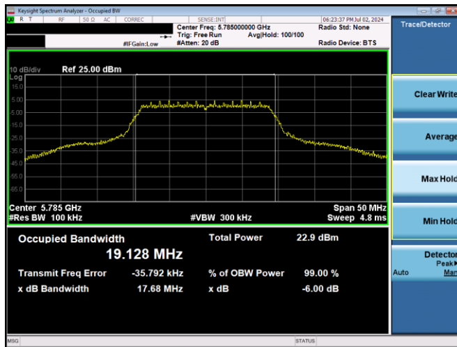
Plot 7-11. 6dB BW & 99% OBW (20MHz BW 802.11n – Ch. 157, MCS0)
