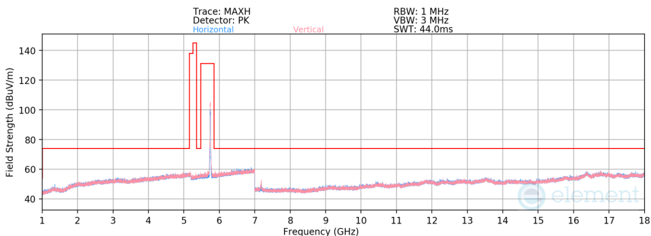
Plot 7-37. Radiated Spurious Emissions above 1GHz (802.11n – Ch. 149)
