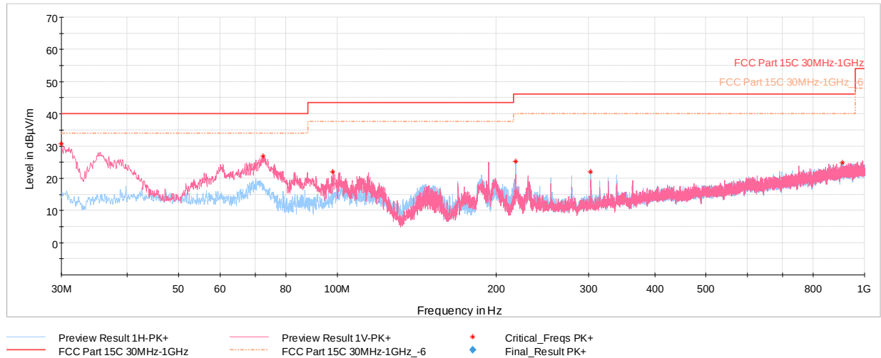
Plot 7-60. Radiated Spurious Emissions – Simultaneous Transmission 30MHz – 1GHz, with AC/DC Adapter & magnetic charger
