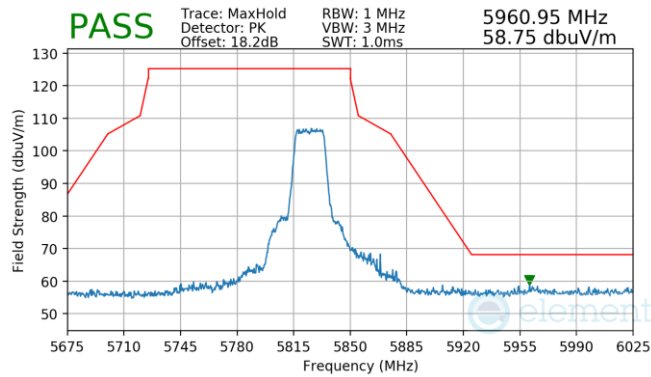
Plot 7-57. (Pk, Ch.165, 802.11n, MCS0)
