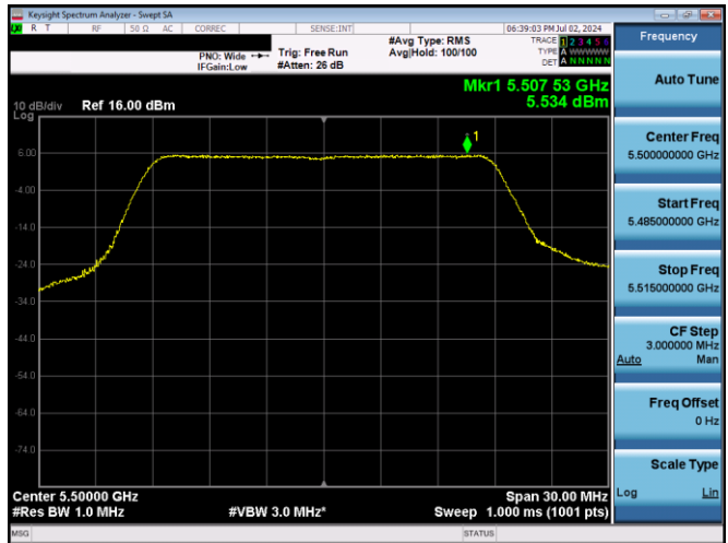
Plot 7-22. PSD (20MHz BW 802.11n - Ch. 100, MCS0)
