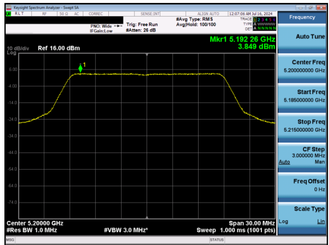
Plot 7-17. ISED PSD (20MHz BW 802.11n - Ch. 40, MCS0)
