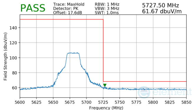
Plot 7-52. (Pk, Ch.136, 802.11n, MCS7)
