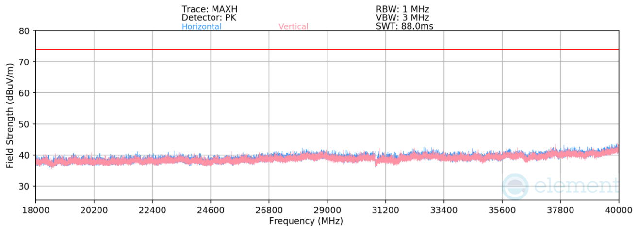
Plot 7-39. Radiated Spurious Emissions 18GHz-40GHz (802.11n – Ch. 157)
