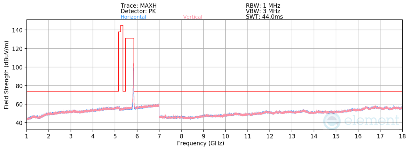
Plot 7-40. Radiated Spurious Emissions above 1GHz (802.11n – Ch. 165)
