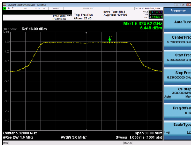
Plot 7-21. PSD (20MHz BW 802.11n - Ch. 64, MCS0)
