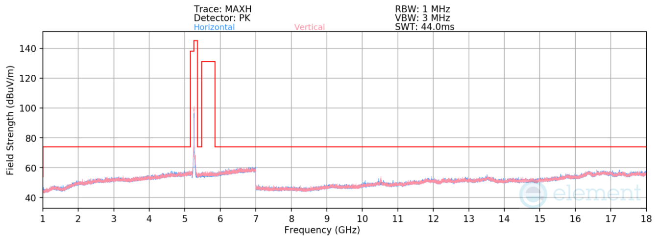
Plot 7-31. Radiated Spurious Emissions above 1GHz (802.11n – Ch. 52)
