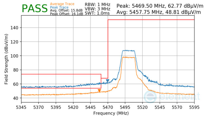
Plot 7-48. (Pk & Avg, Ch.100, 802.11n, MCS0)
