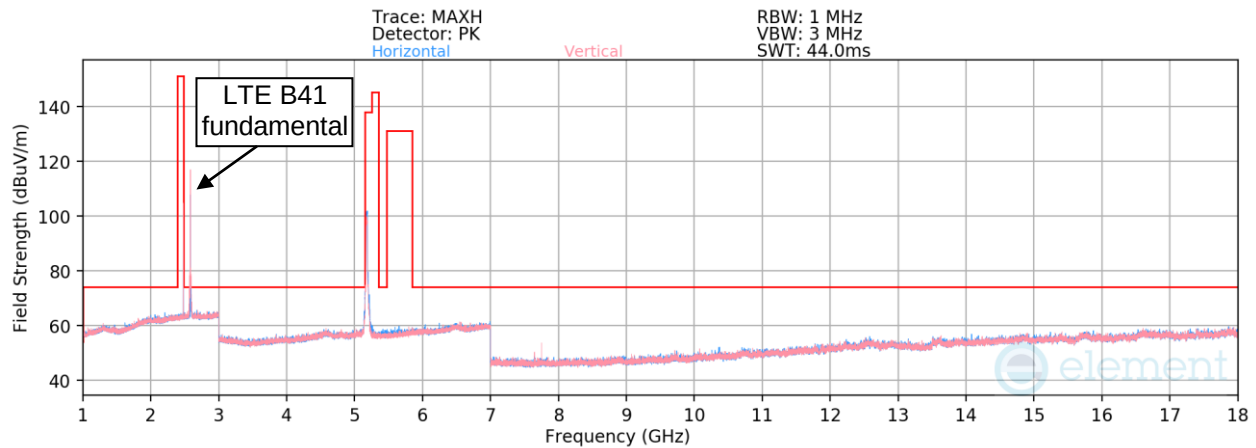
Plot 7-41. Radiated Spurious Emissions Simultaneous Transmission 1GHz – 18GHz
