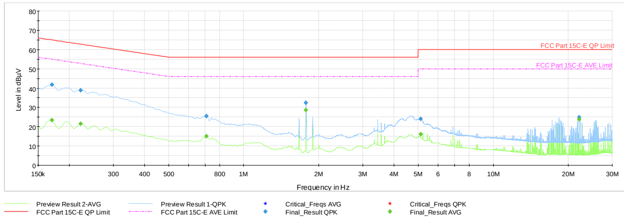
Plot 7-61. AC Line Conducted Plot with 802.11n – Ch.157 (L1), with AC/DC Adapter & magnetic charger
