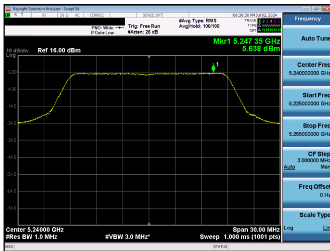
Plot 7-15. PSD (20MHz BW 802.11n - Ch. 48, MCS0)
