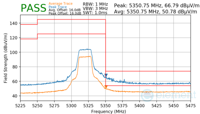
Plot 7-46. (Pk & Avg, Ch.64, 802.11n, MCS0)
