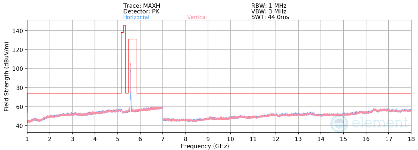
Plot 7-35. Radiated Spurious Emissions above 1GHz (802.11n – Ch. 116)
