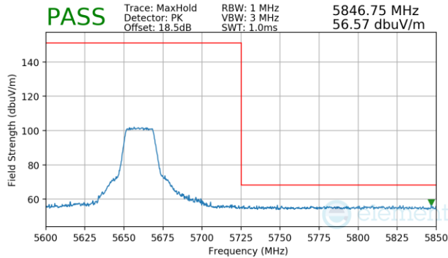
Plot 7-50. (Pk, Ch.132, 802.11n, MCS0)
