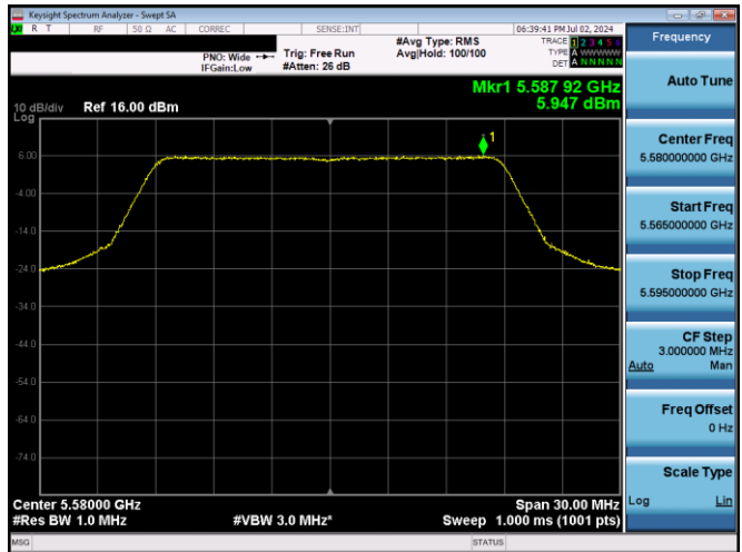
Plot 7-23. PSD (20MHz BW 802.11n - Ch. 116, MCS0)
