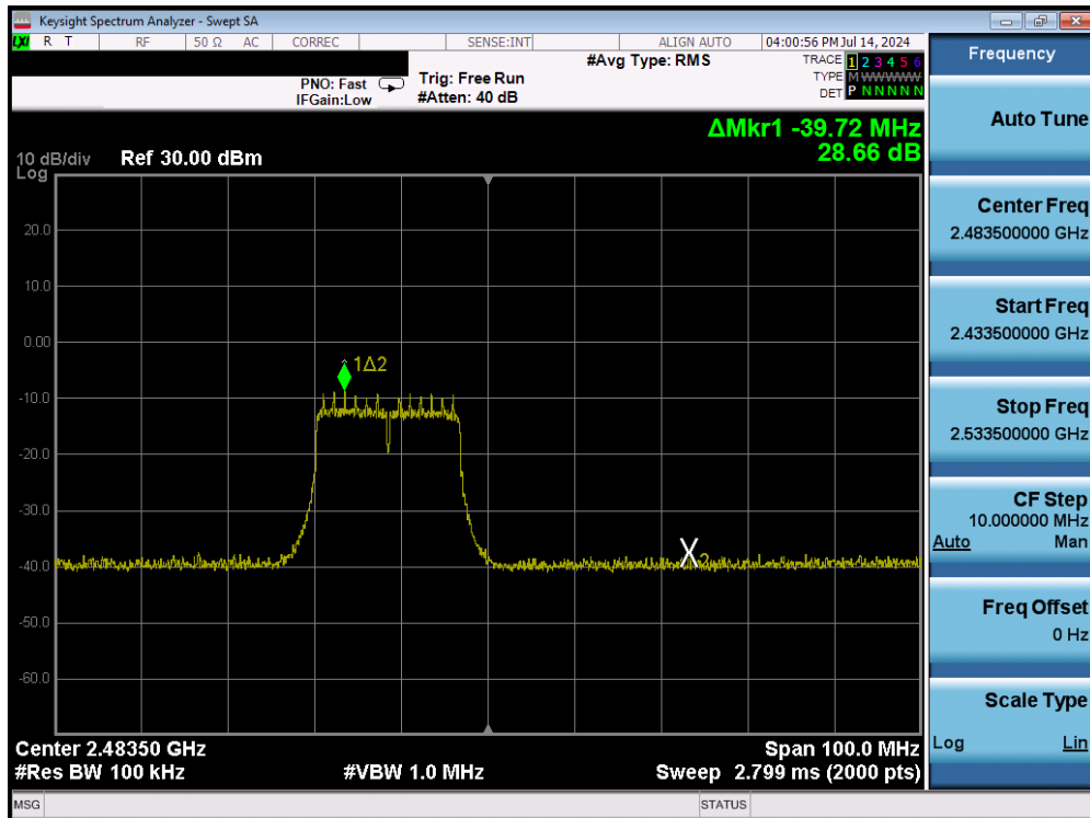
Plot 7-36. Band Edge Plot (802.11g – Ch. 13) – 6Mbps
