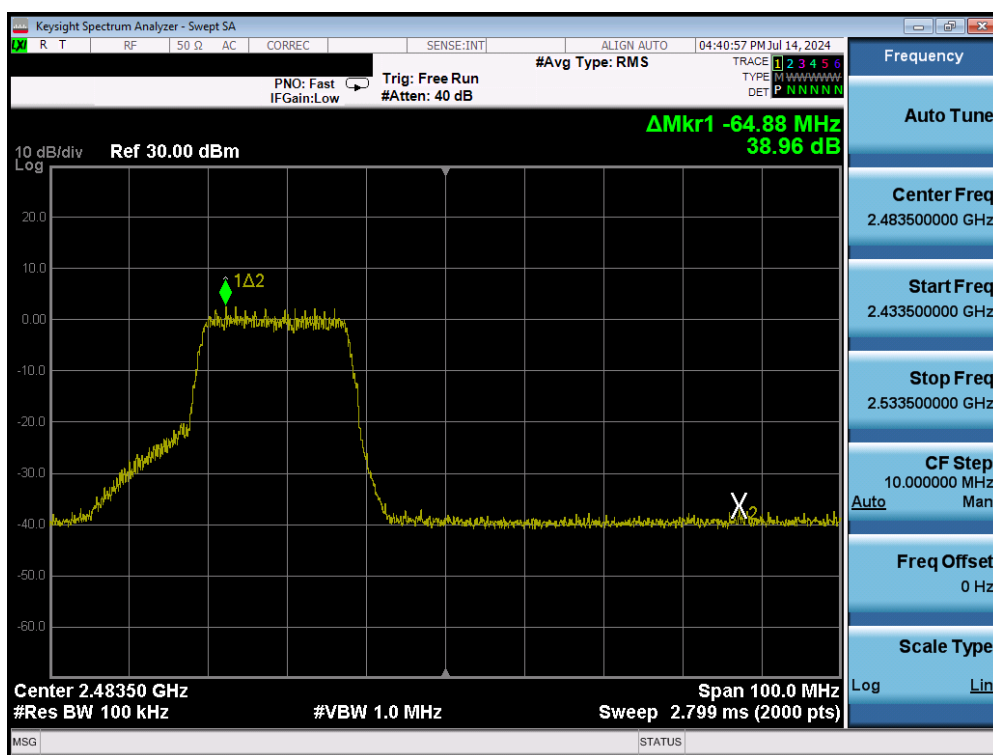
Plot 7-47. Band Edge Plot (802.11n (2.4GHz) – Ch. 11) – MCS7
