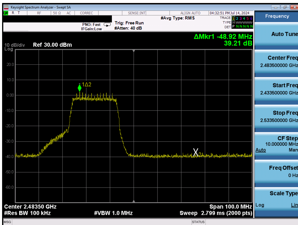
Plot 7-43. Band Edge Plot (802.11n (2.4GHz) – Ch. 12) – MCS0
