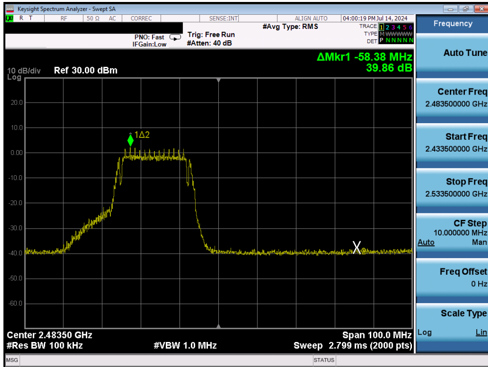
Plot 7-35. Band Edge Plot (802.11g – Ch. 12) – 6Mbps
