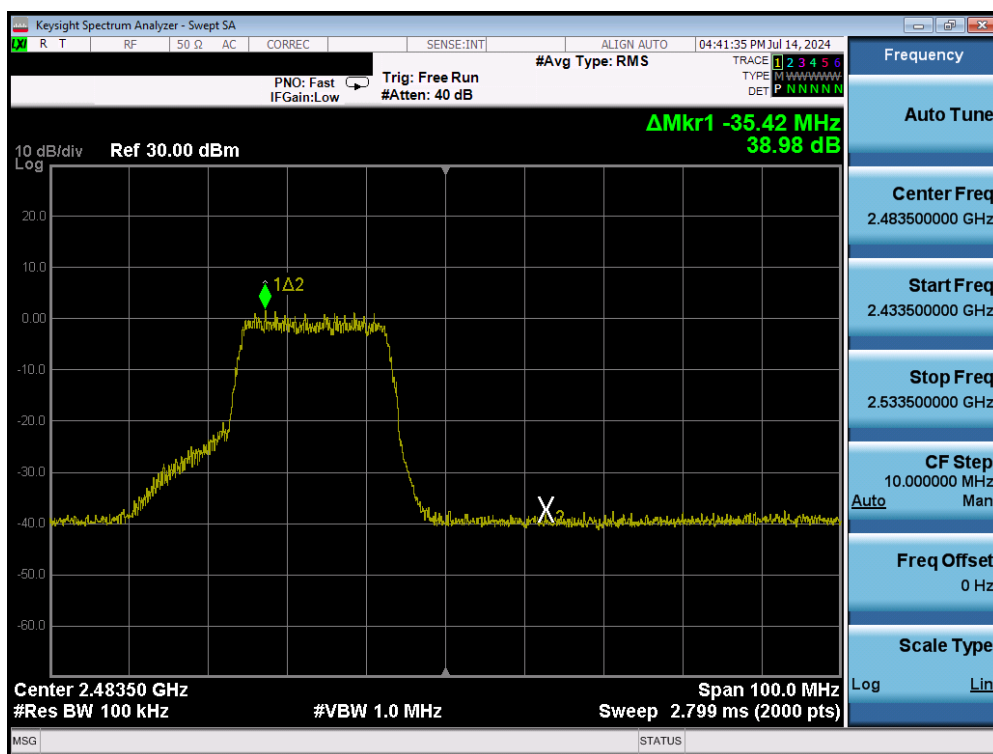
Plot 7-48. Band Edge Plot (802.11n (2.4GHz) – Ch. 12) – MCS7
