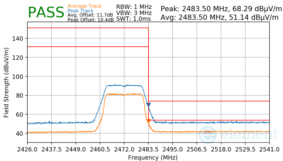
Plot 7-76. Radiated Restricted Upper Band Edge Measurement
