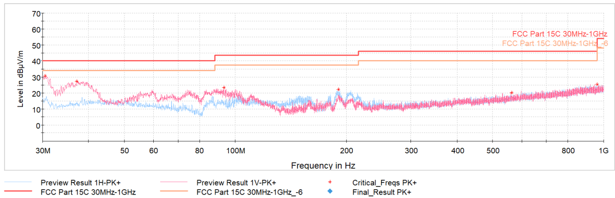
Plot 7-77. Radiated Spurious Emissions below 1GHz 11b Ch.6, with AC/DC Adapter + Magnetic Charger
