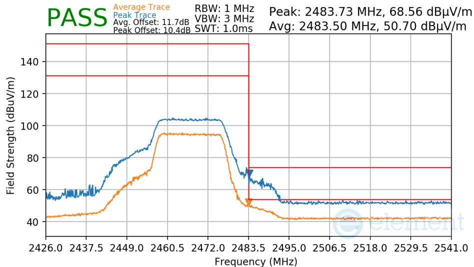
Plot 7-75. Radiated Restricted Upper Band Edge Measurement
