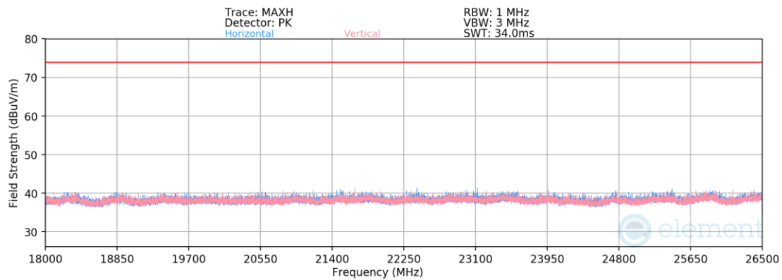
Plot 7-58. Radiated Spurious Emissions Above 18GHz (802.11b – Ch. 6)
