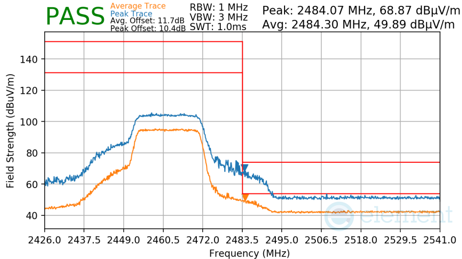
Plot 7-74. Radiated Restricted Upper Band Edge Measurement
