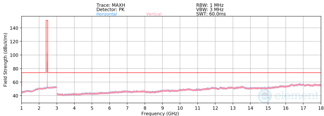
Plot 7-59. Radiated Spurious Emissions above 1GHz (802.11b – Ch. 11)
