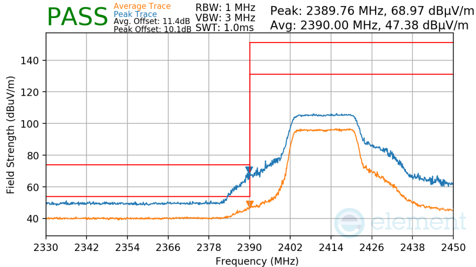
Plot 7-72. Radiated Restricted Lower Band Edge Measurement
