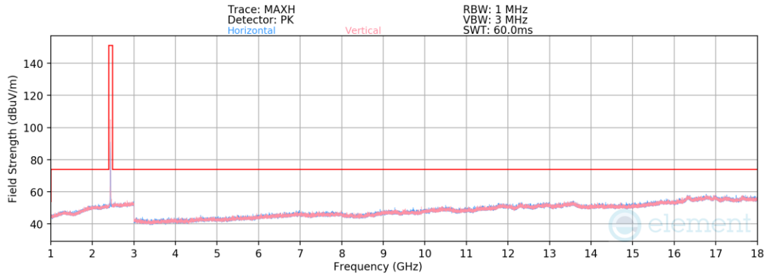
Plot 7-57. Radiated Spurious Emissions above 1GHz (802.11b – Ch. 6)
