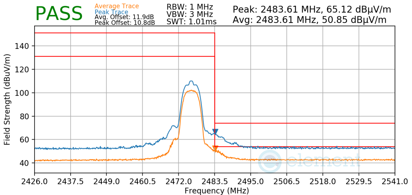
Plot 7-49. Radiated Restricted Upper Band Edge Measurement
