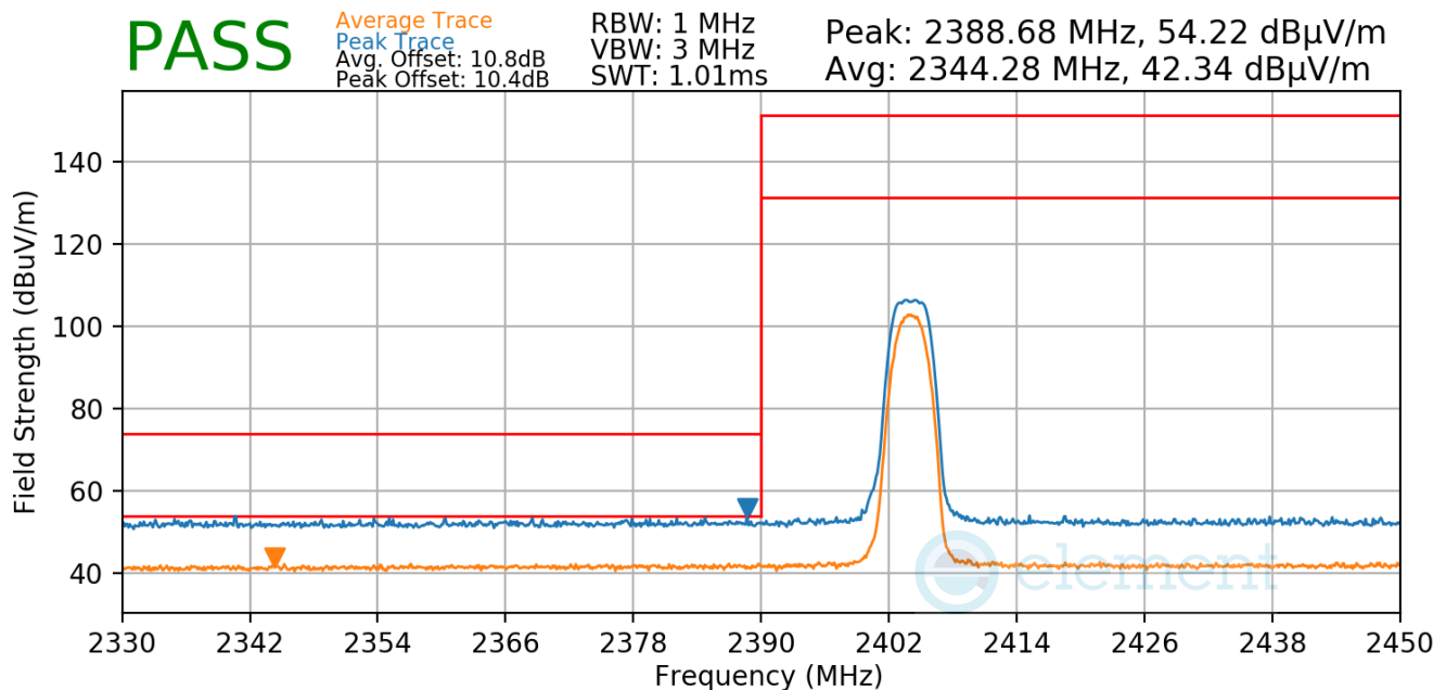
Plot 7-46. Radiated Restricted Lower Band Edge Measurement
