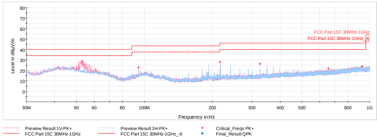
Plot 7-52. Radiated Spurious Emissions Below 1GHz (4Mbps – Ch.73 with AC/DC Adapter)
