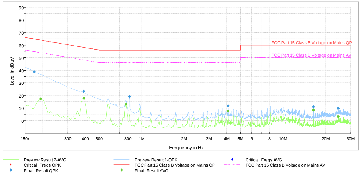
Plot 7-54. AC Line Conducted Plot with Bluetooth HDR (N, 4Mbps - Ch.73 with Laptop)
