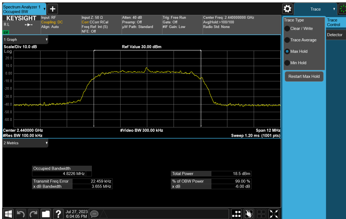
Plot 7-11. 6dB BW & 99% OBW Plot (Bluetooth (HDRp8), 8Mbps – Ch. 37)
