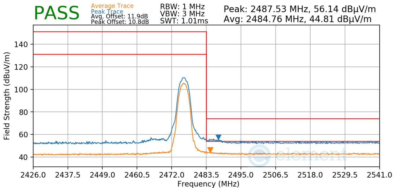
Plot 7-48. Radiated Restricted Upper Band Edge Measurement
