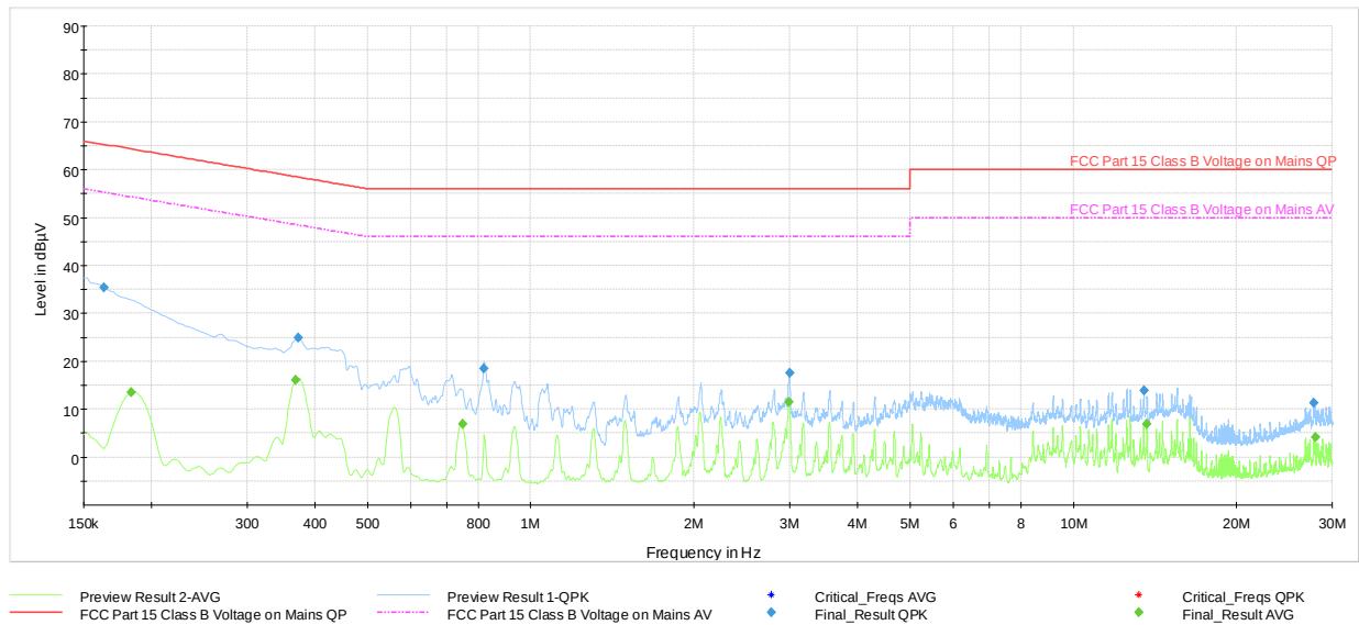
Plot 7-53. AC Line Conducted Plot with Bluetooth HDR (L1, 4Mbps - Ch.73 with Laptop)
