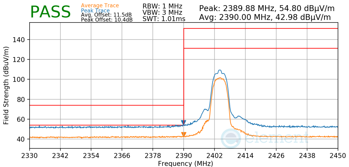
Plot 7-45. Radiated Restricted Lower Band Edge Measurement
