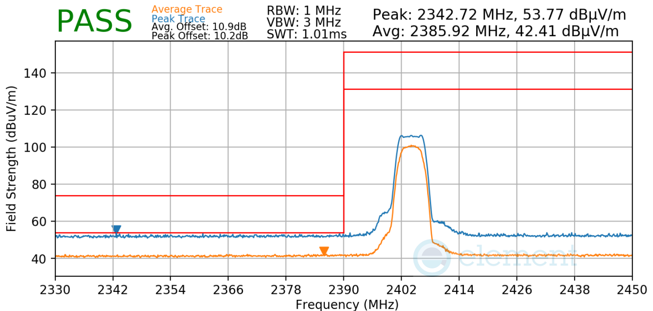
Plot 7-47. Radiated Restricted Lower Band Edge Measurement
