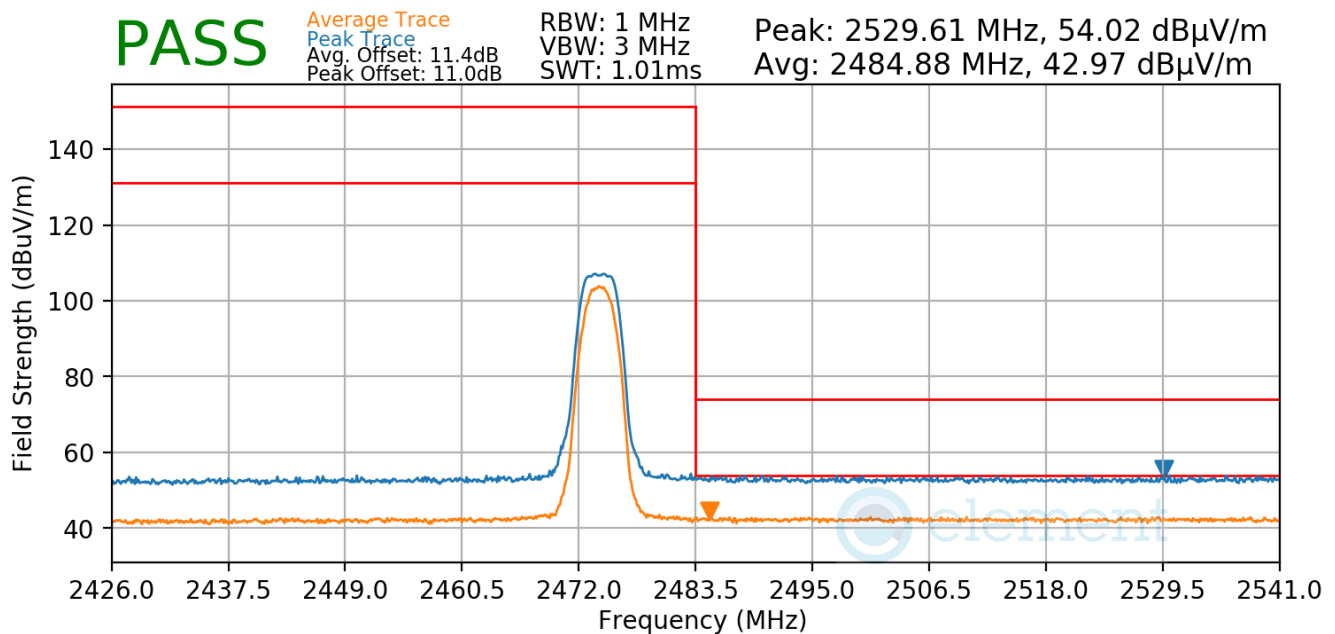
Plot 7-50. Radiated Restricted Upper Band Edge Measurement
