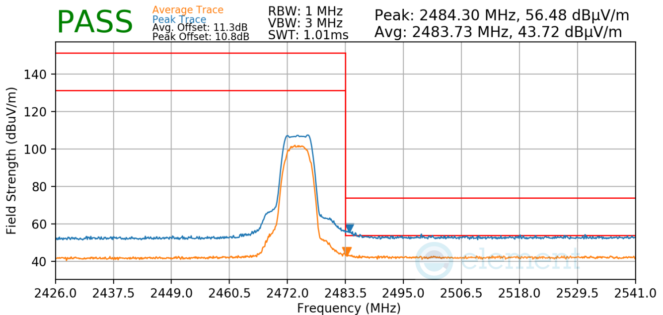
Plot 7-51. Radiated Restricted Upper Band Edge Measurement
