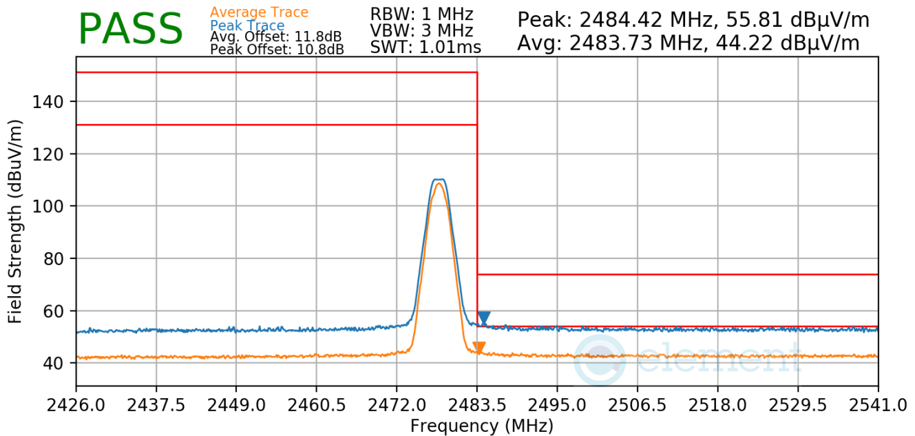
Plot 7-34. Radiated Restricted Upper Band Edge Measurement (Average & Peak)
