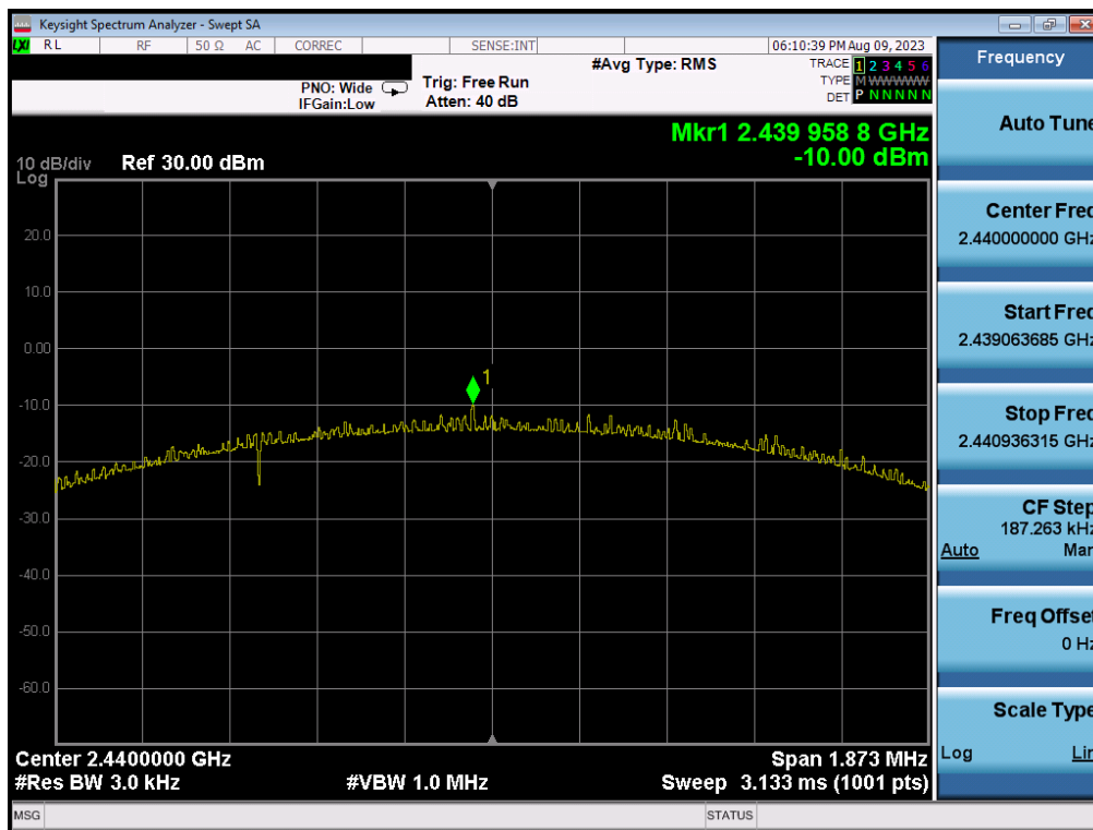
Plot 7-11. Power Spectral Density Plot (Bluetooth (LE), 1Mbps – Ch. 19)
