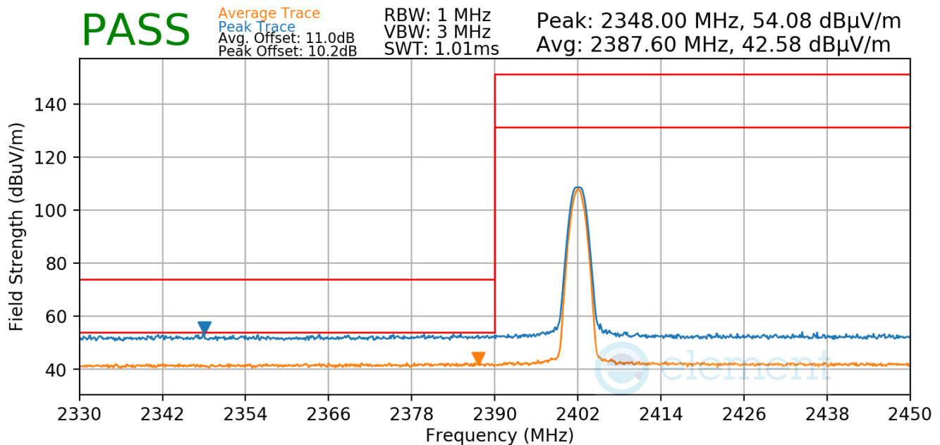
Plot 7-31. Radiated Restricted Lower Band Edge Measurement (Average & Peak)
