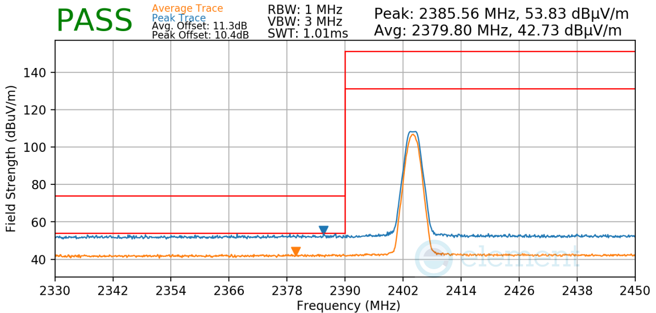
Plot 7-33. Radiated Restricted Lower Band Edge Measurement (Average & Peak)
