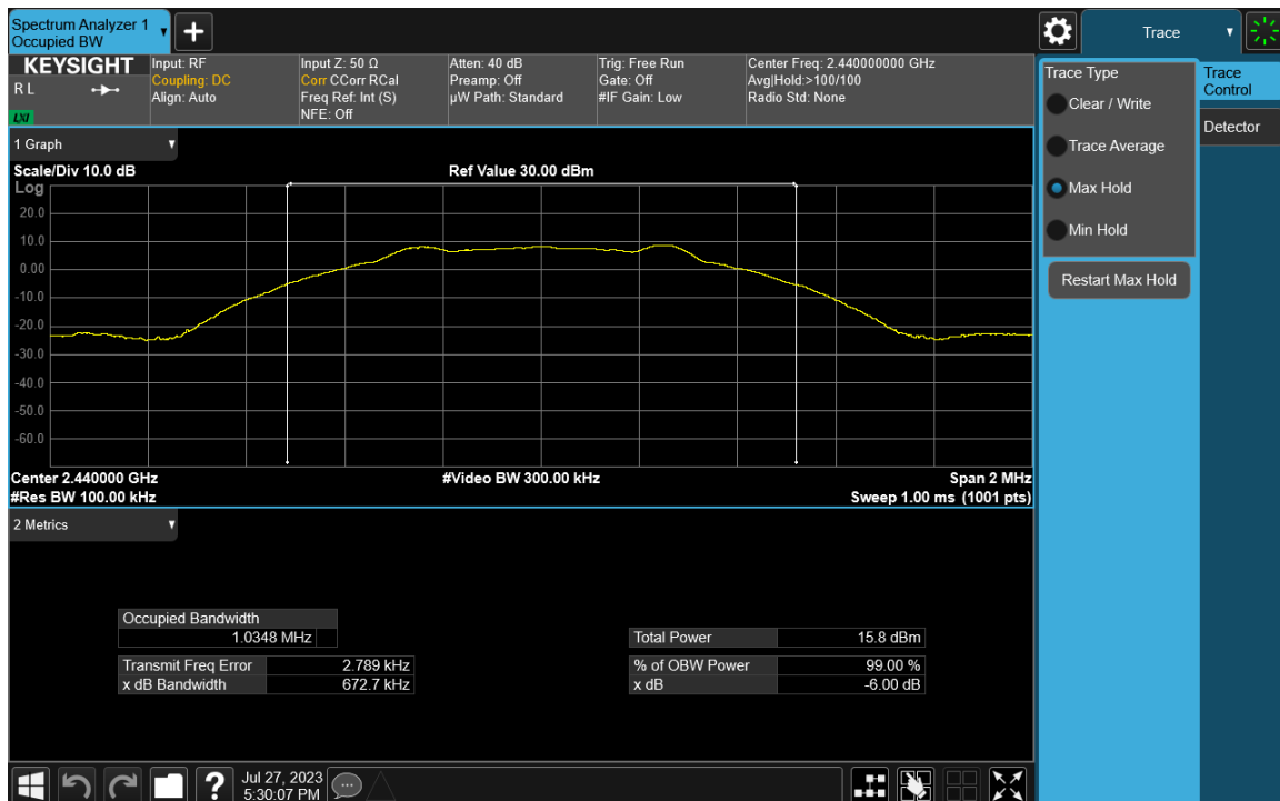
Plot 7-2. 6dB BW & 99% OBW Plot (Bluetooth (LE), 1Mbps – Ch. 19)
