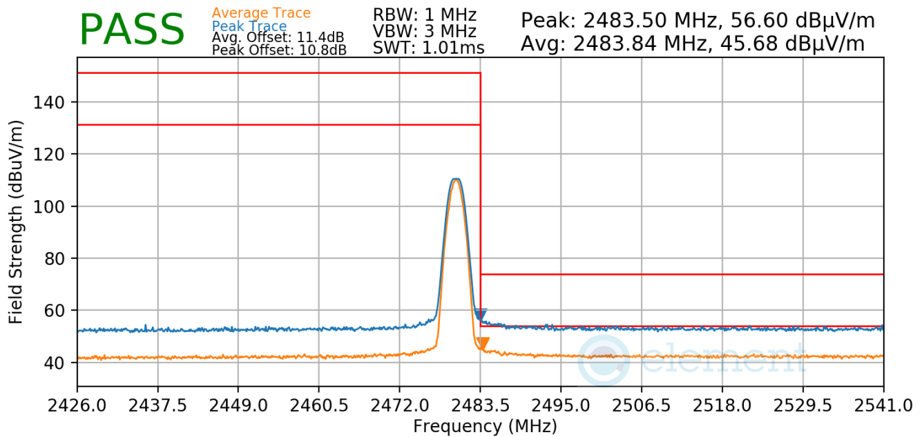
Plot 7-32. Radiated Restricted Upper Band Edge Measurement (Average & Peak)
