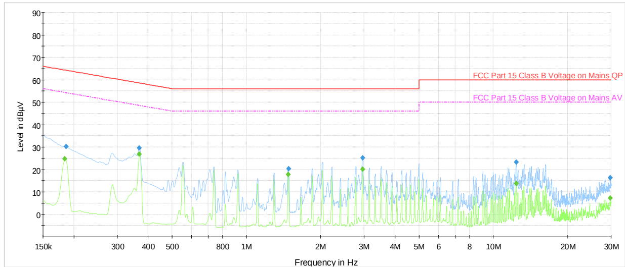
Plot 7-37. AC Line Conducted Plot with Bluetooth LE (L1, 1Mbps – Ch.39 with Laptop)
