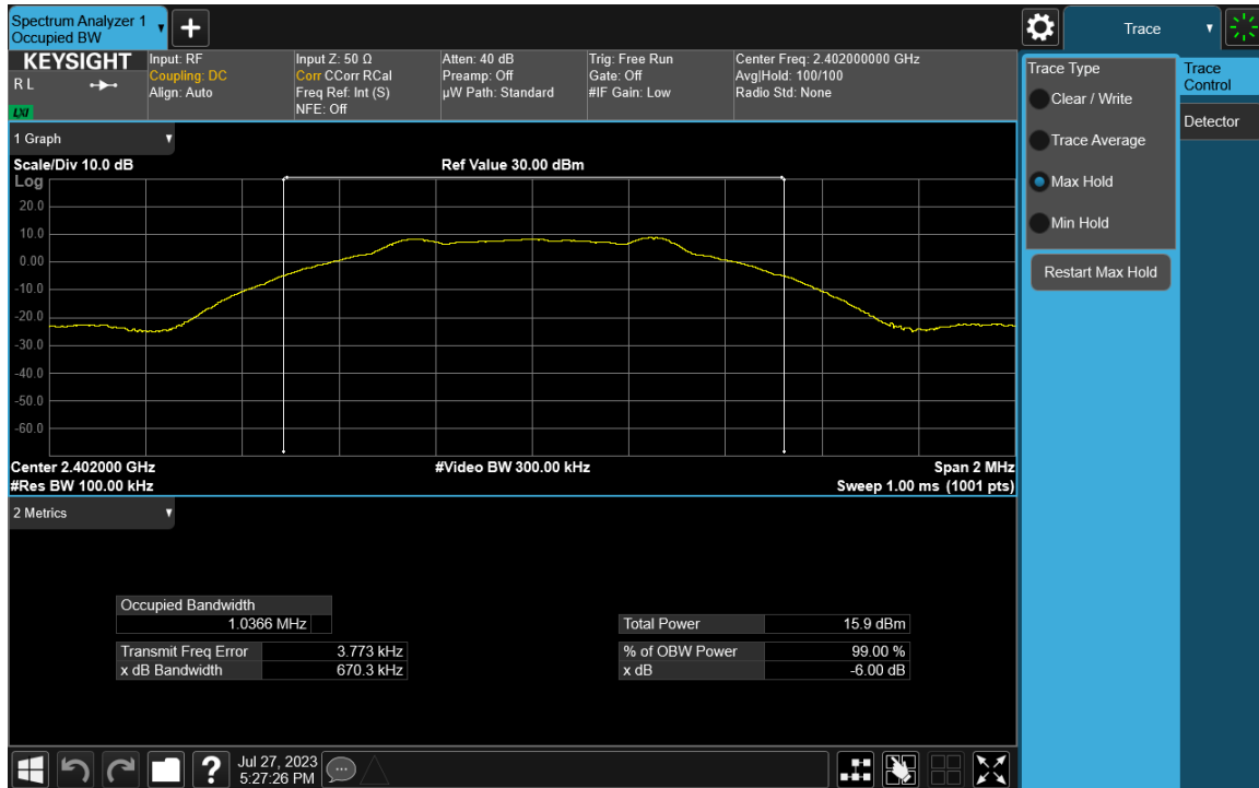
Plot 7-1. 6dB BW & 99% OBW Plot (Bluetooth (LE), 1Mbps – Ch. 0)
