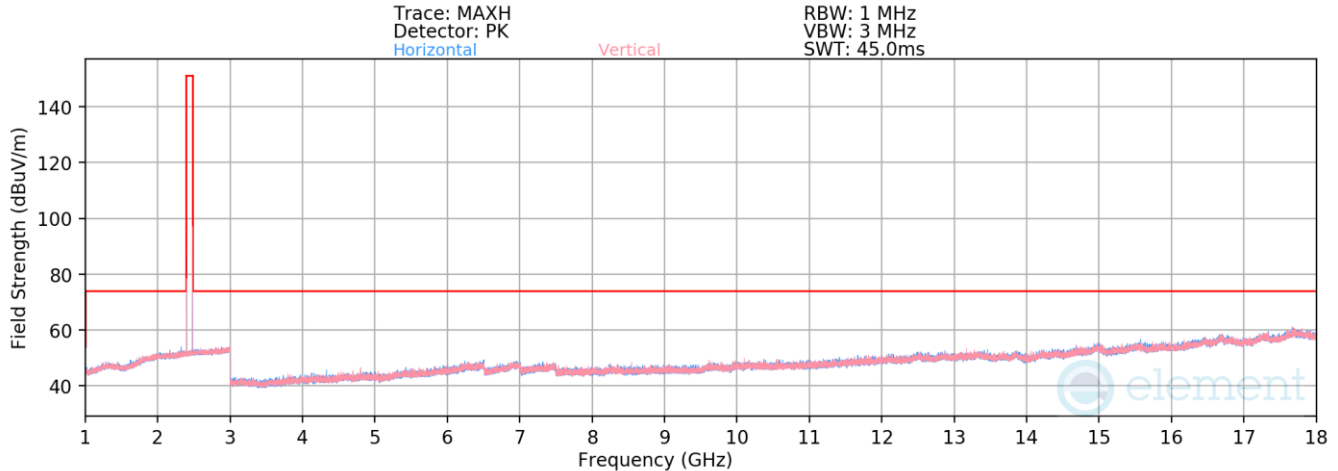
Plot 7-28. Radiated Spurious Emissions – Co-Tx 1-18GHz
