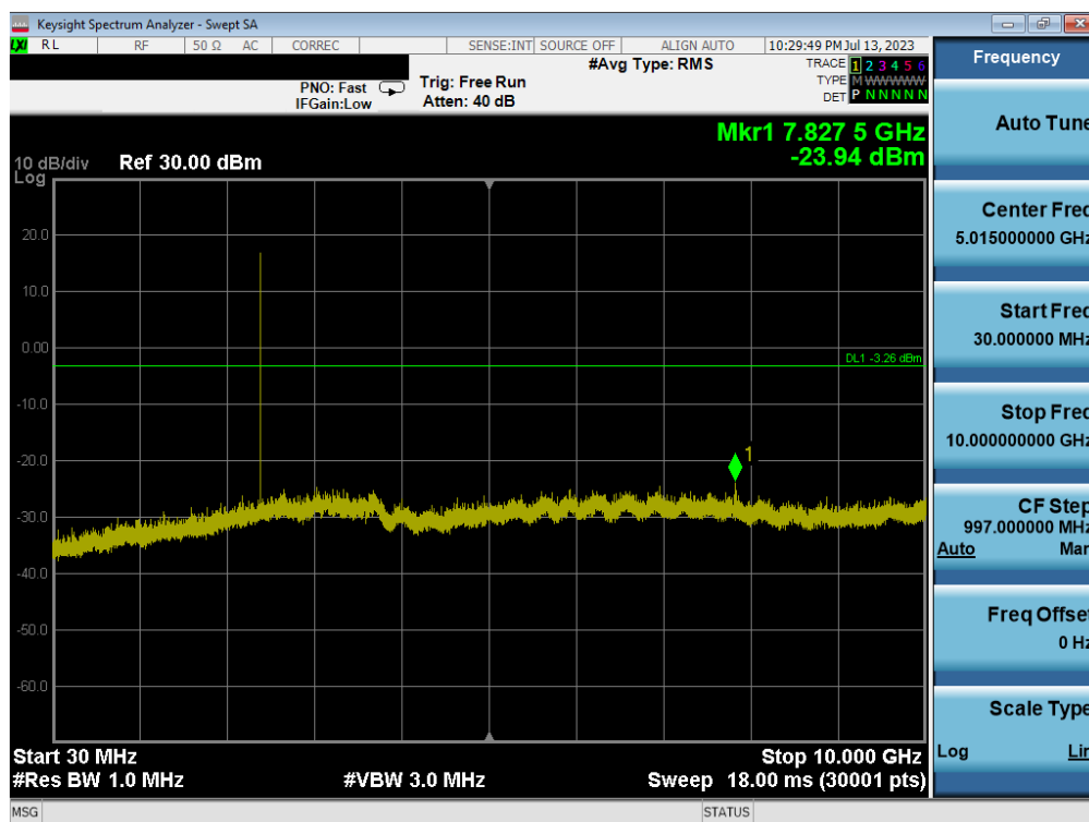
Plot 7-17. Conducted Spurious Plot (Bluetooth (LE), 1Mbps, ePA – Ch. 0)
