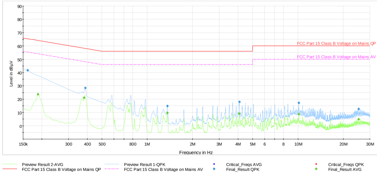
Plot 7-38. AC Line Conducted Plot with Bluetooth LE (N, 1Mbps – Ch.39, with Laptop)
