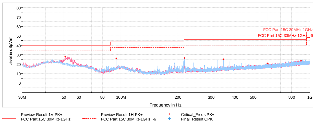
Plot 7-35. Radiated Spurious Emissions Below 1GHz (1Mbps – Ch.39, Pol. H & V, with AC/DC Adapter)
