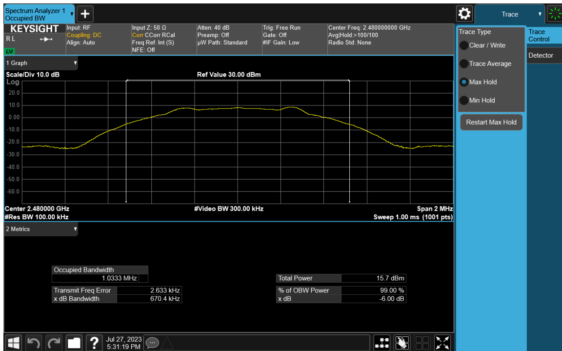
Plot 7-3. 6dB BW & 99% OBW Plot (Bluetooth (LE), 1Mbps – Ch. 39)
