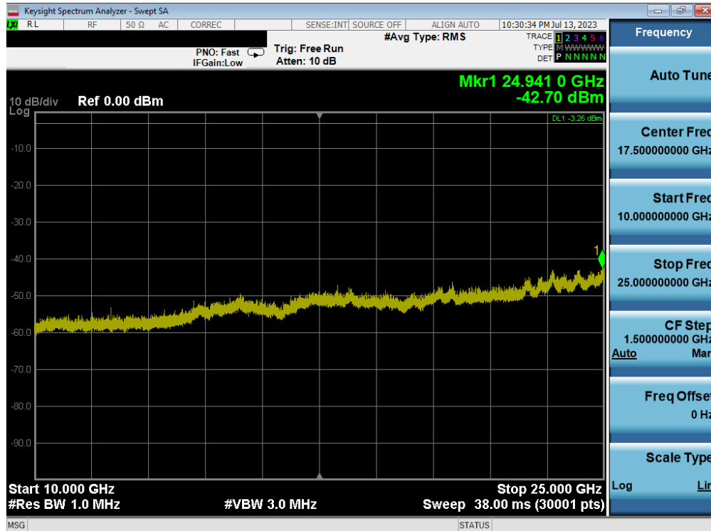
Plot 7-18. Conducted Spurious Plot (Bluetooth (LE), 1Mbps, ePA – Ch. 0)
