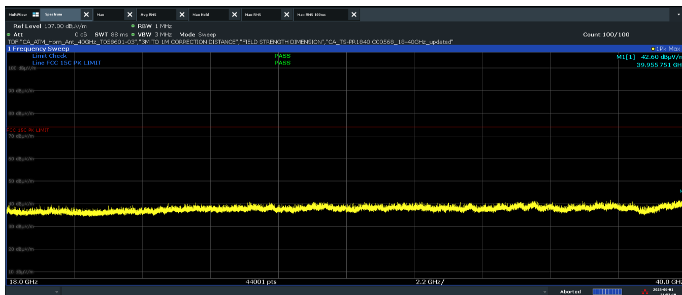
Plot 7-26. Radiated Spurious Emissions Above 18GHz H Polarity (1Mbps – Ch. 39)
