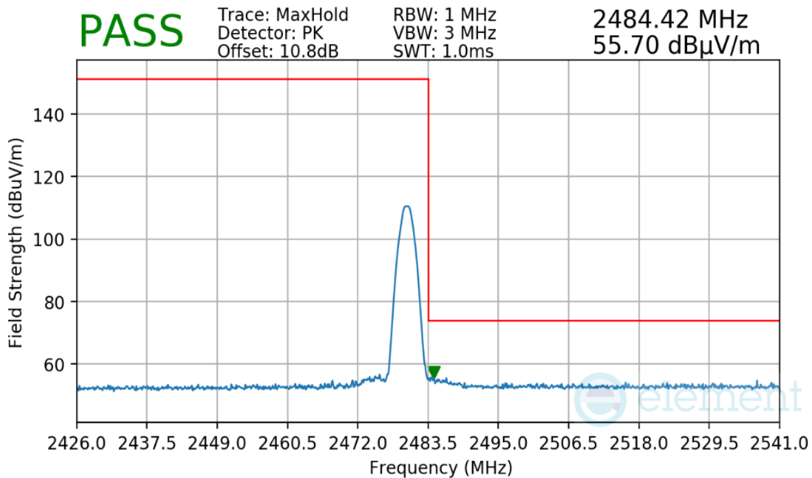
Plot 7-37. Radiated Restricted Upper Band Edge Measurement
