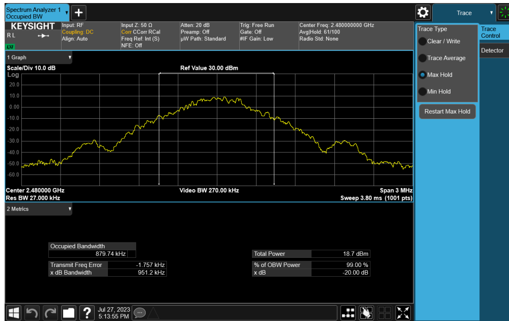
Plot 7-3. 20dB BW and 99% OBW Plot (Bluetooth, GFSK – Ch. 78)
