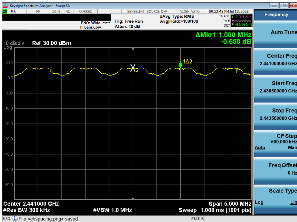
Plot 7-16. Channel Spacing Plot (Bluetooth, 8DPSK)
