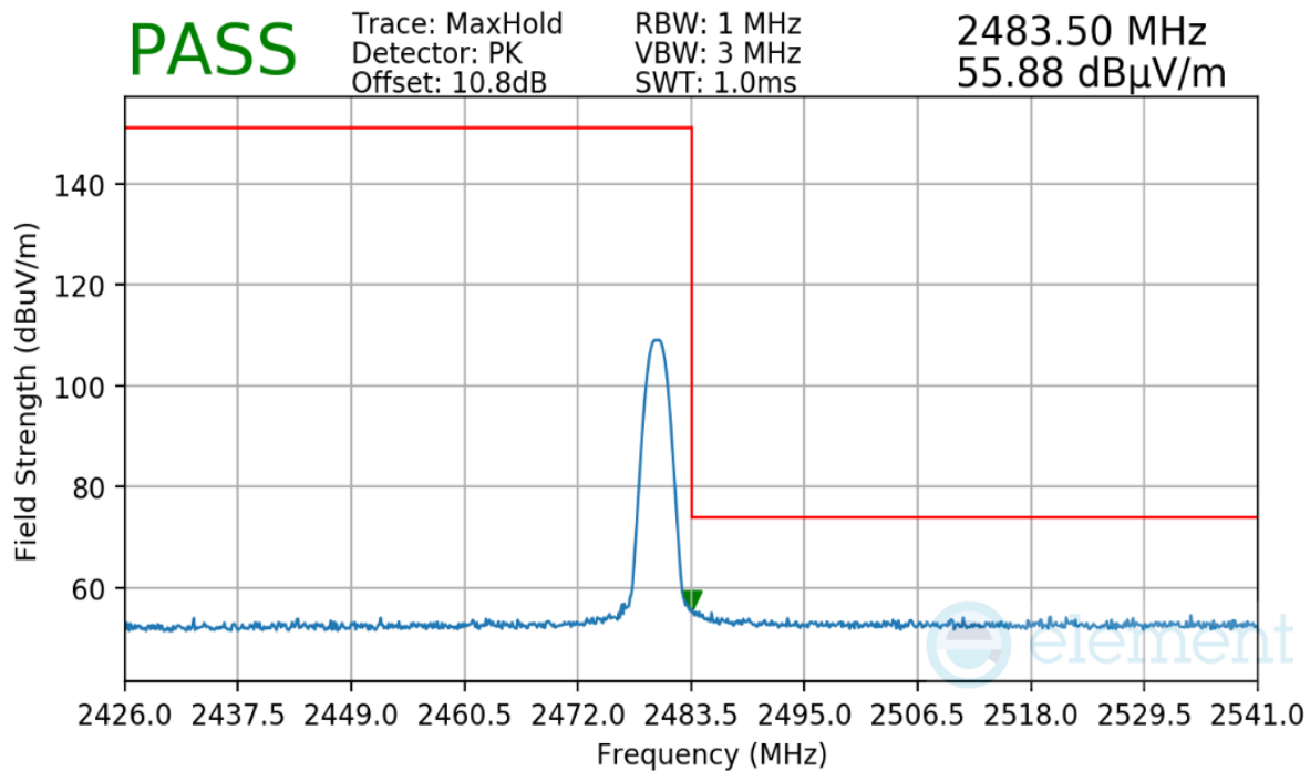
Plot 7-36. Radiated Restricted Upper Band Edge Measurement
