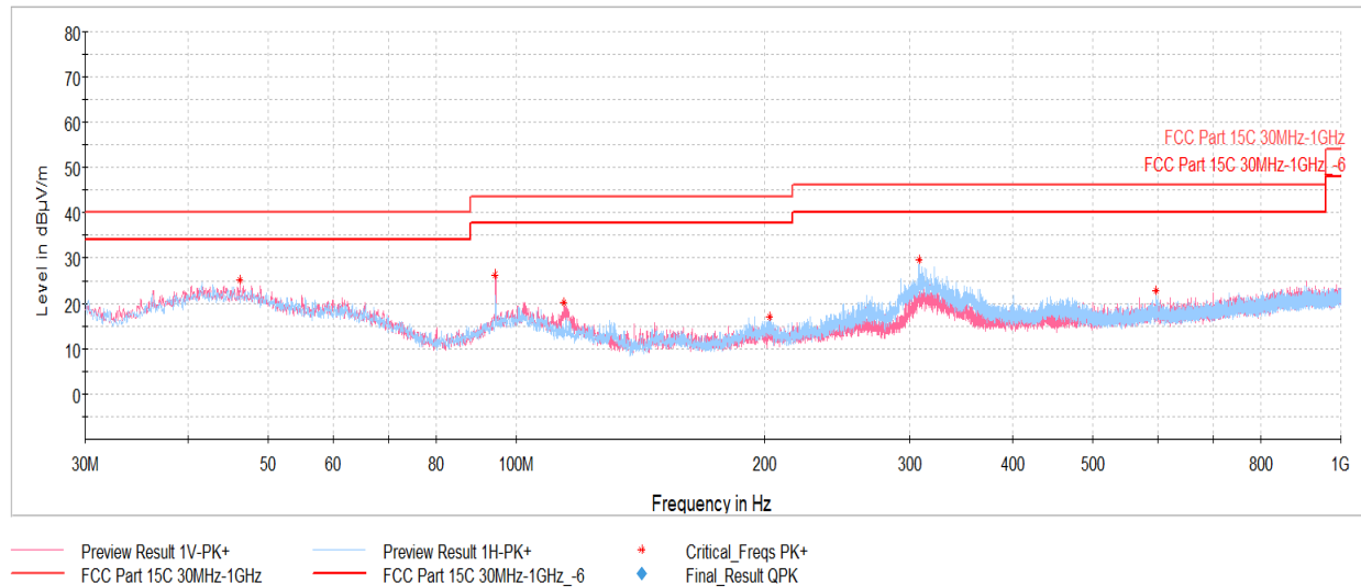
Plot 7-38. Radiated Spurious Emissions Below 1GHz (GFSK – Ch.39, with host PC and USB-C Cable)
