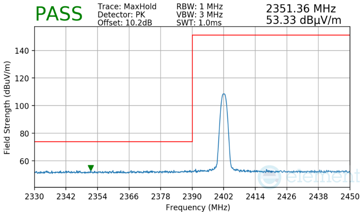
Plot 7-34. Radiated Restricted Lower Band Edge Measurement
