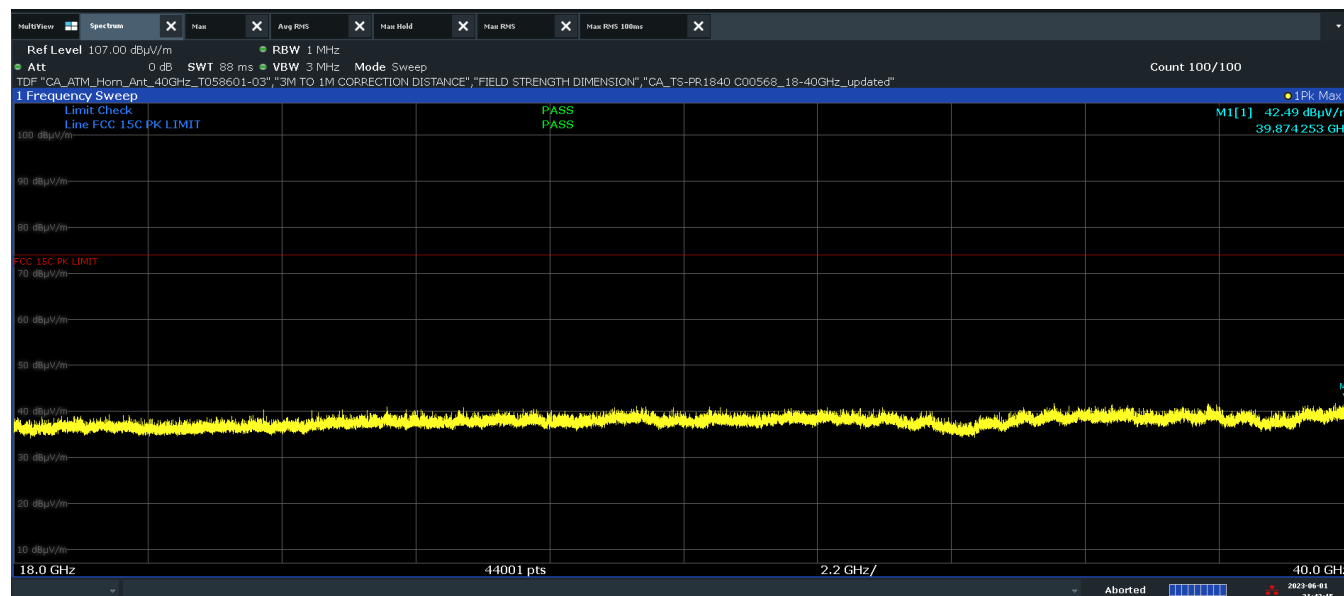
Plot 7-33. Radiated Spurious Emissions above 18GHz (BT GFSK – Ch. 78, Pol V)
