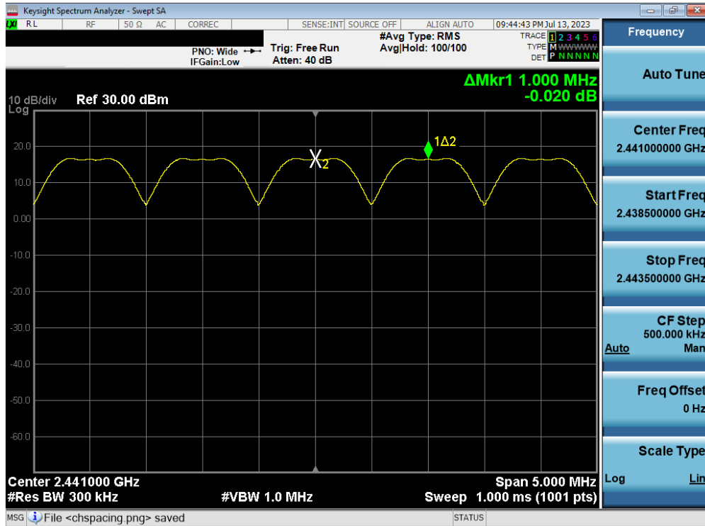
Plot 7-15. Channel Spacing Plot (Bluetooth, GFSK)
