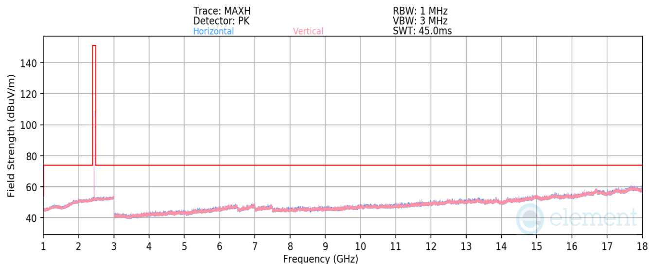
Plot 7-30. Radiated Spurious Emissions above 1GHz (BT GFSK – Ch. 39)
