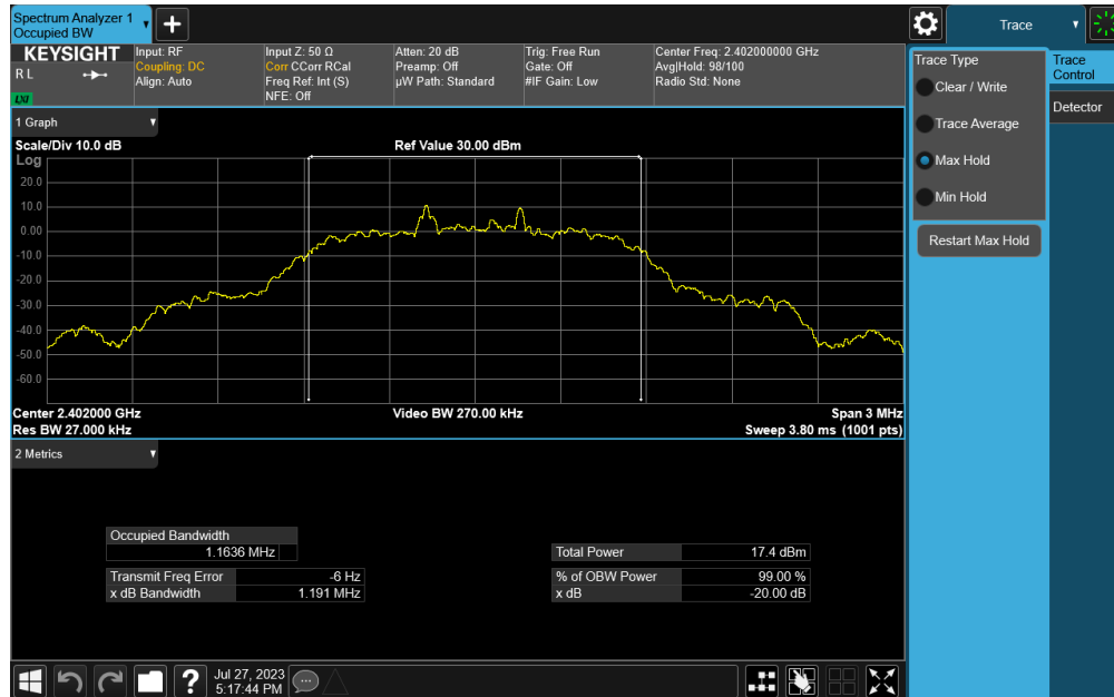
Plot 7-4. 20dB BW and 99% OBW Plot (Bluetooth, 8DPSK – Ch. 0)
