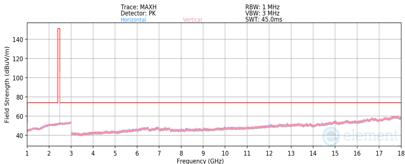
Plot 7-31. Radiated Spurious Emissions above 1GHz (BT GFSK – Ch. 78)
