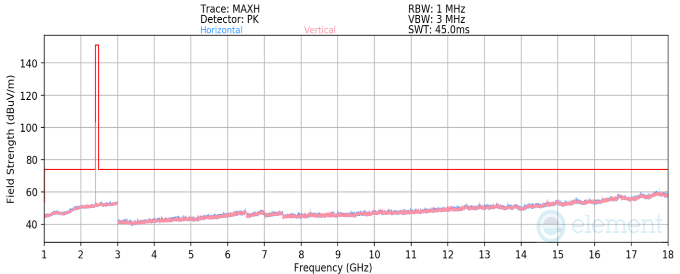
Plot 7-29. Radiated Spurious Emissions above 1GHz (BT GFSK – Ch. 0)
