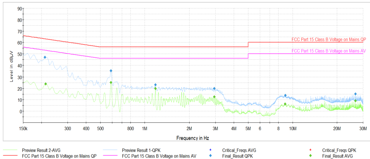
Plot 7-39. AC Line-Conducted Test Plot (L1, GFSK – Ch.39, with host PC and USB-C Cable)
