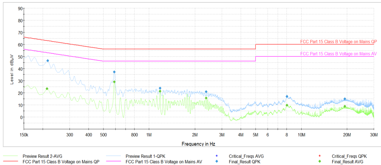
Plot 7-40. AC Line-Conducted Test Plot (N, GFSK – Ch.39, with host PC and USB-C Cable)
