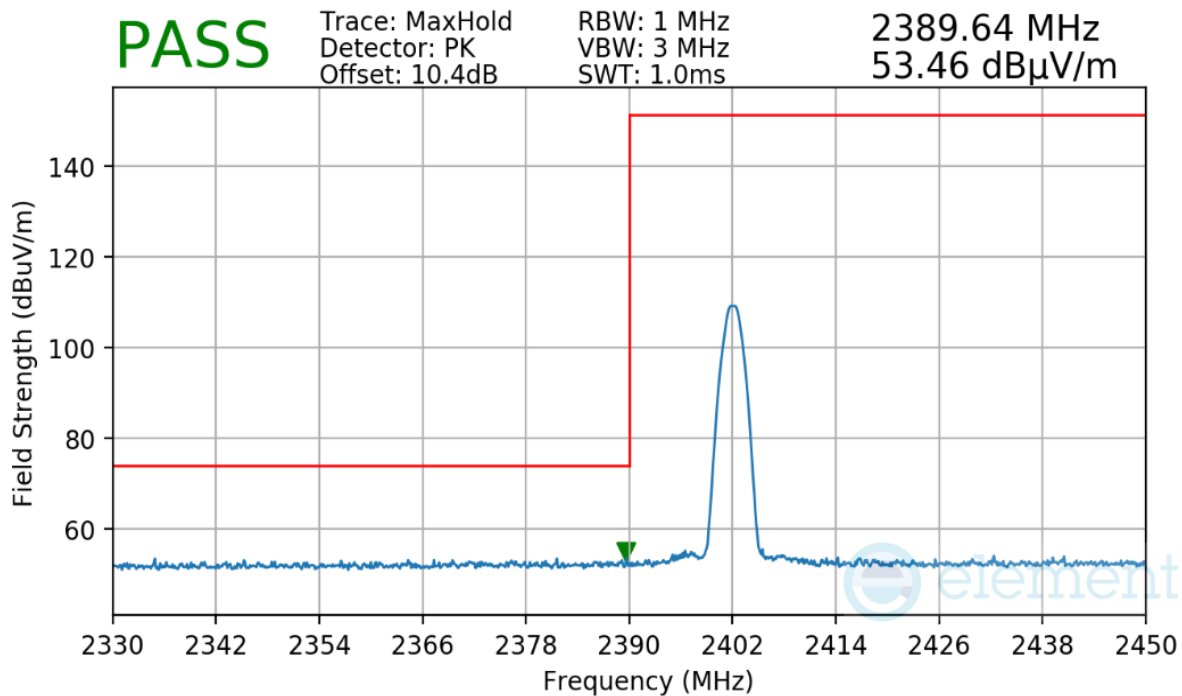
Plot 7-35. Radiated Restricted Lower Band Edge Measurement
