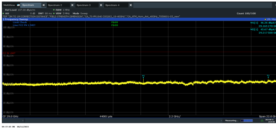
Plot 7-20. Radiated Spurious Emissions Above 18GHz (LE2M – 5844MHz Pol. V)
