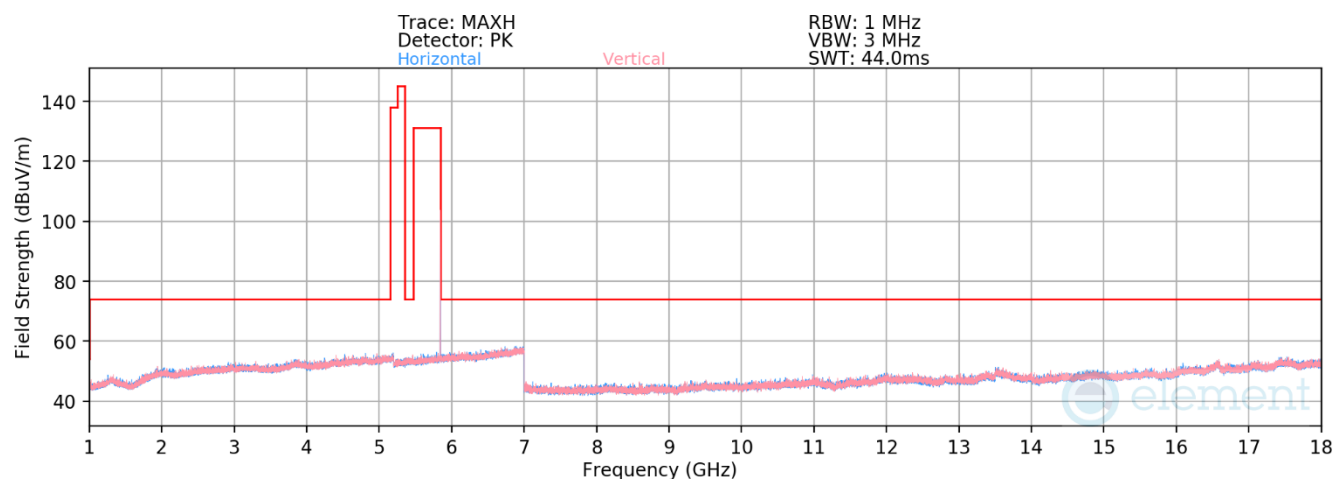
Plot 7-18. Radiated Spurious Emissions 1-18GHz (LE2M – 5844MHz)
