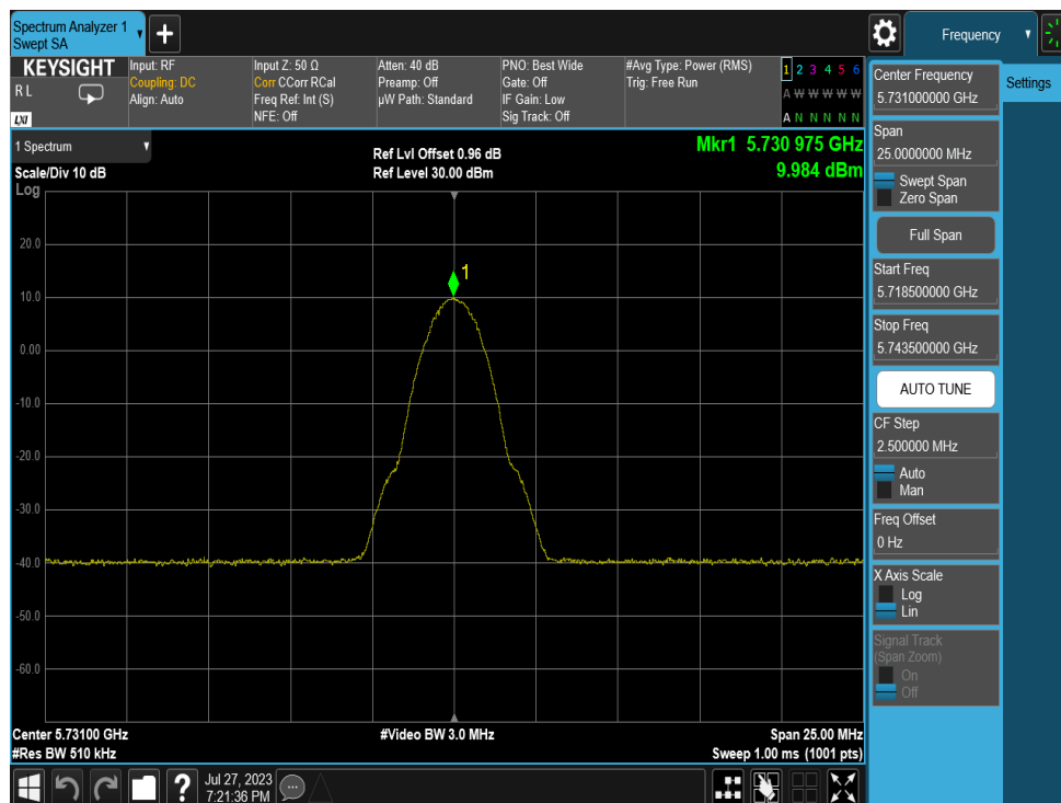
Plot 7-10. PSD (LE2M, 5731MHz)
