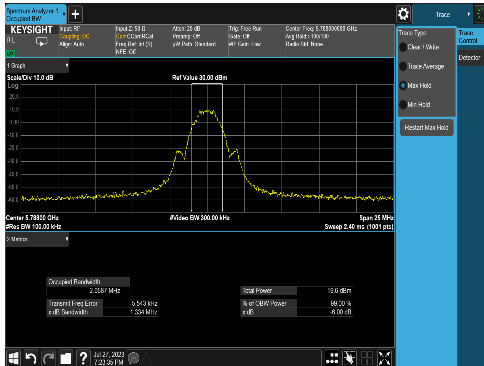
Plot 7-5. 6dB BW & 99% OBW (LE2M, 5788MHz)
