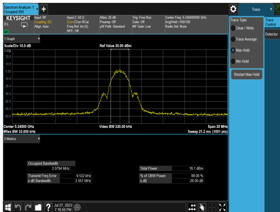
Plot 7-3. 26dB BW & 99% OBW (LE2M, 5245MHz)
