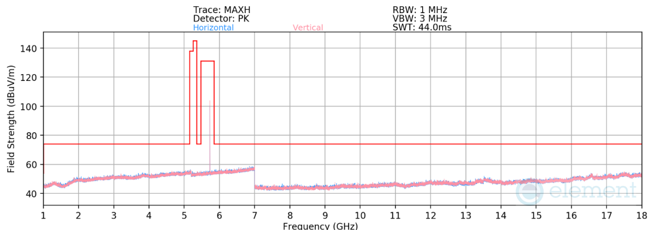
Plot 7-16. Radiated Spurious Emissions 1-18GHz (LE2M – 5731MHz)
