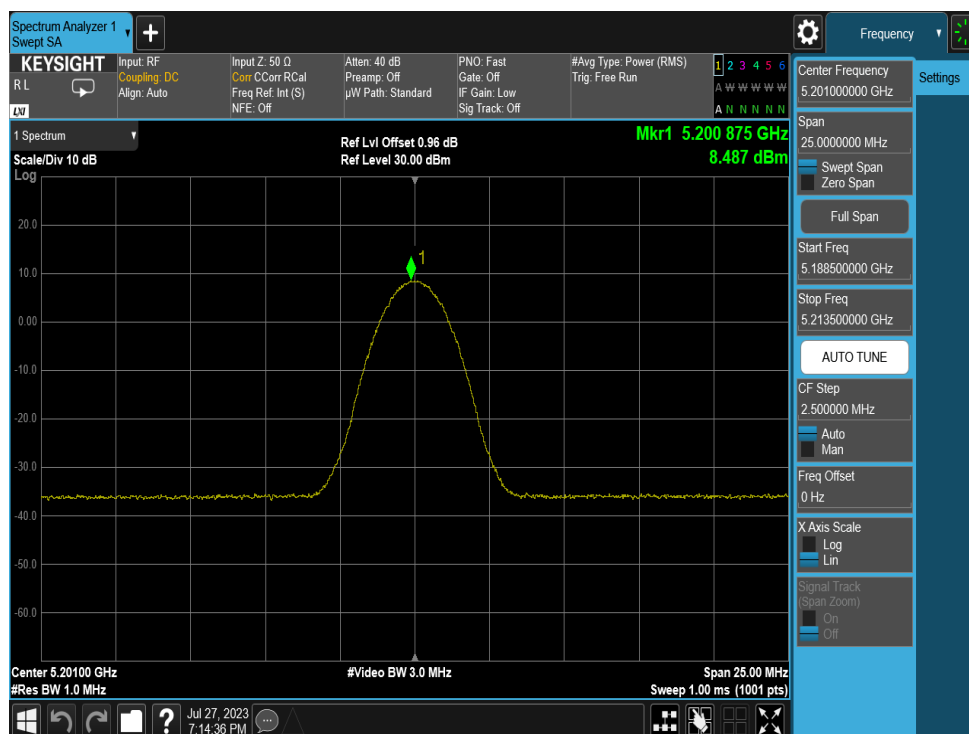
Plot 7-8. PSD (LE2M, 5201MHz)
