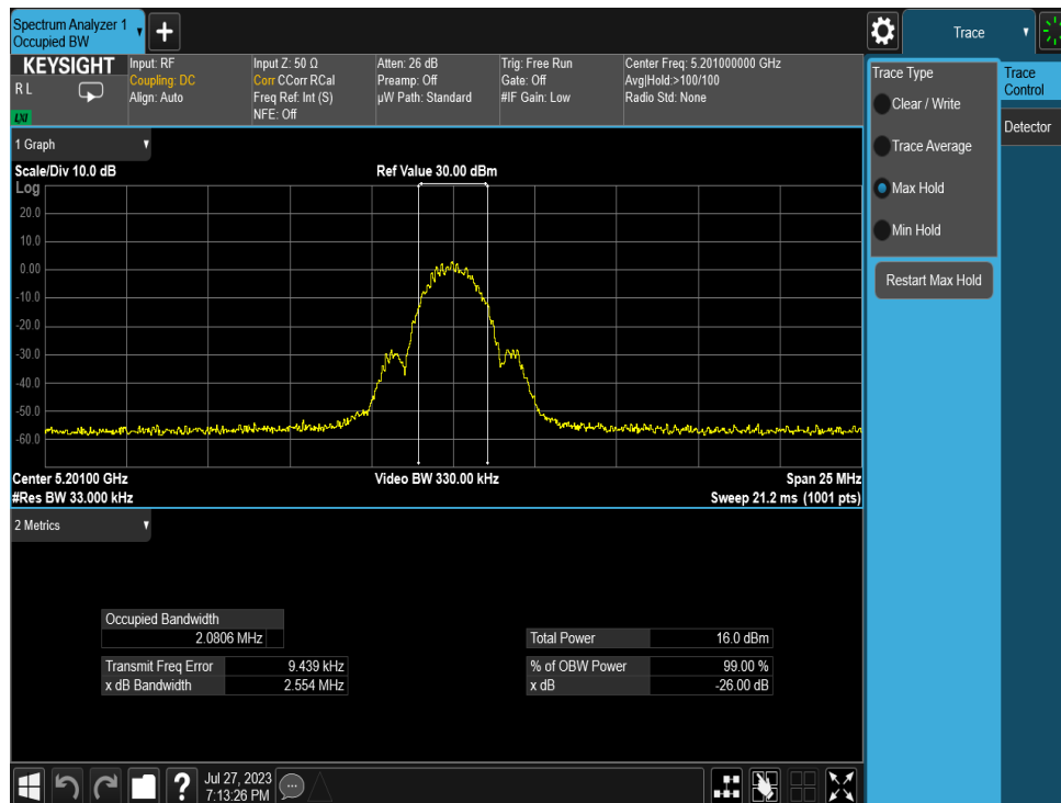
Plot 7-2. 26dB BW & 99% OBW (LE2M, 5201MHz)
