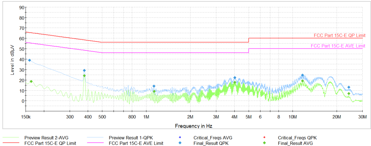
Plot 7-25. AC Line Conducted Plot (LE2M – 5844MHz) (L1) by host PC and USB-C cable
