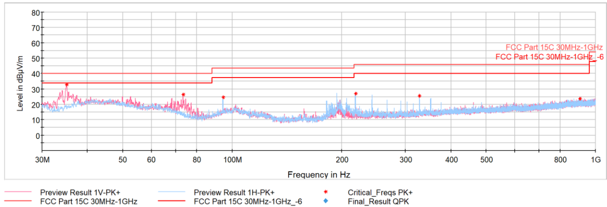
Plot 7-24. RSE 30MHz - 1GHz (LE2M – 5844MHz), with AC/DC Adapter and USB-C cable
