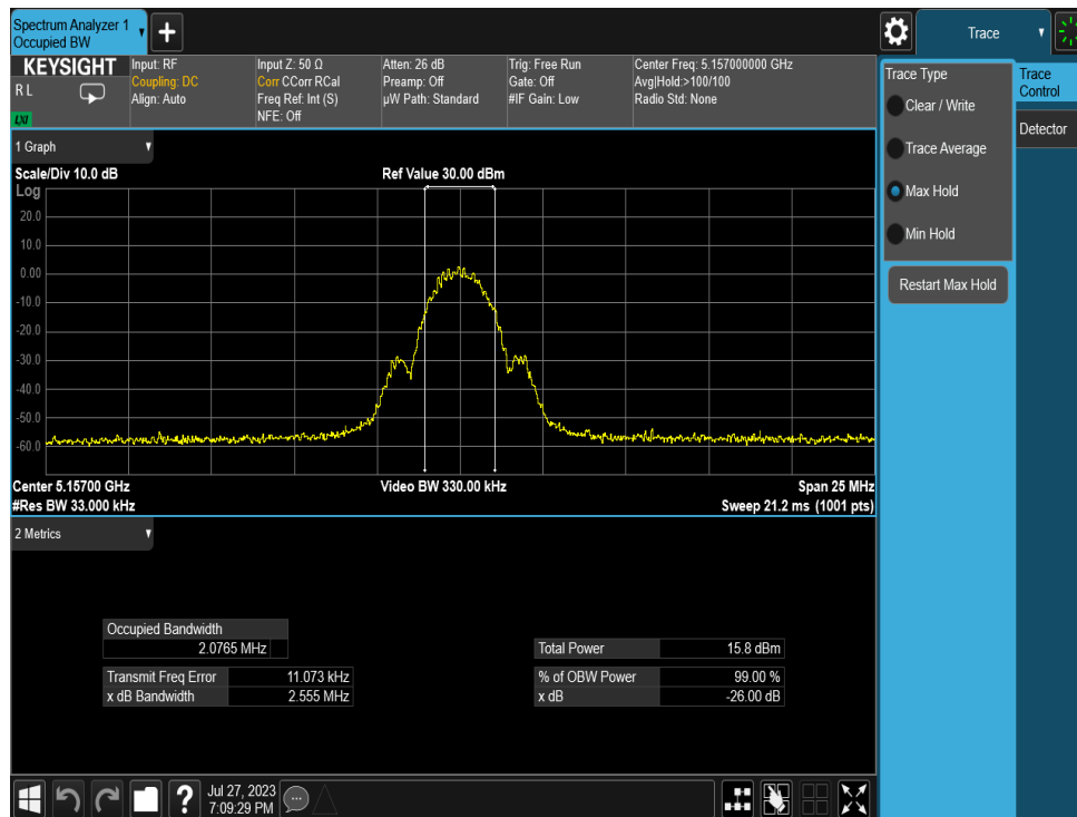
Plot 7-1. 26dB BW & 99% OBW (LE2M, 5157MHz)
