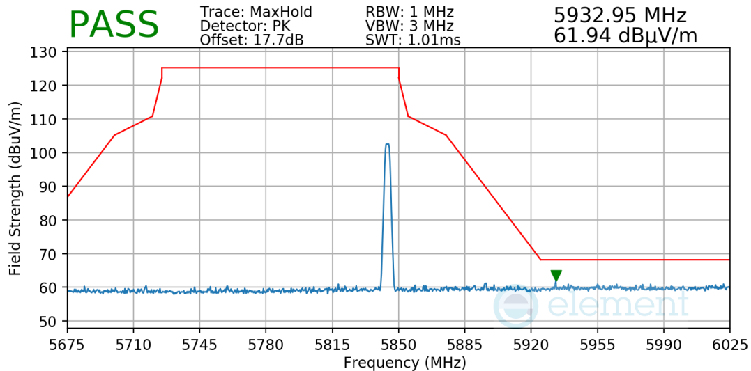
Plot 7-23. Radiated Upper Band Edge Measurement
