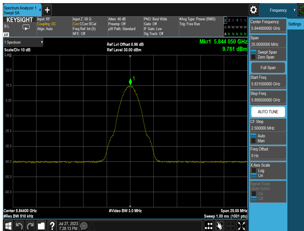
Plot 7-12. PSD (LE2M, 5844MHz)
