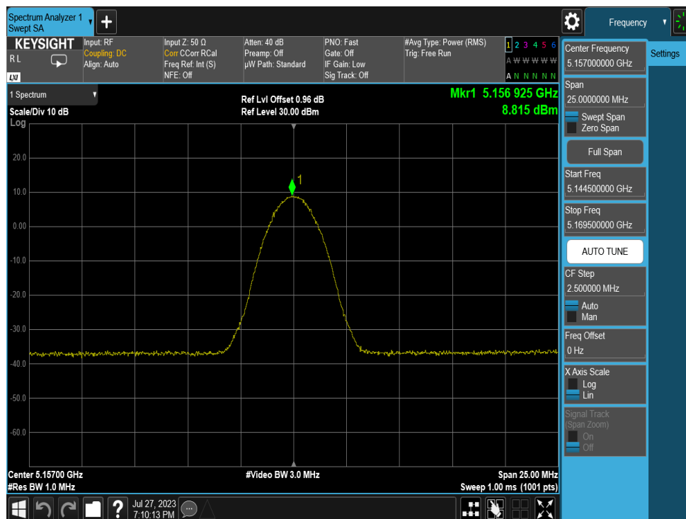
Plot 7-7. PSD (LE2M, 5157MHz)
