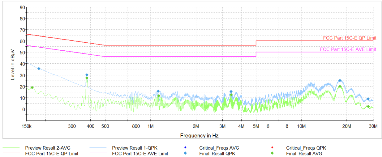
Plot 7-27. AC Line Conducted Plot (LE2M – 5844MHz) (N) by host PC and USB-C cable
