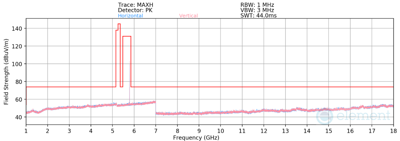
Plot 7-17. Radiated Spurious Emissions 1-18GHz (LE2M – 5788MHz)
