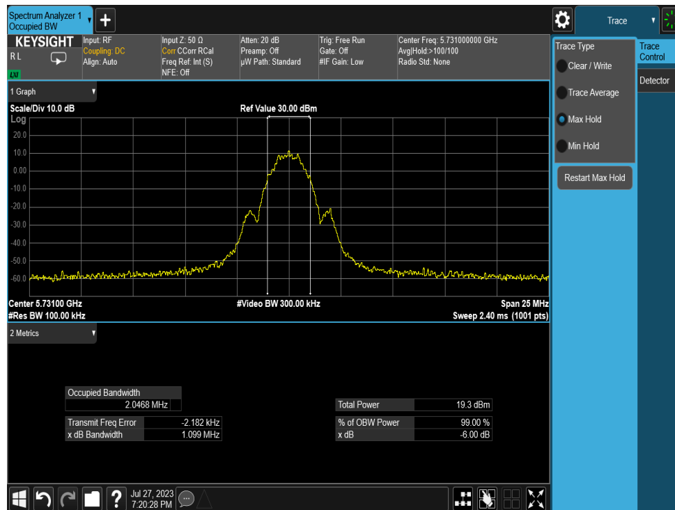
Plot 7-4. 6dB BW & 99% OBW (LE2M, 5731MHz)
