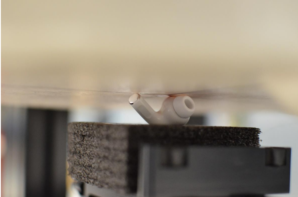
SAR Test Setup Photo 1: Head, Left Earbud, 0 mm
