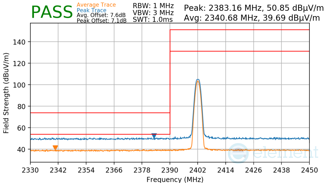
Plot 7-27. Radiated Restricted Lower Band Edge Measurement (Average & Peak)
