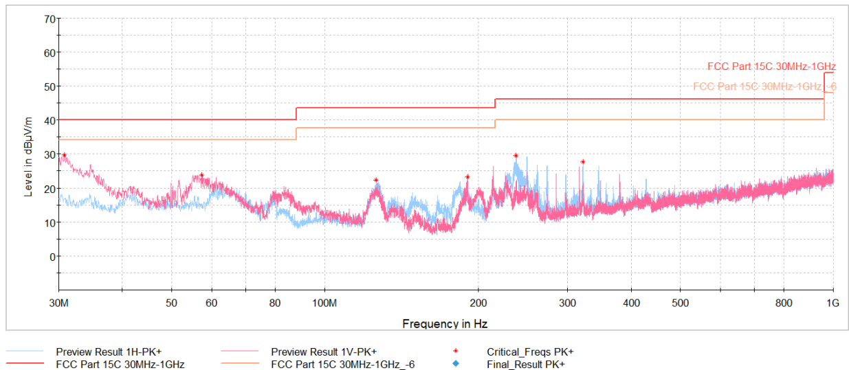
Plot 7-31. Radiated Spurious Emissions Below 1GHz (1Mbps, – Ch.19, Pol. H & V, host PC with USB-C cable)
