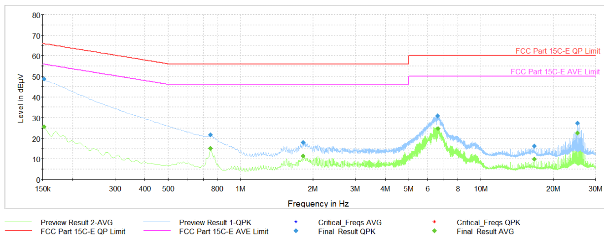
Plot 7-33. AC Line Conducted Plot with Bluetooth LE (N, 1Mbps – Ch.19, host PC with USB-C cable)
