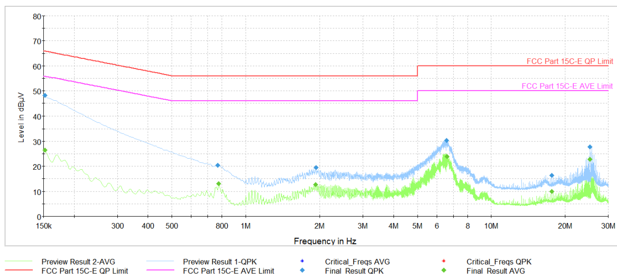
Plot 7-32. AC Line Conducted Plot with Bluetooth LE (L1, 1Mbps – Ch.19, host PC with USB-C cable)
