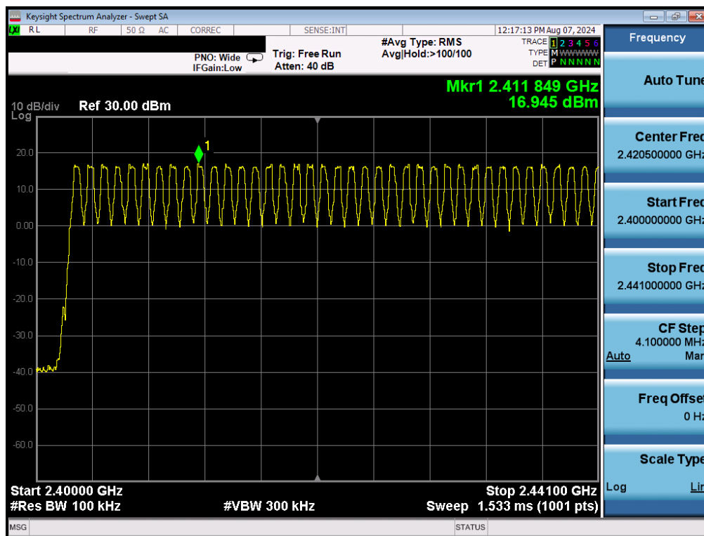
Plot 7-19. Low End Spectrum Channel Hopping Plot (Bluetooth, GFSK)
