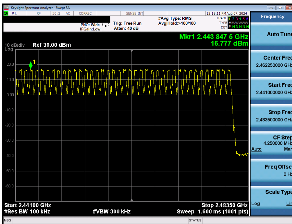
Plot 7-20. High End Spectrum Channel Hopping Plot (Bluetooth, GFSK)
