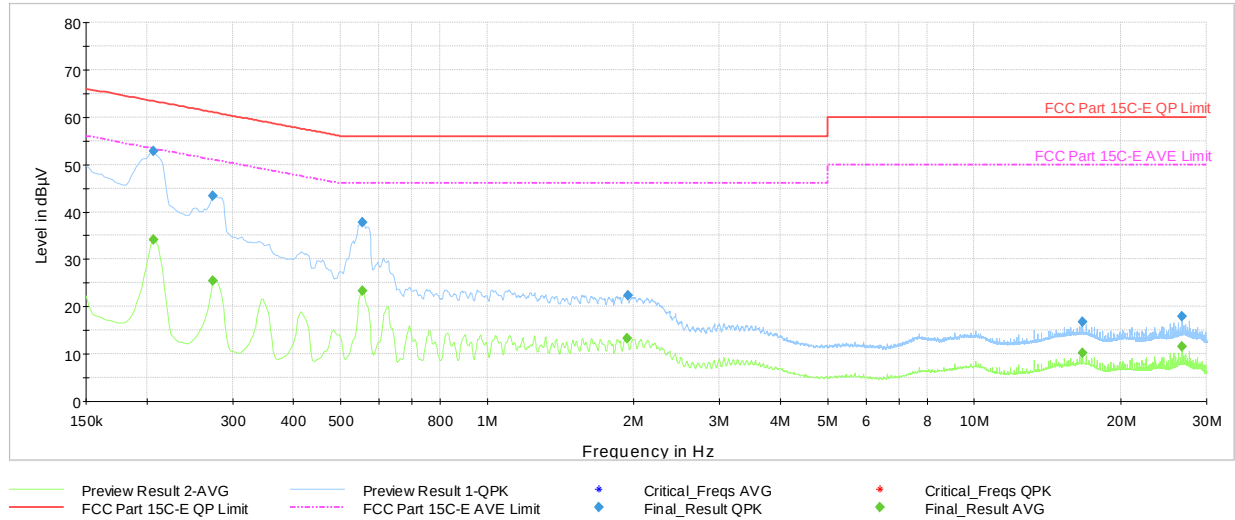
Plot 7-39. AC Line-Conducted Test Plot (N, GFSK – Ch.78, with host PC with USB-C cable)
