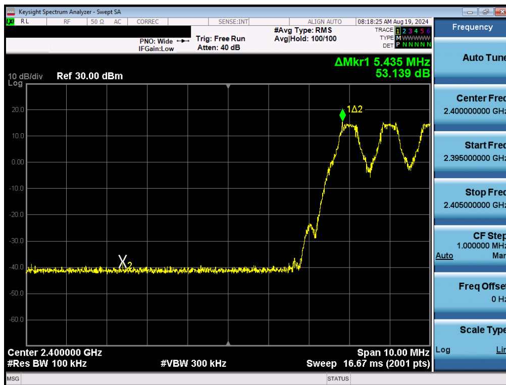
Plot 7-9. Band Edge Plot (Bluetooth with Hopping Enabled, GFSK)
