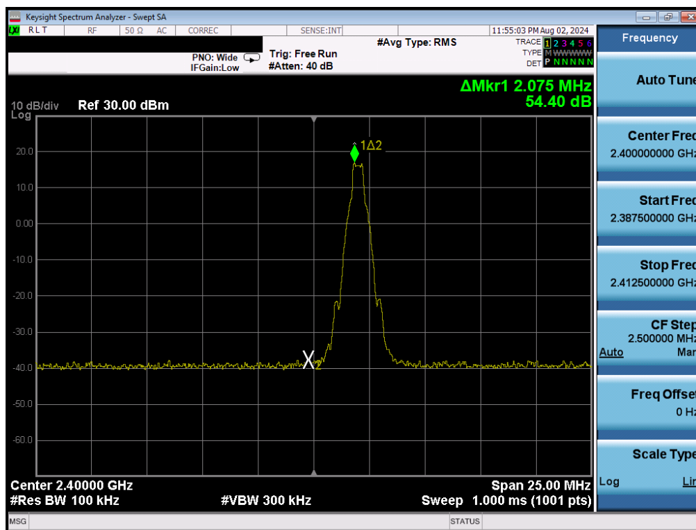
Plot 7-7. Band Edge Plot (Bluetooth with Hopping Disabled, GFSK – Ch. 0)
