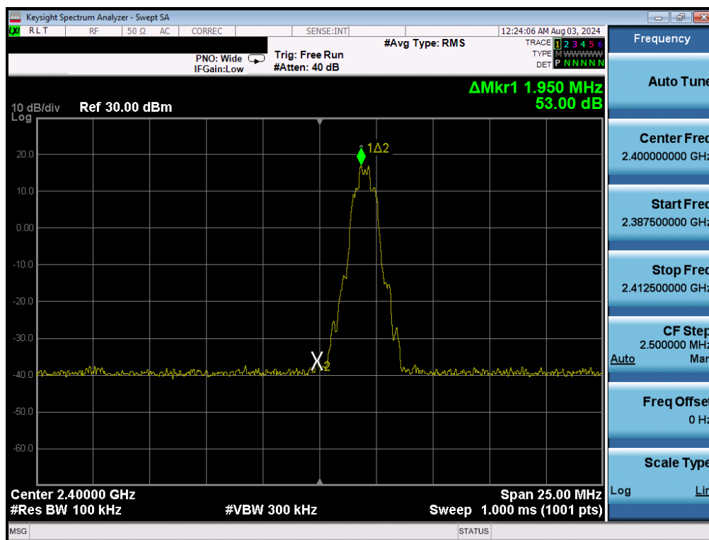
Plot 7-11. Band Edge Plot (Bluetooth with Hopping Disabled, 8DPSK – Ch. 0)
