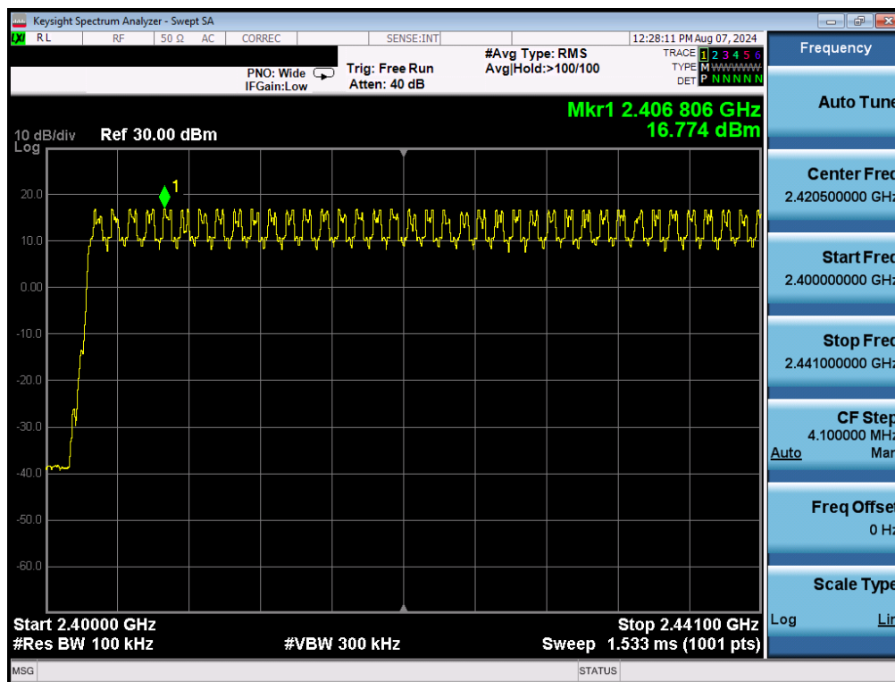
Plot 7-21. Low End Spectrum Channel Hopping Plot (Bluetooth, 8DPSK)
