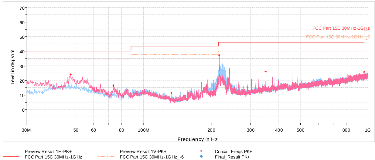
Plot 7-37. Radiated Spurious Emissions Below 1GHz (GFSK – Ch.78, with AC/DC Adapter & USB-C Cable)
