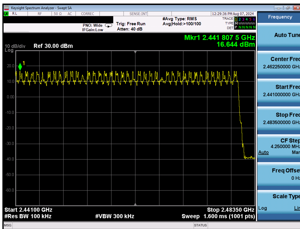
Plot 7-22. High End Spectrum Channel Hopping Plot (Bluetooth, 8DPSK)
