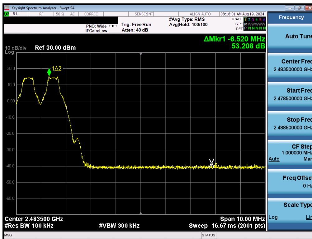
Plot 7-10. Band Edge Plot (Bluetooth with Hopping Enabled, GFSK)
