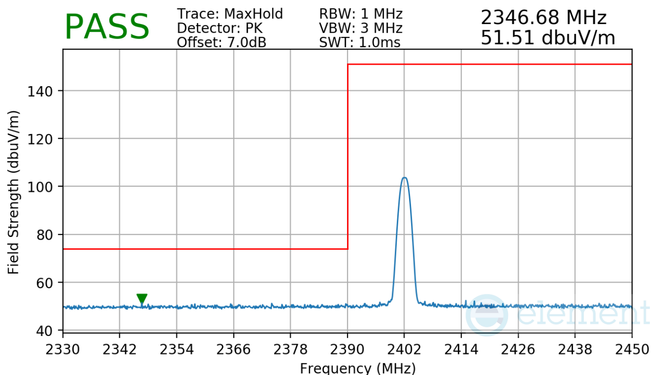
Plot 7-33. Radiated Restricted Lower Band Edge Measurement
