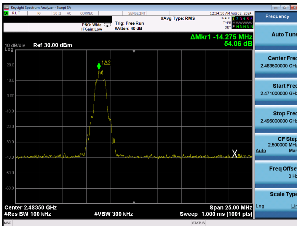
Plot 7-12. Band Edge Plot (Bluetooth with Hopping Disabled, 8DPSK – Ch. 78)
