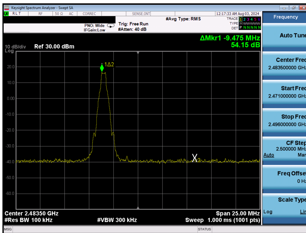
Plot 7-8. Band Edge Plot (Bluetooth with Hopping Disabled, GFSK – Ch. 78)
