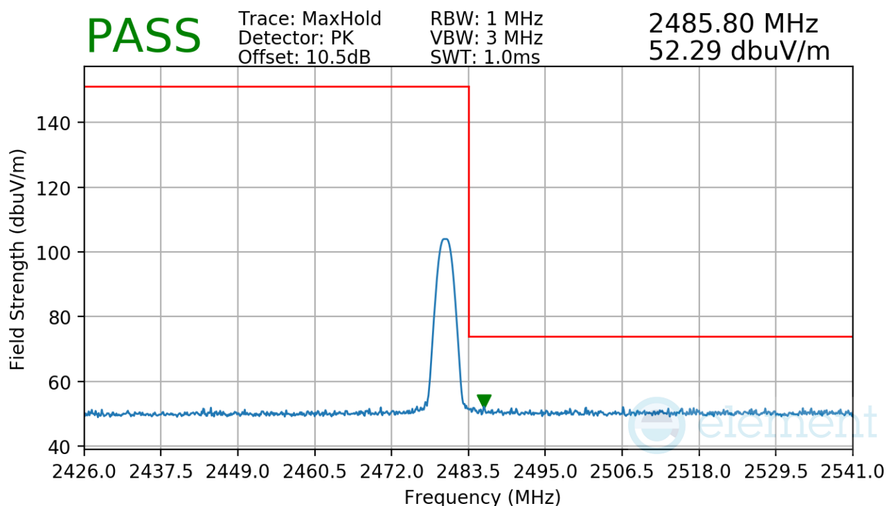
Plot 7-35. Radiated Restricted Upper Band Edge Measurement
