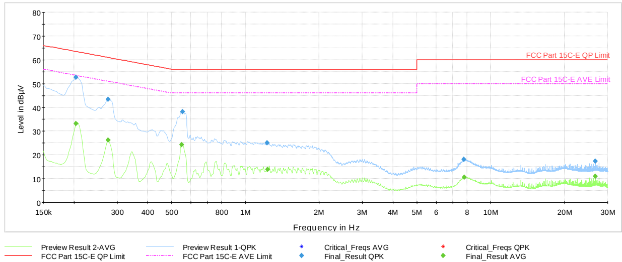
Plot 7-38. AC Line-Conducted Test Plot (L1, GFSK – Ch.78, with host PC with USB-C cable)
