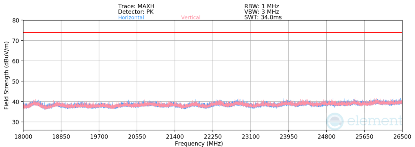
Plot 7-32. Radiated Spurious Emissions above 18GHz (BT GFSK – Ch. 78)
