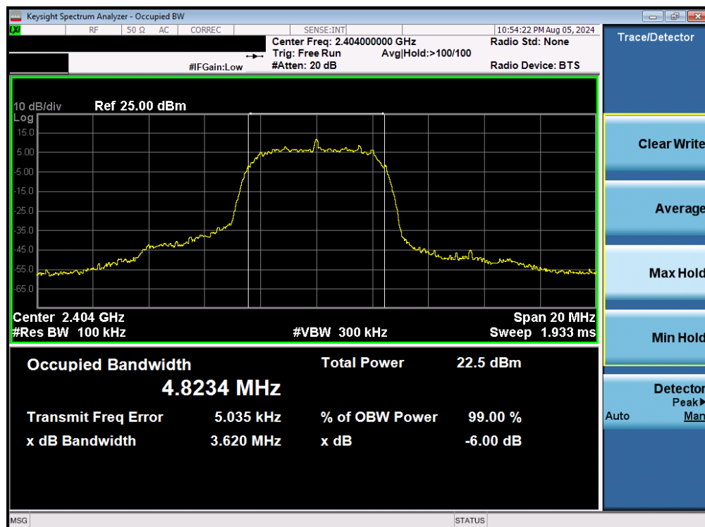
Plot 7-10. 6dB BW & 99% OBW Plot (Bluetooth (HDRp8), 8Mbps, – Ch. 1)
