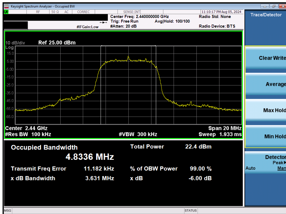
Plot 7-11. 6dB BW & 99% OBW Plot (Bluetooth (HDRp8), 8Mbps, – Ch. 37)
