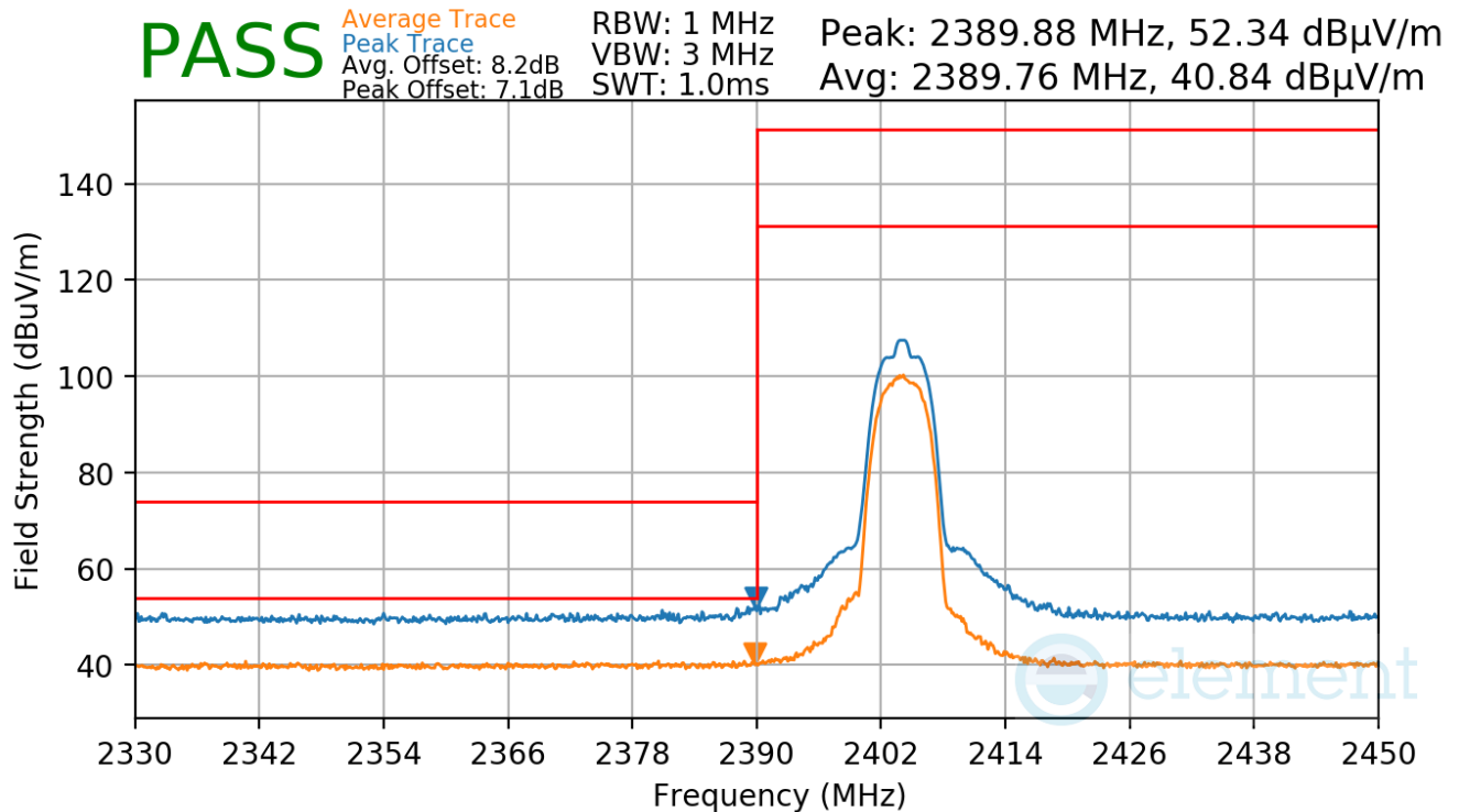
Plot 7-44. Radiated Restricted Lower Band Edge Measurement
