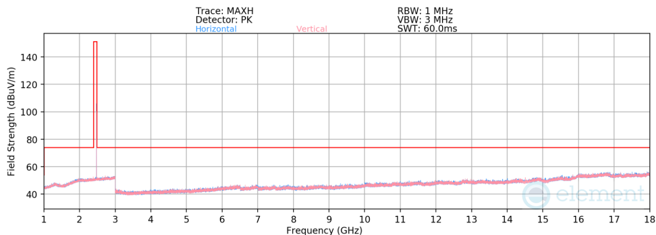
Plot 7-42. Radiated Spurious Emissions 1-18GHz (4Mbps, HDR4, - Ch. 73)
