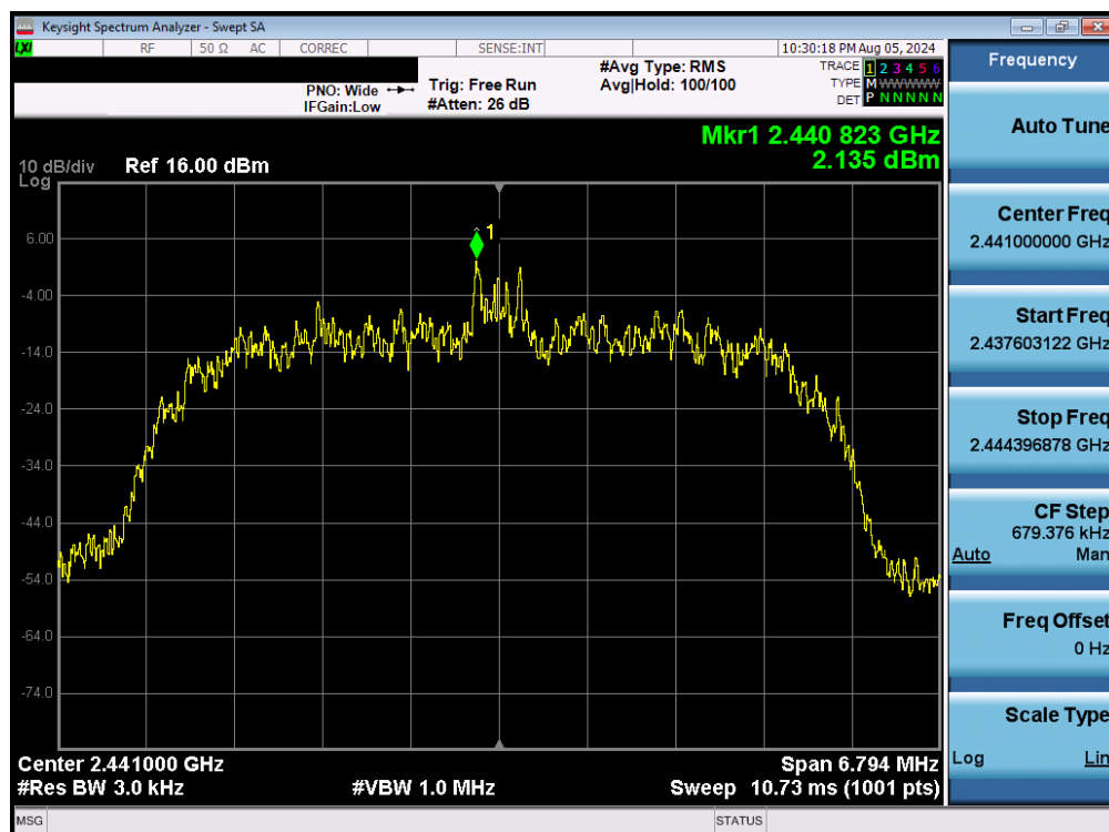
Plot 7-17. Power Spectral Density Plot (Bluetooth (HDR8), 8Mbps, – Ch. 38)
