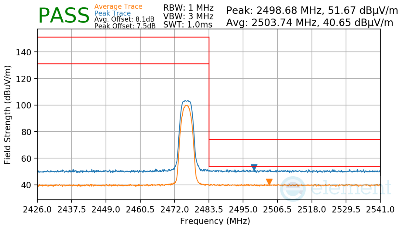
Plot 7-49. Radiated Restricted Upper Band Edge Measurement
