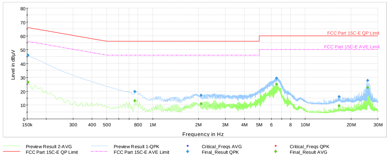
Plot 7-52. AC Line Conducted Plot with Bluetooth HDR (L1, 4Mbps - Ch.38 with host PC and USB-C cable)
