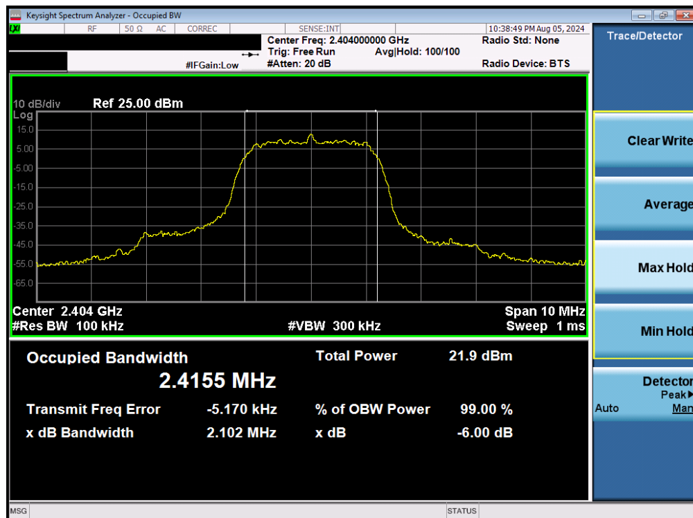
Plot 7-7. 6dB BW & 99% OBW Plot (Bluetooth (HDRp4), 4Mbps, – Ch. 1)
