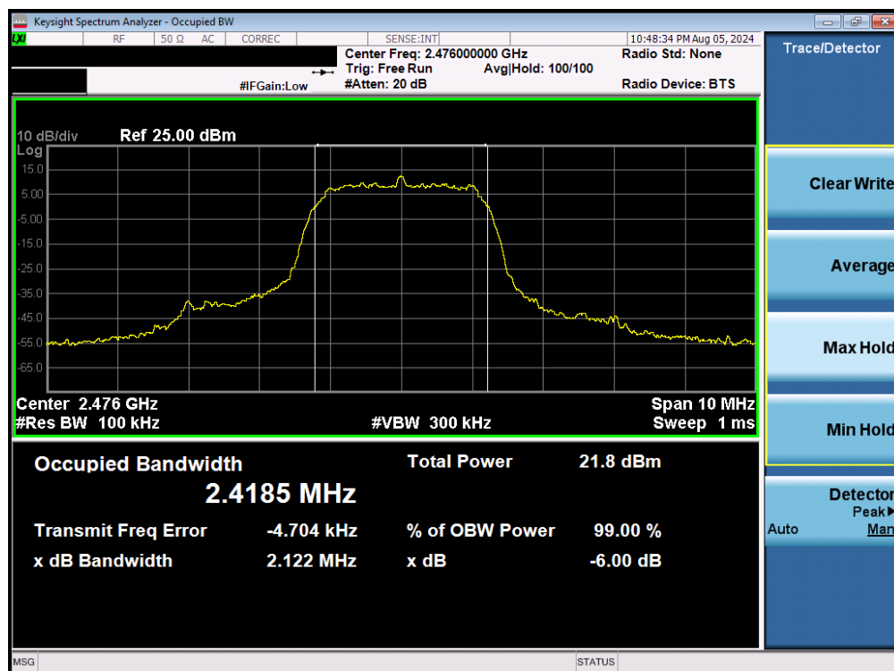
Plot 7-9. 6dB BW & 99% OBW Plot (Bluetooth (HDRp4), 4Mbps, – Ch. 73)
