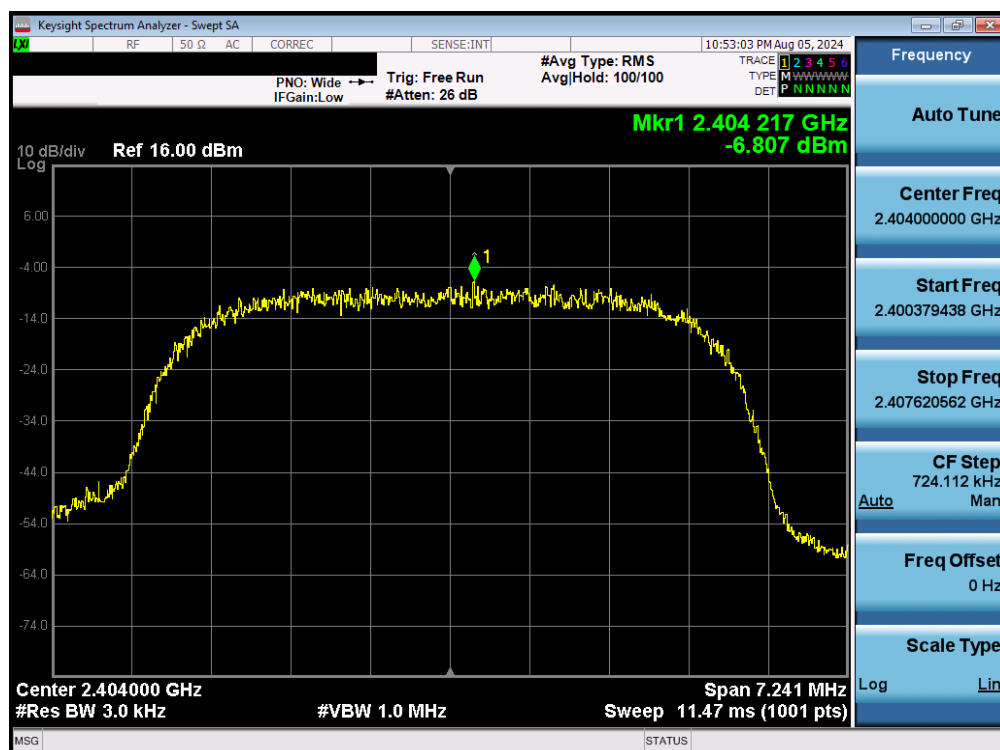
Plot 7-22. Power Spectral Density Plot (Bluetooth (HDRp8), 8Mbps, – Ch. 1)
