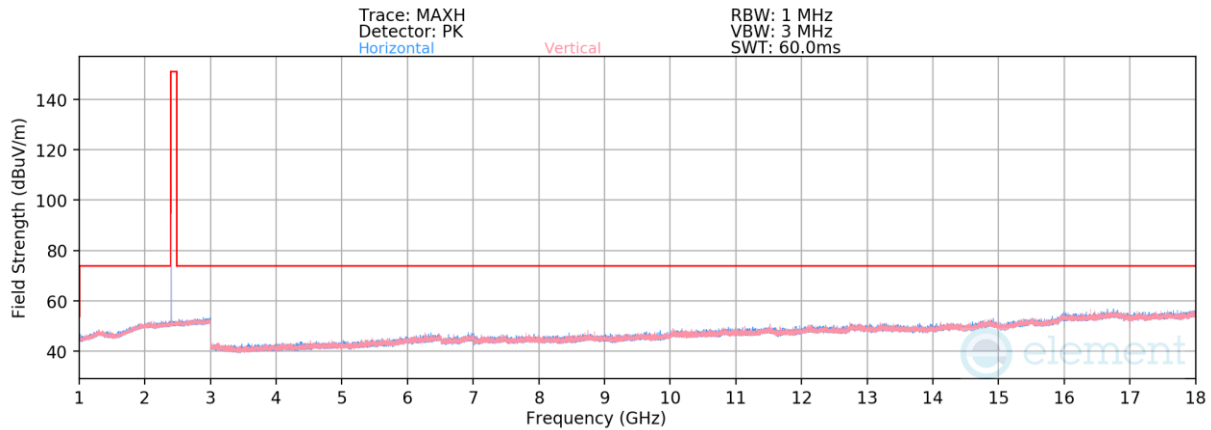
Plot 7-39. Radiated Spurious Emissions 1-18GHz (4Mbps, HDR4, – Ch. 1)
