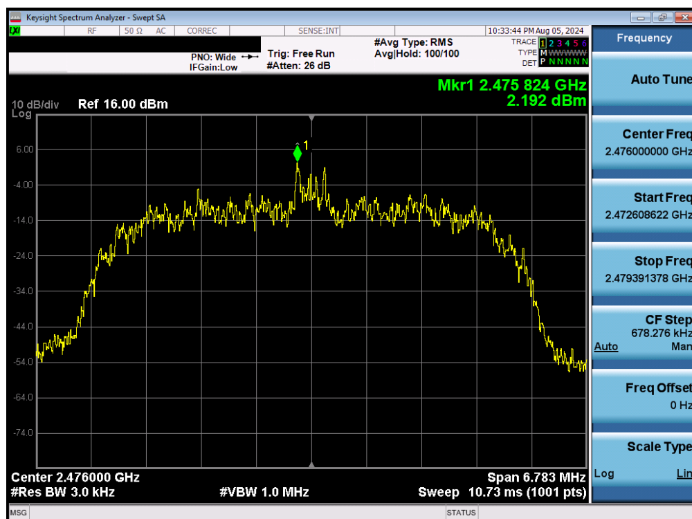
Plot 7-18. Power Spectral Density Plot (Bluetooth (HDR8), 8Mbps, – Ch. 73)
