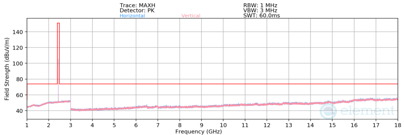
Plot 7-40. Radiated Spurious Emissions 1-18GHz (4Mbps, HDR4, – Ch. 38)
