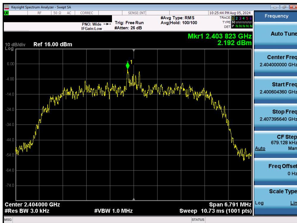
Plot 7-16. Power Spectral Density Plot (Bluetooth (HDR8), 8Mbps, – Ch. 1)
