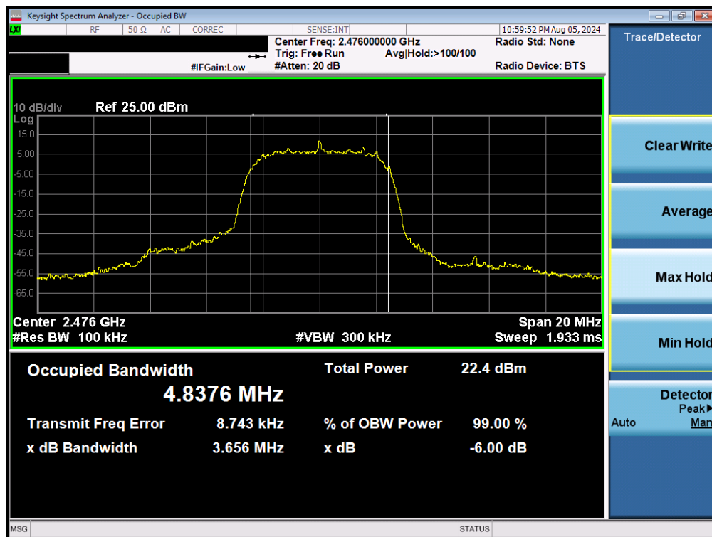
Plot 7-12. 6dB BW & 99% OBW Plot (Bluetooth (HDRp8), 8Mbps, – Ch. 73)
