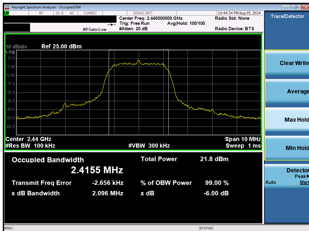
Plot 7-8. 6dB BW & 99% OBW Plot Bluetooth (HDRp4), 4Mbps, – Ch. 37)
