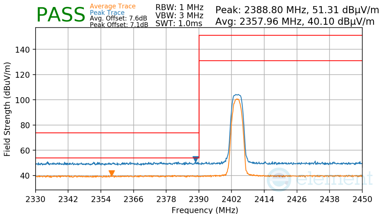
Plot 7-45. Radiated Restricted Lower Band Edge Measurement
