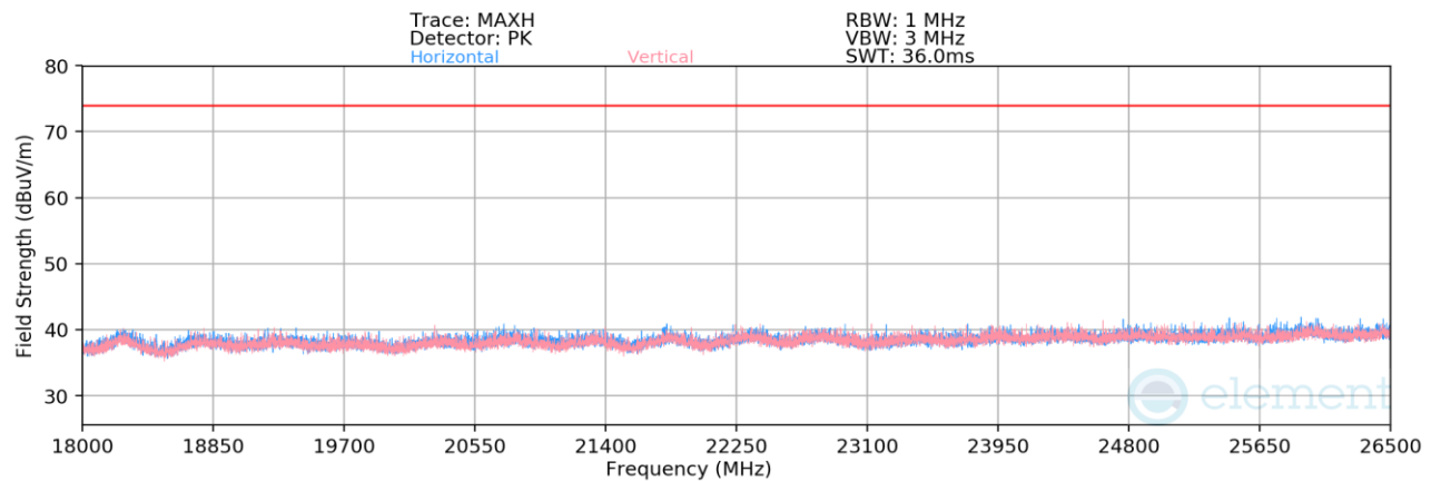
Plot 7-41. Radiated Spurious Emissions Above 18GHz (4Mbps, HDR4, – Ch. 38)
