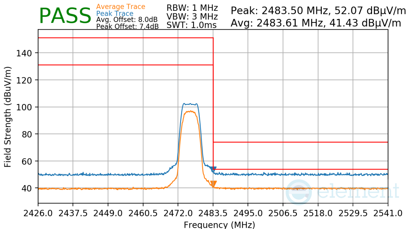
Plot 7-50. Radiated Restricted Upper Band Edge Measurement
