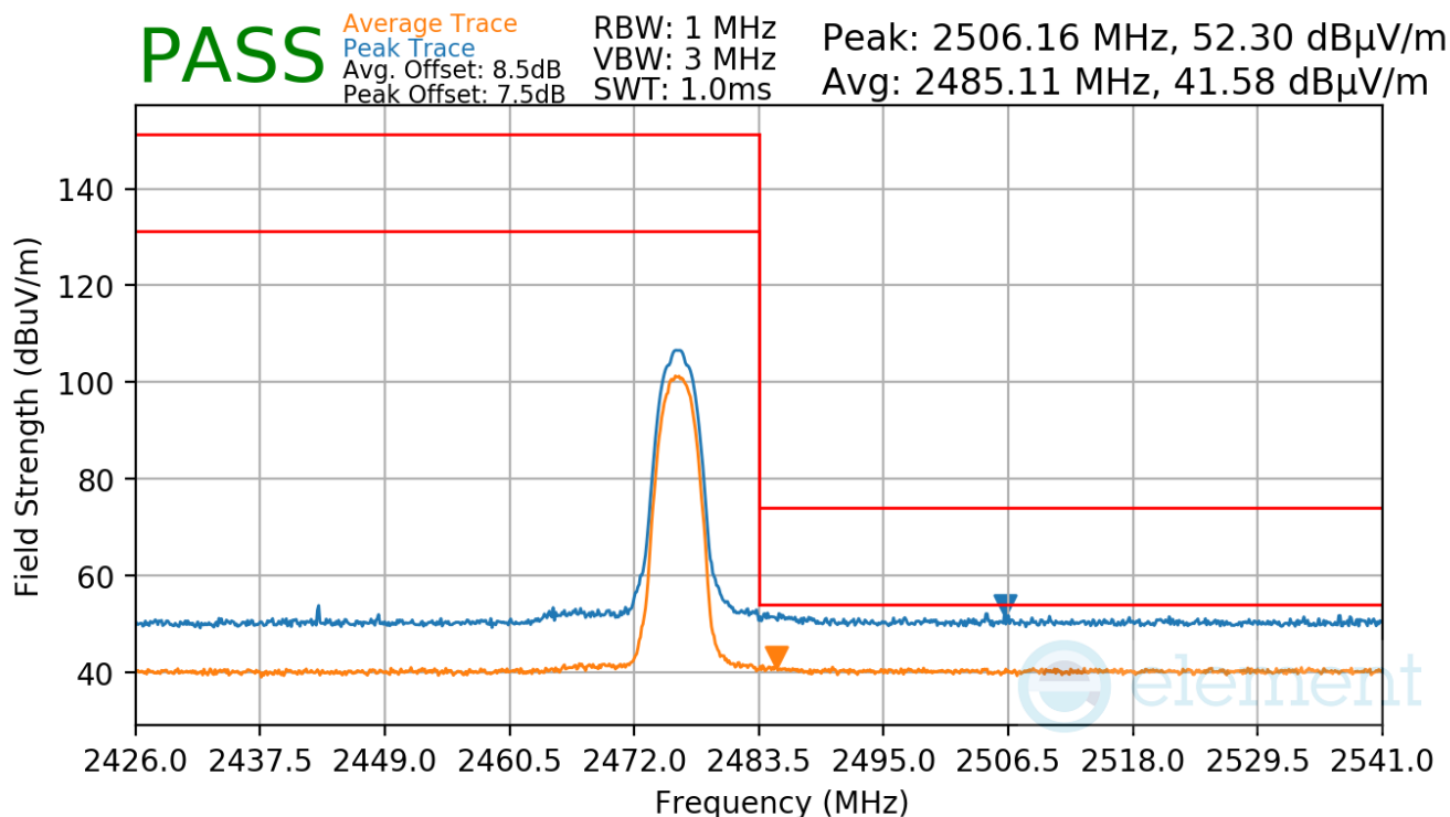
Plot 7-47. Radiated Restricted Upper Band Edge Measurement
