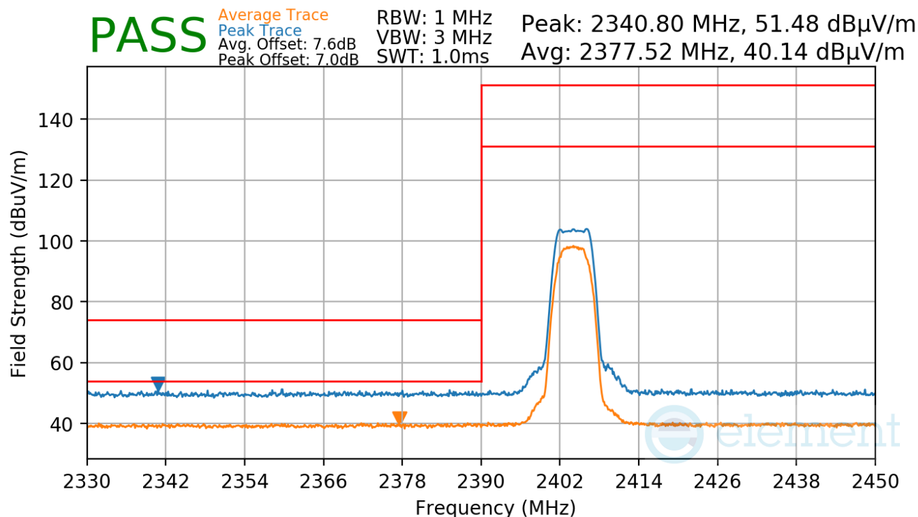
Plot 7-46. Radiated Restricted Lower Band Edge Measurement
