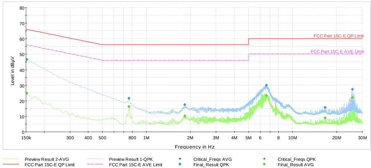
Plot 7-53. AC Line Conducted Plot with Bluetooth HDR (N, 4Mbps - Ch.38 with host PC and USB-C cable)
