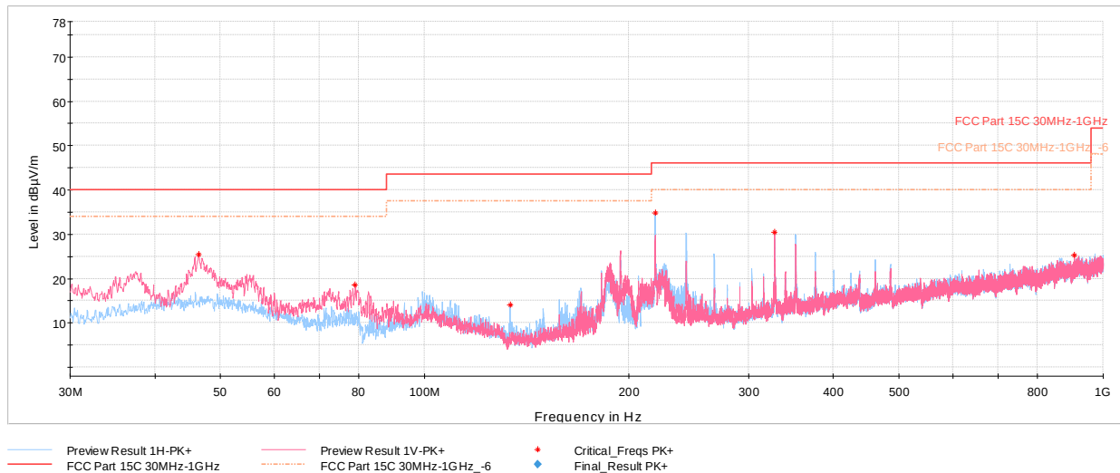
Plot 7-51. Radiated Spurious Emissions Below 1GHz (4Mbps, – Ch.38 with AC/DC Adapter and USB-C cable)
