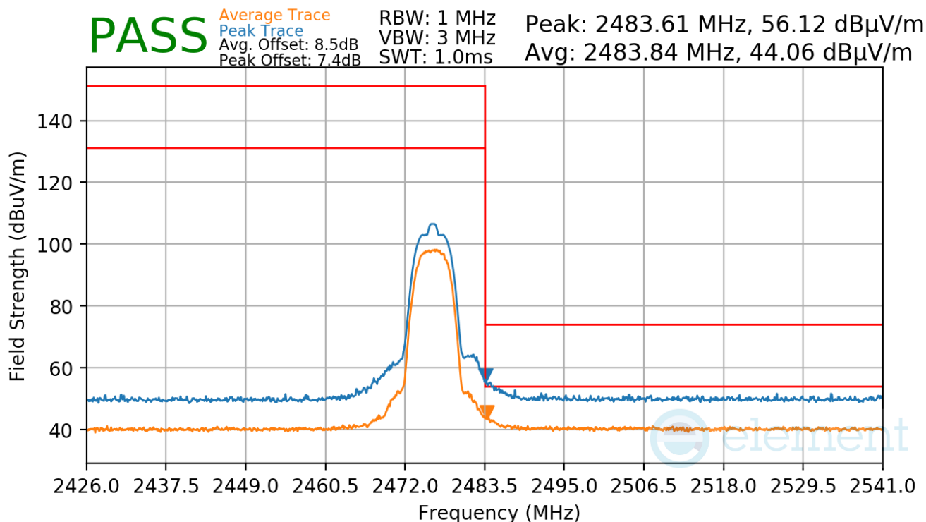
Plot 7-48. Radiated Restricted Upper Band Edge Measurement
