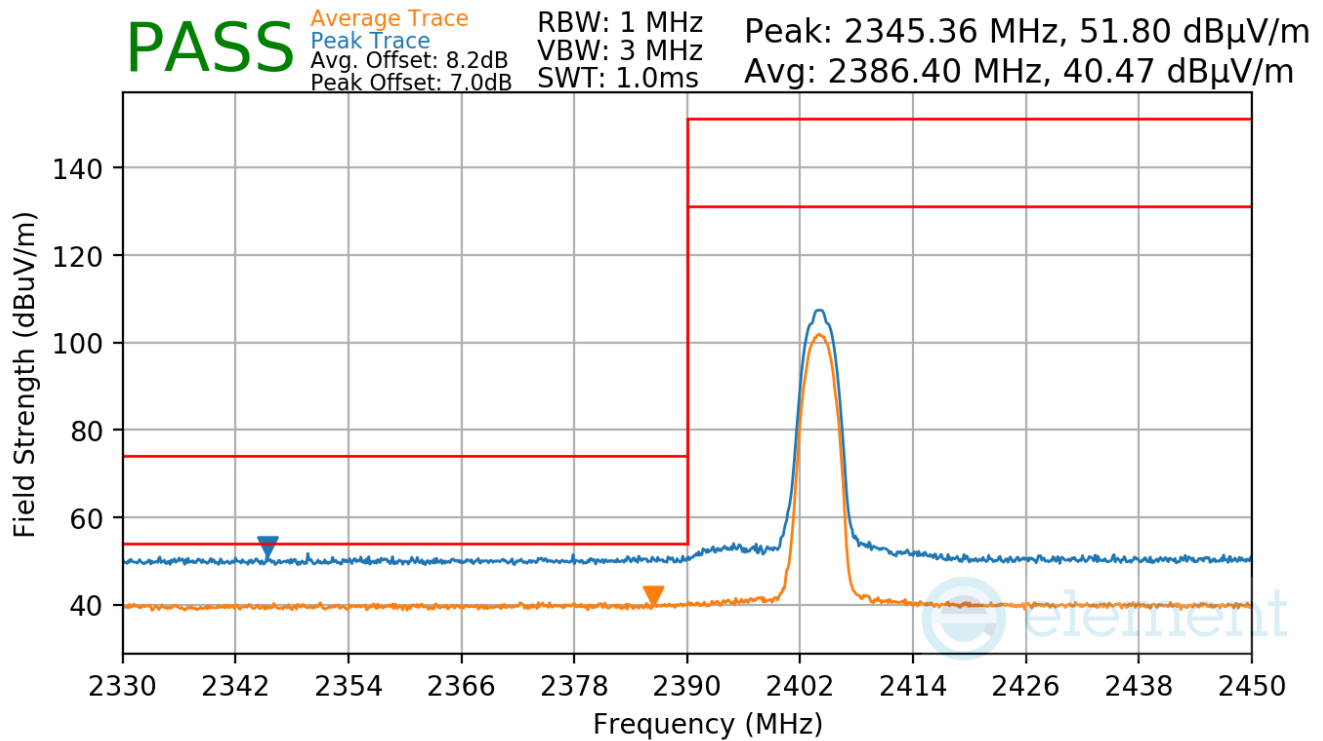
Plot 7-43. Radiated Restricted Lower Band Edge Measurement
