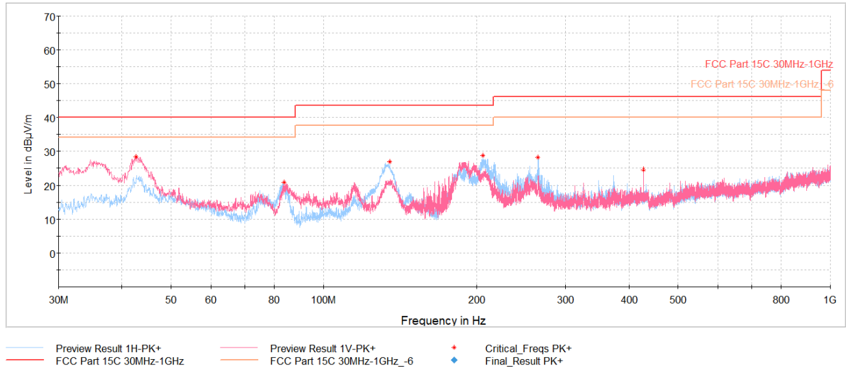
Plot 7-31. Radiated Spurious Emissions Below 1GHz (1Mbps – Ch.19, Pol. H & V, with host PC and USB-C Cable)
