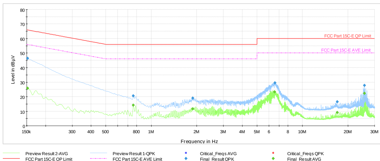
Plot 7-32. AC Line Conducted Plot with Bluetooth LE (L1, 1Mbps – Ch.19 with host PC and USB-C Cable)
