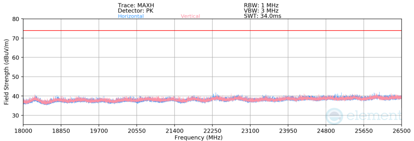
Plot 7-32. Radiated Spurious Emissions above 18GHz (BT GFSK – Ch. 78)
