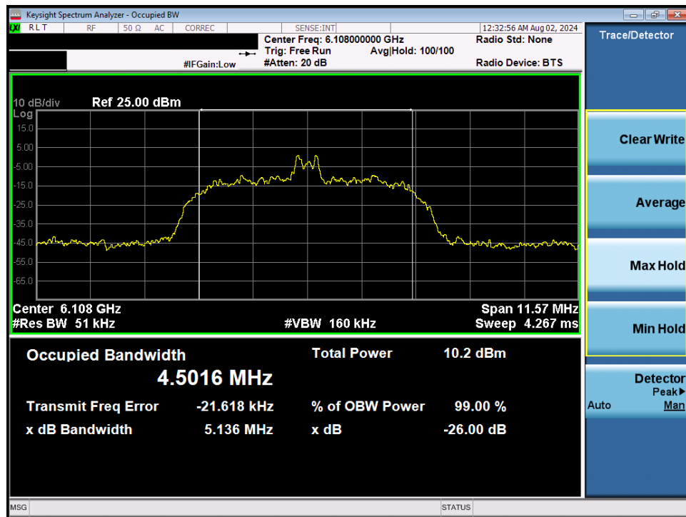
Plot 7-10. 26dB BW & 99% OBW (NB UNII HDR8 – 6108MHz)
