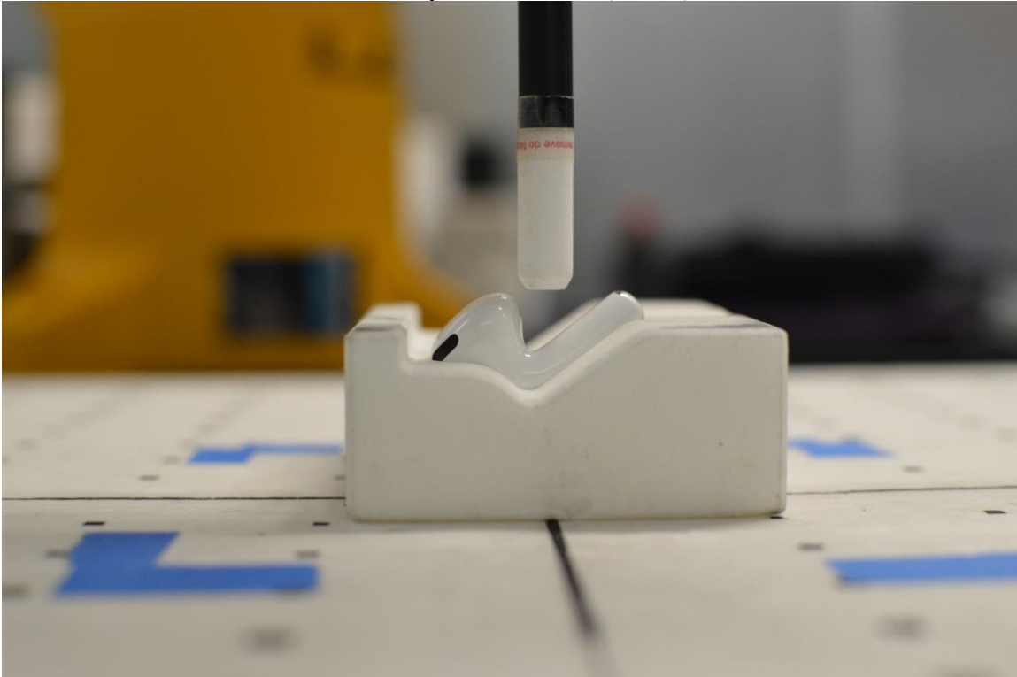
SAR Test Setup Photo 5: Head, Front, 2 mm
