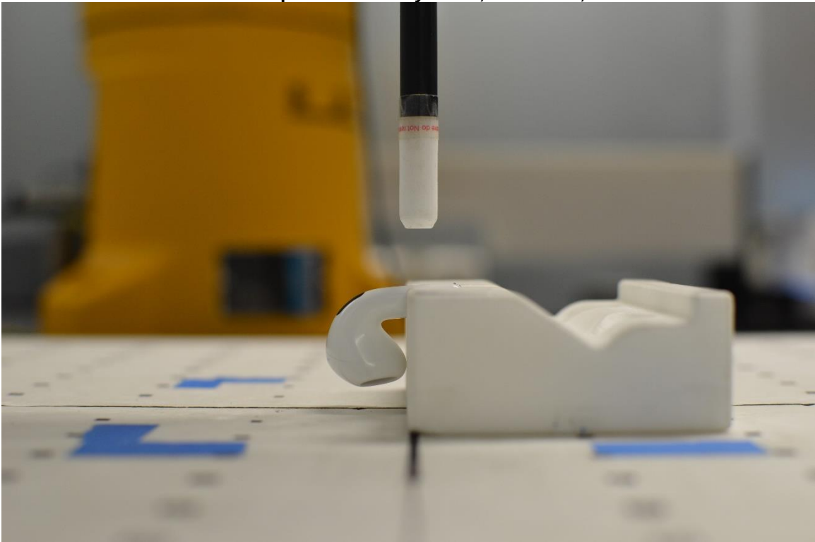
SAR Test Setup Photo 8: Body-Worn, Back Side, 9.45 mm
