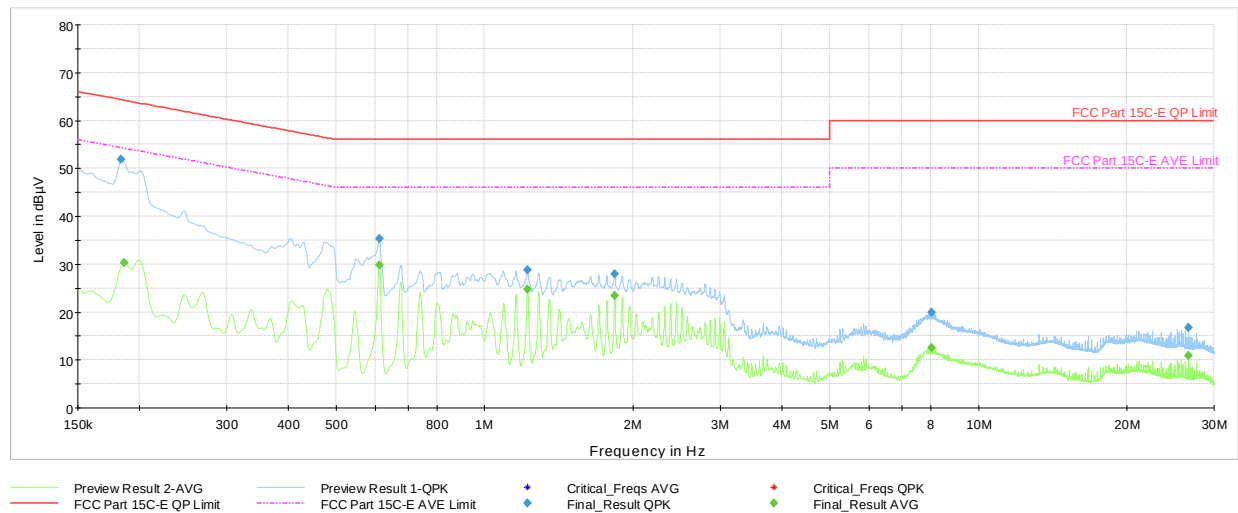
Plot 7-38. AC Line-Conducted Test Plot (L1, GFSK – Ch.78, with host PC and USB-C cable)
