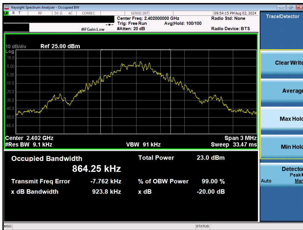
Plot 7-1. 20dB BW and 99% OBW Plot (Bluetooth, GFSK, – Ch. 0)
