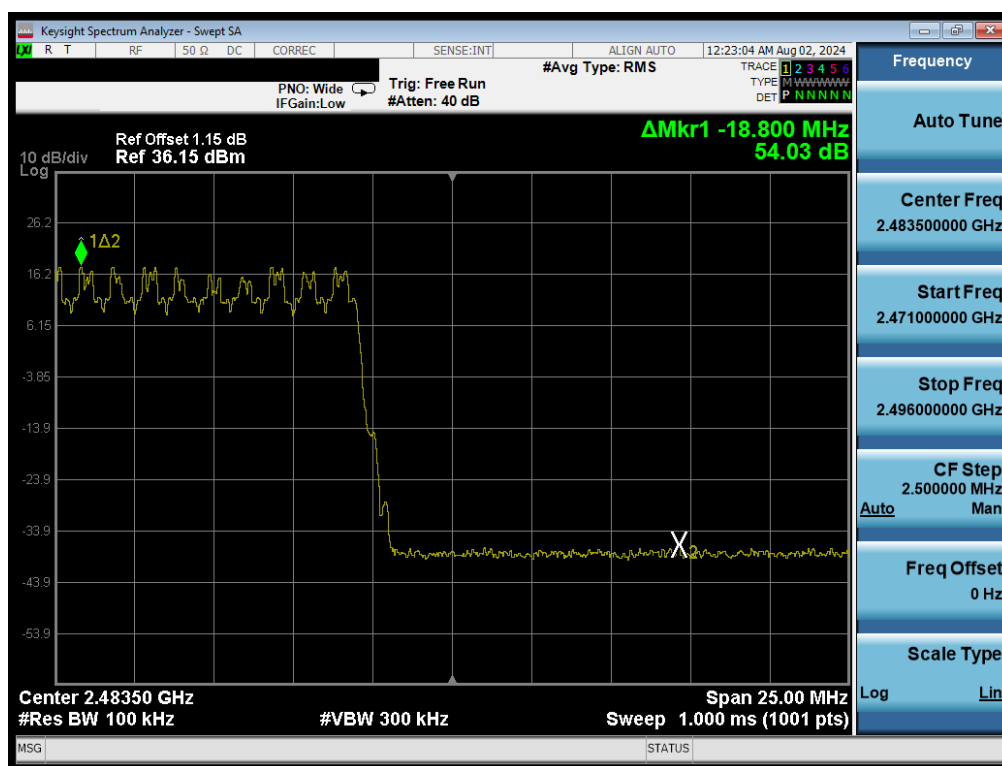
Plot 7-14. Band Edge Plot (Bluetooth with Hopping Enabled, 8DPSK)
