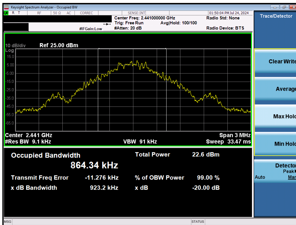
Plot 7-2. 20dB BW and 99% OBW Plot (Bluetooth, GFSK, – Ch. 39)
