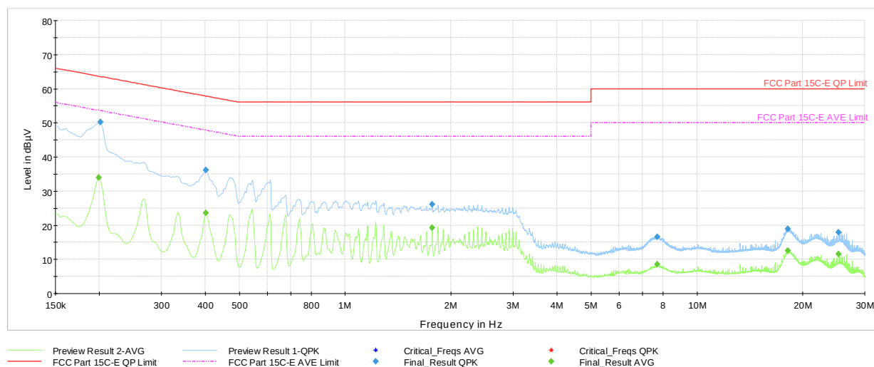
Plot 7-39. AC Line-Conducted Test Plot (N, GFSK – Ch.78, with host PC and USB-C cable)
