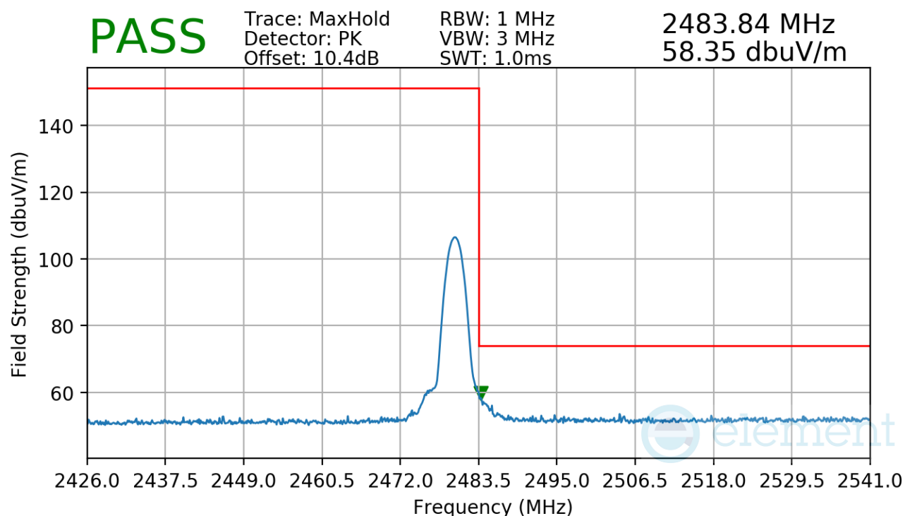
Plot 7-36. Radiated Restricted Upper Band Edge Measurement
