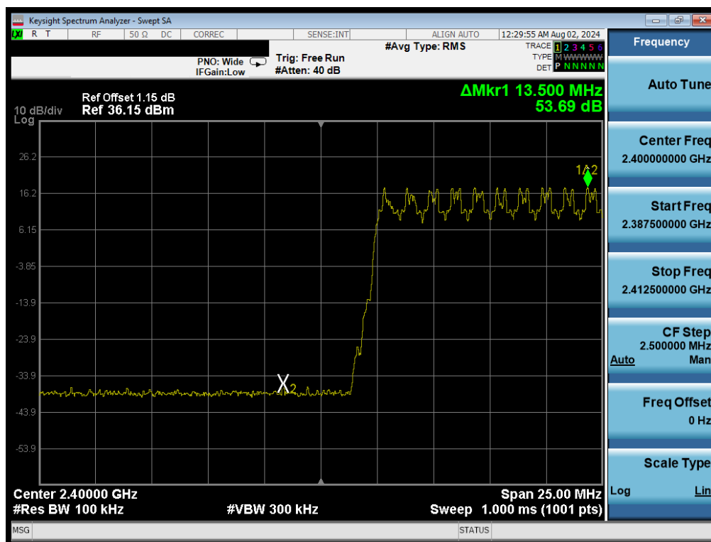
Plot 7-13. Band Edge Plot (Bluetooth with Hopping Enabled, 8DPSK)
