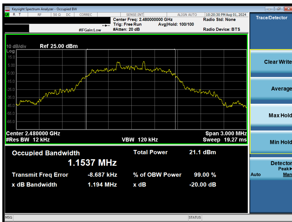
Plot 7-6. 20dB BW and 99% OBW Plot (Bluetooth, 8DPSK – Ch. 78)
