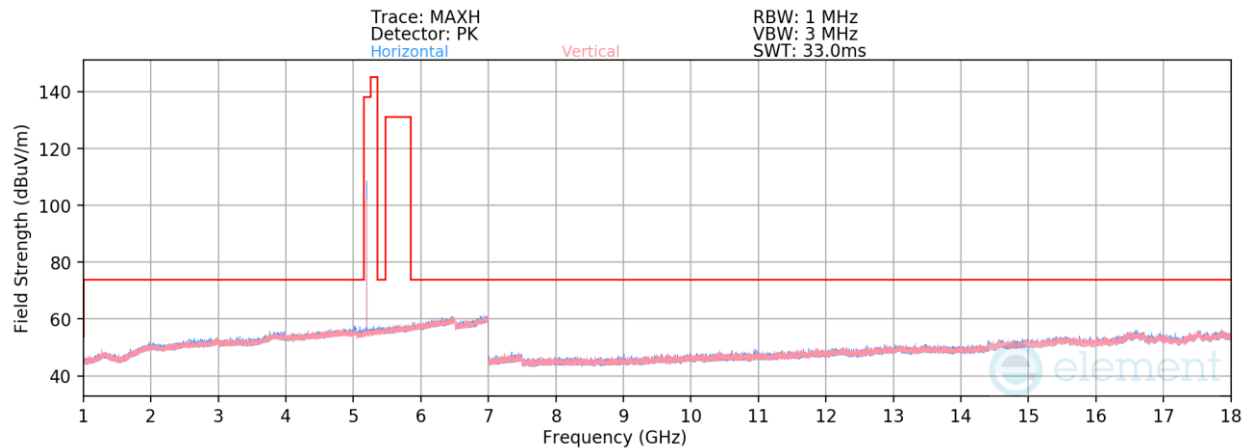
Plot 7-74. Radiated Spurious Emissions 1-18GHz (NB UNII BDR – 5201MHz)
