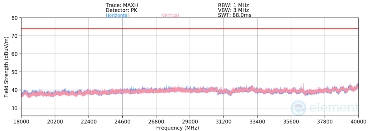
Plot 7-75. Radiated Spurious Emissions 18-40GHz (NB UNII BDR – 2404MHz)
