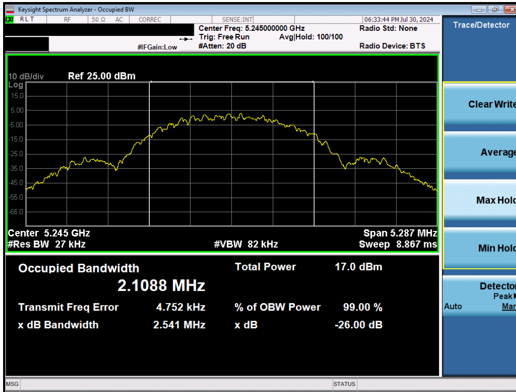
Plot 7-6. 26dB BW & 99% OBW (NB UNII LE2M – 5245MHz)
