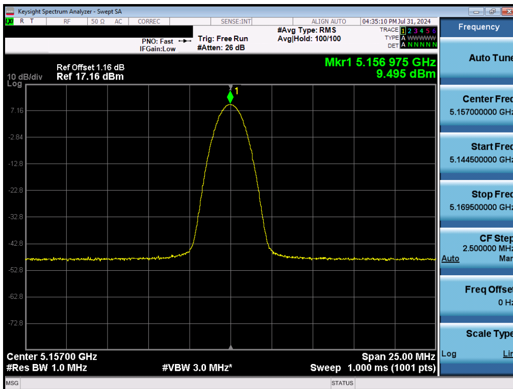
7-37. FCC PSD (NB UNII BDR – 5157MHz)
