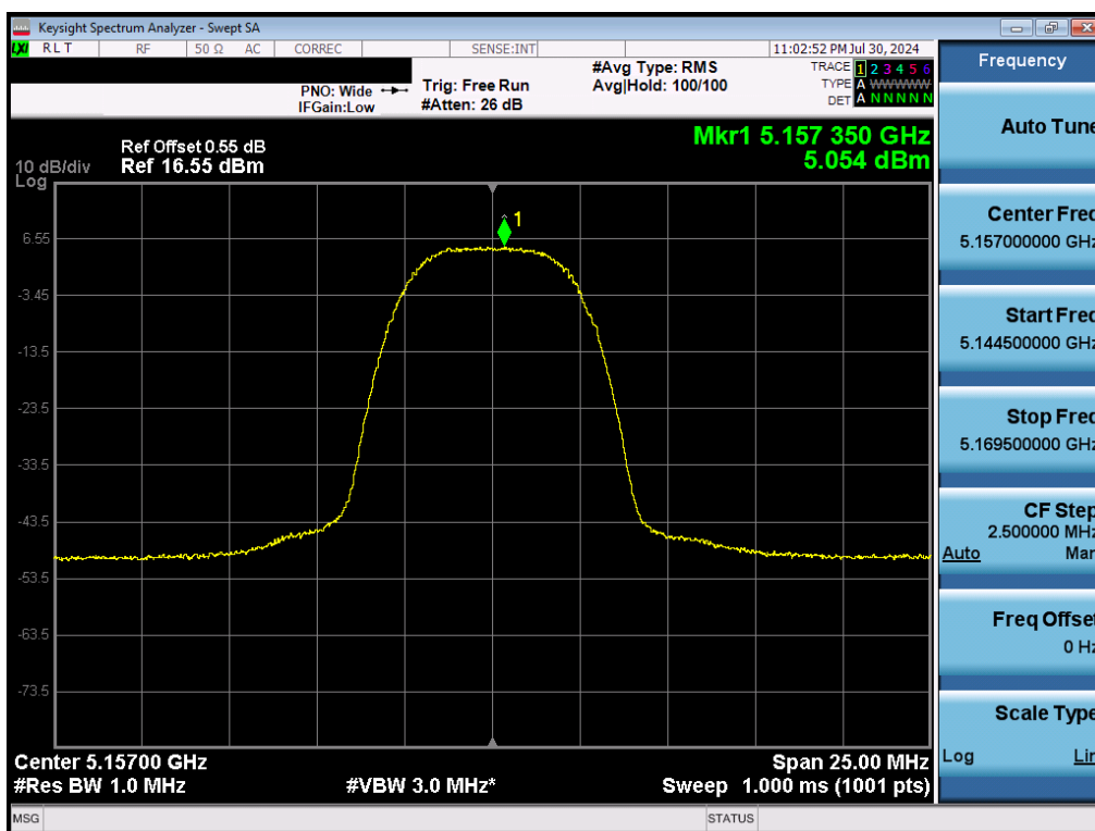
7-52. FCC PSD (NB UNII HDRp8 – 5157MHz)
