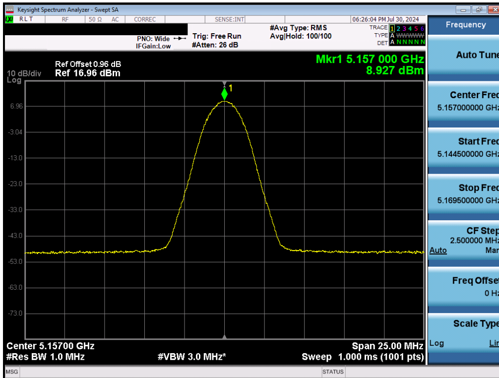
7-40. FCC PSD (NB UNII LE2M – 5157MHz)
