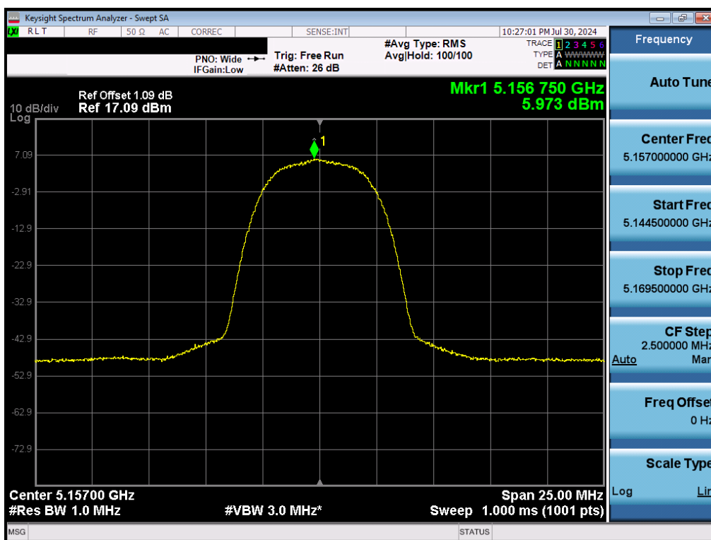
7-46. FCC PSD (NB UNII HDR8 – 5157MHz)
