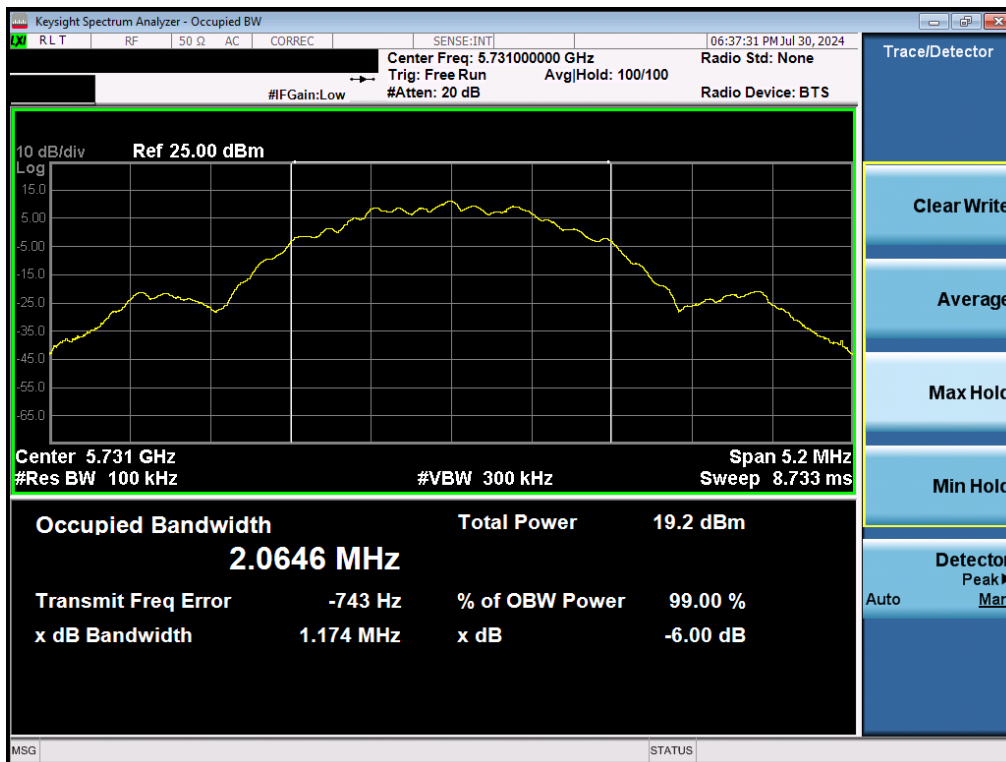
Plot 7-22. 6dB BW & 99% OBW (NB UNII LE2M – 5731MHz)
