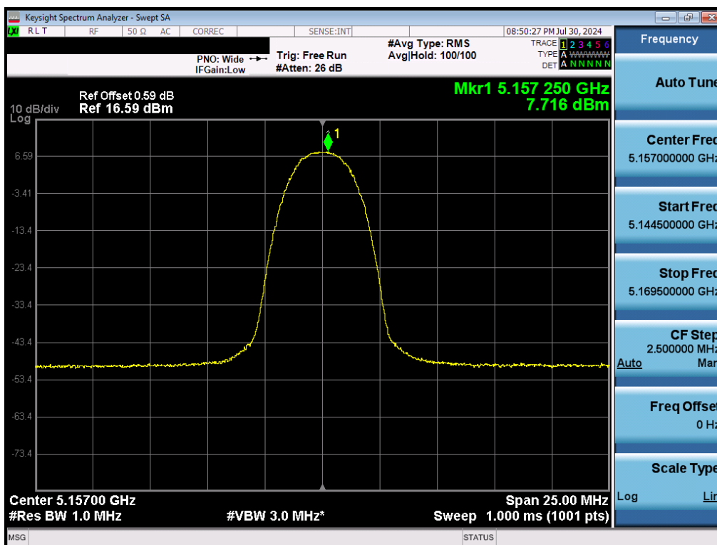
7-49. FCC PSD (NB UNII HDRp4 – 5157MHz)
