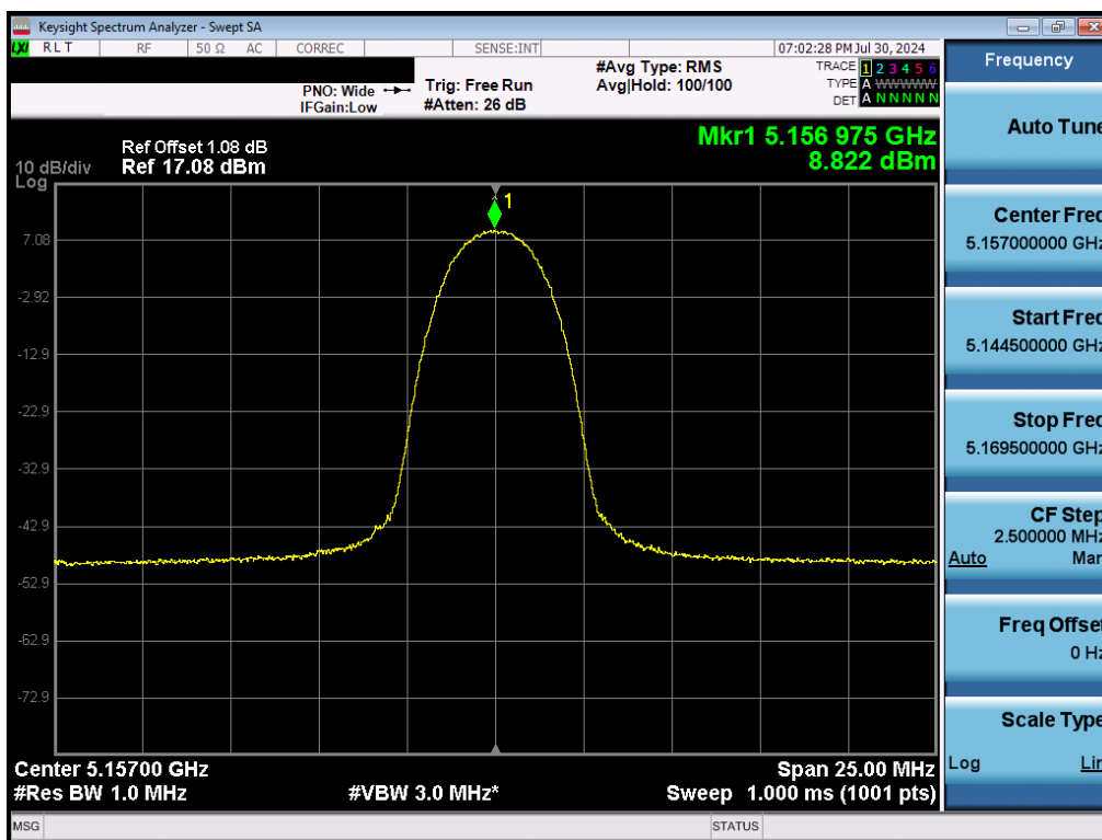
7-43. FCC PSD (NB UNII HDR4 – 5157MHz)
