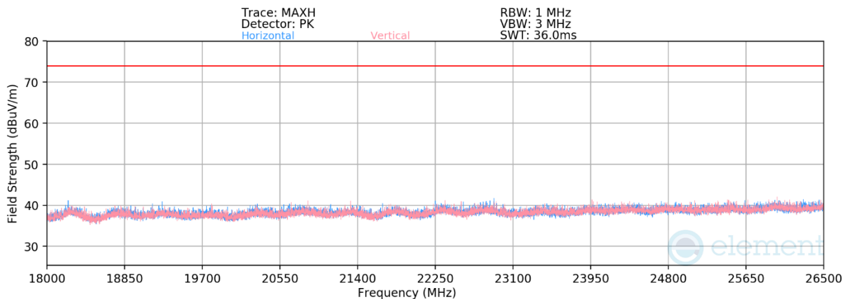
Plot 7-41. Radiated Spurious Emissions Above 18GHz (4Mbps, HDR4, – Ch. 38)
