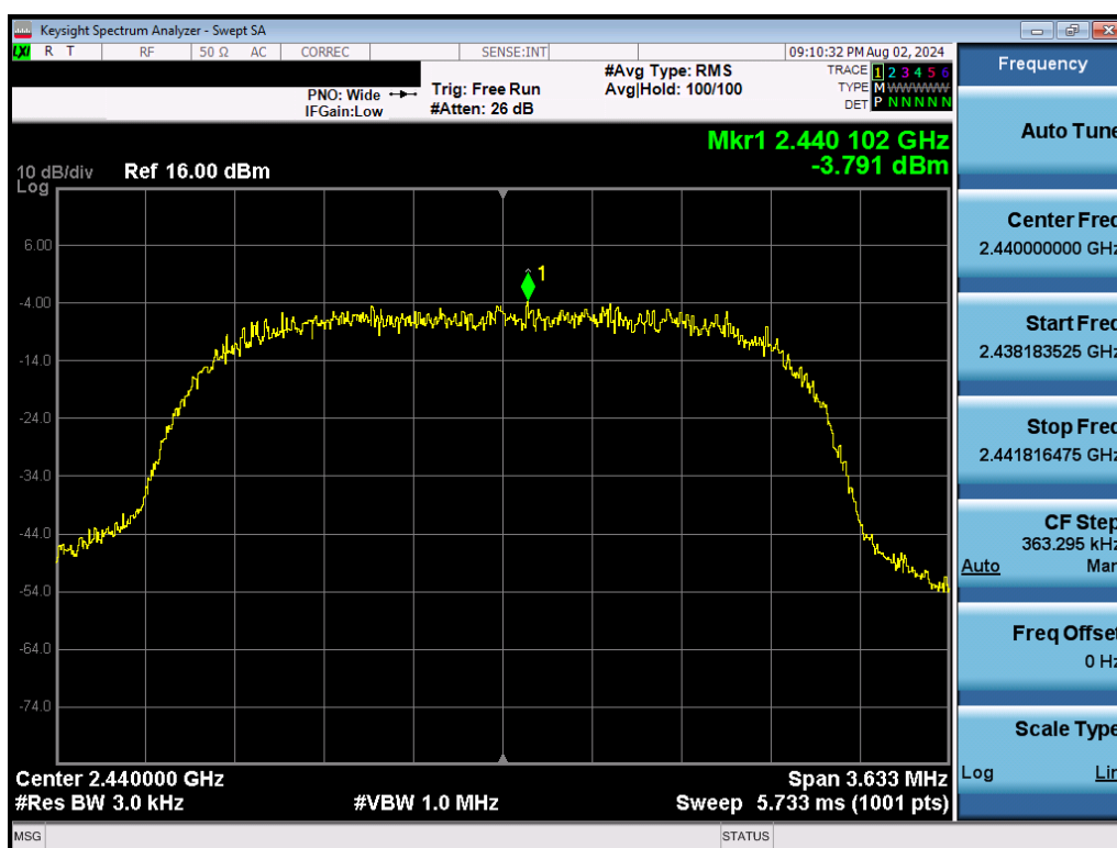
Plot 7-20. Power Spectral Density Plot (Bluetooth (HDRp4), 4Mbps, – Ch. 37)
