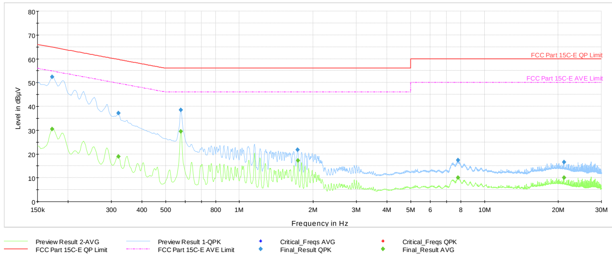
Plot 7-53. AC Line Conducted Plot with Bluetooth HDR (N, 4Mbps - Ch.38 with host PC and USB-C cable))
