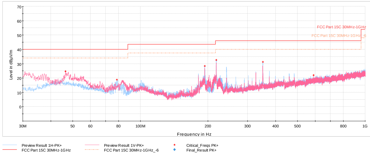
Plot 7-51. Radiated Spurious Emissions Below 1GHz (4Mbps, – Ch.38 with AC/DC Adapter and USB-C cable)
