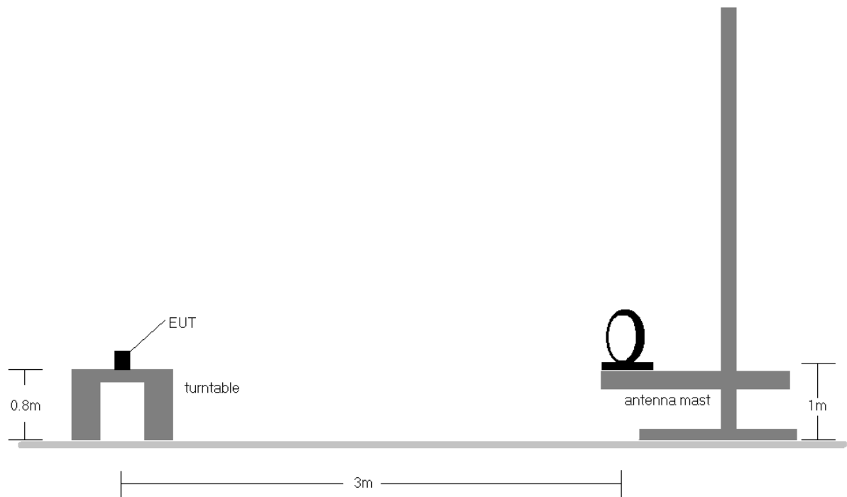
Figure 7-7. Radiated Test Setup < 30MHz
