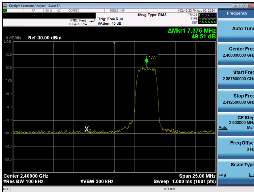
Plot 7-29. Band Edge Plot (Bluetooth (HDRp4), – Ch. 1)
