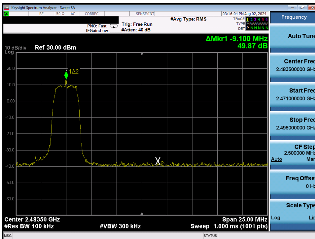
Plot 7-30. Band Edge Plot (Bluetooth (HDRp4), – Ch. 73)
