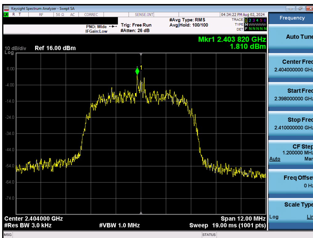
Plot 7-16. Power Spectral Density Plot (Bluetooth (HDR8), 8Mbps, – Ch. 1)
