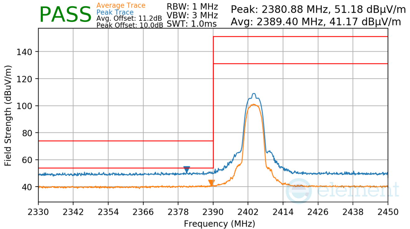
Plot 7-44. Radiated Restricted Lower Band Edge Measurement
