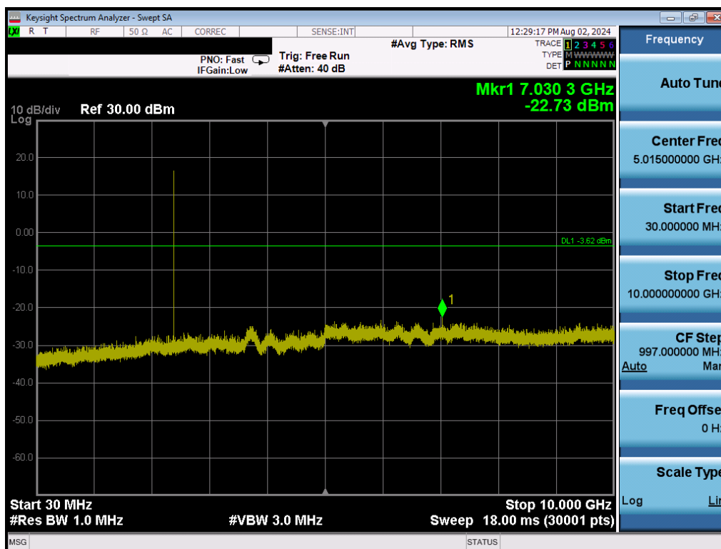
Plot 7-17. Conducted Spurious Plot (Bluetooth (LE), 1Mbps – Ch. 0)
