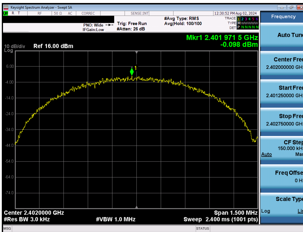
Plot 7-7. Power Spectral Density Plot (Bluetooth (LE), 1Mbps – Ch. 0)
