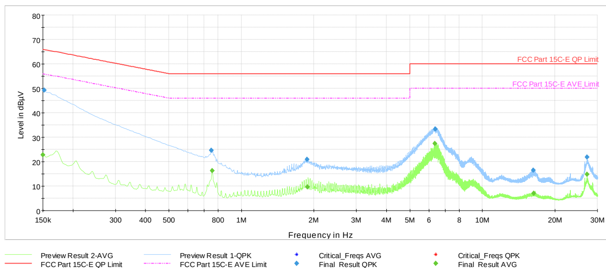
Plot 7-35. AC Line Conducted Plot with Bluetooth LE (L1, 1Mbps – Ch.19 with host PC and USB-C cable)
