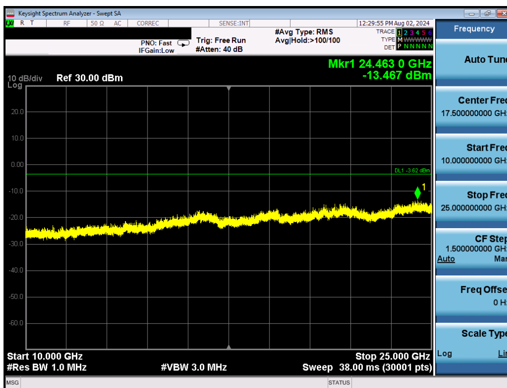
Plot 7-18. Conducted Spurious Plot (Bluetooth (LE), 1Mbps – Ch. 0)
