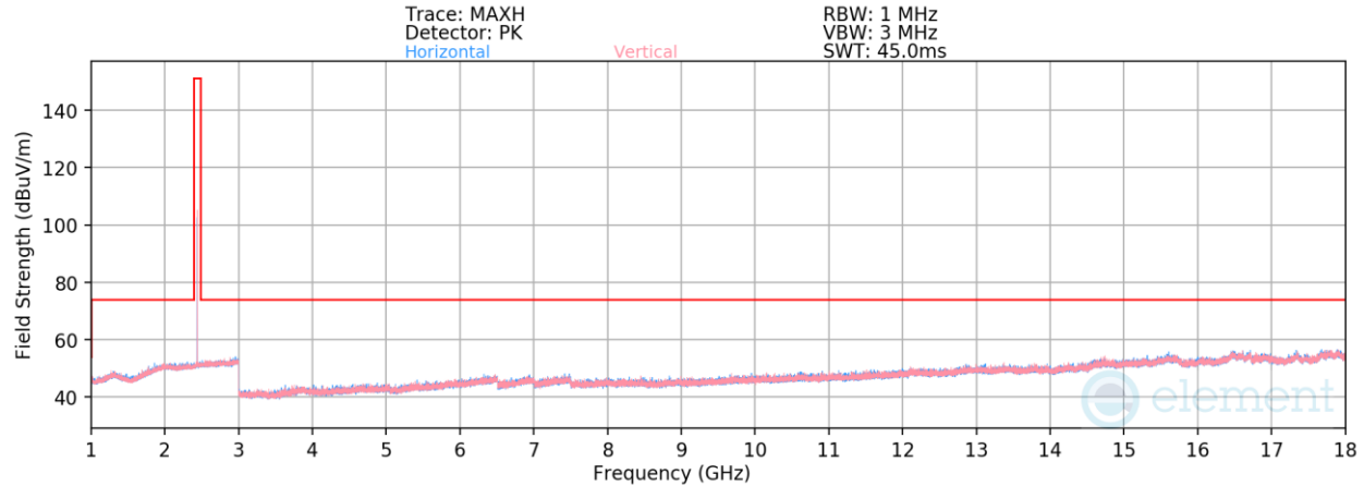
Plot 7-24. Radiated Spurious Emissions 1-18GHz (1Mbps – Ch. 19)
