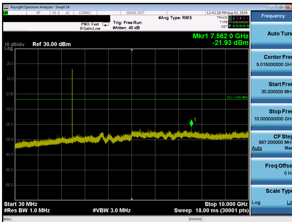
Plot 7-21. Conducted Spurious Plot (Bluetooth (LE), 1Mbps – Ch. 39)
