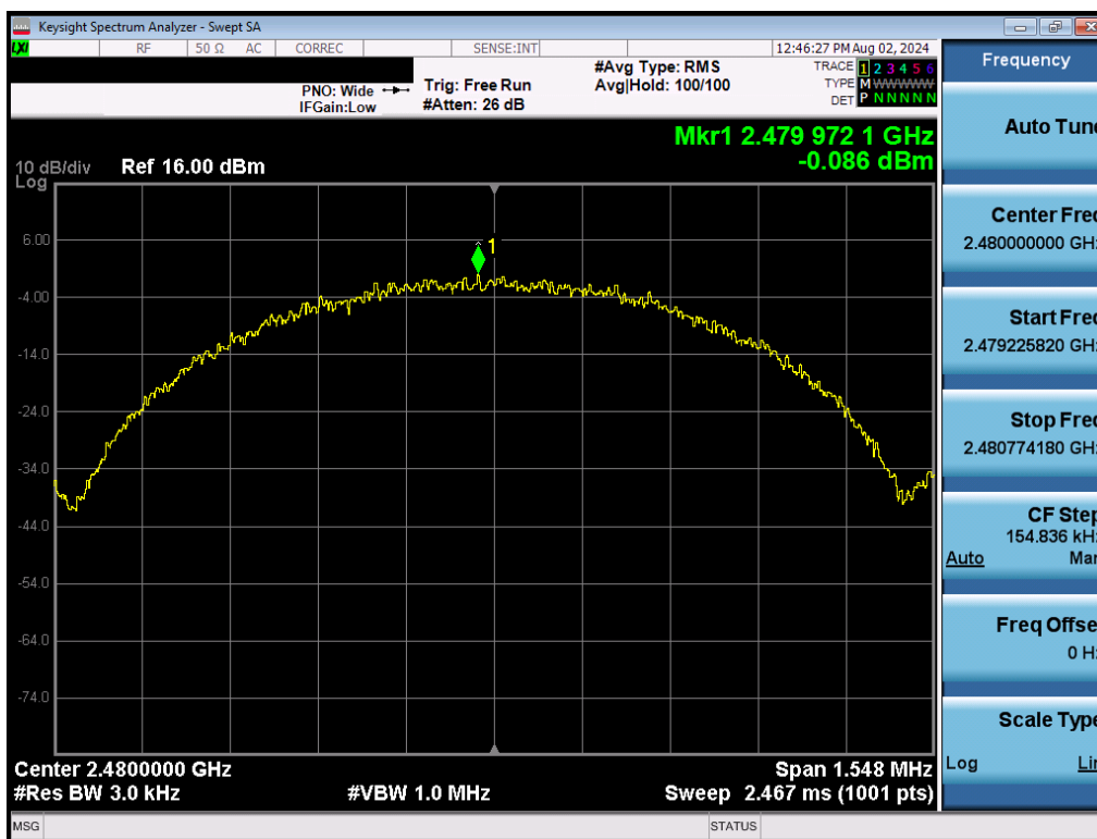
Plot 7-9. Power Spectral Density Plot (Bluetooth (LE), 1Mbps – Ch. 39)
