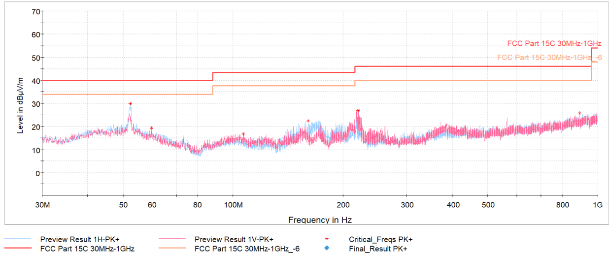
Plot 7-34. Co-Tx Radiated Spurious Emissions Below 1GHz with host PC and USB-C cable
