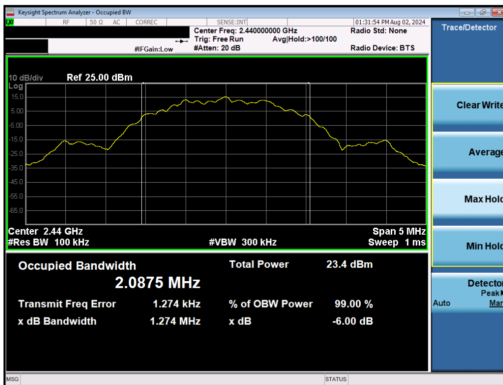
Plot 7-5. 6dB BW & 99% OBW Plot (Bluetooth (LE), 2Mbps – Ch. 19)
