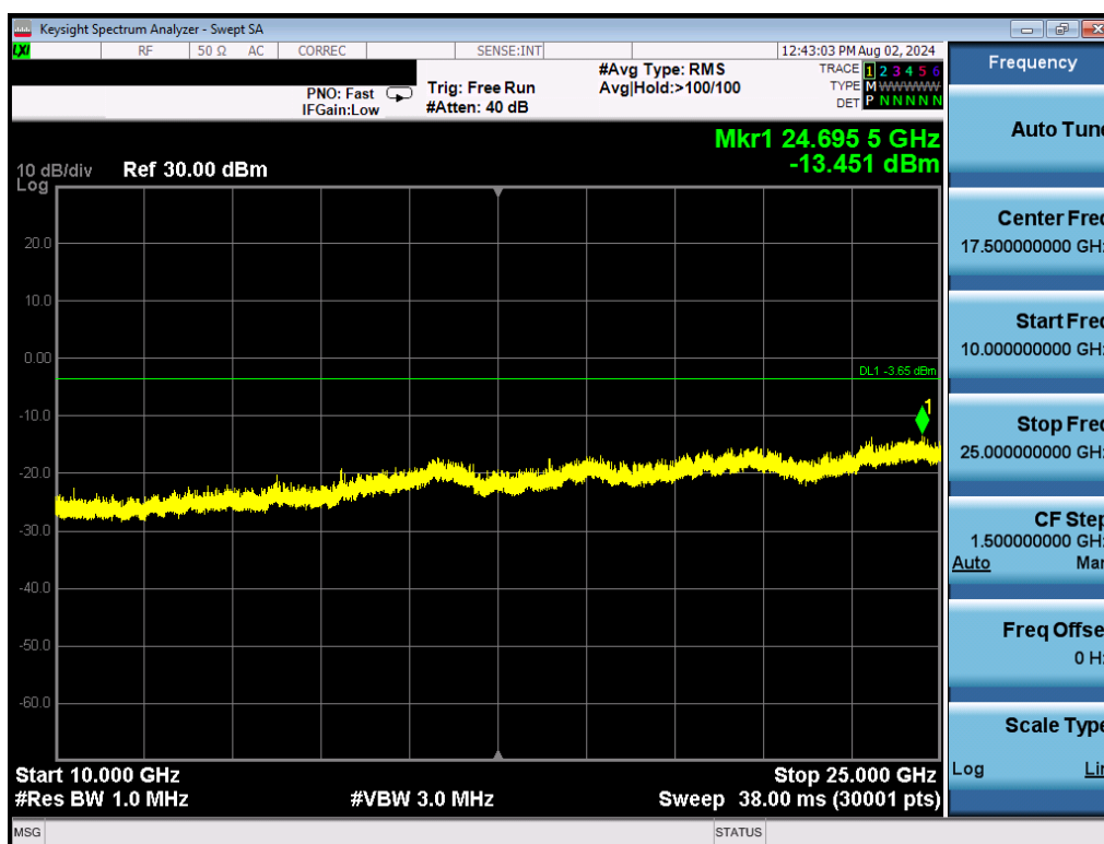
Plot 7-22. Conducted Spurious Plot (Bluetooth (LE), 1Mbps – Ch. 39)
