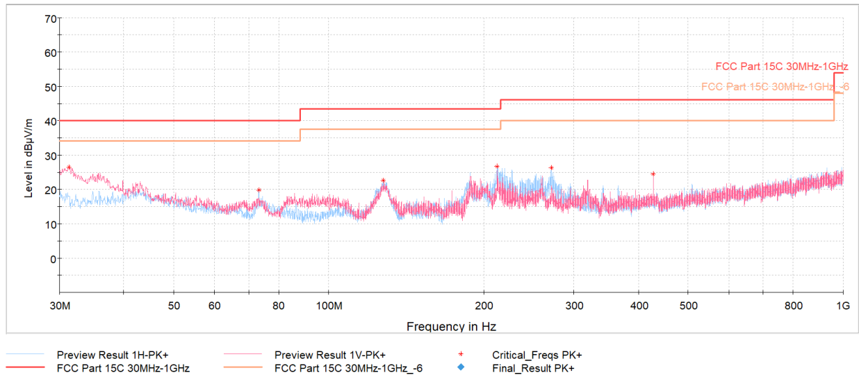
Plot 7-33. Radiated Spurious Emissions Below 1GHz (1Mbps – Ch.19, Pol. H & V, with host PC and USB-C cable)
