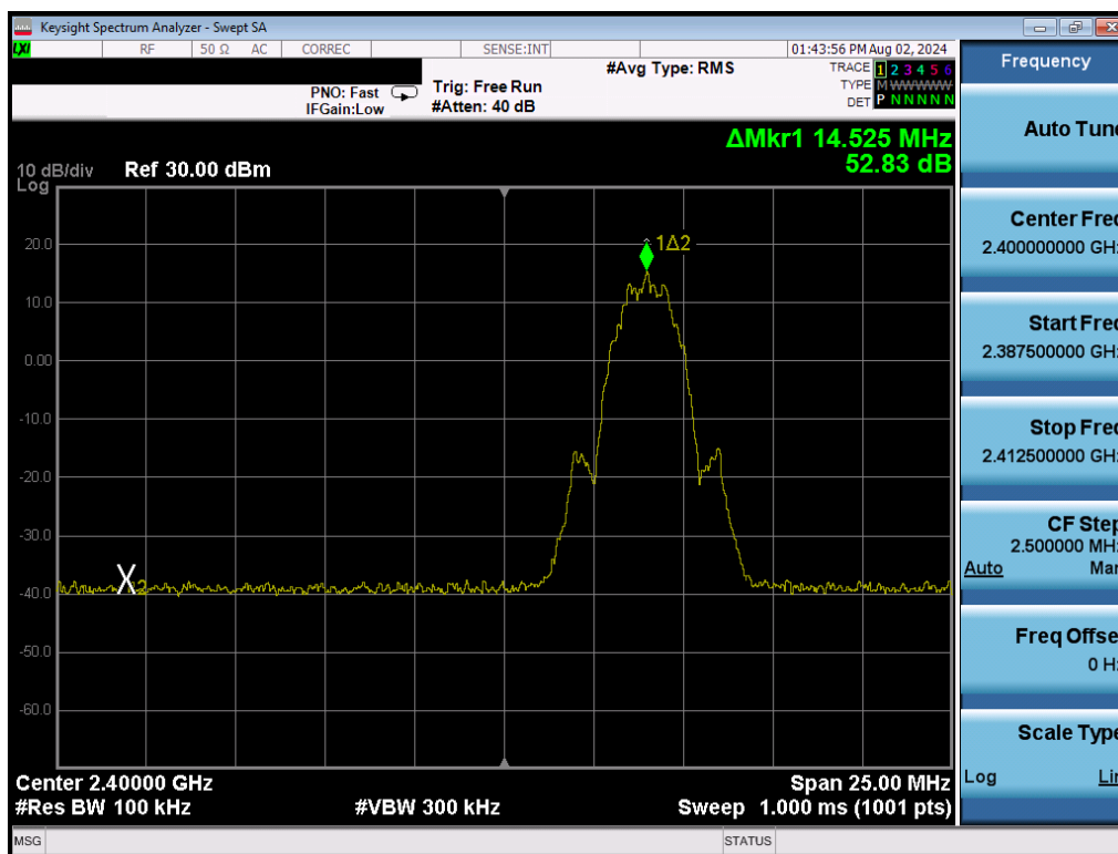
Plot 7-15. Band Edge Plot (Bluetooth (LE), 2Mbps – Ch. 1)
