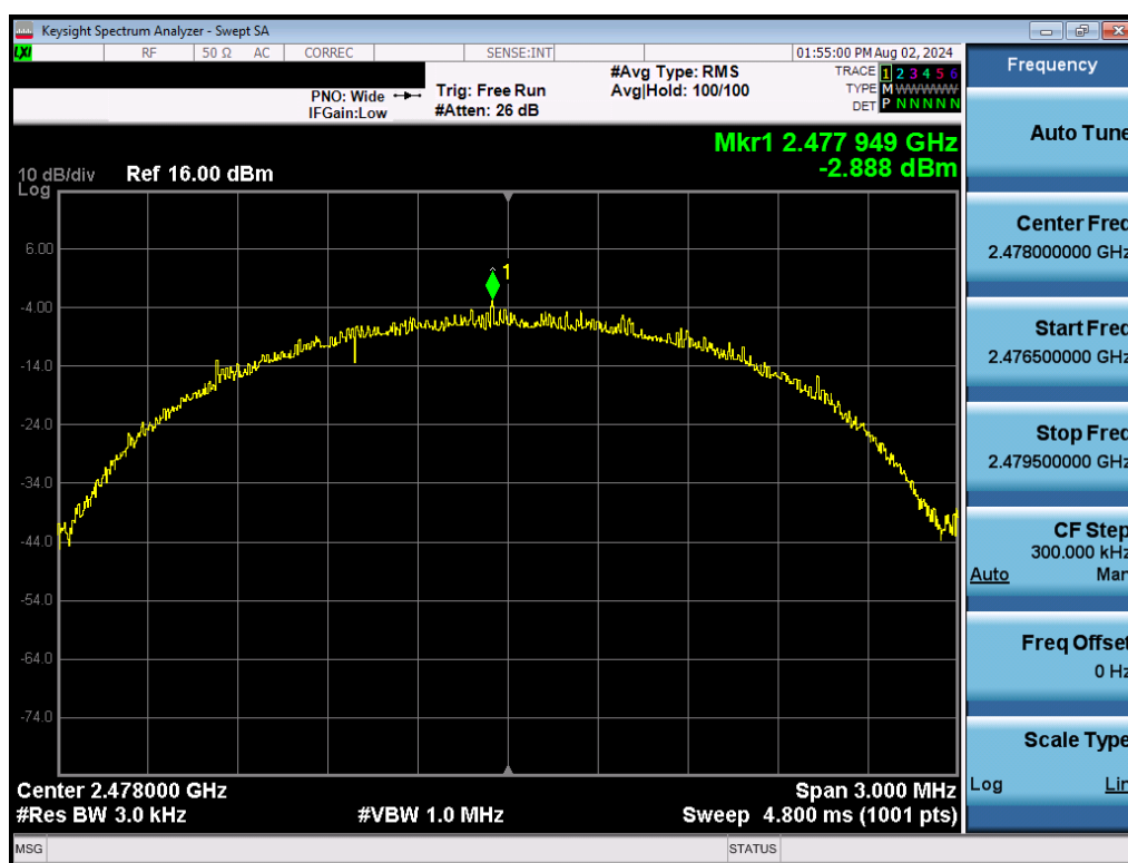
Plot 7-12. Power Spectral Density Plot (Bluetooth (LE), 2Mbps – Ch. 38)
