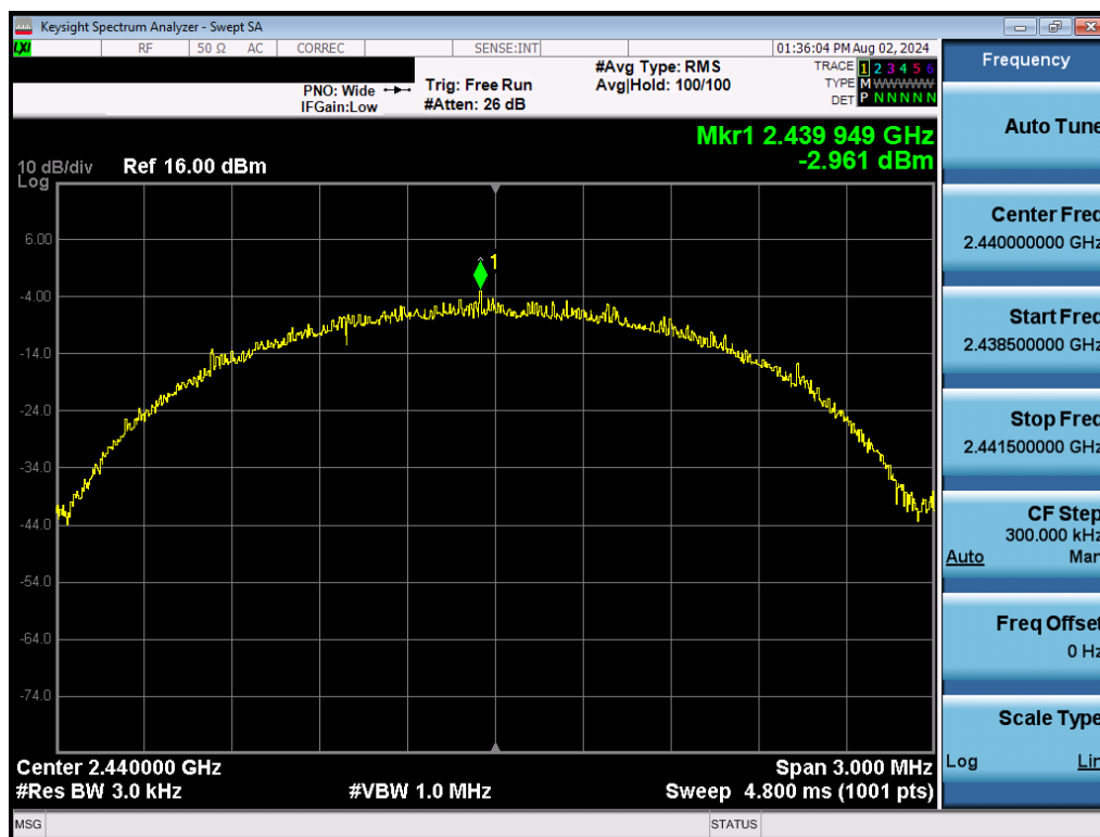
Plot 7-11. Power Spectral Density Plot (Bluetooth (LE), 2Mbps – Ch. 19)
