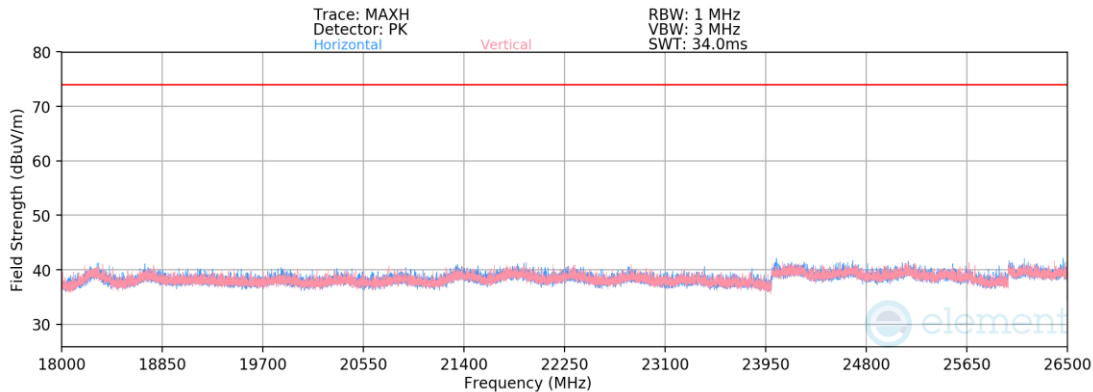
Plot 7-28. Radiated Spurious Emissions – Cot-Tx Above 18GHz
