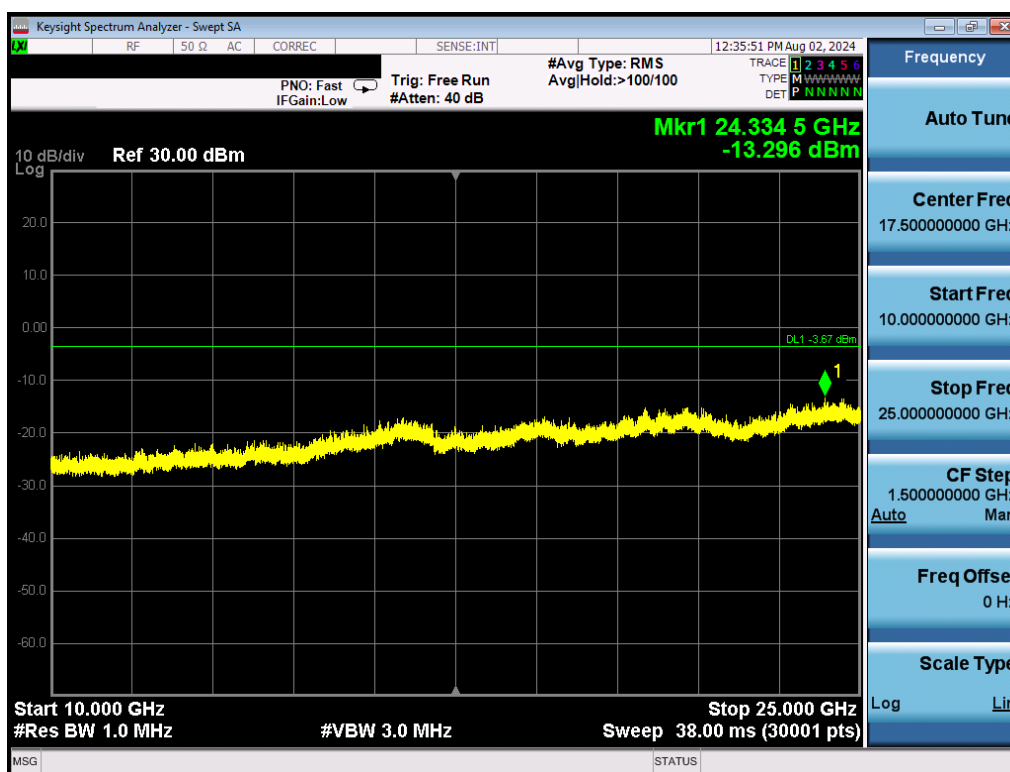
Plot 7-20. Conducted Spurious Plot (Bluetooth (LE), 1Mbps – Ch. 19)
