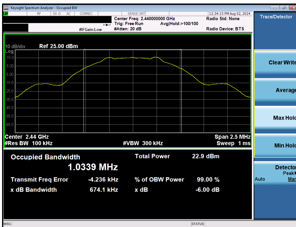
Plot 7-2. 6dB BW & 99% OBW Plot (Bluetooth (LE), 1Mbps – Ch. 19)
