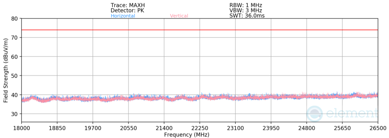
Plot 7-25. Radiated Spurious Emissions Above 18GHz (1Mbps – Ch. 19)
