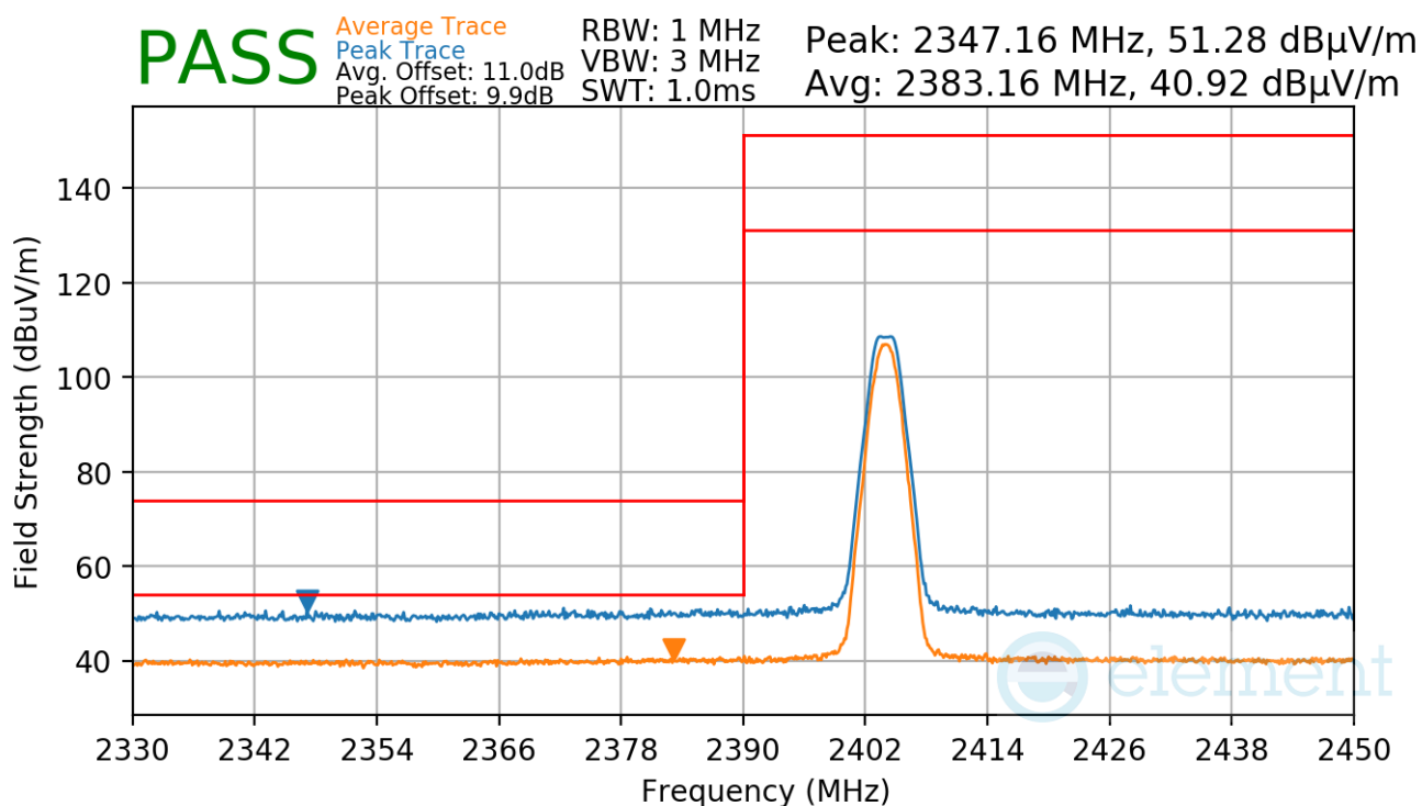
Plot 7-31. Radiated Restricted Lower Band Edge Measurement (Average & Peak)
