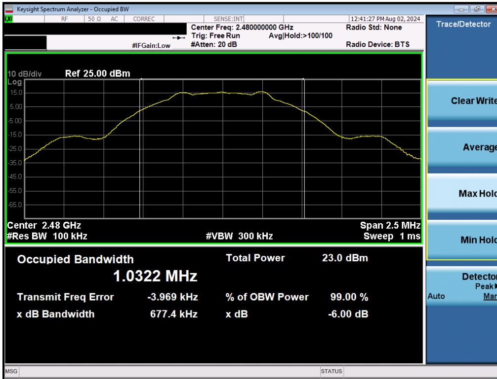
Plot 7-3. 6dB BW & 99% OBW Plot (Bluetooth (LE), 1Mbps – Ch. 39)
