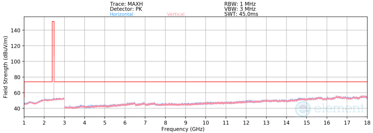
Plot 7-26. Radiated Spurious Emissions 1-18GHz (1Mbps – Ch. 39)
