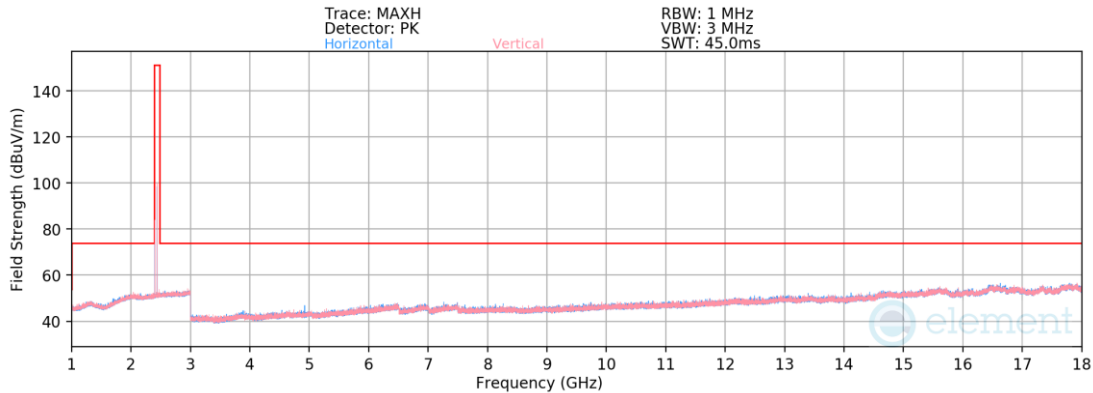
Plot 7-27. Radiated Spurious Emissions – Cot-Tx 1-18GHz
