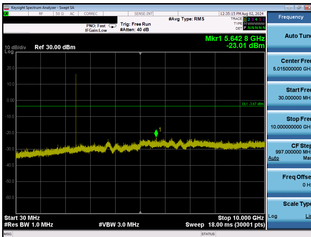
Plot 7-19. Conducted Spurious Plot (Bluetooth (LE), 1Mbps – Ch. 19)
