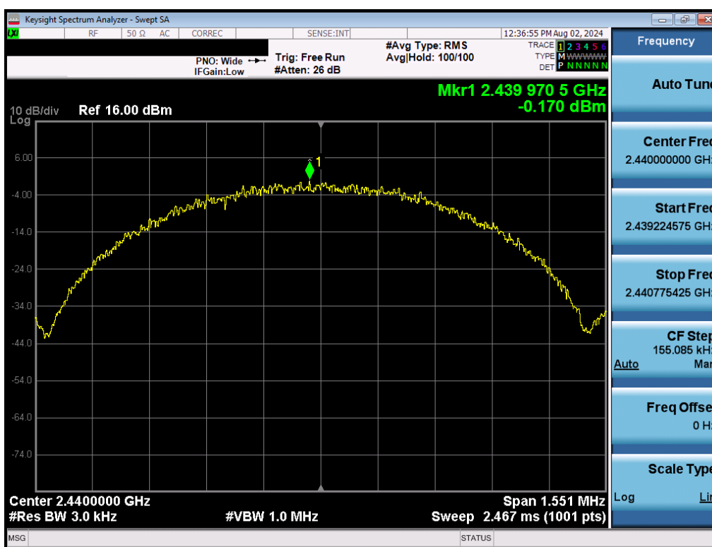
Plot 7-8. Power Spectral Density Plot (Bluetooth (LE), 1Mbps – Ch. 19)
