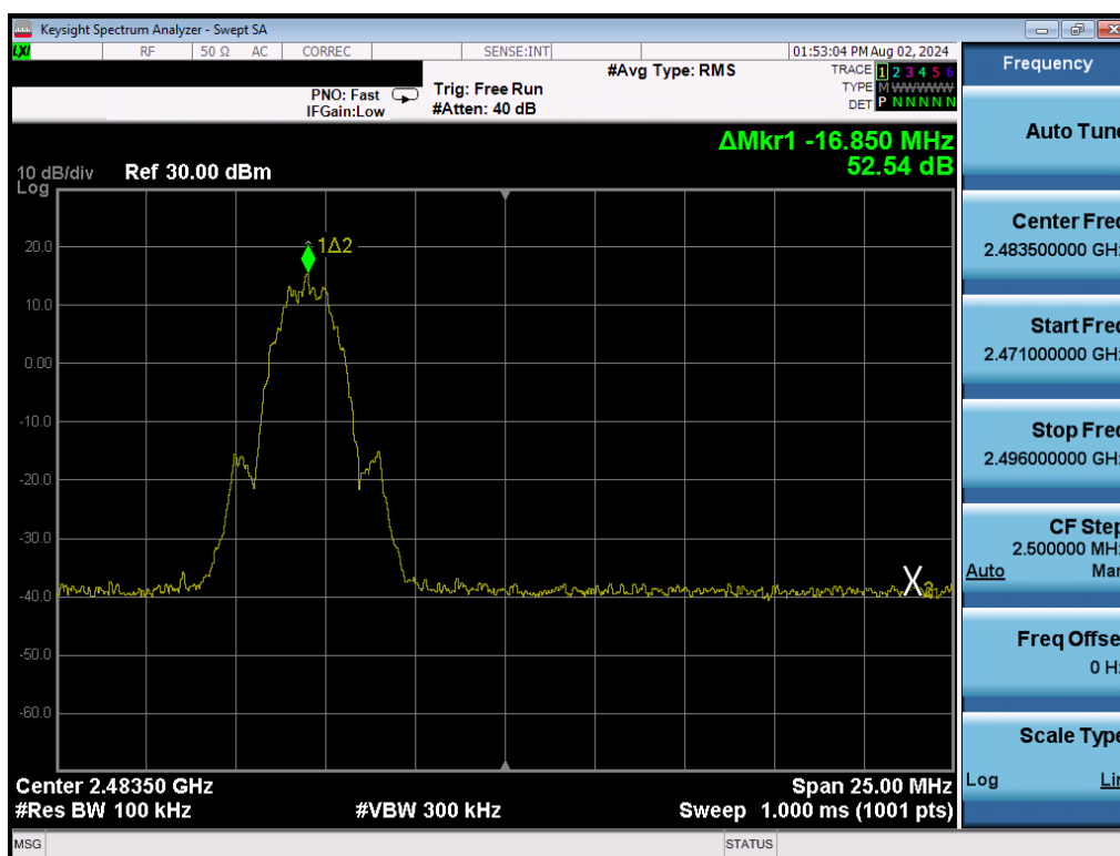
Plot 7-16. Band Edge Plot (Bluetooth (LE), 2Mbps – Ch. 38)
