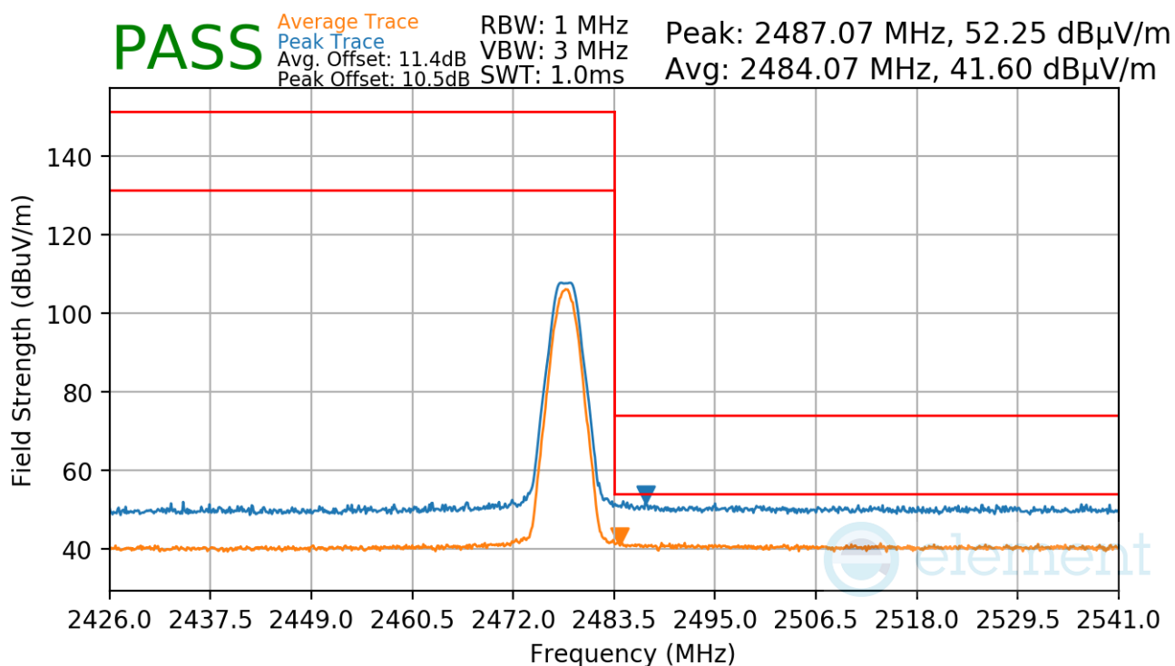
Plot 7-32. Radiated Restricted Upper Band Edge Measurement (Average & Peak)
